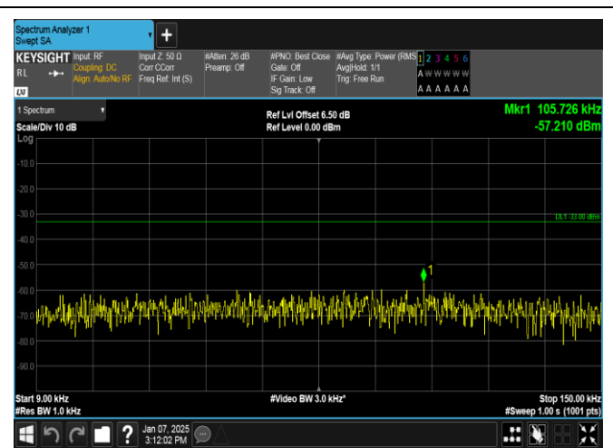
Band12-3MHz-QPSK-23095-1RB#0-0.009~0.15-PASS
