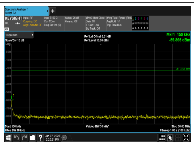
Band12-1.4MHz-16QAM-23017-1RB#5-0.15~30-PASS
