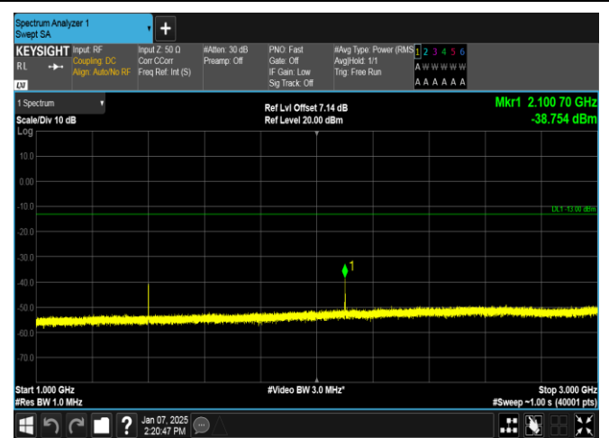
Band12-1.4MHz-16QAM-23017-1RB#5-1000~3000-PASS
