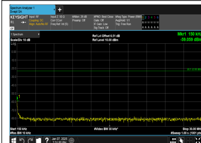
Band12-1.4MHz-QPSK-23173-1RB#5-0.15~30-PASS
