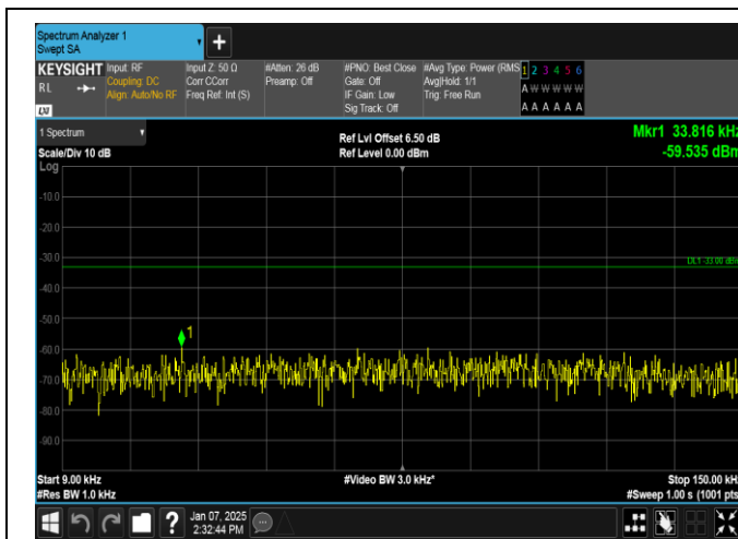
Band12-1.4MHz-16QAM-23173-1RB#5-0.009~0.15-PASS
