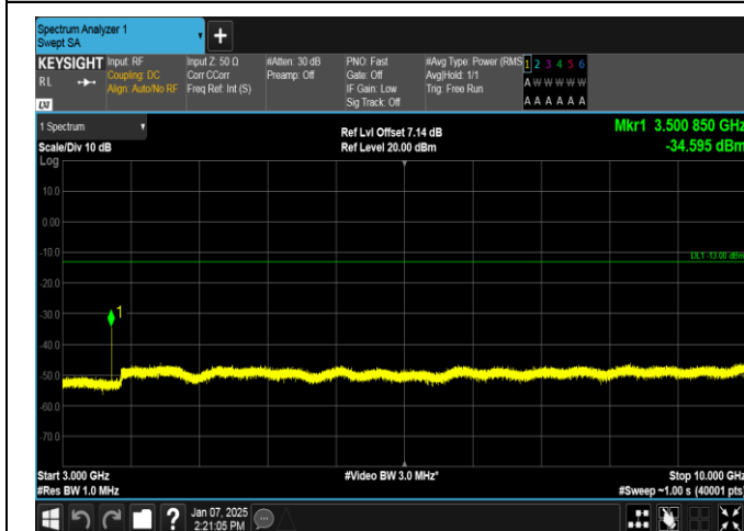
Band12-1.4MHz-16QAM-23017-1RB#5-3000~10000-PASS
