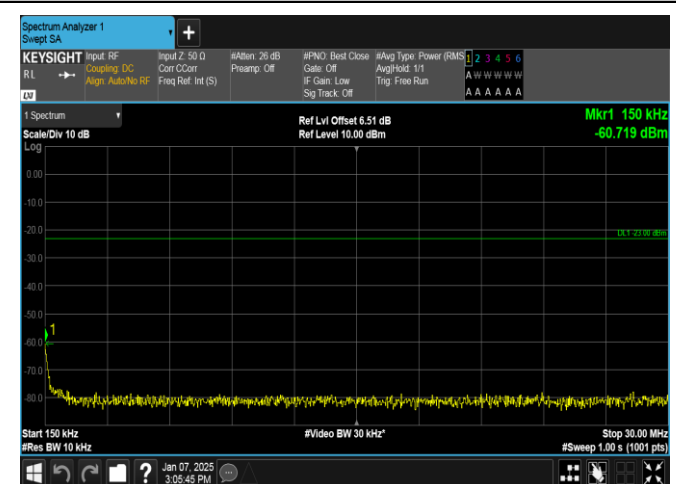
Band12-3MHz-QPSK-23025-1RB#0-0.15~30-PASS
