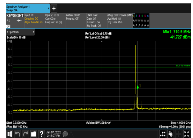
Band12-1.4MHz-16QAM-23017-1RB#0-30~1000-PASS
