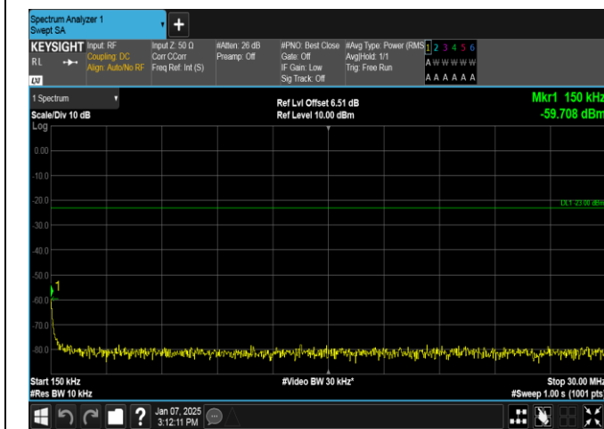
Band12-3MHz-QPSK-23095-1RB#0-0.15~30-PASS
