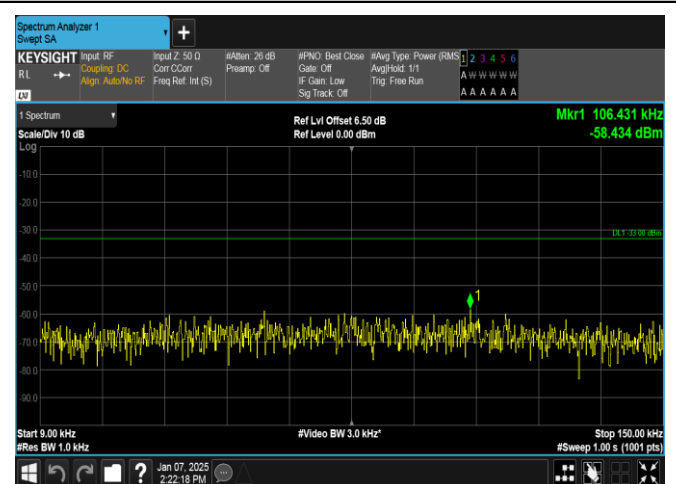
Band12-1.4MHz-16QAM-23017-6RB#0-0.009~0.15-PASS
