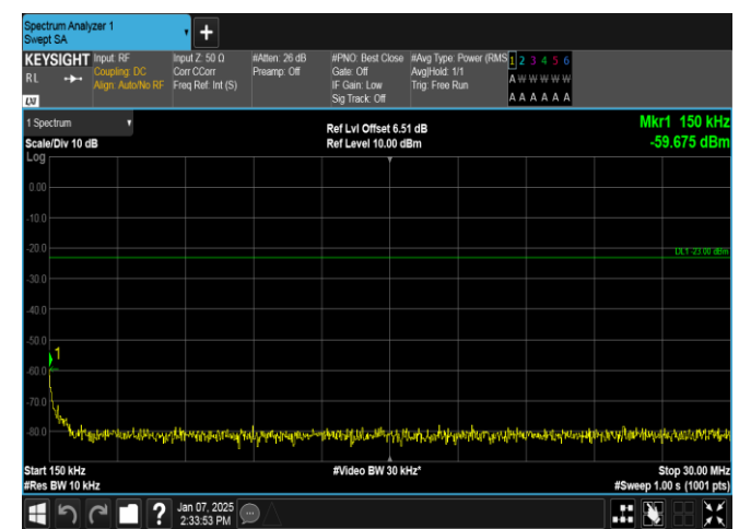
Band12-1.4MHz-QPSK-23173-6RB#0-0.15~30-PASS
