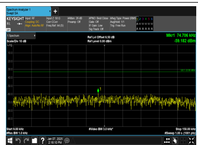
Band12-1.4MHz-16QAM-23017-1RB#0-0.009~0.15-PASS
