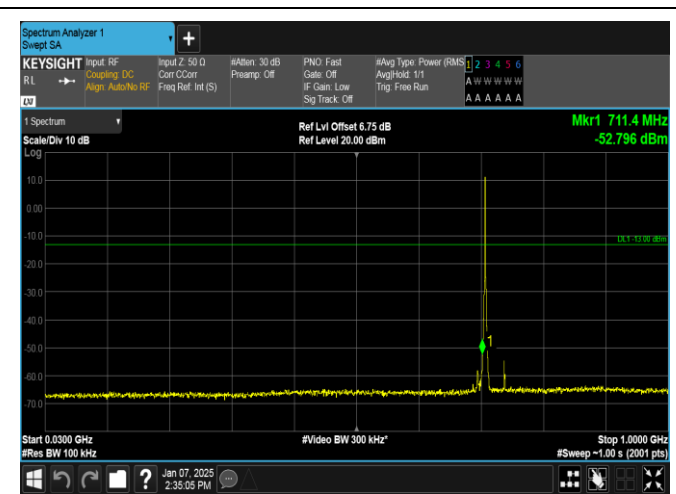
Band12-1.4MHz-16QAM-23173-6RB#0-30~1000-PASS
