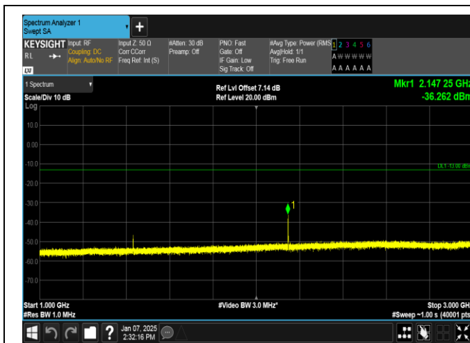
Band12-1.4MHz-QPSK-23173-1RB#5-1000~3000-PASS
