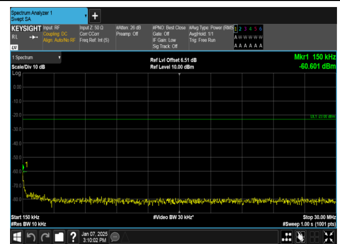
Band12-3MHz-QPSK-23025-15RB#0-0.15~30-PASS
