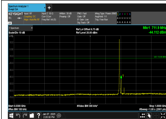
Band12-1.4MHz-16QAM-23017-1RB#5-30~1000-PASS
