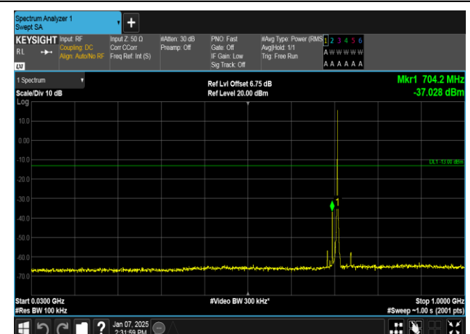
Band12-1.4MHz-QPSK-23173-1RB#5-30~1000-PASS
