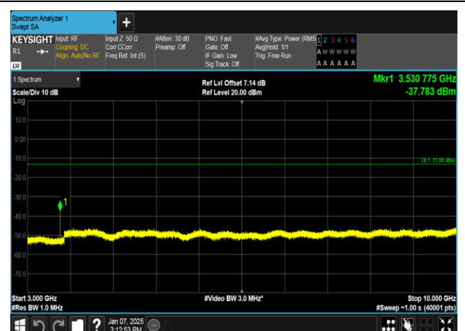
Band12-3MHz-QPSK-23095-1RB#0-3000~10000-PASS
