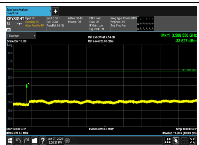
Band12-3MHz-QPSK-23025-1RB#14-3000~10000-PASS
