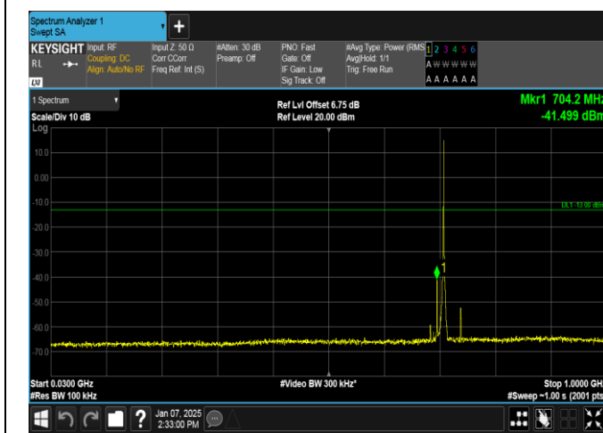
Band12-1.4MHz-16QAM-23173-1RB#5-30~1000-PASS
