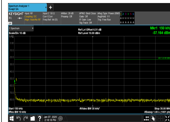
Band12-1.4MHz-16QAM-23017-1RB#0-0.15~30-PASS
