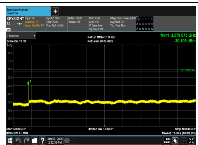
Band12-1.4MHz-QPSK-23173-1RB#5-3000~10000-PASS
