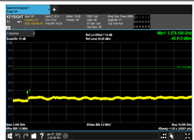
Band12-1.4MHz-16QAM-23173-6RB#0-3000~10000-PASS
