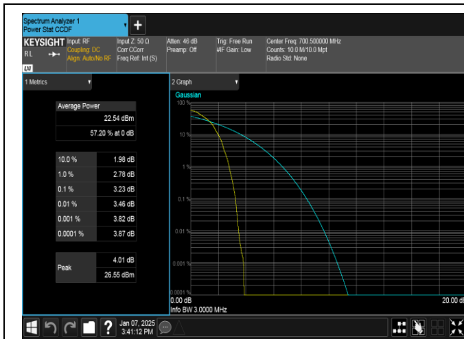
Band12-3MHz-QPSK-23025-1RB#0-PASS
