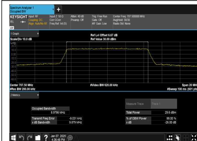
Band12-10MHz-16QAM-23095-50RB#0-PASS
