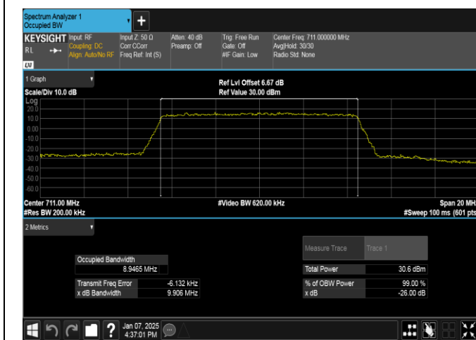
Band12-10MHz-QPSK-23130-50RB#0-PASS
