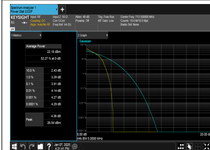
Band12-5MHz-QPSK-23155-1RB#0-PASS
