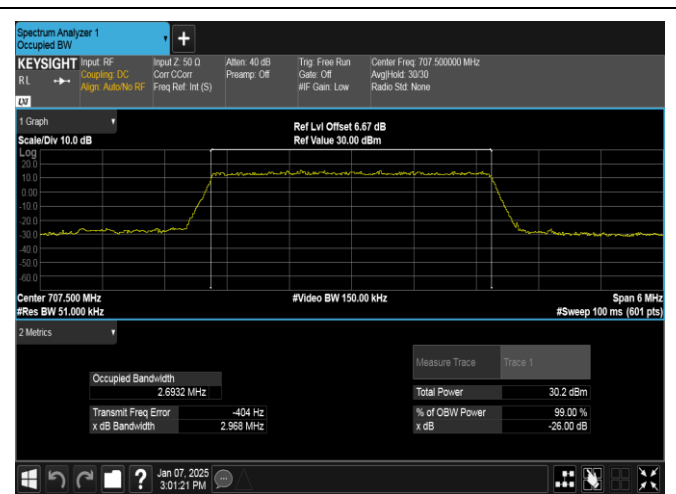
Band12-3MHz-QPSK-23095-15RB#0-PASS
