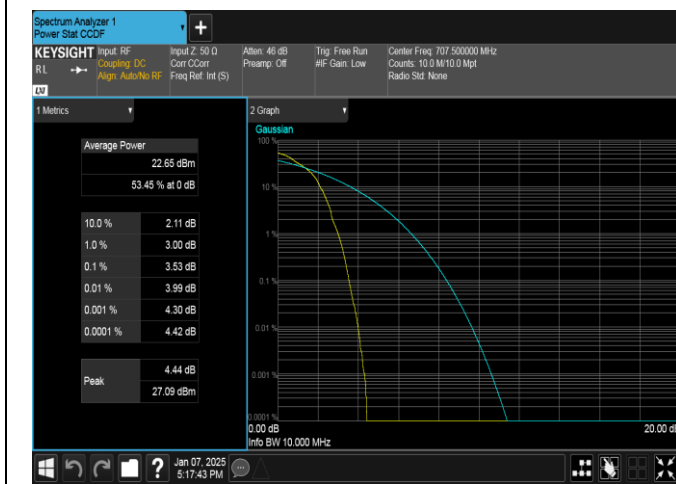
Band12-10MHz-QPSK-23095-1RB#0-PASS
