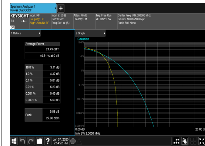
Band12-1.4MHz-16QAM-23095-1RB#0-PASS
