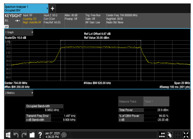
Band12-10MHz-16QAM-23060-50RB#0-PASS
