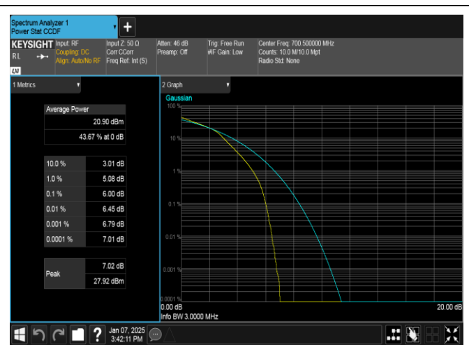
Band12-3MHz-16QAM-23025-15RB#0-PASS
