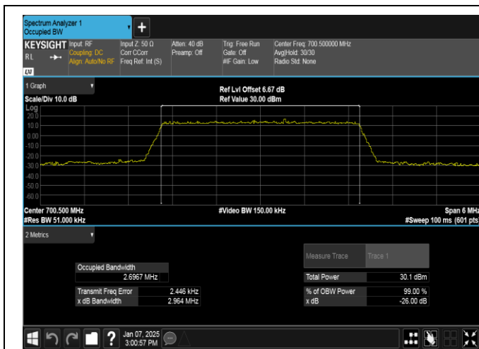
Band12-3MHz-QPSK-23025-15RB#0-PASS
