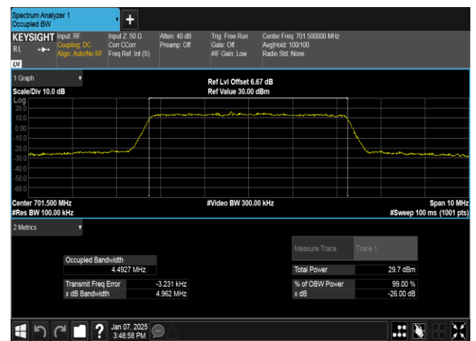
Band12-5MHz-16QAM-23035-25RB#0-PASS
