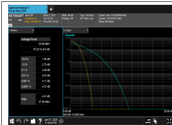
Band12-10MHz-QPSK-23060-1RB#0-PASS
