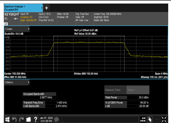
Band12-3MHz-16QAM-23025-15RB#0-PASS
