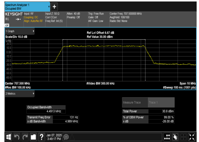
Band12-5MHz-QPSK-23095-25RB#0-PASS
