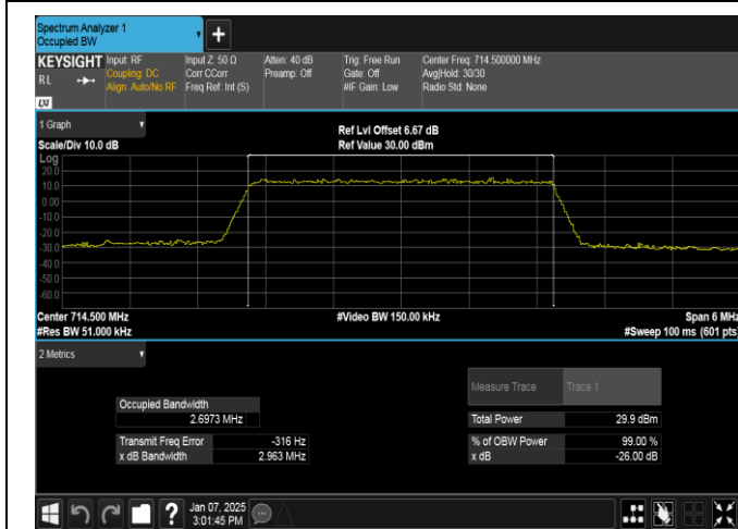
Band12-3MHz-QPSK-23165-15RB#0-PASS
