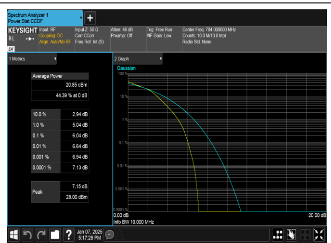
Band12-10MHz-16QAM-23060-50RB#0-PASS
