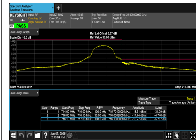
Band12-1.4MHz-QPSK-23173-1RB#5-PASS
