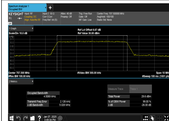
Band12-5MHz-16QAM-23095-25RB#0-PASS
