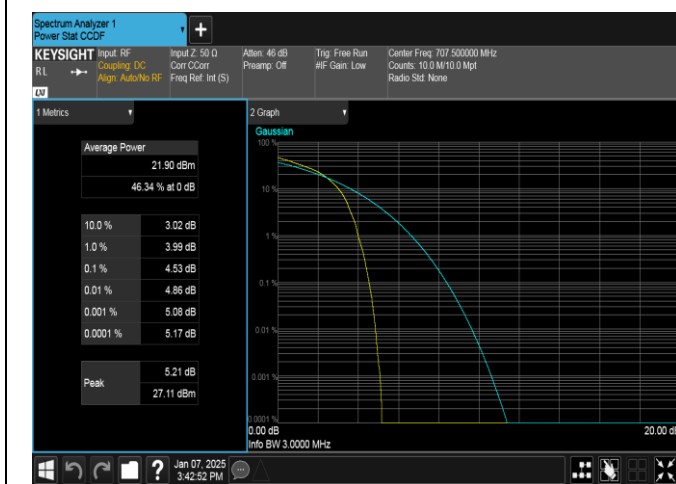
Band12-3MHz-16QAM-23095-1RB#0-PASS
