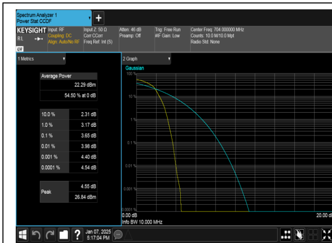
Band12-10MHz-16QAM-23060-1RB#0-PASS
