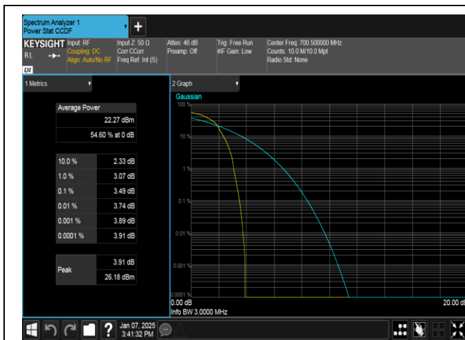
Band12-3MHz-16QAM-23025-1RB#0-PASS
