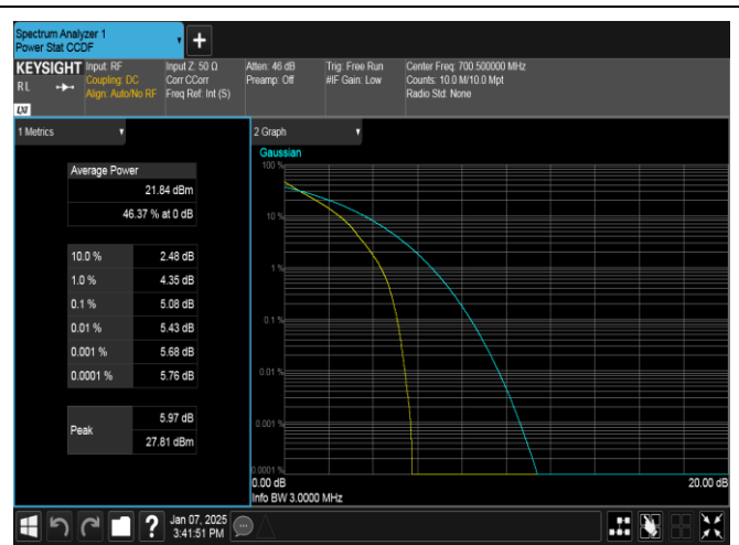
Band12-3MHz-QPSK-23025-15RB#0-PASS
