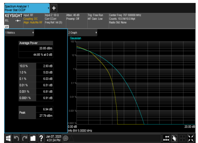
Band12-5MHz-16QAM-23095-25RB#0-PASS
