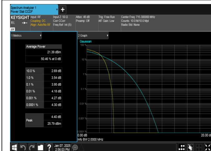
Band12-1.4MHz-16QAM-23173-1RB#0-PASS
