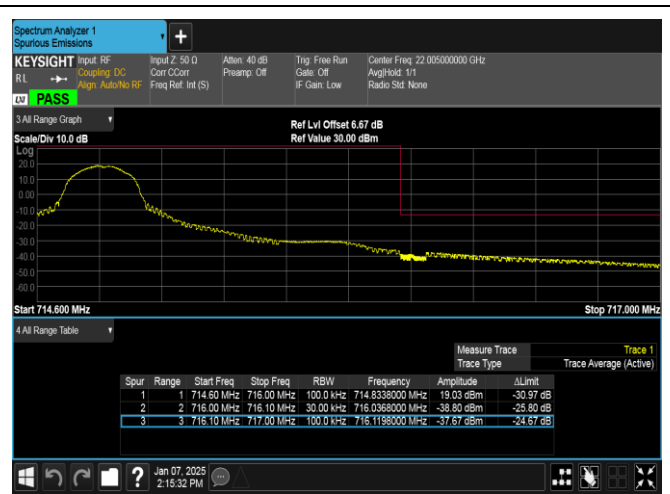
Band12-1.4MHz-QPSK-23173-1RB#0-PASS
