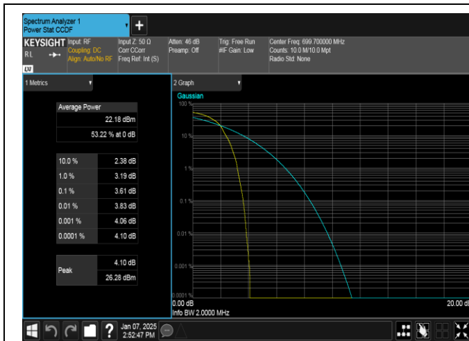
Band12-1.4MHz-16QAM-23017-1RB#0-PASS
