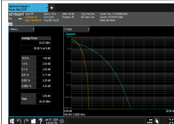
Band12-3MHz-QPSK-23165-1RB#0-PASS
