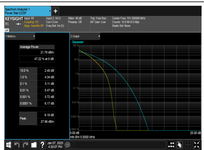
Band12-5MHz-QPSK-23035-25RB#0-PASS
