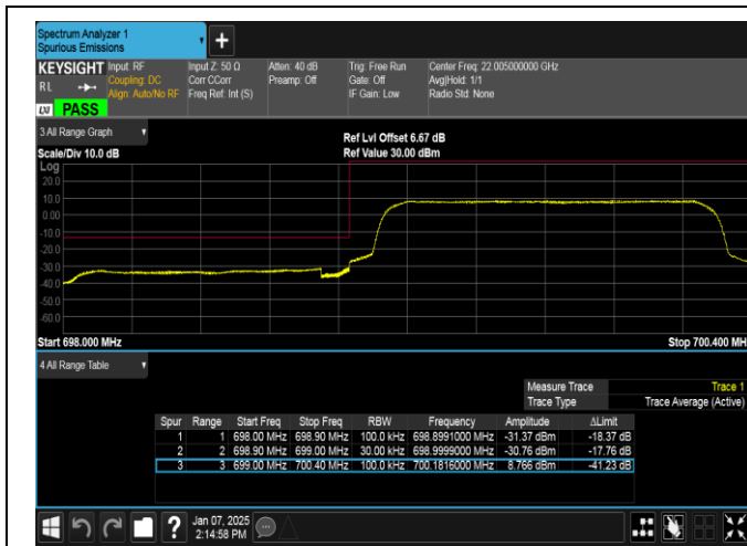
Band12-1.4MHz-QPSK-23017-6RB#0-PASS
