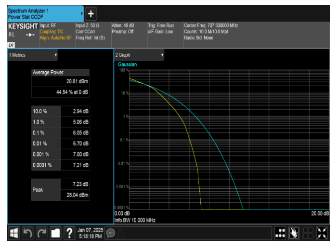
Band12-10MHz-16QAM-23095-50RB#0-PASS
