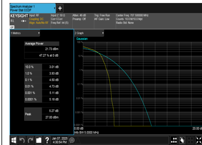
Band12-5MHz-16QAM-23095-1RB#0-PASS
