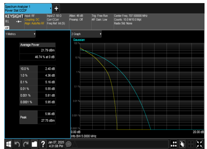
Band12-5MHz-QPSK-23095-25RB#0-PASS
