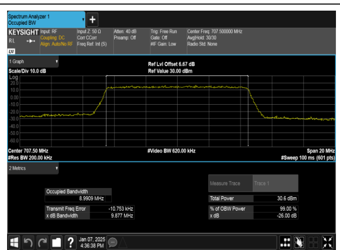
Band12-10MHz-QPSK-23095-50RB#0-PASS
