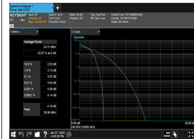
Band12-5MHz-QPSK-23095-1RB#0-PASS
