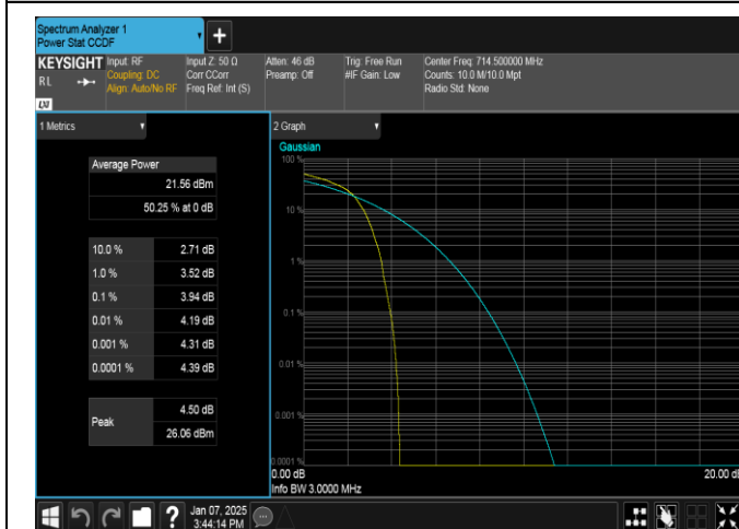
Band12-3MHz-16QAM-23165-1RB#0-PASS
