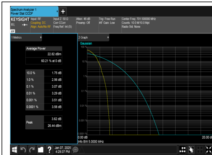
Band12-5MHz-QPSK-23035-1RB#0-PASS
