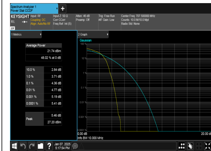
Band12-10MHz-16QAM-23095-1RB#0-PASS
