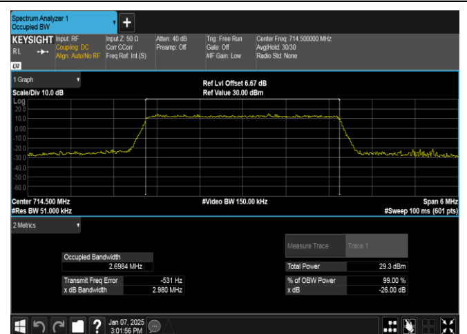
Band12-3MHz-16QAM-23165-15RB#0-PASS
