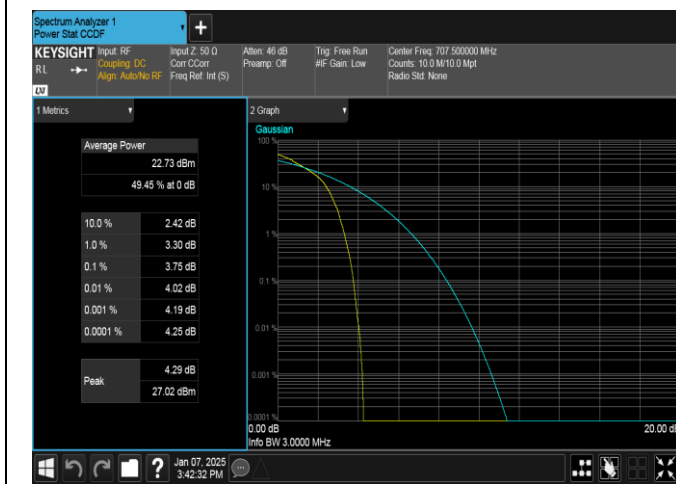
Band12-3MHz-QPSK-23095-1RB#0-PASS
