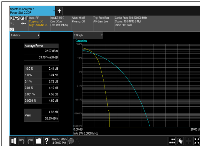
Band12-5MHz-16QAM-23035-1RB#0-PASS
