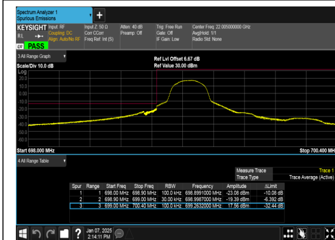
Band12-1.4MHz-16QAM-23017-1RB#0-PASS
