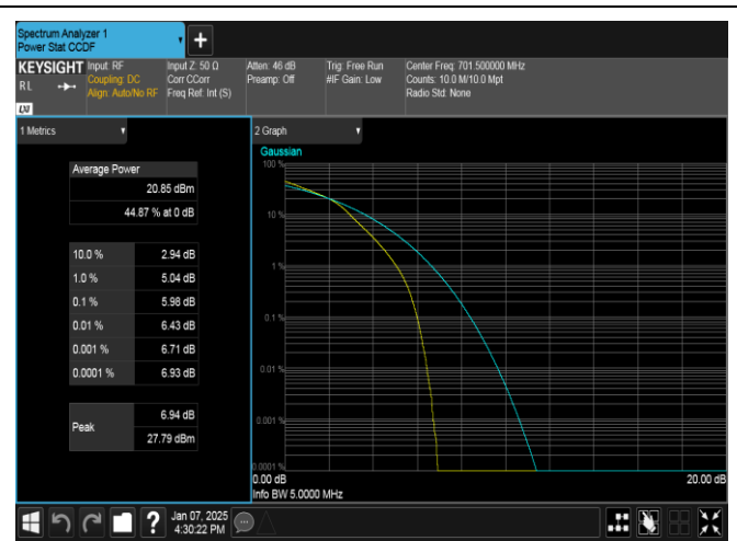
Band12-5MHz-16QAM-23035-25RB#0-PASS
