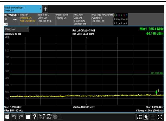
Band7-20MHz-16QAM-20850-100RB#0-30~1000-PASS
