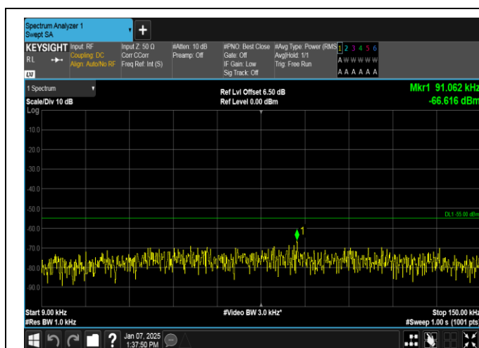
Band7-20MHz-OPSK-21100-1RB#99-0.009~0.15-PASS
