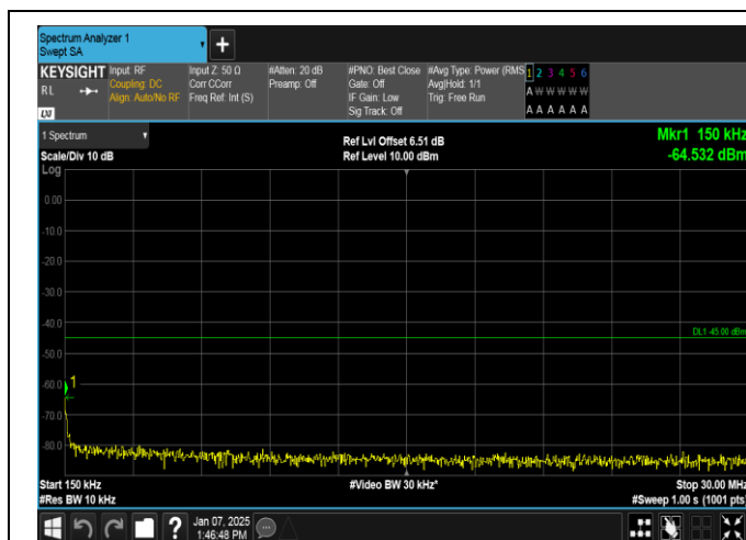
Band7-20MHz-16QAM-21350-100RB#0-0.15~30-PASS
