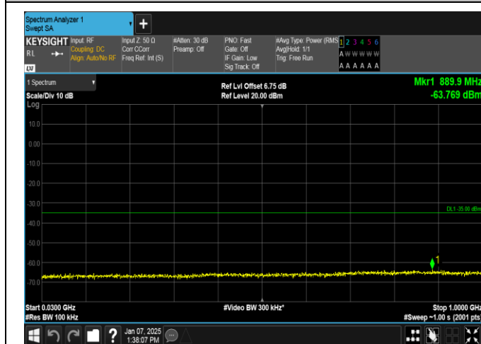
Band7-20MHz-QPSK-21100-1RB#99-30~1000-PASS
