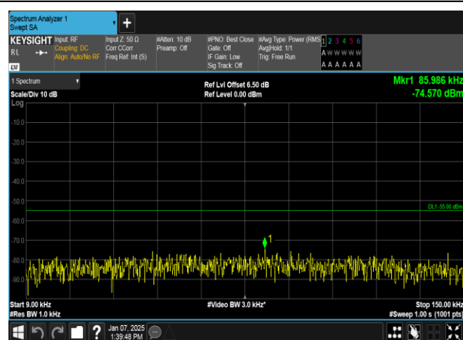
Band7-20MHz-QPSK-21100-100RB#0-0.009~0.15-PASS
