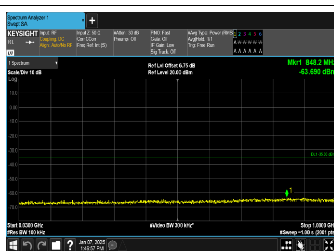
Band7-20MHz-16QAM-21350-100RB#0-30~1000-PASS
