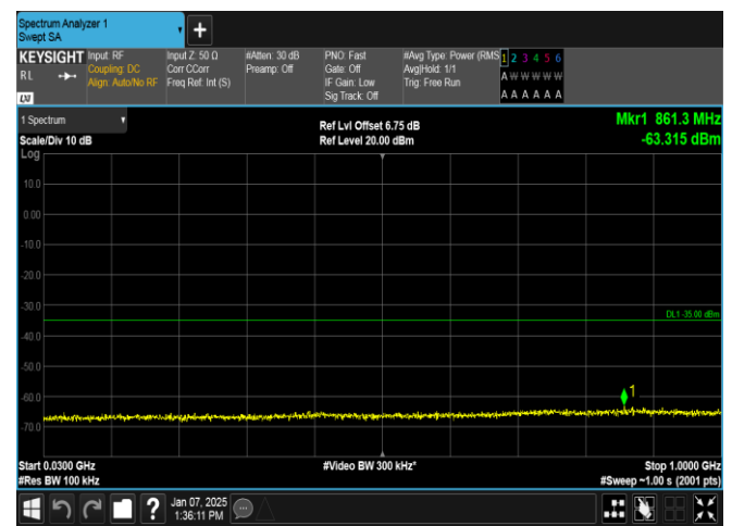
Band7-20MHz-QPSK-21100-1RB#0-30~1000-PASS
