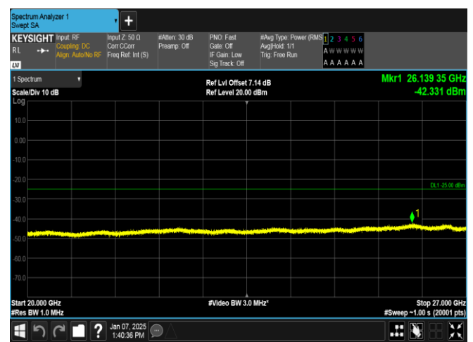
Band7-20MHz-QPSK-21100-100RB#0-20000~27000-PASS
