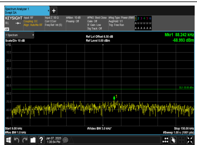
Band7-20MHz-QPSK-21100-1RB#0-0.009~0.15-PASS
