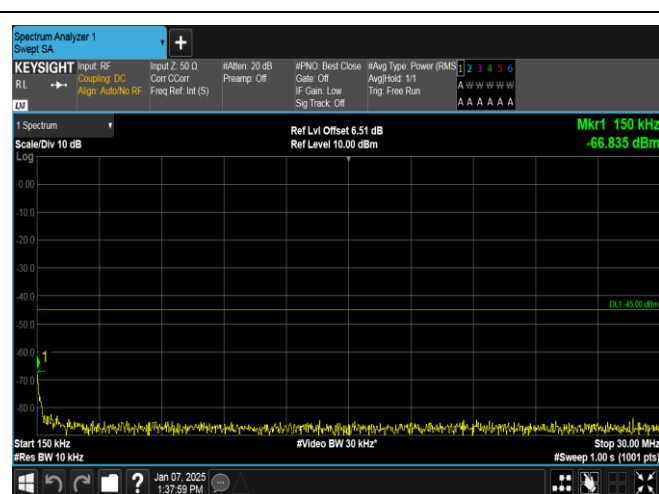
Band7-20MHz-OPSK-21100-1RB#99-0.15~30-PASS
