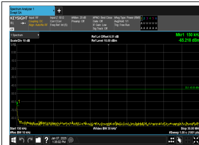
Band7-20MHz-16QAM-20850-100RB#0-0.15~30-PASS
