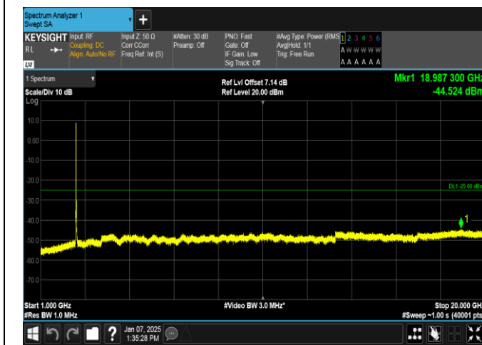
Band7-20MHz-16QAM-20850-100RB#0-1000~20000-PASS
