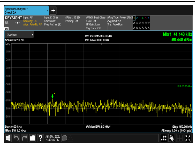
Band7-20MHz-16QAM-21350-1RB#0-0.009~0.15-PASS
