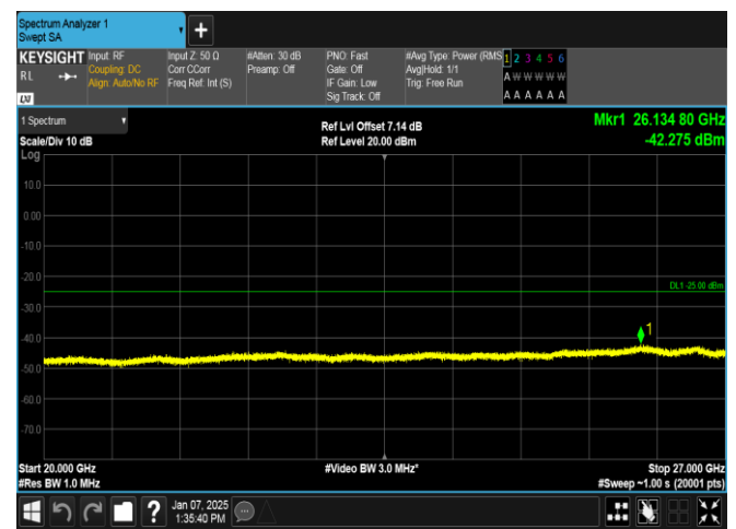
Band7-20MHz-16QAM-20850-100RB#0-20000~27000-PASS
