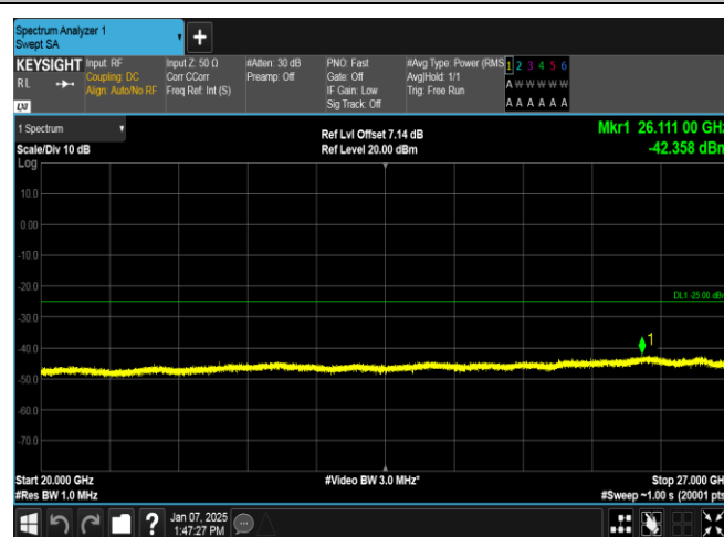
Band7-20MHz-16QAM-21350-100RB#0-20000~27000-PASS
