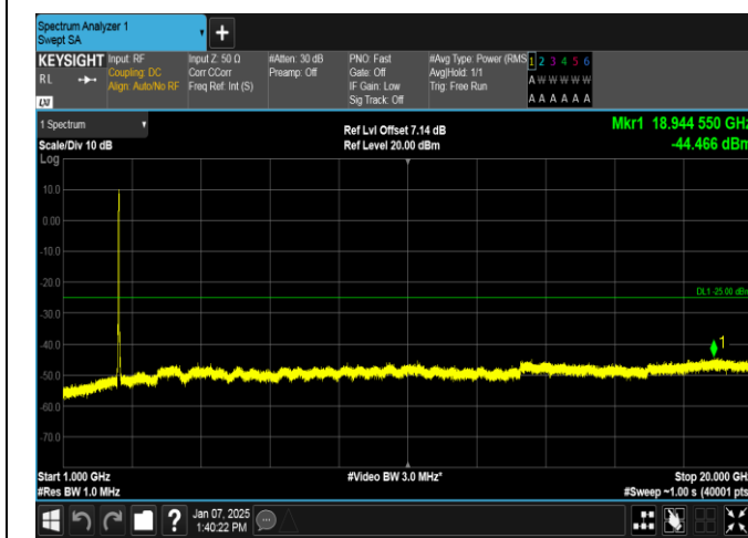
Band7-20MHz-QPSK-21100-100RB#0-1000~20000-PASS
