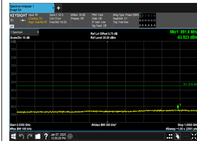
Band7-15MHz-16QAM-21375-1RB#74-30~1000-PASS
