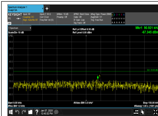
Band7-15MHz-16QAM-20825-1RB#74-0.009~0.15-PASS
