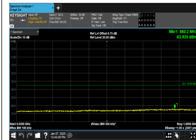
Band7-15MHz-16QAM-20825-1RB#74-30~1000-PASS
