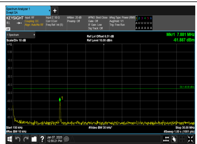
Band7-15MHz-16QAM-21375-1RB#74-0.15~30-PASS
