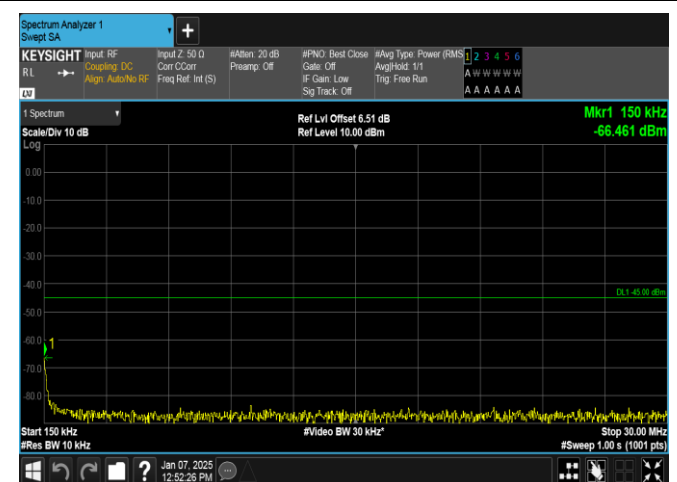
Band7-15MHz-QPSK-21375-1RB#0-0.15~30-PASS
