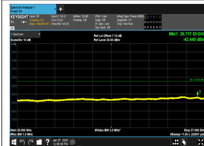
Band7-15MHz-16QAM-21375-1RB#74-20000~27000-PASS
