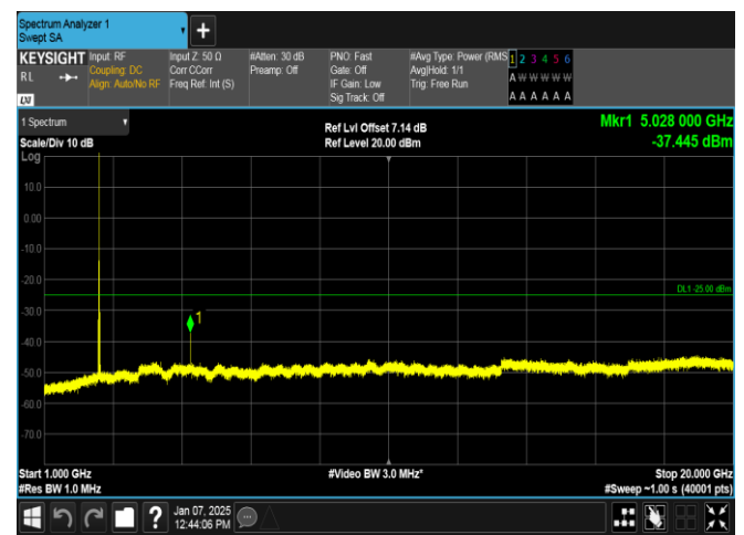
Band7-15MHz-16QAM-20825-1RB#74-1000~20000-PASS
