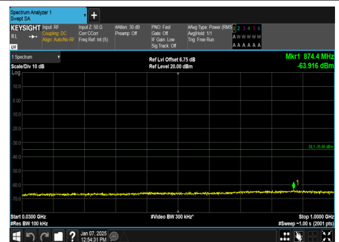
Band7-15MHz-QPSK-21375-1RB#74-30~1000-PASS
