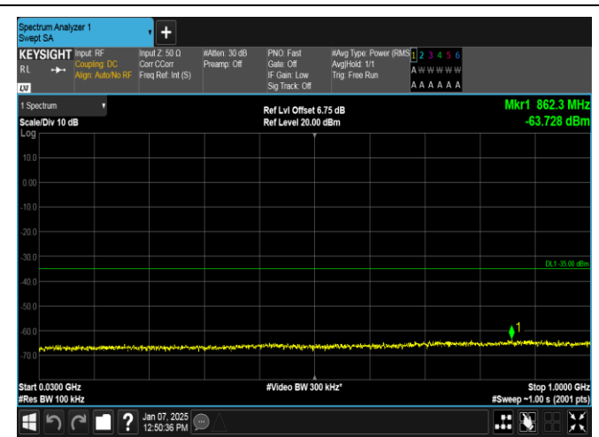
Band7-15MHz-QPSK-21100-75RB#0-30~1000-PASS
