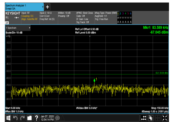
Band7-15MHz-QPSK-21375-1RB#74-0.009~0.15-PASS
