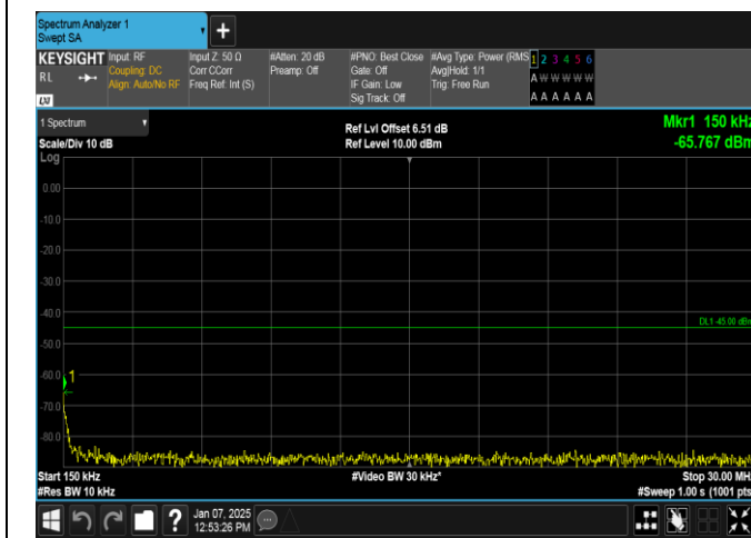
Band7-15MHz-16QAM-21375-1RB#0-0.15~30-PASS
