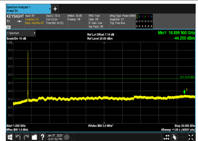
Band7-15MHz-16QAM-21100-75RB#0-1000~20000-PASS
