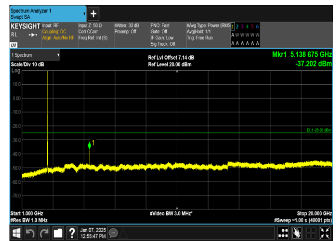
Band7-15MHz-16QAM-21375-1RB#74-1000~20000-PASS
