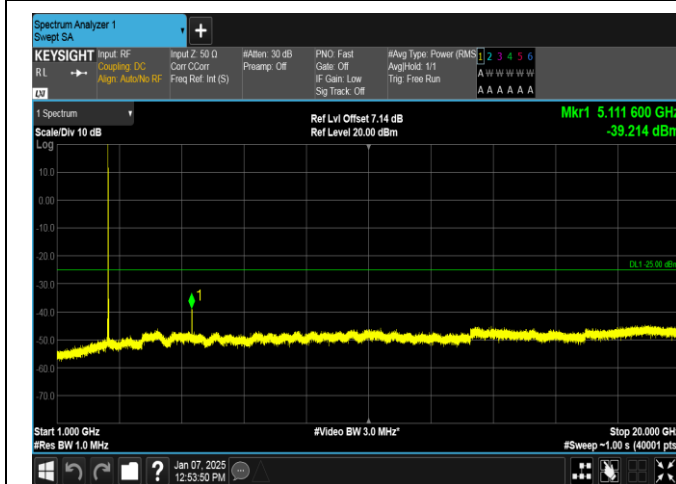
Band7-15MHz-16QAM-21375-1RB#0-1000~20000-PASS
