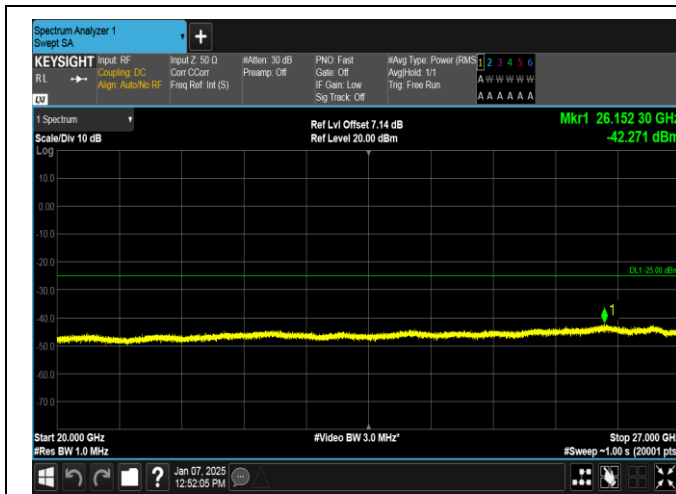
Band7-15MHz-16QAM-21100-75RB#0-20000~27000-PASS
