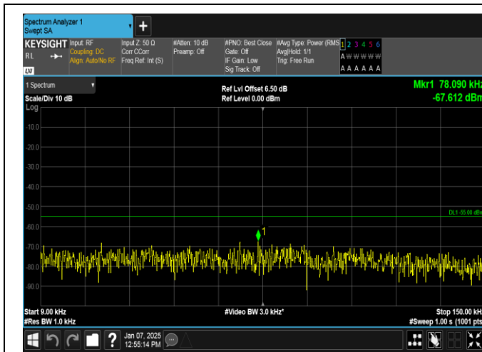
Band7-15MHz-16QAM-21375-1RB#74-0.009~0.15-PASS
