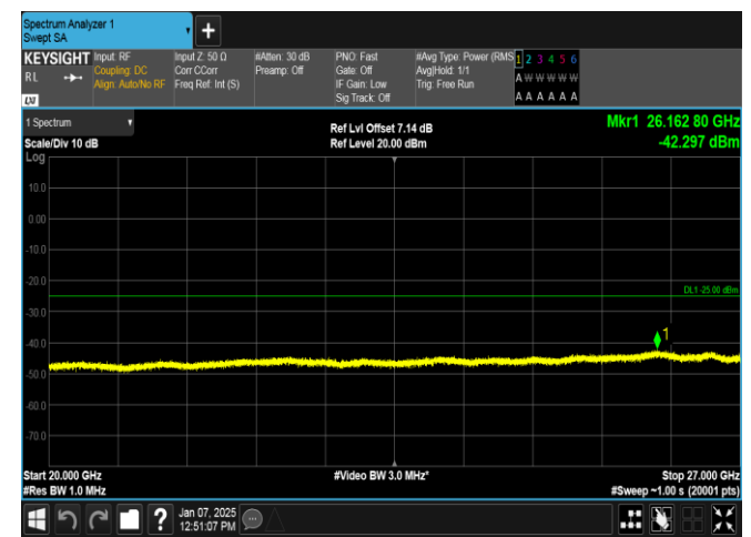
Band7-15MHz-QPSK-21100-75RB#0-20000~27000-PASS
