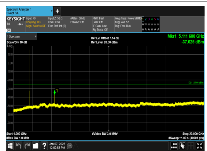
Band7-15MHz-QPSK-21375-1RB#0-1000~20000-PASS
