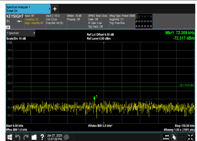
Band7-15MHz-16QAM-21375-75RB#0-0.009~0.15-PASS
