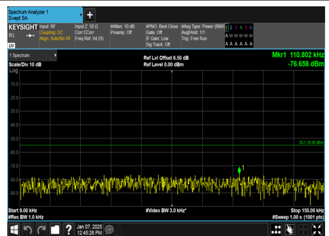
Band7-15MHz-16QAM-20825-75RB#0-0.009~0.15-PASS
