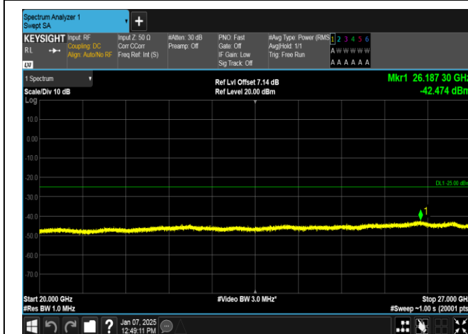
Band7-15MHz-QPSK-21100-1RB#74-20000~27000-PASS
