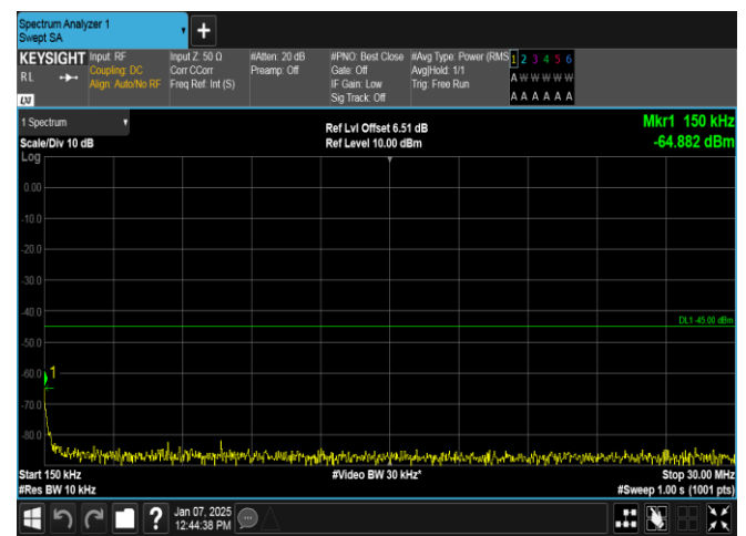
Band7-15MHz-QPSK-20825-75RB#0-0.15~30-PASS
