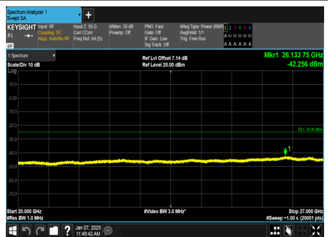
Band7-10MHz-16QAM-21400-1RB#0-20000~27000-PASS
