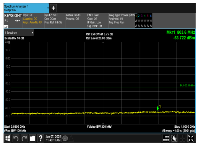
Band7-10MHz-16QAM-21400-1RB#0-30~1000-PASS
