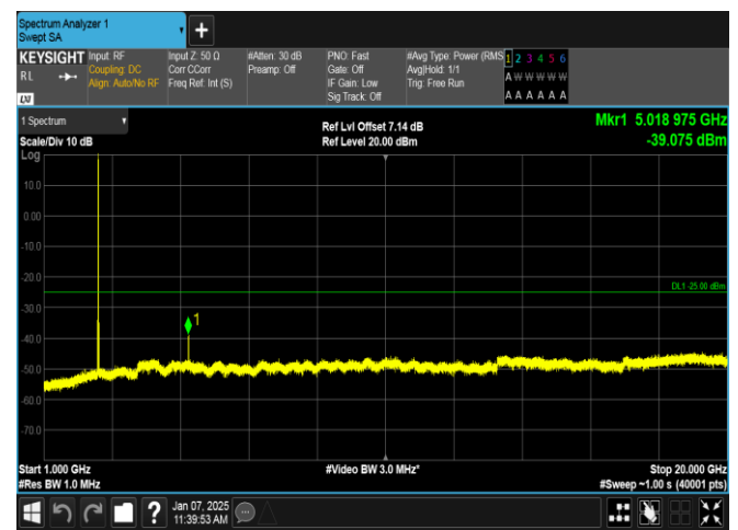
Band7-10MHz-16QAM-20800-1RB#49-1000~20000-PASS
