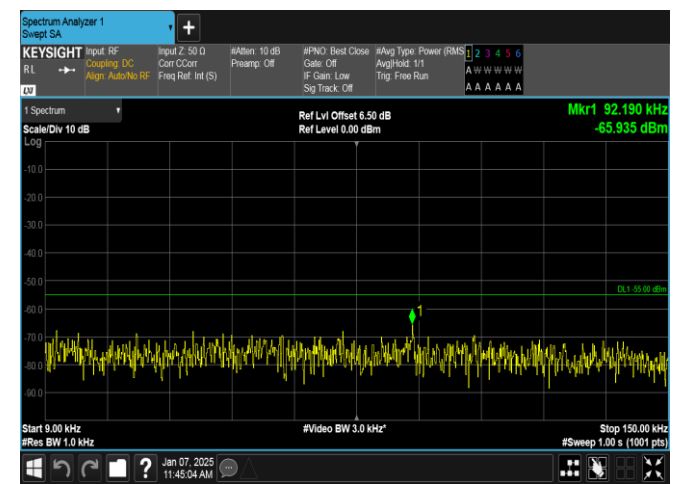
Band7-10MHz-16QAM-21100-1RB#49-0.009~0.15-PASS
