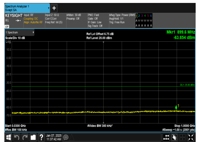
Band7-10MHz-16QAM-20800-1RB#0-30~1000-PASS
