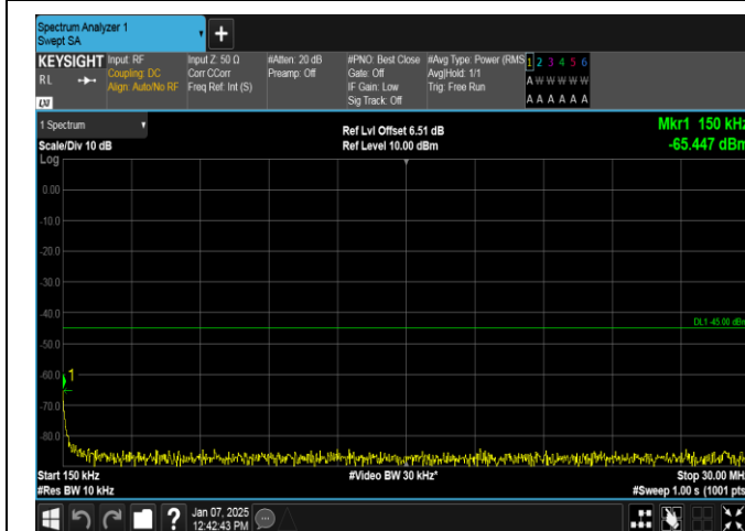
Band7-15MHz-QPSK-20825-1RB#74-0.15~30-PASS
