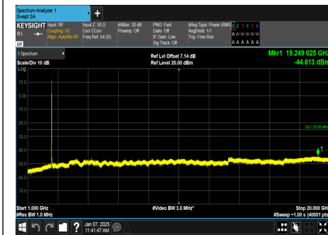
Band7-10MHz-16QAM-20800-50RB#0-1000~20000-PASS
