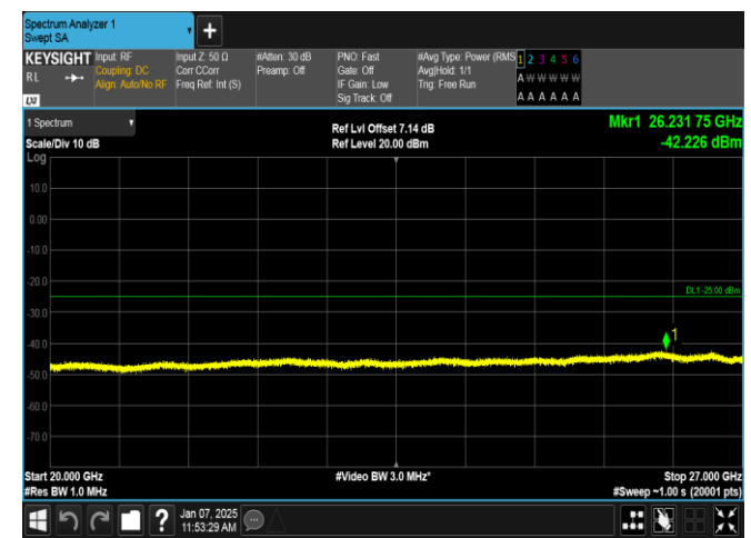
Band7-10MHz-16QAM-21400-50RB#0-20000~27000-PASS
