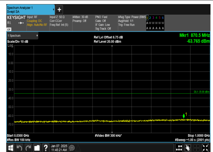
Band7-10MHz-16QAM-21100-1RB#49-30~1000-PASS
