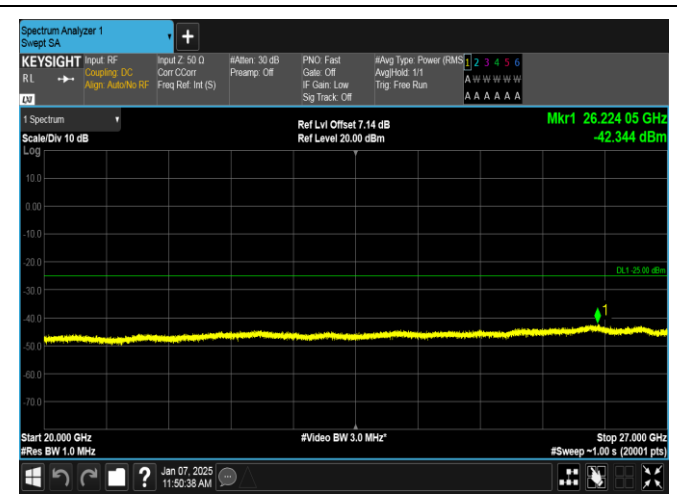
Band7-10MHz-QPSK-21400-1RB#49-20000~27000-PASS
