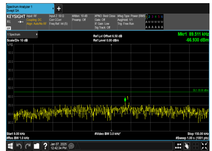
Band7-15MHz-QPSK-20825-1RB#74-0.009~0.15-PASS
