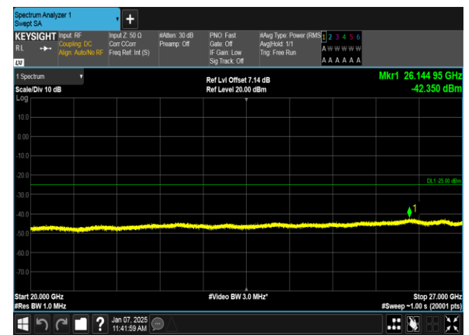
Band7-10MHz-16QAM-20800-50RB#0-20000~27000-PASS
