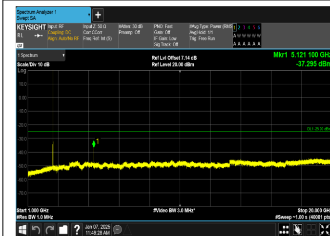
Band7-10MHz-16QAM-21400-1RB#0-1000~20000-PASS
