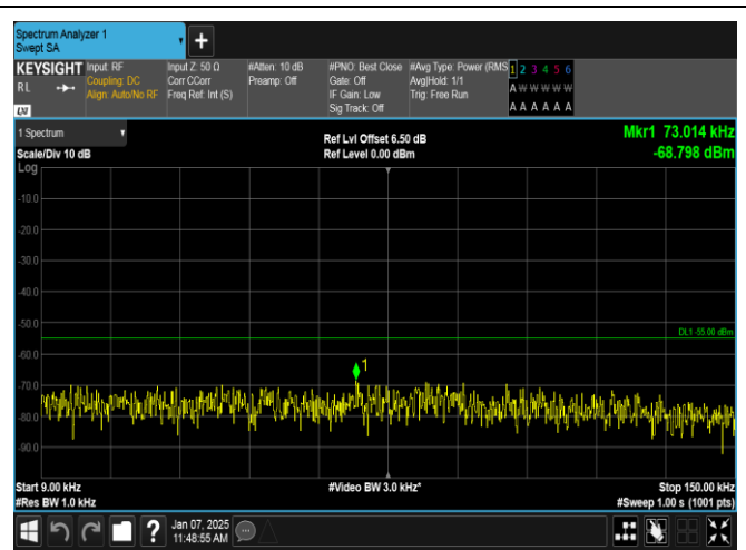
Band7-10MHz-16QAM-21400-1RB#0-0.009~0.15-PASS
