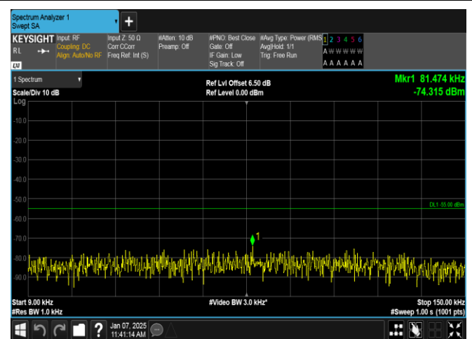
Band7-10MHz-16QAM-20800-50RB#0-0.009~0.15-PASS
