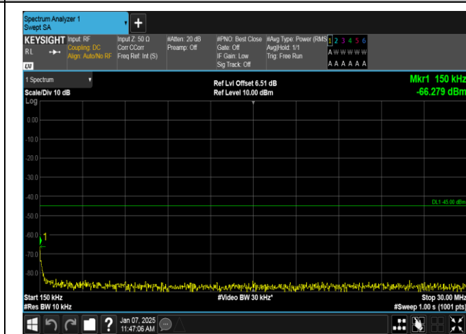
Band7-10MHz-16QAM-21100-50RB#0-0.15~30-PASS
