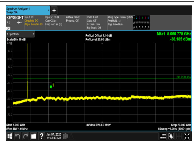
Band7-10MHz-16QAM-21100-1RB#0-1000~20000-PASS
