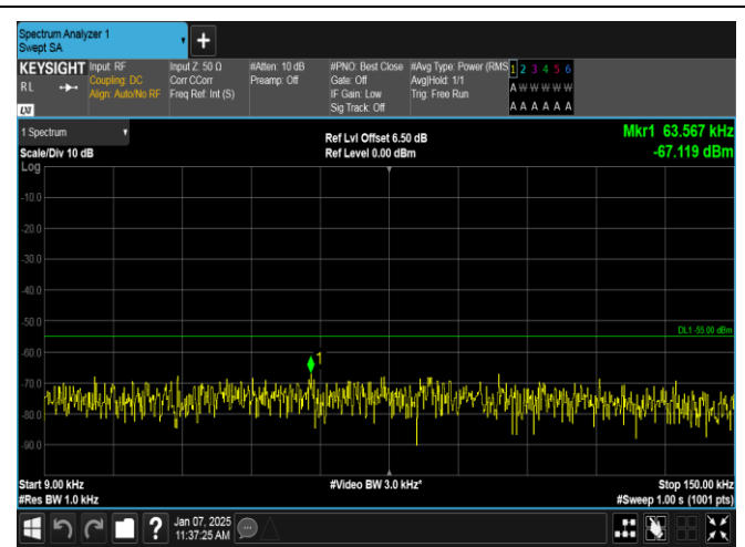
Band7-10MHz-16QAM-20800-1RB#0-0.009~0.15-PASS
