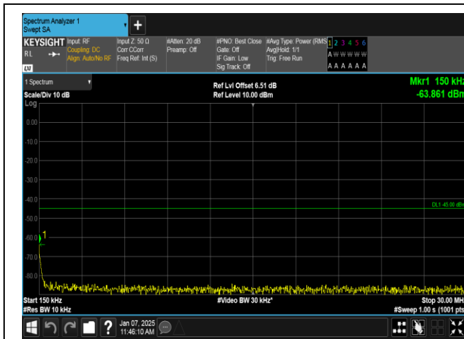
Band7-10MHz-QPSK-21100-50RB#0-0.15~30-PASS
