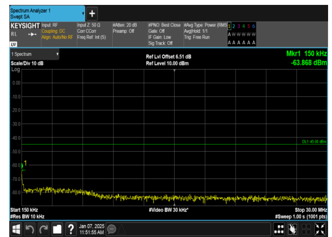
Band7-10MHz-QPSK-21400-50RB#0-0.15~30-PASS
