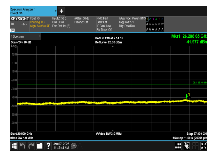
Band7-10MHz-16QAM-21100-50RB#0-20000~27000-PASS
