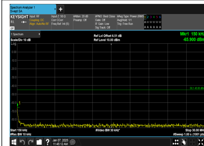
Band7-10MHz-16QAM-21100-1RB#49-0.15~30-PASS
