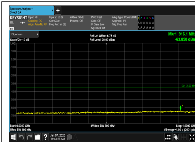
Band7-10MHz-16QAM-21100-1RB#0-30~1000-PASS
