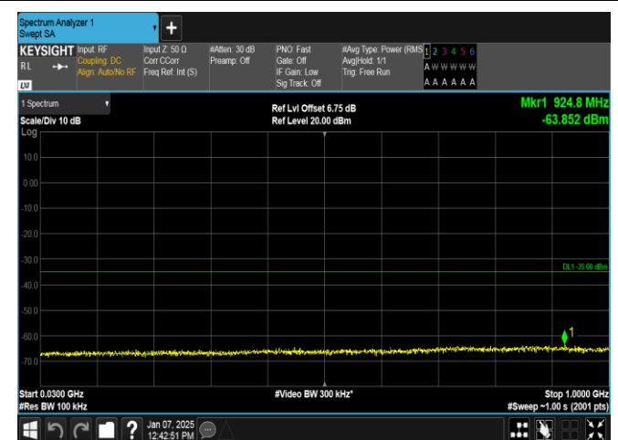
Band7-15MHz-QPSK-20825-1RB#74-30~1000-PASS
