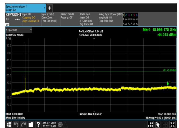
Band7-10MHz-QPSK-21400-50RB#0-1000~20000-PASS
