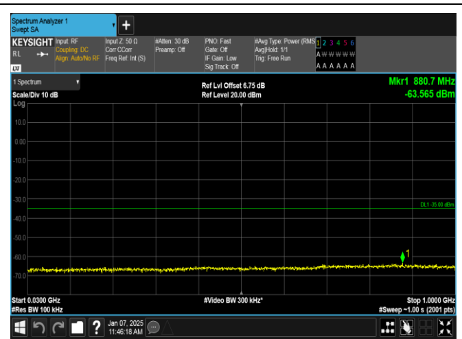
Band7-10MHz-QPSK-21100-50RB#0-30~1000-PASS
