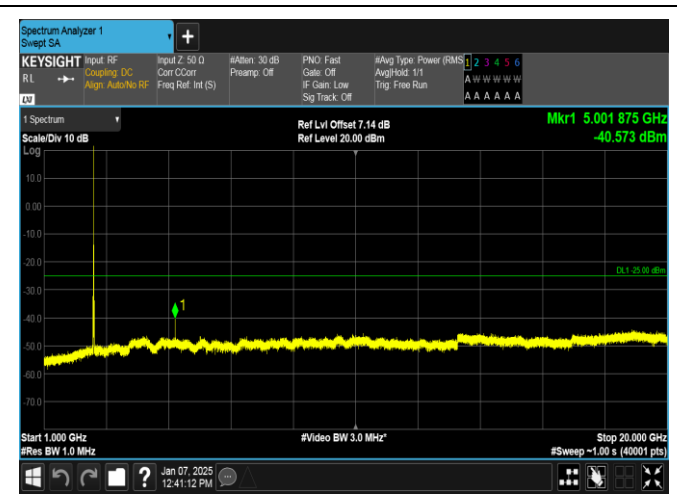
Band7-15MHz-QPSK-20825-1RB#0-1000~20000-PASS
