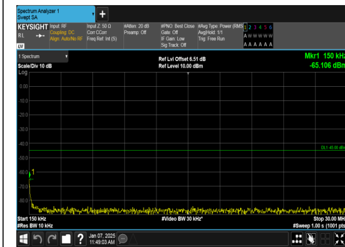
Band7-10MHz-16QAM-21400-1RB#0-0.15~30-PASS
