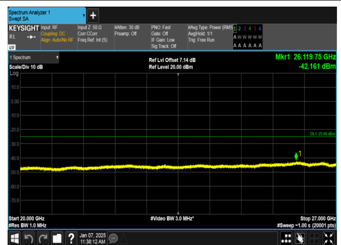
Band7-10MHz-16QAM-20800-1RB#0-20000~27000-PASS
