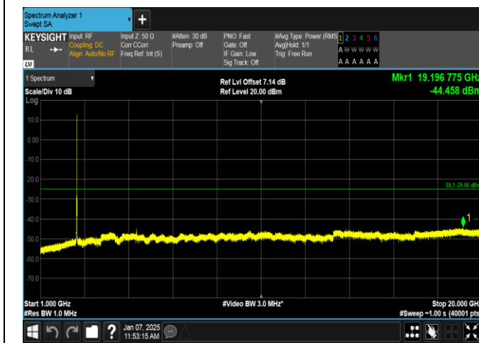
Band7-10MHz-16QAM-21400-50RB#0-1000~20000-PASS
