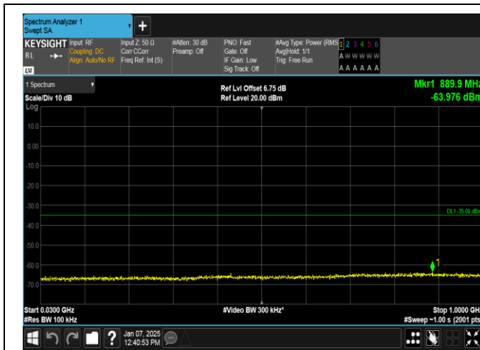
Band7-15MHz-QPSK-20825-1RB#0-30~1000-PASS
