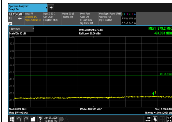
Band7-15MHz-QPSK-20825-75RB#0-30~1000-PASS
