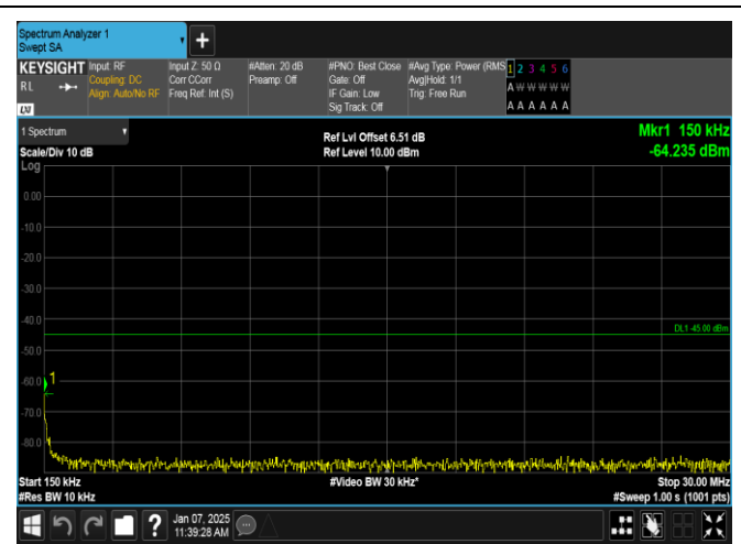
Band7-10MHz-16QAM-20800-1RB#49-0.15~30-PASS
