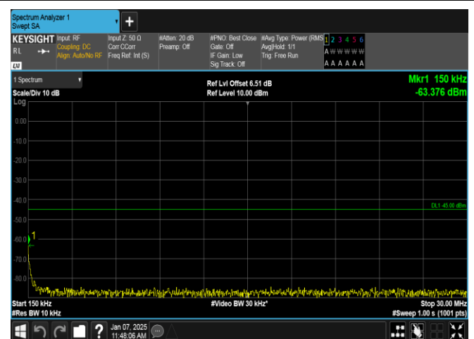
Band7-10MHz-QPSK-21400-1RB#0-0.15~30-PASS
