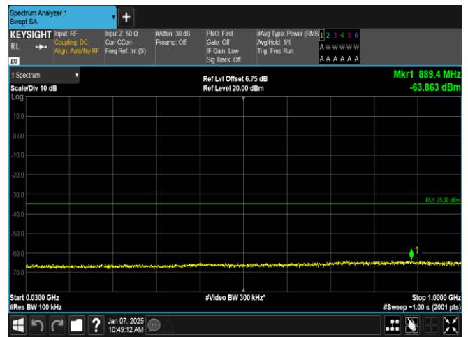
Band7-5MHz-16QAM-21425-25RB#0-30~1000-PASS
