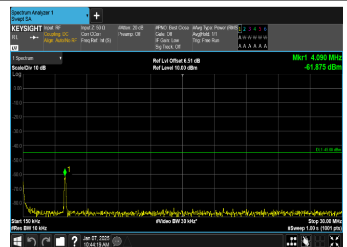
Band7-5MHz-QPSK-21425-1RB#0-0.15~30-PASS
