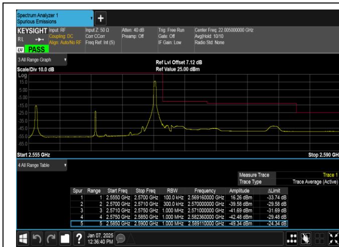
Band7-15MHz-16QAM-21375-1RB#74-PASS
