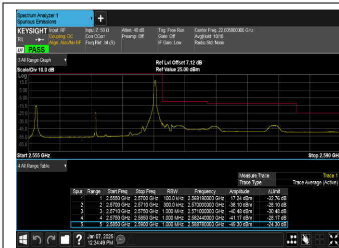
Band7-15MHz-QPSK-21375-1RB#74-PASS
