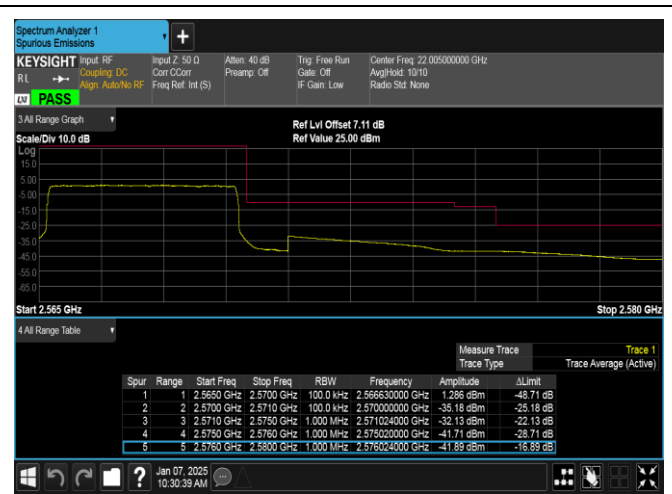
Band7-5MHz-QPSK-21425-25RB#0-PASS
