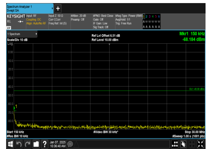
Band7-5MHz-QPSK-20775-25RB#0-0.15~30-PASS
