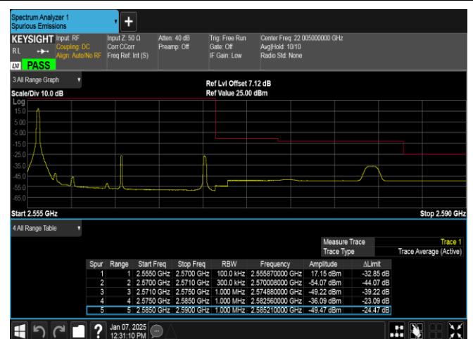
Band7-15MHz-QPSK-21375-1RB#0-PASS
