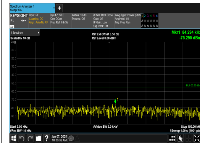
Band7-5MHz-QPSK-20775-25RB#0-0.009~0.15-PASS
