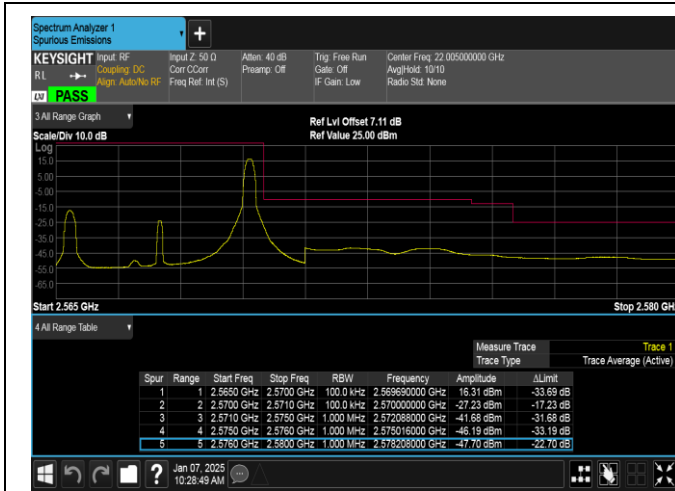
Band7-5MHz-16QAM-21425-1RB#24-PASS
