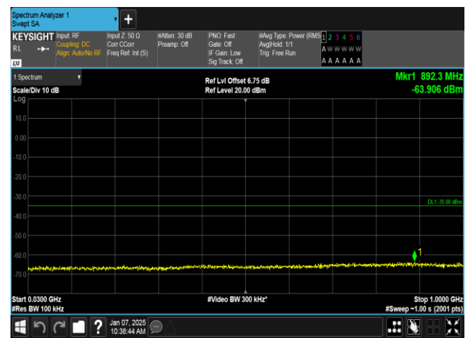
Band7-5MHz-QPSK-21100-1RB#0-30~1000-PASS
