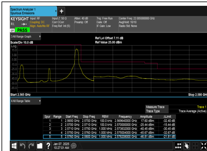
Band7-5MHz-QPSK-21425-1RB#24-PASS
