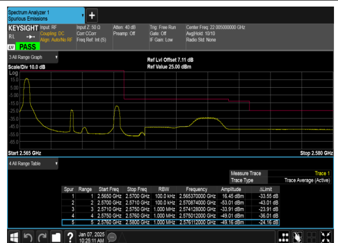
Band7-5MHz-16QAM-21425-1RB#0-PASS
