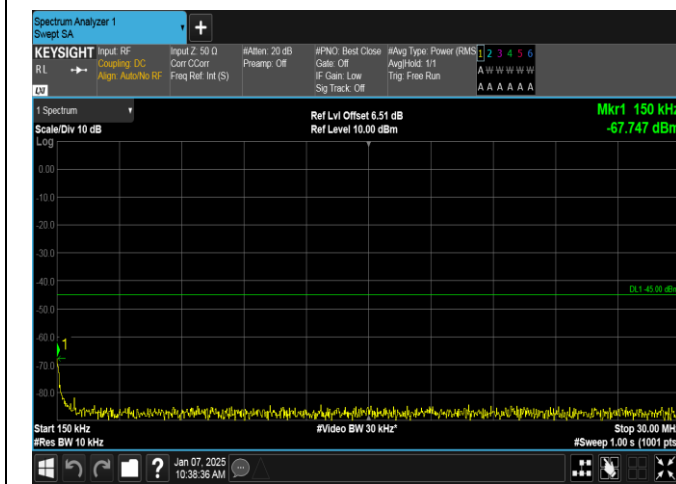
Band7-5MHz-QPSK-21100-1RB#0-0.15~30-PASS
