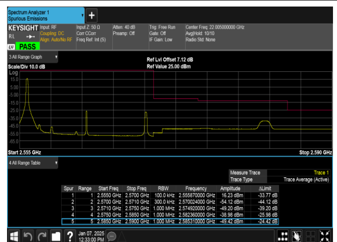
Band7-15MHz-16QAM-21375-1RB#0-PASS
