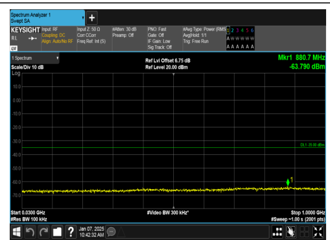
Band7-5MHz-QPSK-21100-25RB#0-30~1000-PASS
