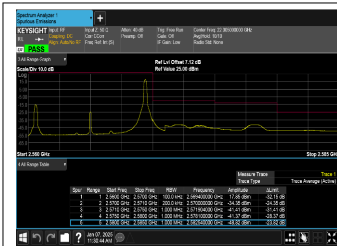
Band7-10MHz-QPSK-21400-1RB#49-PASS
