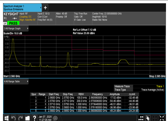
Band7-10MHz-QPSK-21400-1RB#0-PASS
