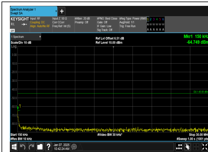
Band7-5MHz-QPSK-21100-25RB#0-0.15~30-PASS
