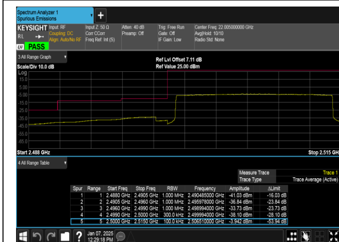
Band7-15MHz-16QAM-20825-75RB#0-PASS
