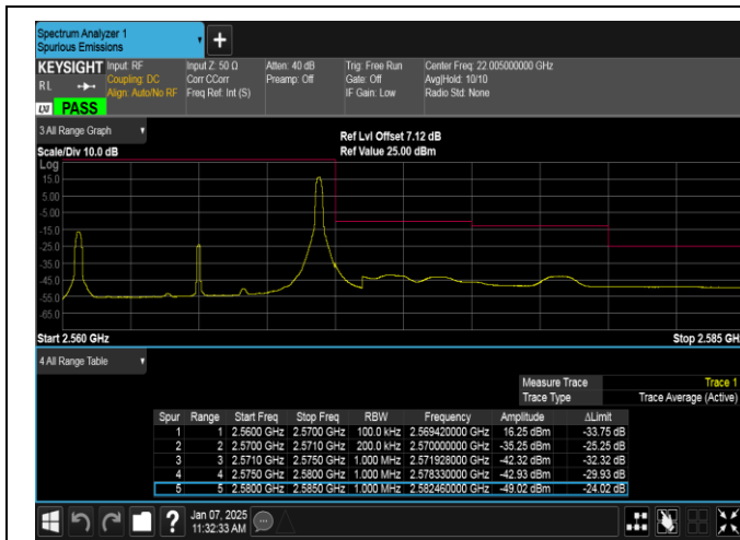
Band7-10MHz-16QAM-21400-1RB#49-PASS
