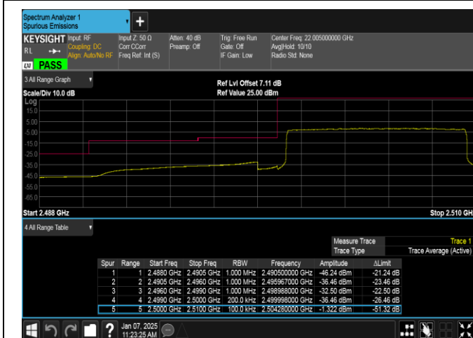
Band7-10MHz-QPSK-20800-50RB#0-PASS
