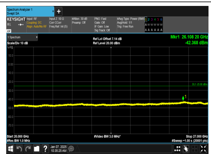
Band7-5MHz-QPSK-20775-1RB#24-20000~27000-PASS
