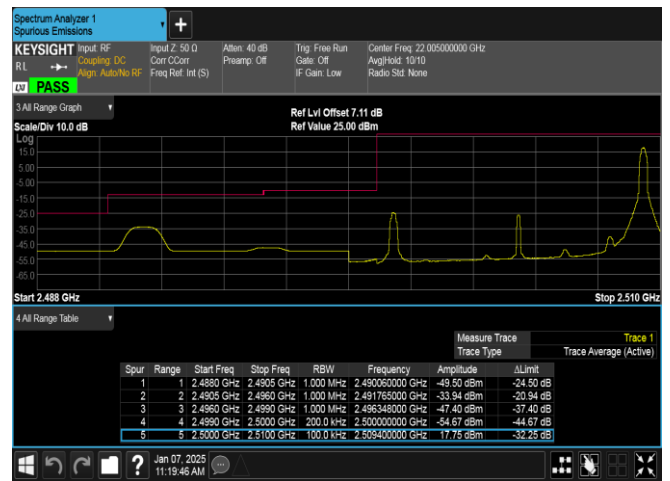
Band7-10MHz-QPSK-20800-1RB#49-PASS
