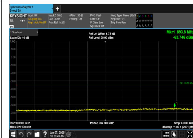
Band7-5MHz-QPSK-20775-25RB#0-30~1000-PASS
