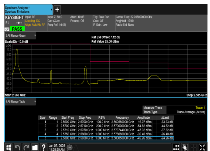
Band7-10MHz-16QAM-21400-1RB#0-PASS
