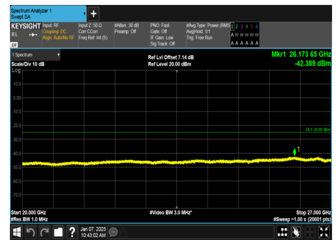
Band7-5MHz-QPSK-21100-25RB#0-20000~27000-PASS
