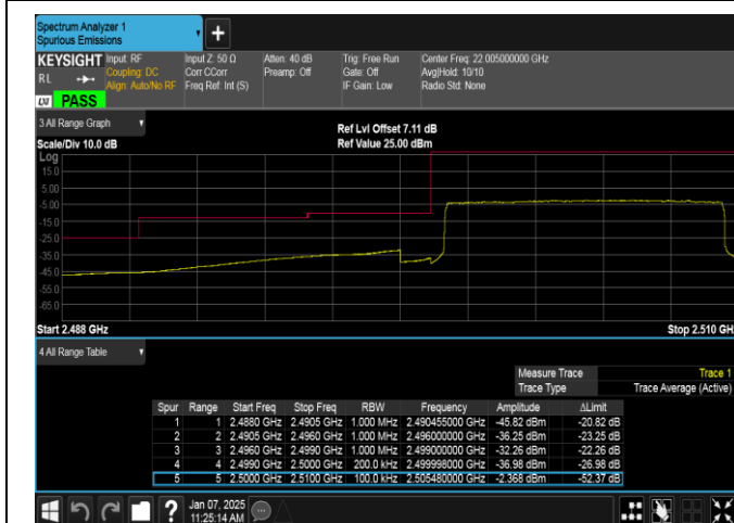
Band7-10MHz-16QAM-20800-50RB#0-PASS
