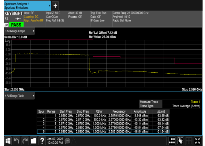
Band7-15MHz-16QAM-21375-75RB#0-PASS
