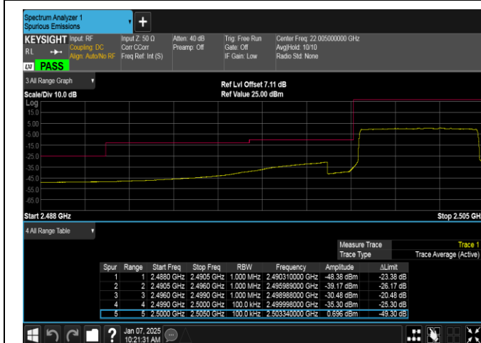
Band7-5MHz-16QAM-20775-25RB#0-PASS
