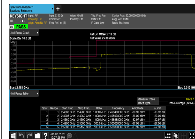
Band7-15MHz-QPSK-20825-75RB#0-PASS
