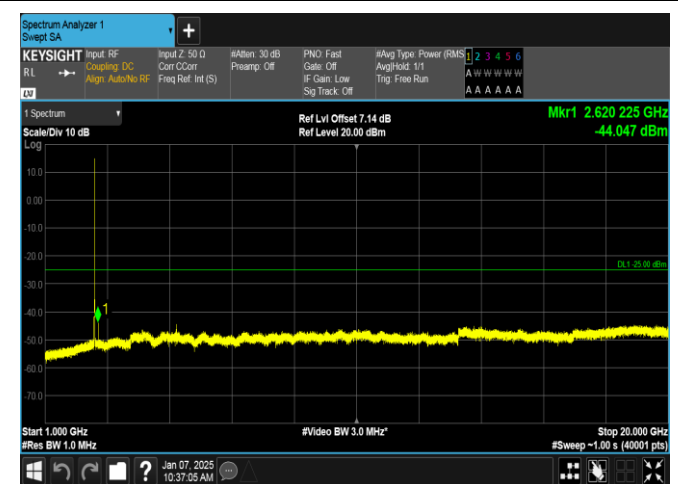
Band7-5MHz-QPSK-20775-25RB#0-1000~20000-PASS
