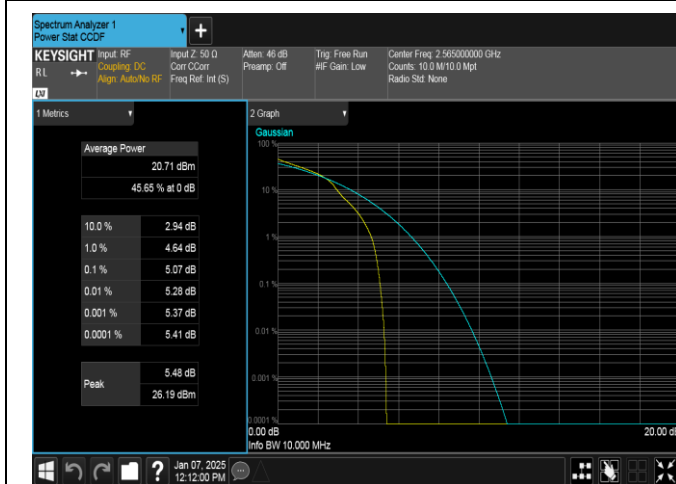
Band7-10MHz-16QAM-21400-1RB#0-PASS
