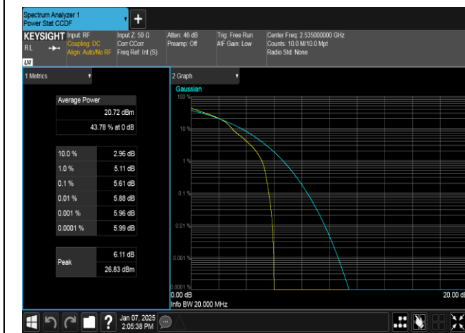
Band7-20MHz-16QAM-21100-1RB#0-PASS
