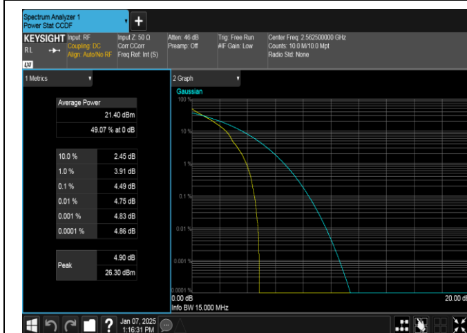
Band7-15MHz-QPSK-21375-1RB#0-PASS
