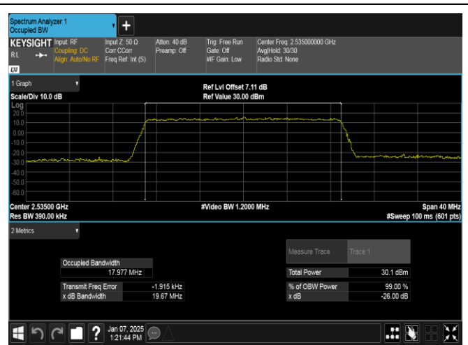
Band7-20MHz-QPSK-21100-100RB#0-PASS
