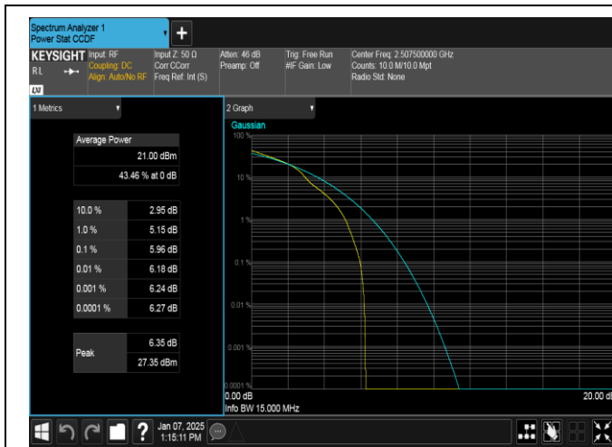
Band7-15MHz-16QAM-20825-1RB#0-PASS
