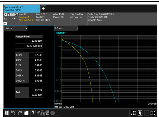
Band7-10MHz-QPSK-20800-50RB#0-PASS
