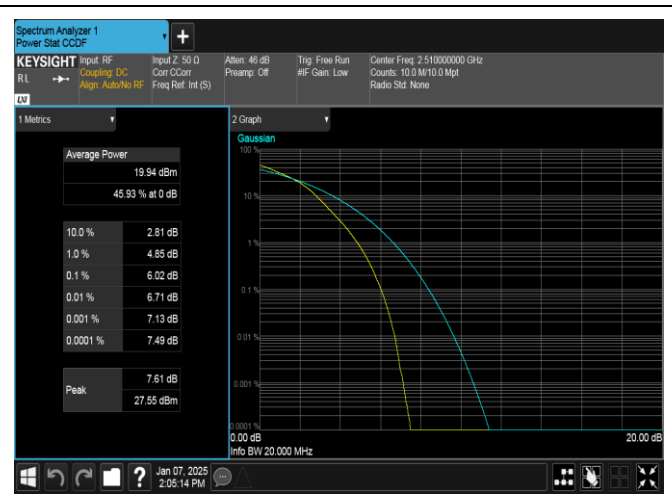
Band7-20MHz-16QAM-20850-100RB#0-PASS
