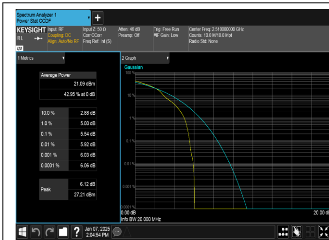
Band7-20MHz-16QAM-20850-1RB#0-PASS
