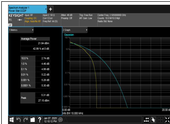
Band7-10MHz-QPSK-20800-1RB#0-PASS
