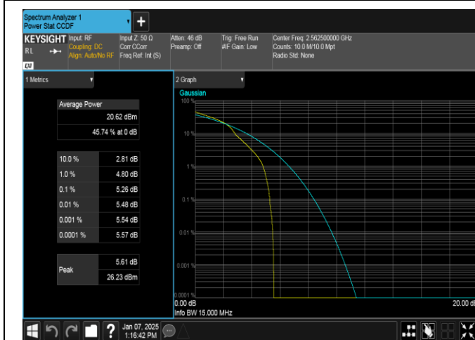
Band7-15MHz-16QAM-21375-1RB#0-PASS
