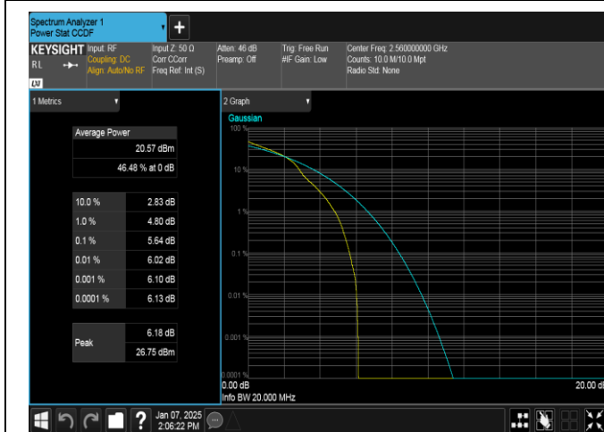
Band7-20MHz-16QAM-21350-1RB#0-PASS
