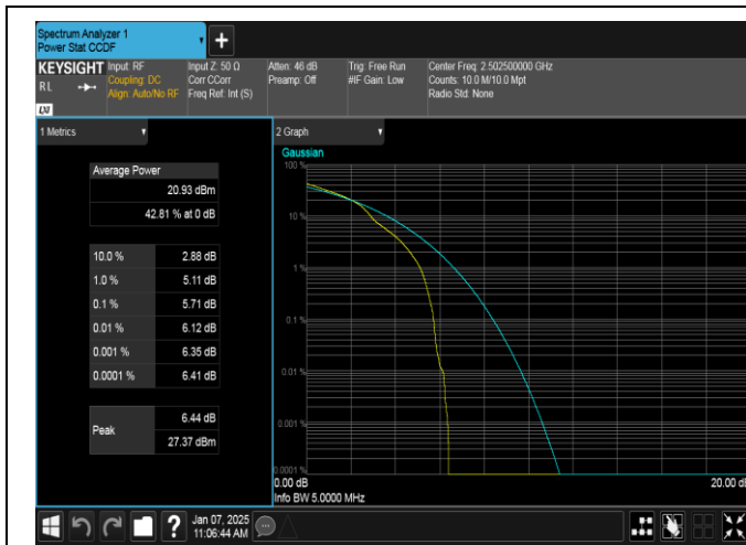
Band7-5MHz-16QAM-20775-1RB#0-PASS
