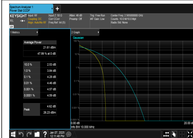
Band7-10MHz-QPSK-21400-1RB#0-PASS
