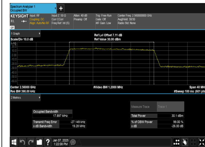
Band7-20MHz-QPSK-21350-100RB#0-PASS
