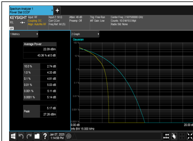
Band7-15MHz-QPSK-20825-1RB#0-PASS
