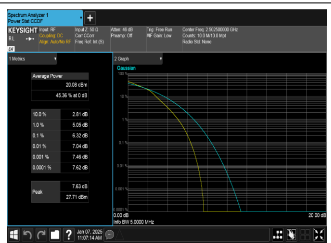
Band7-5MHz-16QAM-20775-25RB#0-PASS
