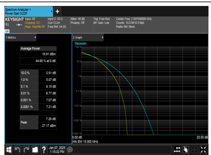
Band7-15MHz-16QAM-20825-75RB#0-PASS
