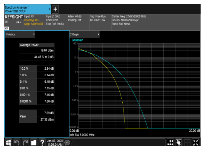
Band7-5MHz-16QAM-21425-25RB#0-PASS
