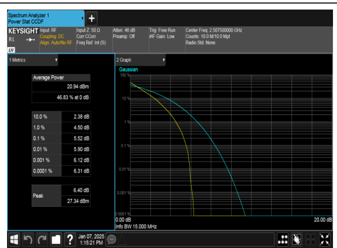
Band7-15MHz-QPSK-20825-75RB#0-PASS
