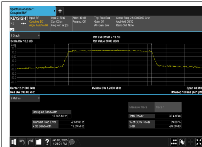
Band7-20MHz-QPSK-20850-100RB#0-PASS
