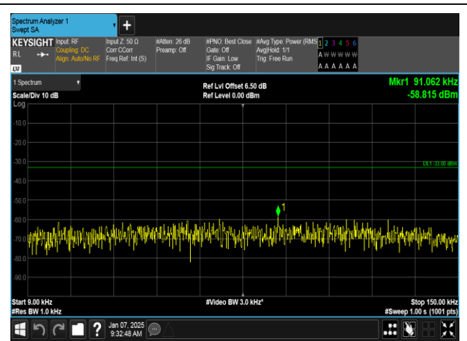
Band5-10MHz-16QAM-20450-1RB#0-0.009~0.15-PASS
