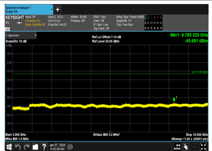
Band5-10MHz-16QAM-20450-1RB#0-3000~10000-PASS
