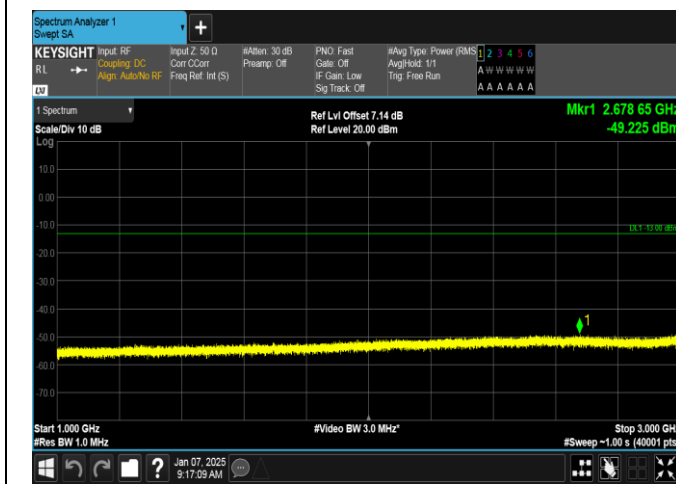
Band5-5MHz-16QAM-20625-25RB#0-1000~3000-PASS
