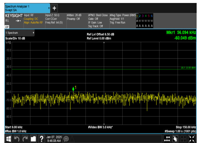
Band5-10MHz-QPSK-20600-1RB#49-0.009~0.15-PASS
