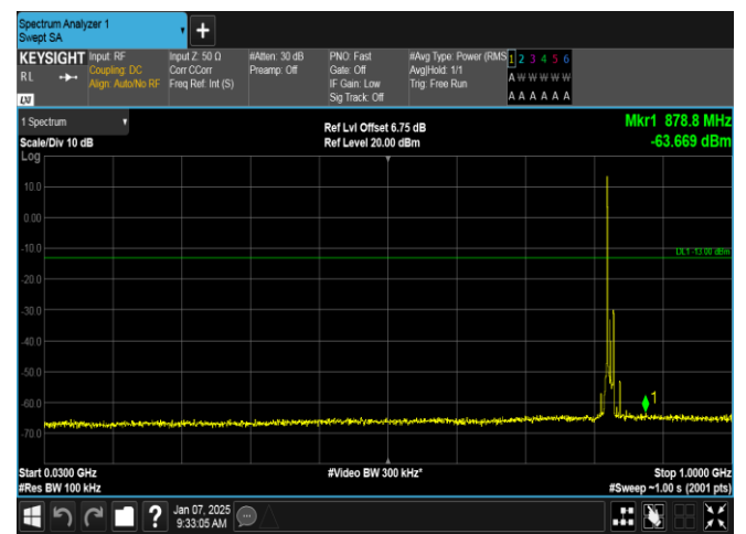
Band5-10MHz-16QAM-20450-1RB#0-30~1000-PASS
