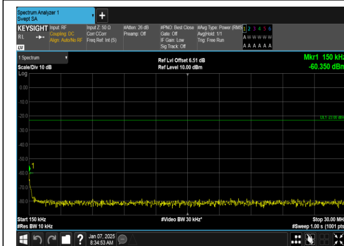
Band5-3MHz-16QAM-20525-1RB#14-0.15~30-PASS
