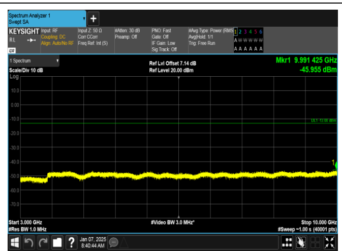
Band5-3MHz-QPSK-20635-1RB#14-3000~10000-PASS
