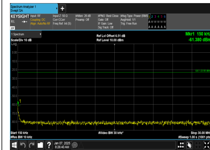
Band5-3MHz-16QAM-20415-1RB#0-0.15~30-PASS
