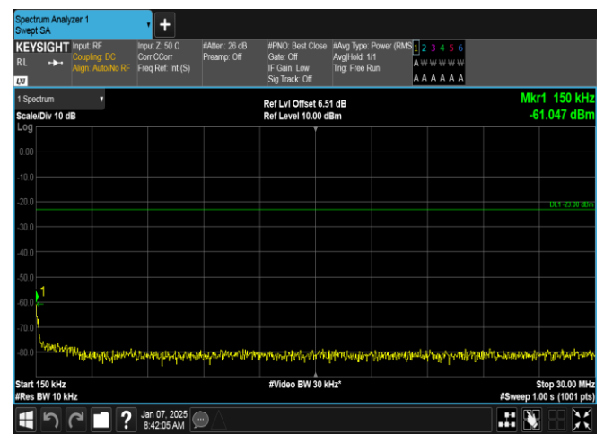
Band5-3MHz-QPSK-20635-15RB#0-0.15~30-PASS
