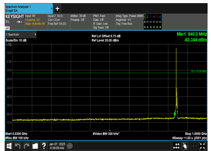
Band5-3MHz-16QAM-20635-1RB#0-30~1000-PASS
