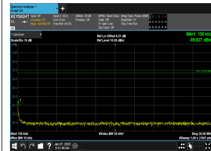
Band5-3MHz-QPSK-20525-1RB#0-0.15~30-PASS
