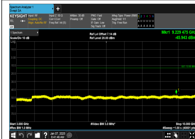
Band5-3MHz-16QAM-20635-1RB#14-3000~10000-PASS
