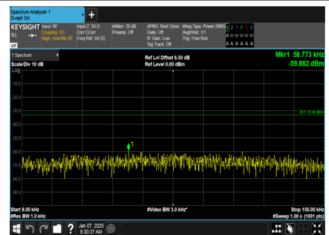
Band5-3MHz-16QAM-20415-15RB#0-0.009~0.15-PASS
