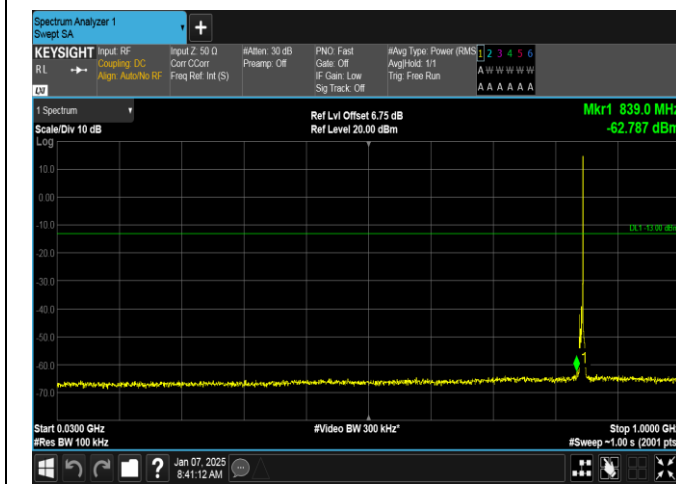
Band5-3MHz-16QAM-20635-1RB#14-30~1000-PASS
