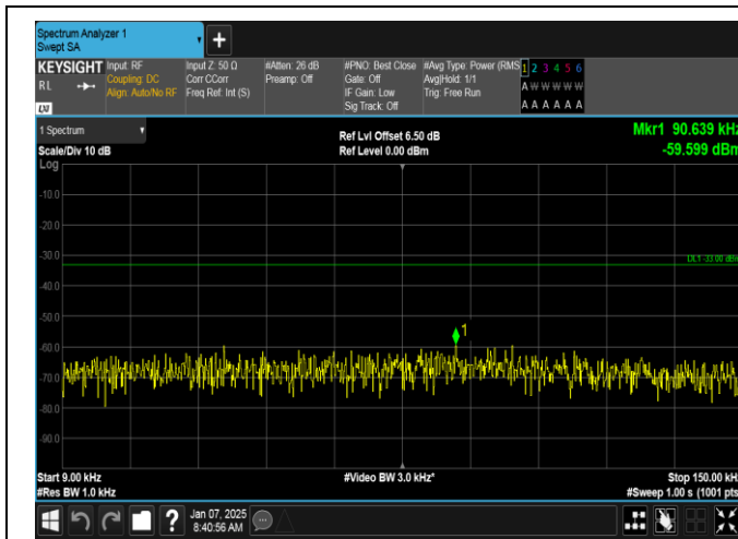
Band5-3MHz-16QAM-20635-1RB#14-0.009~0.15-PASS
