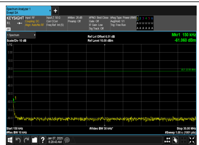
Band5-3MHz-16QAM-20415-1RB#14-0.15~30-PASS
