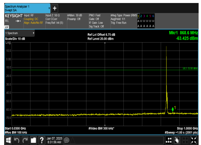
Band5-3MHz-QPSK-20525-1RB#0-30~1000-PASS
