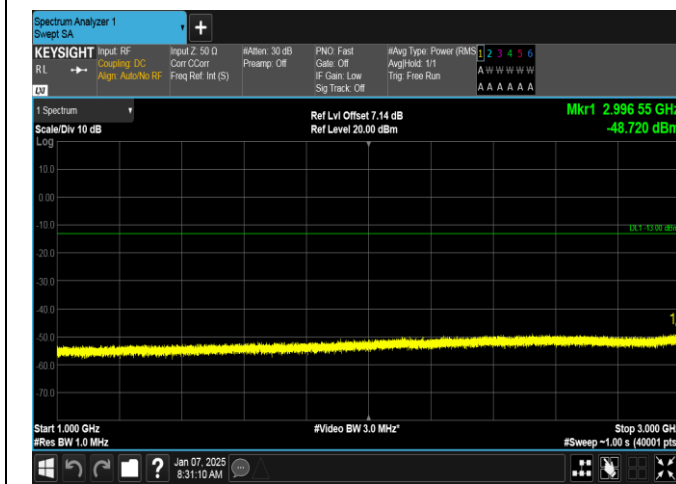
Band5-3MHz-16QAM-20415-15RB#0-1000~3000-PASS
