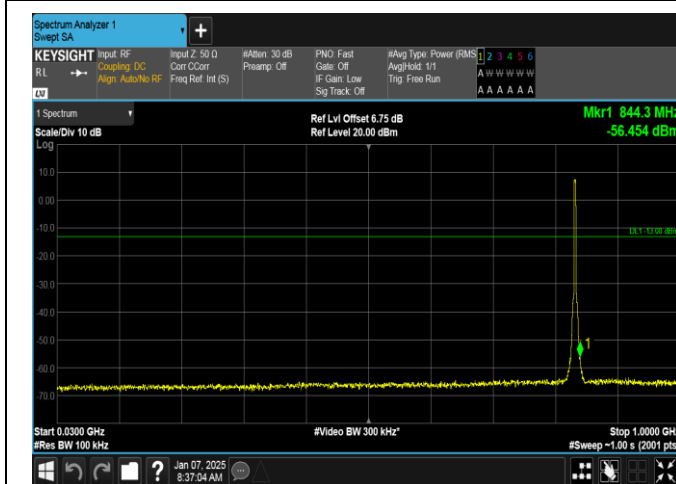
Band5-3MHz-16QAM-20525-15RB#0-30~1000-PASS
