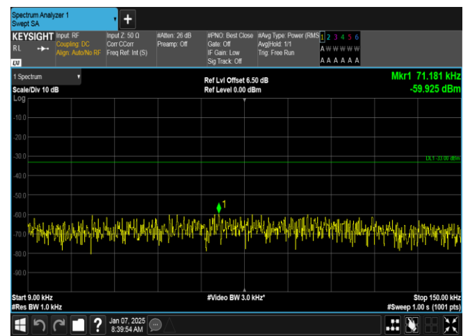
Band5-3MHz-QPSK-20635-1RB#14-0.009~0.15-PASS
