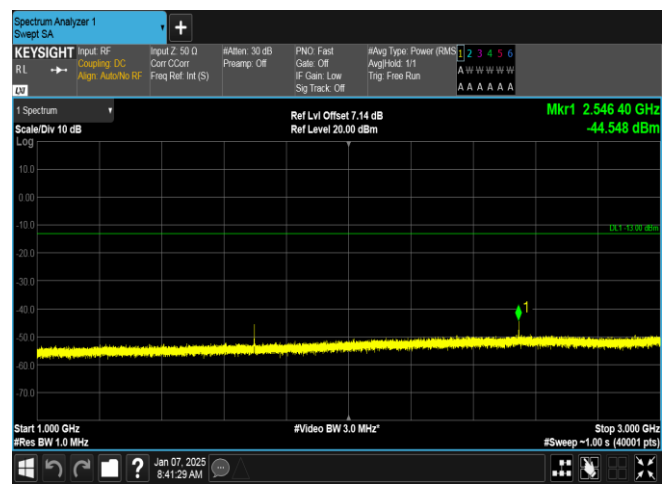
Band5-3MHz-16QAM-20635-1RB#14-1000~3000-PASS
