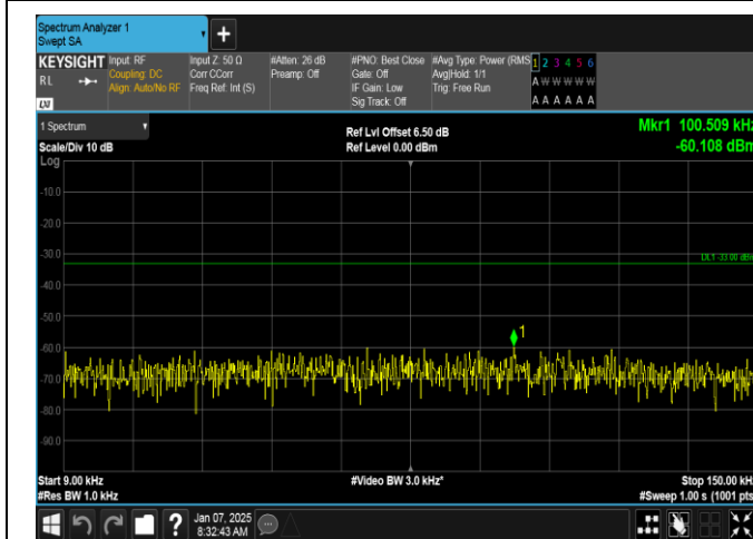
Band5-3MHz-16QAM-20525-1RB#0-0.009~0.15-PASS
