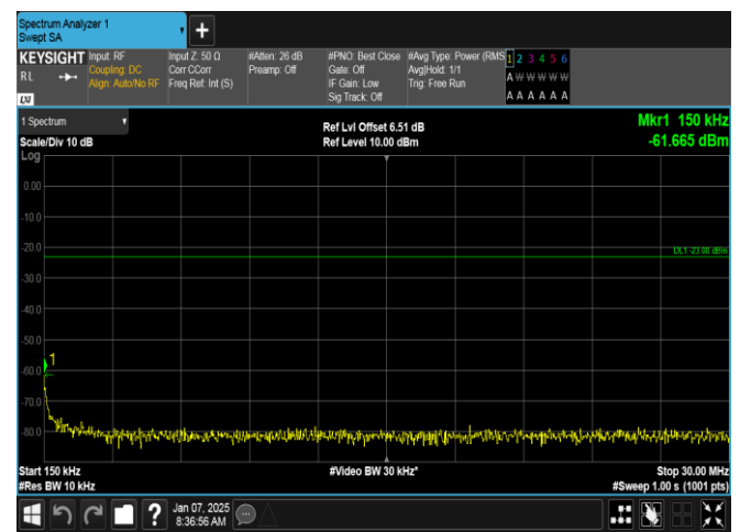
Band5-3MHz-16QAM-20525-15RB#0-0.15~30-PASS
