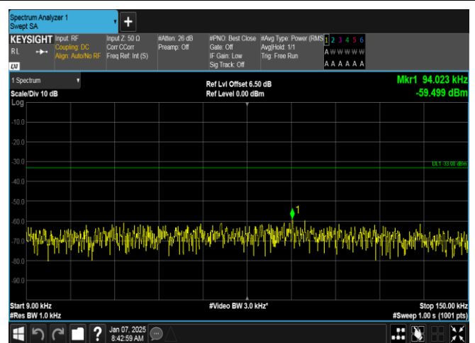
Band5-3MHz-16QAM-20635-15RB#0-0.009~0.15-PASS
