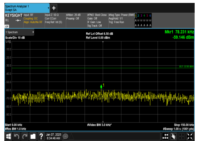
Band5-3MHz-16QAM-20525-1RB#14-0.009~0.15-PASS
