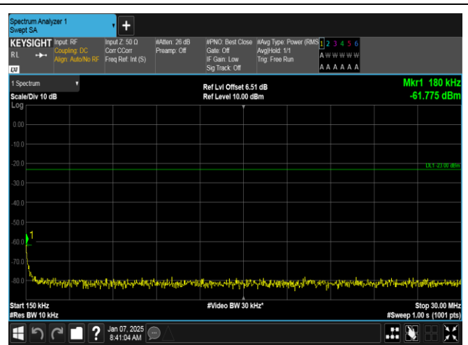
Band5-3MHz-16QAM-20635-1RB#14-0.15~30-PASS
