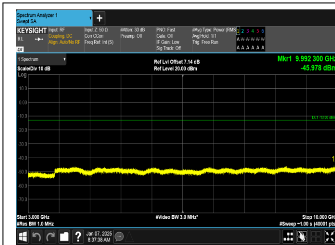
Band5-3MHz-16QAM-20525-15RB#0-3000~10000-PASS
