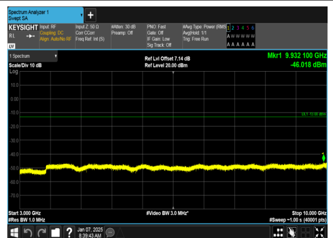
Band5-3MHz-16QAM-20635-1RB#0-3000~10000-PASS
