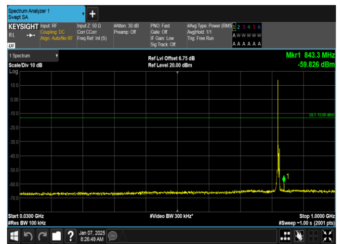
Band5-3MHz-16QAM-20415-1RB#0-30~1000-PASS
