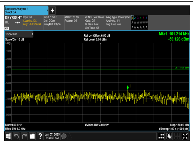
Band5-3MHz-16QAM-20635-1RB#0-0.009~0.15-PASS
