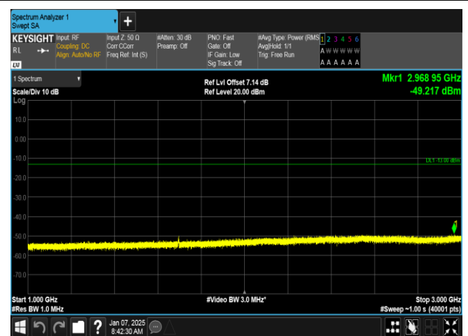
Band5-3MHz-QPSK-20635-15RB#0-1000~3000-PASS
