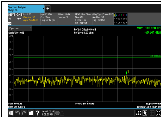
Band5-3MHz-16QAM-20415-1RB#14-0.009~0.15-PASS
