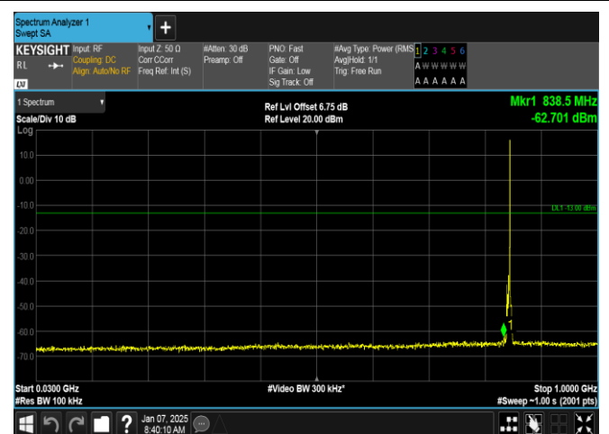
Band5-3MHz-QPSK-20635-1RB#14-30~1000-PASS
