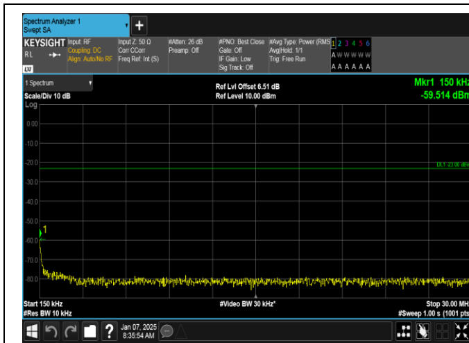
Band5-3MHz-QPSK-20525-15RB#0-0.15~30-PASS
