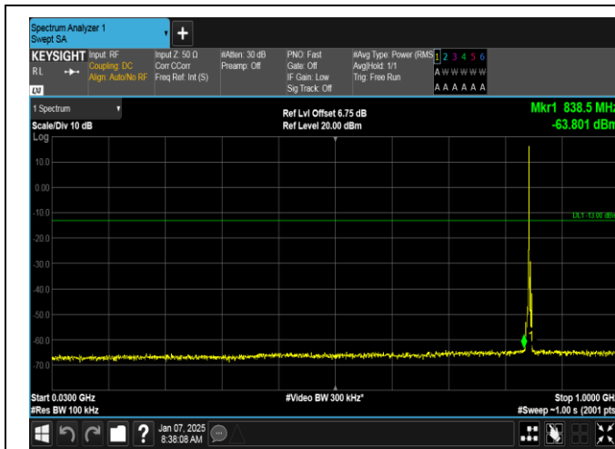
Band5-3MHz-QPSK-20635-1RB#0-30~1000-PASS
