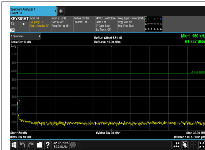
Band5-3MHz-16QAM-20415-15RB#0-0.15~30-PASS
