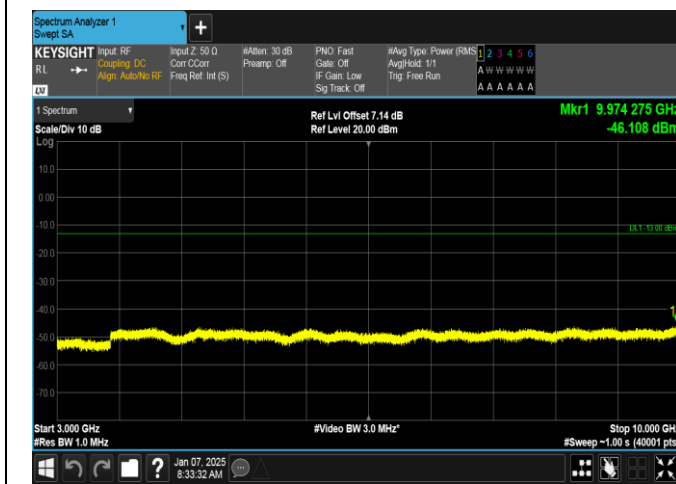
Band5-3MHz-16QAM-20525-1RB#0-3000~10000-PASS
