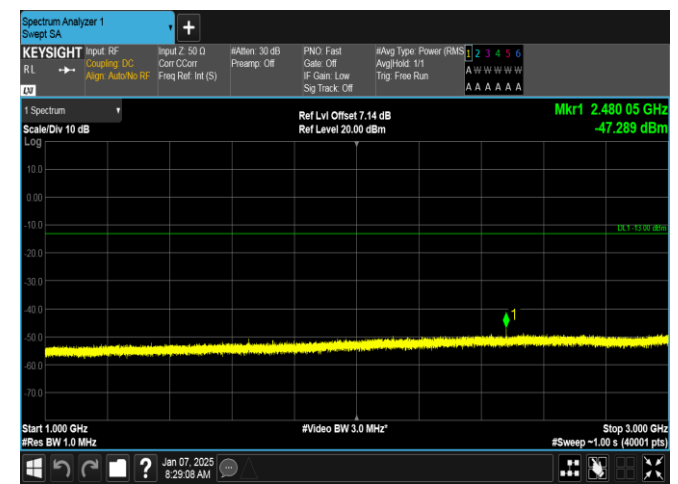
Band5-3MHz-16QAM-20415-1RB#14-1000~3000-PASS
