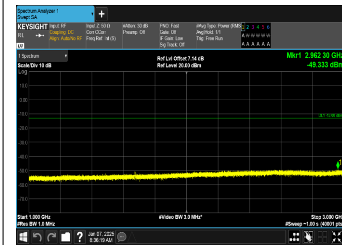
Band5-3MHz-QPSK-20525-15RB#0-1000~3000-PASS
