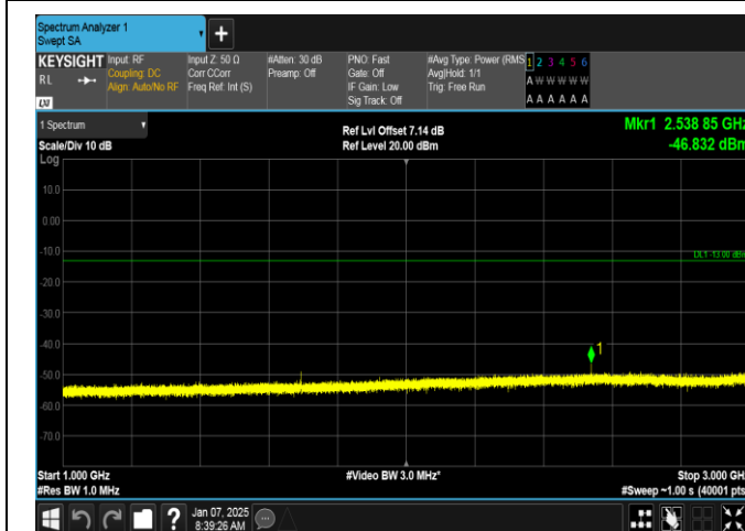
Band5-3MHz-16QAM-20635-1RB#0-1000~3000-PASS
