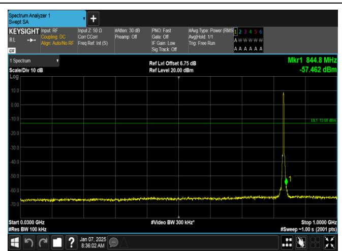
Band5-3MHz-QPSK-20525-15RB#0-30~1000-PASS
