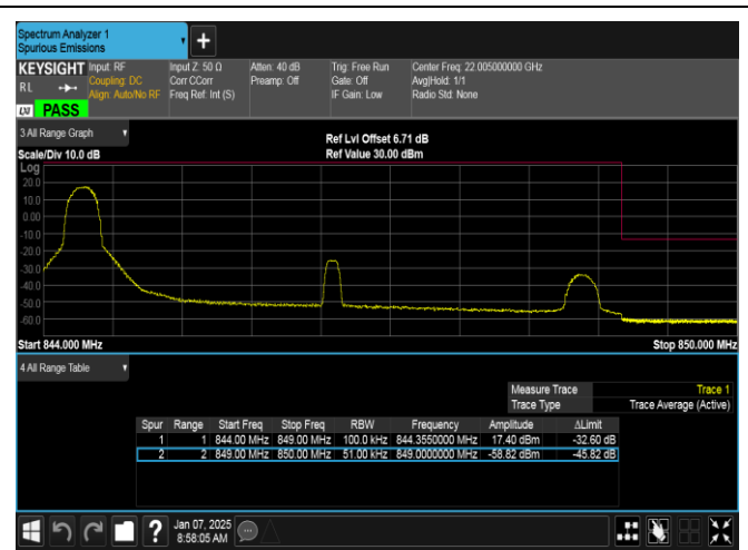
Band5-5MHz-16QAM-20625-1RB#0-PASS
