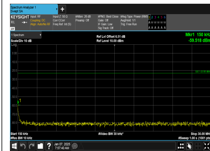
Band5-1.4MHz-QPSK-20525-1RB#0-0.15~30-PASS
