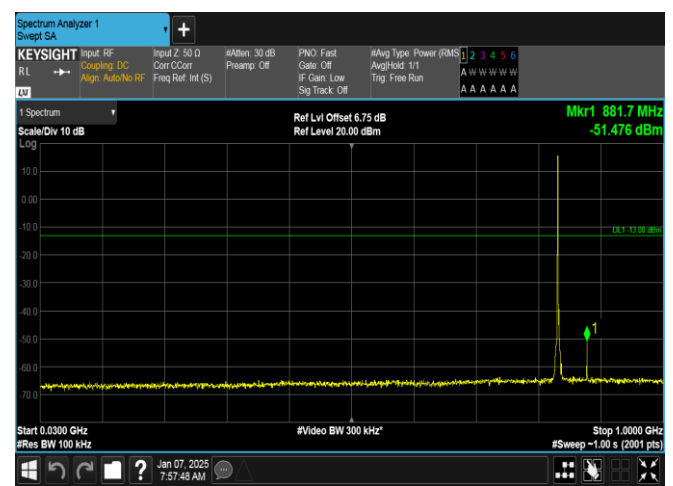
Band5-1.4MHz-QPSK-20525-1RB#0-30~1000-PASS
