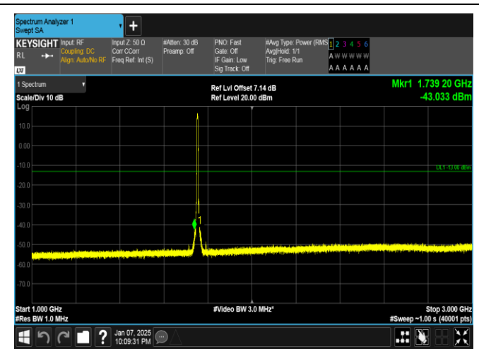
Band4-5MHz-QPSK-20375-25RB#0-1000~3000-PASS
