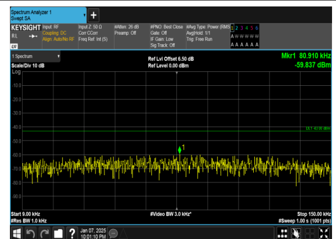
Band4-5MHz-16QAM-20175-1RB#24-0.009~0.15-PASS
