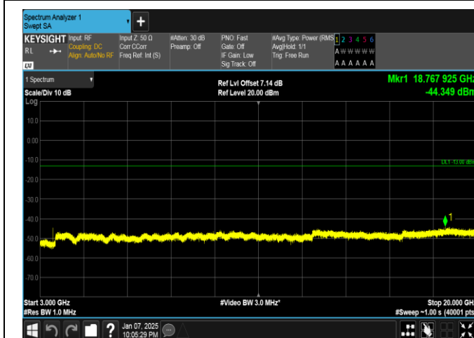
Band4-5MHz-QPSK-20375-1RB#0-3000~20000-PASS
