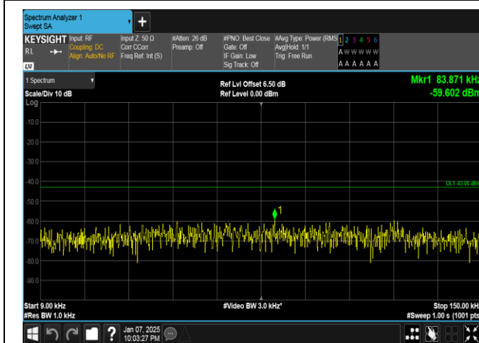
Band4-5MHz-16QAM-20175-25RB#0-0.009~0.15-PASS
