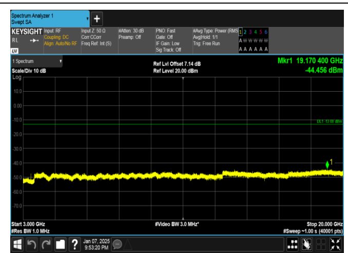
Band4-5MHz-16QAM-19975-1RB#0-3000~20000-PASS
