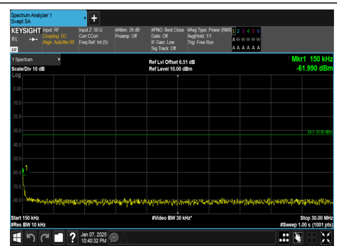
Band4-10MHz-QPSK-20000-1RB#0-0.15~30-PASS
