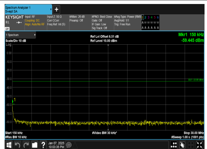
Band4-5MHz-16QAM-20175-25RB#0-0.15~30-PASS
