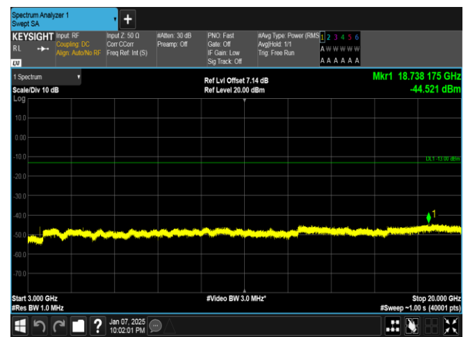
Band4-5MHz-16QAM-20175-1RB#24-3000~20000-PASS
