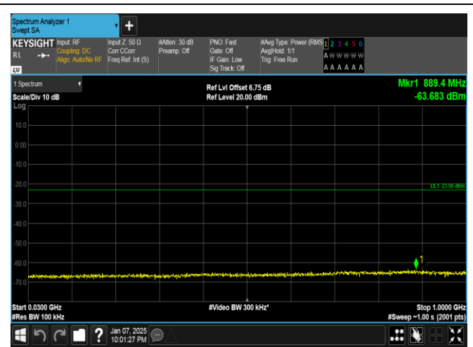
Band4-5MHz-16QAM-20175-1RB#24-30~1000-PASS
