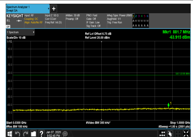
Band4-5MHz-16QAM-19975-1RB#0-30~1000-PASS
