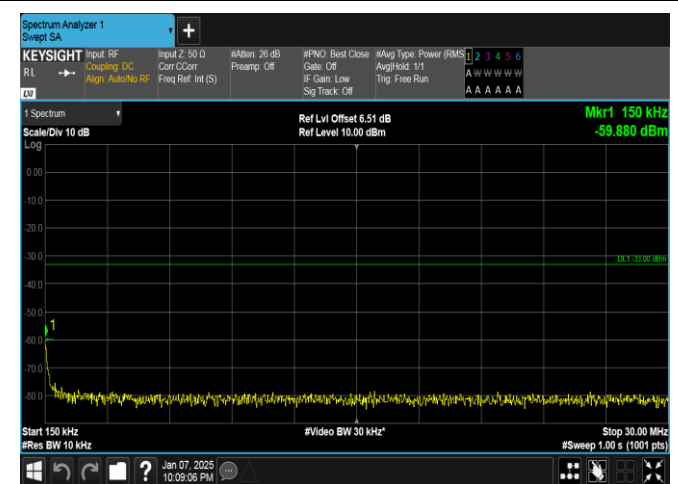
Band4-5MHz-QPSK-20375-25RB#0-0.15~30-PASS
