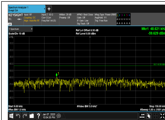
Band4-5MHz-QPSK-20375-1RB#0-0.009~0.15-PASS
