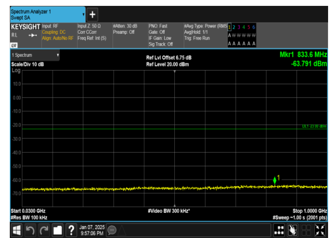
Band4-5MHz-16QAM-19975-25RB#0-30~1000-PASS
