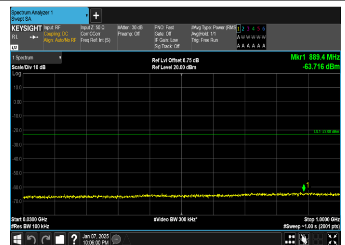
Band4-5MHz-16QAM-20375-1RB#0-30~1000-PASS
