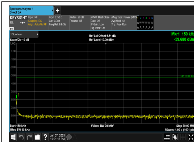
Band4-5MHz-16QAM-20175-1RB#24-0.15~30-PASS
