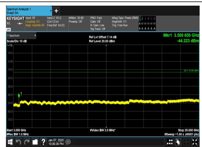
Band4-5MHz-16QAM-20375-1RB#0-3000~20000-PASS
