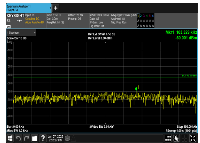
Band4-5MHz-16QAM-19975-1RB#0-0.009~0.15-PASS
