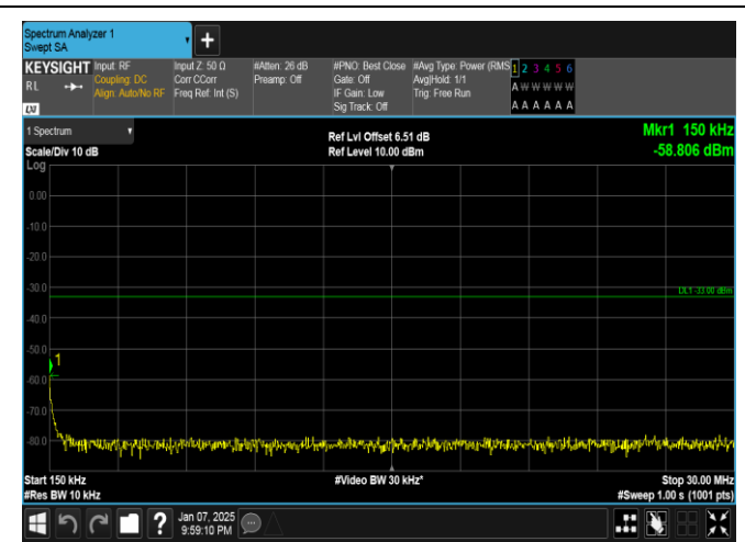
Band4-5MHz-16QAM-20175-1RB#0-0.15~30-PASS
