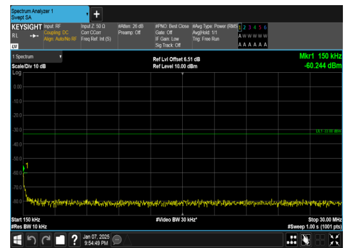
Band4-5MHz-16QAM-19975-1RB#24-0.15~30-PASS
