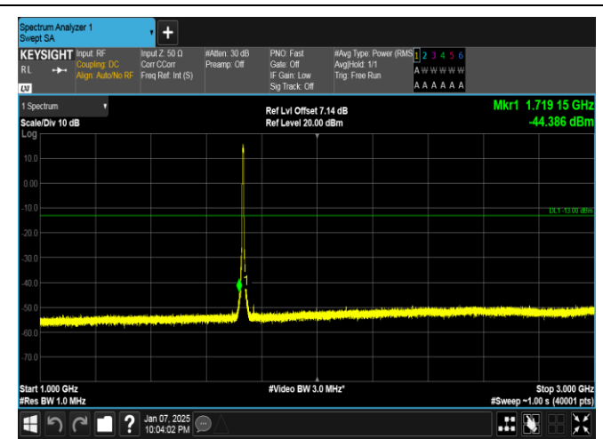
Band4-5MHz-16QAM-20175-25RB#0-1000~3000-PASS
