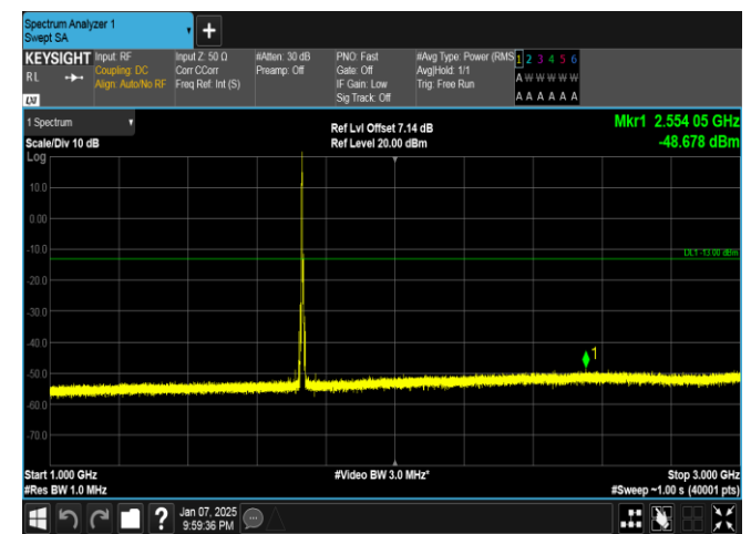
Band4-5MHz-16QAM-20175-1RB#0-1000~3000-PASS
