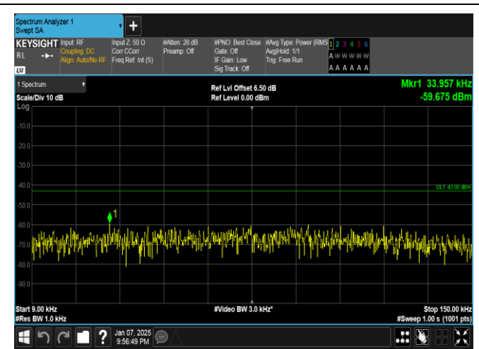
Band4-5MHz-16QAM-19975-25RB#0-0.009~0.15-PASS
