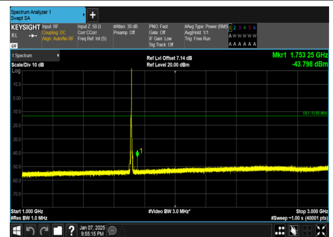
Band4-5MHz-16QAM-19975-1RB#24-1000~3000-PASS
