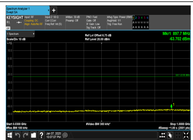
Band4-5MHz-QPSK-20375-1RB#24-30~1000-PASS
