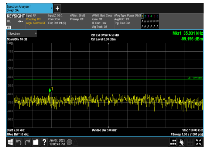
Band4-5MHz-16QAM-20375-1RB#0-0.009~0.15-PASS
