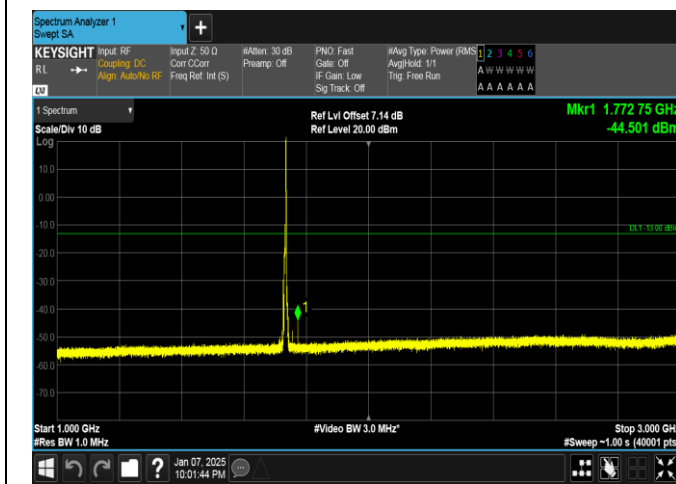
Band4-5MHz-16QAM-20175-1RB#24-1000~3000-PASS
