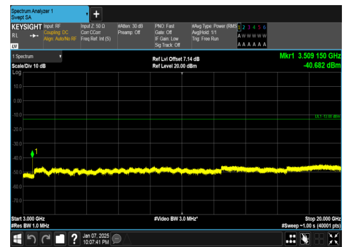
Band4-5MHz-QPSK-20375-1RB#24-3000~20000-PASS
