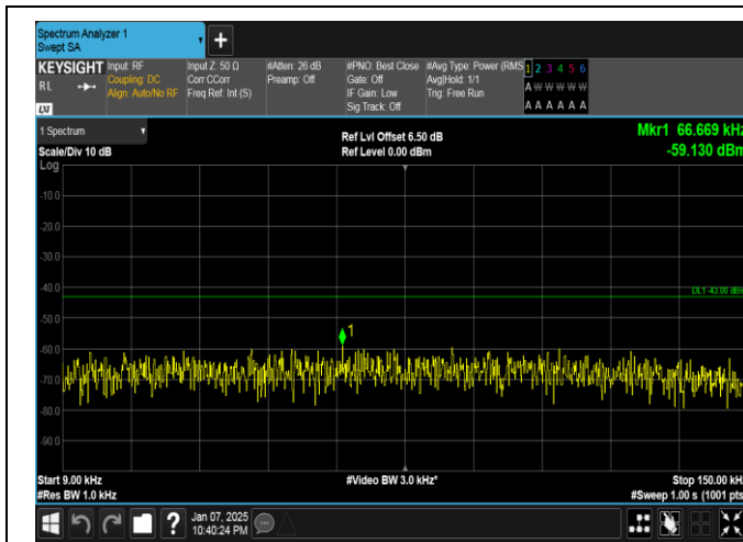
Band4-10MHz-QPSK-20000-1RB#0-0.009~0.15-PASS
