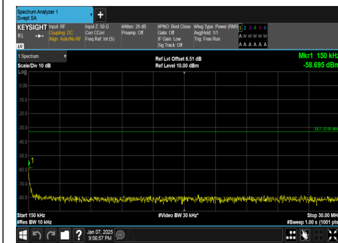
Band4-5MHz-16QAM-19975-25RB#0-0.15~30-PASS
