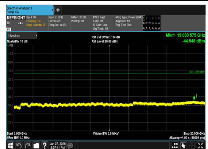
Band4-5MHz-16QAM-19975-25RB#0-3000~20000-PASS
