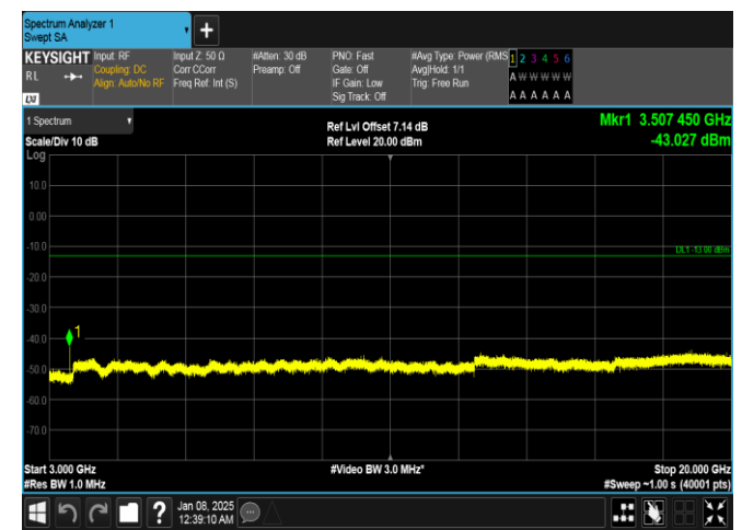
Band4-20MHz-QPSK-20300-1RB#99-3000~20000-PASS
