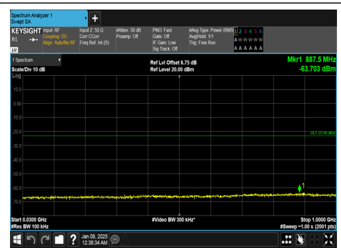
Band4-20MHz-QPSK-20300-1RB#99-30~1000-PASS
