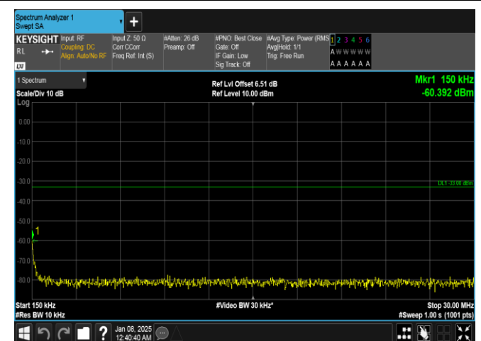
Band4-20MHz-QPSK-20300-100RB#0-0.15~30-PASS
