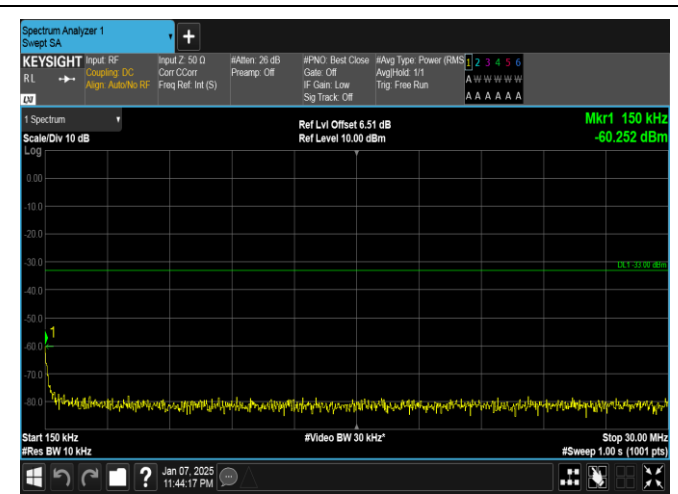
Band4-15MHz-QPSK-20325-1RB#0-0.15~30-PASS
