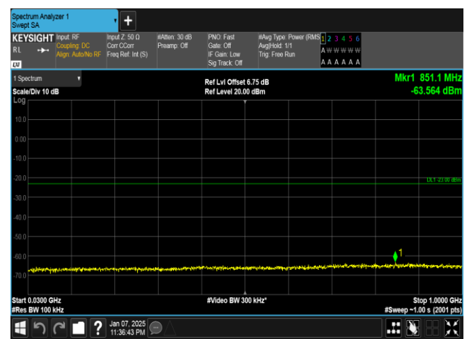
Band4-15MHz-16QAM-20025-75RB#0-30~1000-PASS
