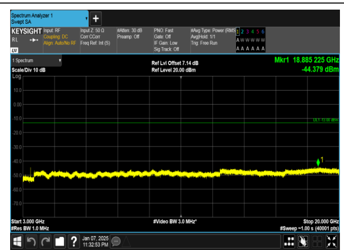
Band4-15MHz-16QAM-2025-1RB#0-3000~20000-PASS
