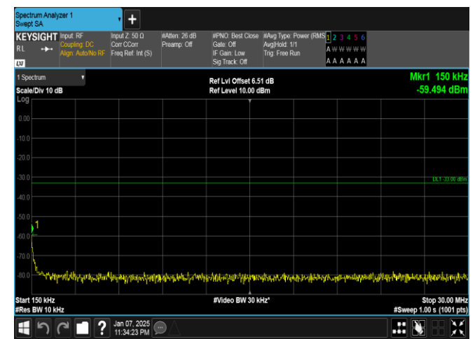
Band4-15MHz-16QAM-2025-1RB#74-0.15~30-PASS
