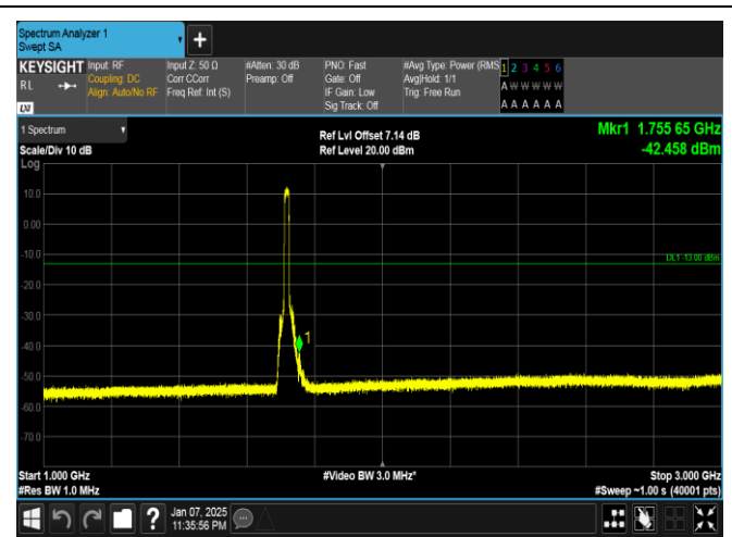
Band4-15MHz-QPSK-20025-75RB#0-1000~3000-PASS
