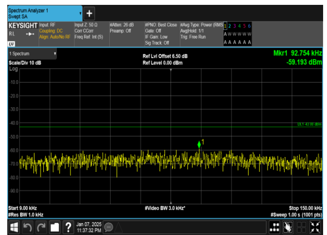
Band4-15MHz-QPSK-20175-1RB#0-0.009~0.15-PASS
