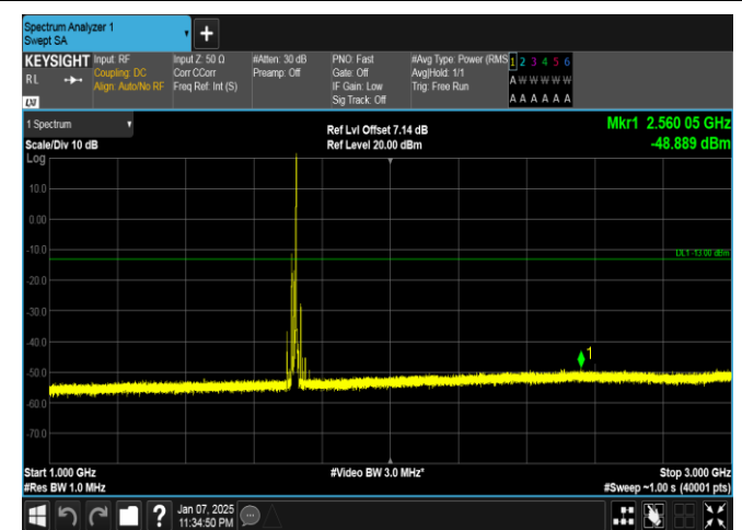
Band4-15MHz-16QAM-2025-1RB#74-1000~3000-PASS
