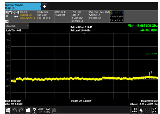
Band4-15MHz-16QAM-20175-1RB#74-3000~20000-PASS
