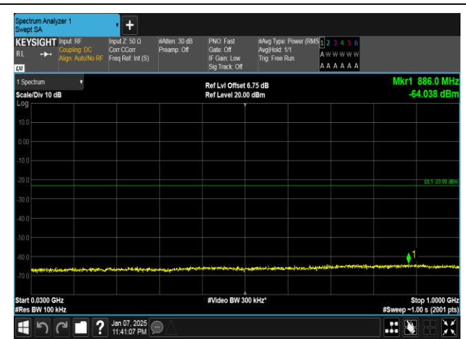
Band4-15MHz-16QAM-20175-1RB#74-30~1000-PASS
