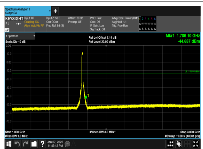
Band4-15MHz-QPSK-20325-75RB#0-1000~3000-PASS
