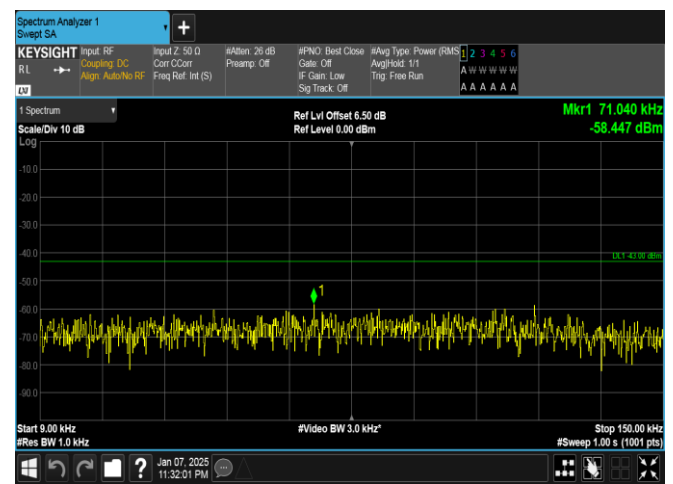
Band4-15MHz-16QAM-20025-1RB#0-0.009~0.15-PASS
