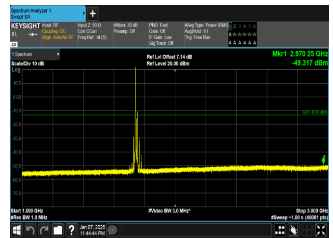
Band4-15MHz-QPSK-20325-1RB#0-1000~3000-PASS
