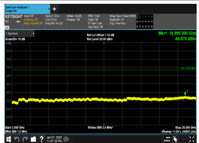
Band4-15MHz-16QAM-20025-75RB#0-3000~20000-PASS
