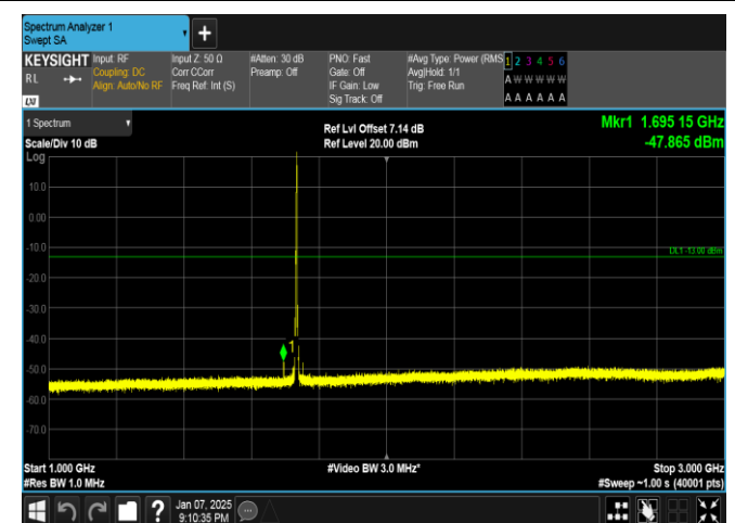
Band4-3MHz-QPSK-20175-1RB#14-1000~3000-PASS
