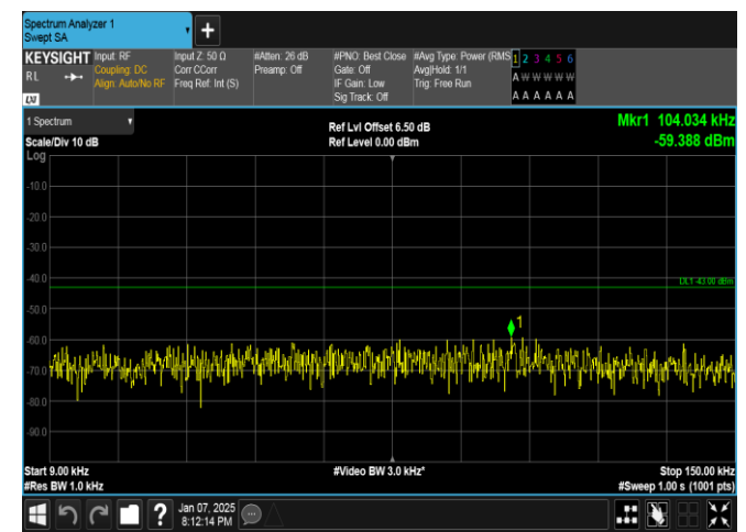
Band4-1.4MHz-16QAM-19957-1RB#0-0.009~0.15-PASS
