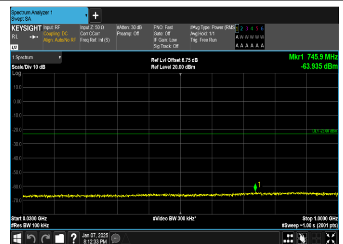
Band4-1.4MHz-16QAM-19957-1RB#0-30~1000-PASS
