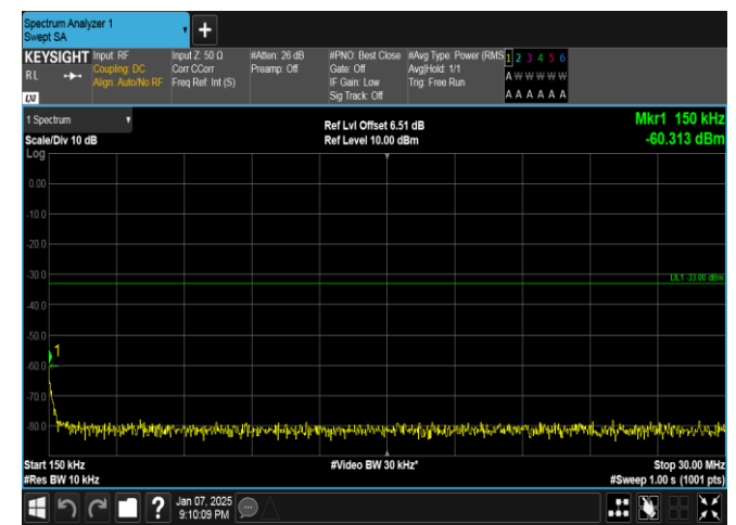
Band4-3MHz-QPSK-20175-1RB#14-0.15~30-PASS
