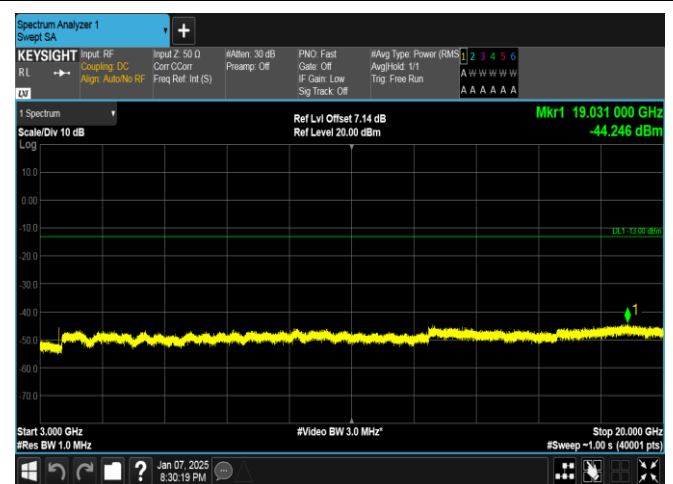
Band4-1.4MHz-16QAM-20393-6RB#0-3000~20000-PASS
