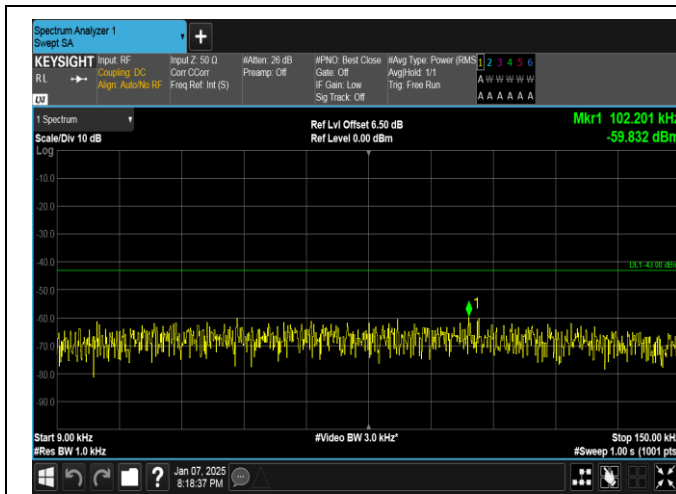
Band4-1.4MHz-16QAM-20175-1RB#0-0.009~0.15-PASS
