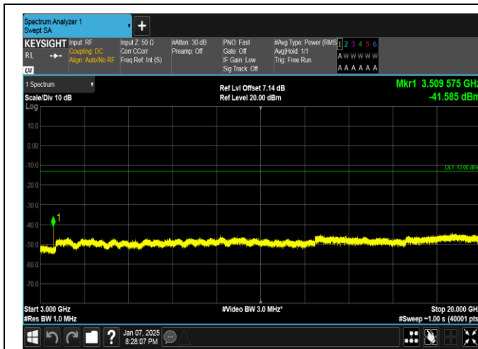
Band4-1.4MHz-16QAM-20393-1RB#5-3000~20000-PASS
