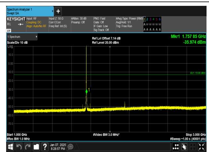
Band4-1.4MHz-QPSK-20393-6RB#0-1000~3000-PASS
