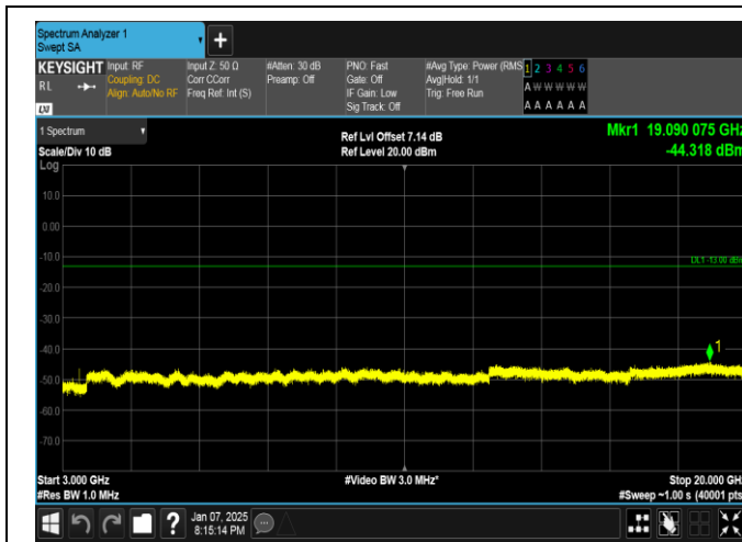
Band4-1.4MHz-16QAM-19957-1RB#5-3000~20000-PASS
