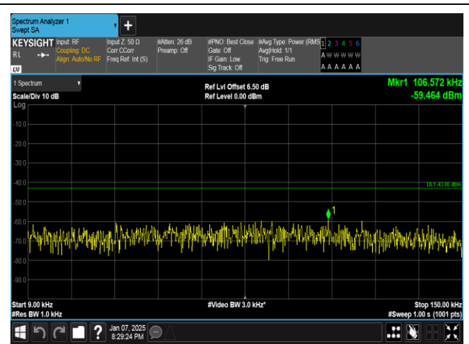
Band4-1.4MHz-16QAM-20393-6RB#0-0.009~0.15-PASS
