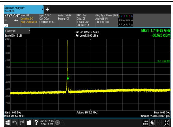
Band4-3MHz-QPSK-19965-15RB#0-1000~3000-PASS
