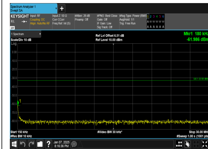
Band4-1.4MHz-16QAM-19957-6RB#0-0.15~30-PASS
