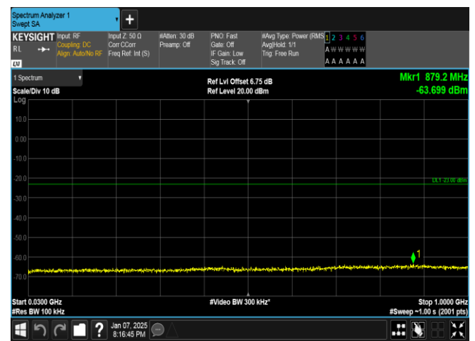
Band4-1.4MHz-16QAM-19957-6RB#0-30~1000-PASS
