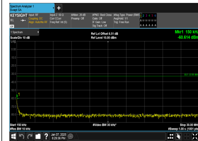
Band4-1.4MHz-16QAM-20393-6RB#0-0.15~30-PASS
