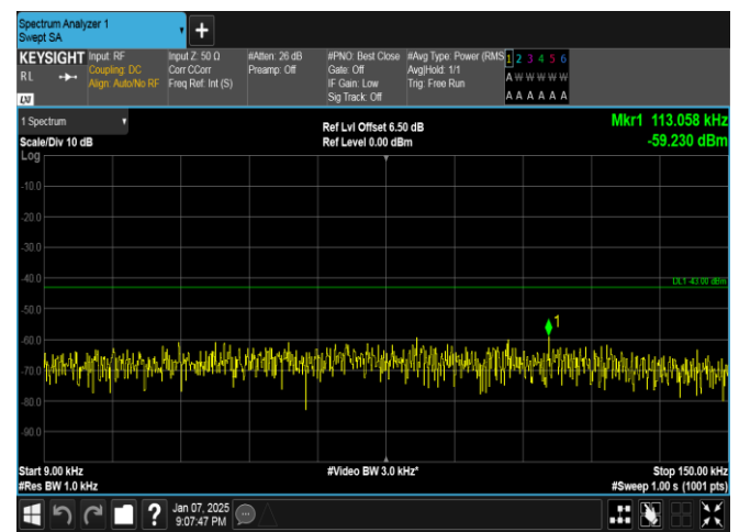
Band4-3MHz-QPSK-20175-1RB#0-0.009~0.15-PASS
