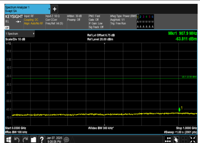
Band4-3MHz-QPSK-20175-1RB#0-30~1000-PASS
