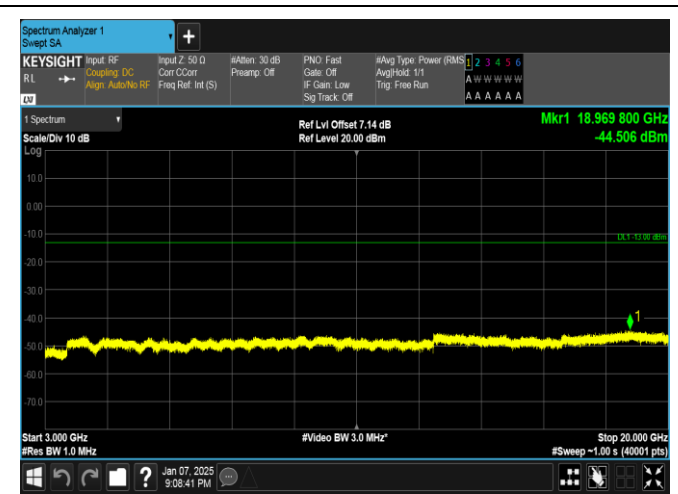
Band4-3MHz-QPSK-20175-1RB#0-3000~20000-PASS
