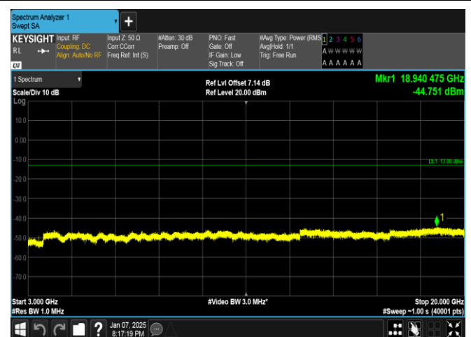
Band4-1.4MHz-16QAM-19957-6RB#0-3000~20000-PASS
