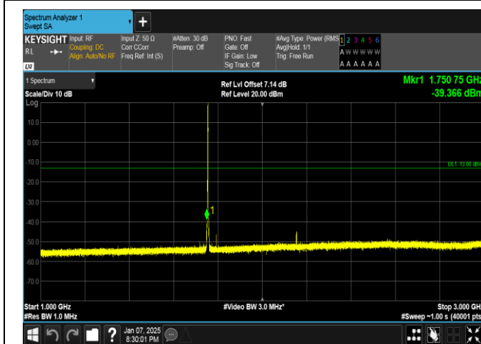
Band4-1.4MHz-16QAM-20393-6RB#0-1000~3000-PASS
