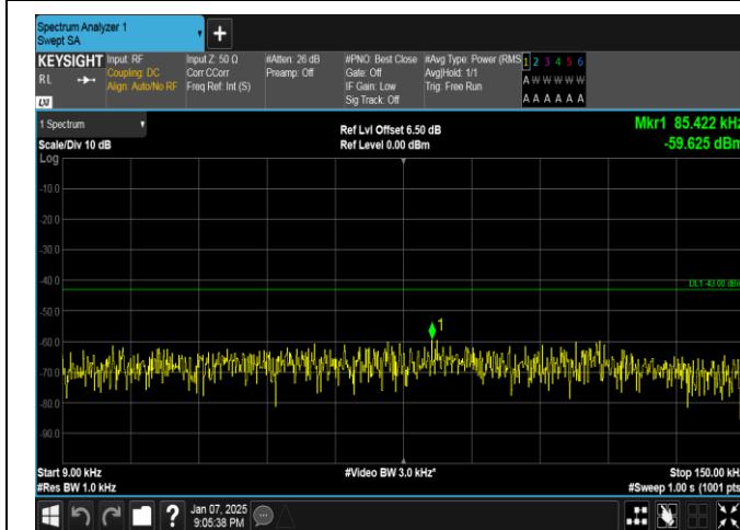
Band4-3MHz-QPSK-19965-15RB#0-0.009~0.15-PASS
