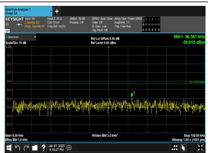
Band4-1.4MHz-16QAM-19957-6RB#0-0.009~0.15-PASS
