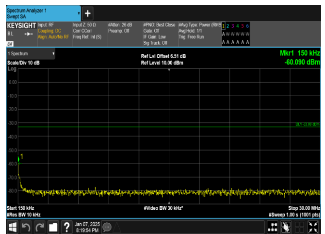
Band4-1.4MHz-QPSK-20175-1RB#5-0.15~30-PASS
