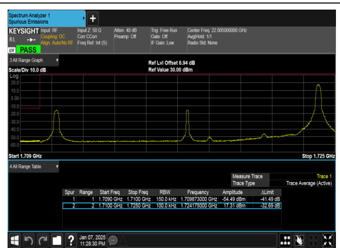
Band4-15MHz-16QAM-20025-1RB#74-PASS
