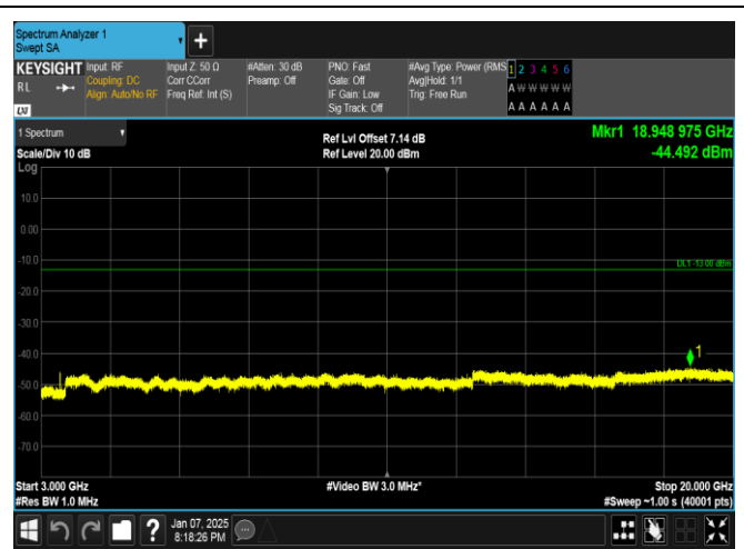
Band4-1.4MHz-QPSK-20175-1RB#0-3000~20000-PASS
