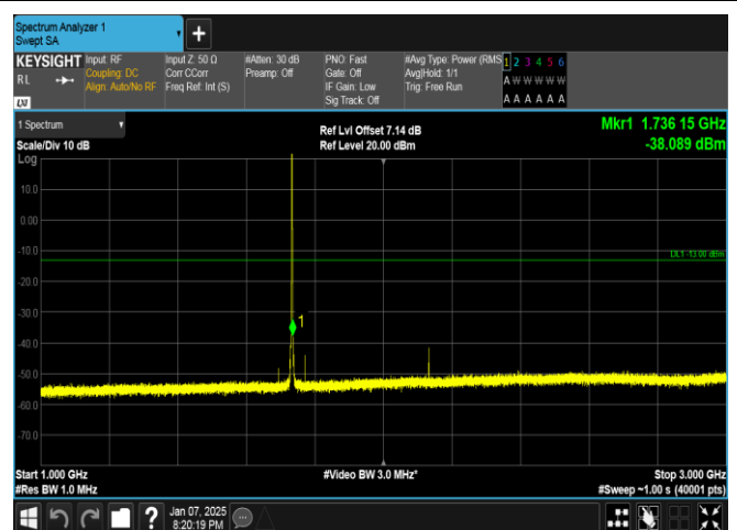
Band4-1.4MHz-QPSK-20175-1RB#5-1000~3000-PASS
