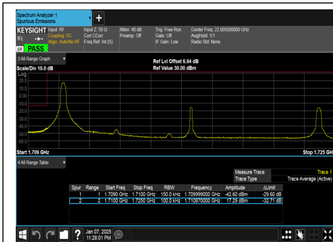
Band4-15MHz-16QAM-20025-1RB#0-PASS
