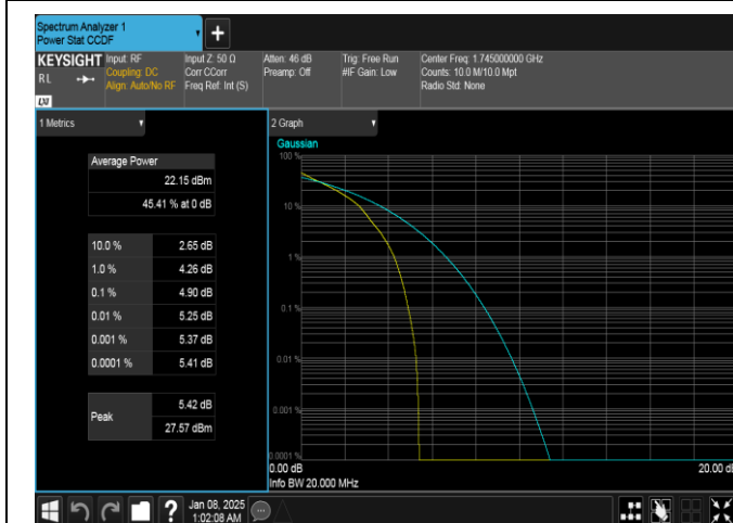
Band4-20MHz-QPSK-20300-1RB#0-PASS
