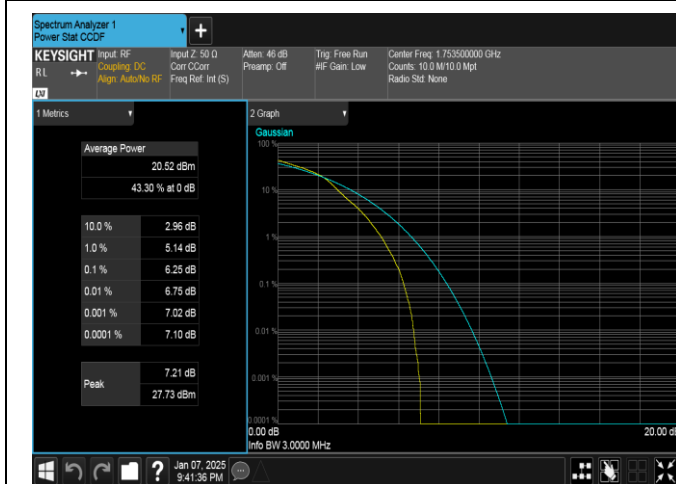
Band4-3MHz-16QAM-20385-1RB#0-PASS
