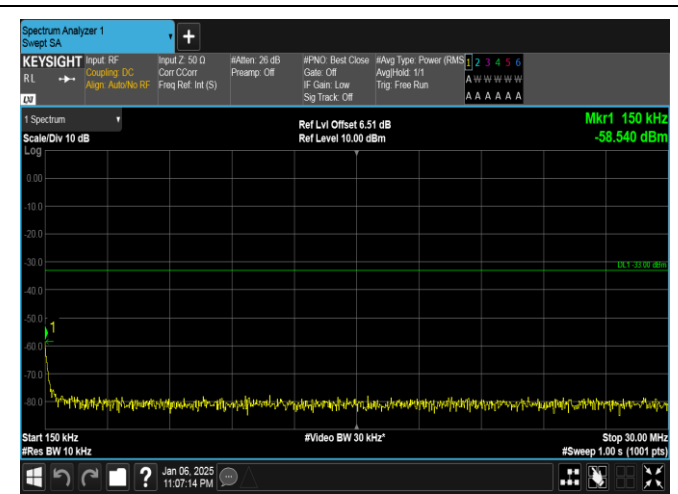
Band2-20MHz-QPSK-18700-1RB#0-0.15~30-PASS
