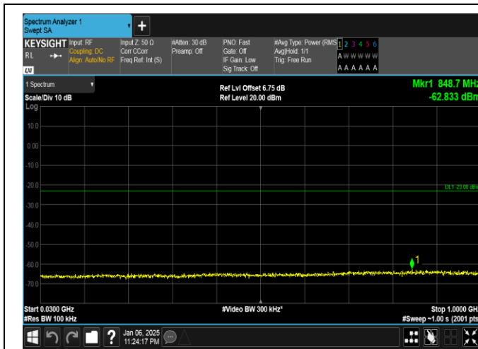
Band2-20MHz-QPSK-19100-100RB#0-30~1000-PASS
