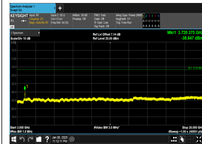
Band2-20MHz-QPSK-18700-100RB#0-3000~20000-PASS
