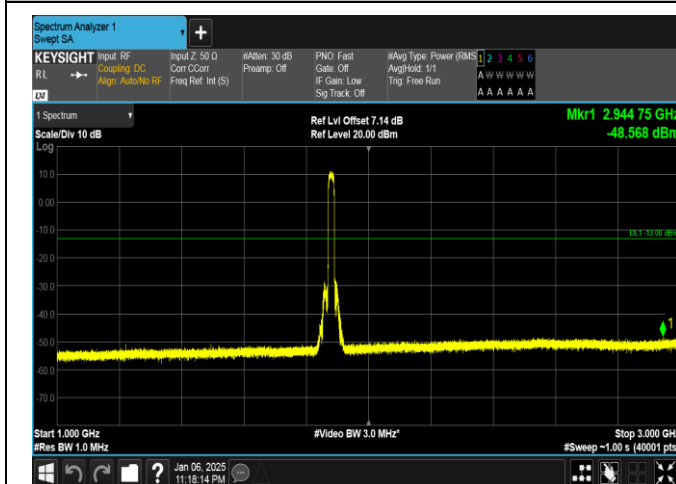
Band2-20MHz-QPSK-18900-100RB#0-1000~3000-PASS
