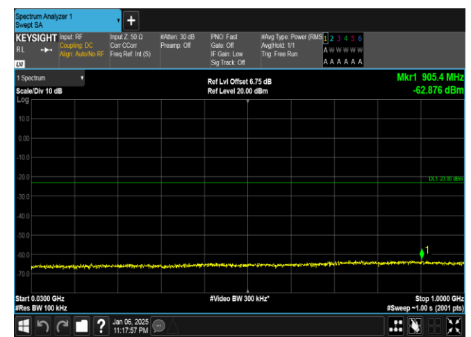
Band2-20MHz-QPSK-18900-100RB#0-30~1000-PASS
