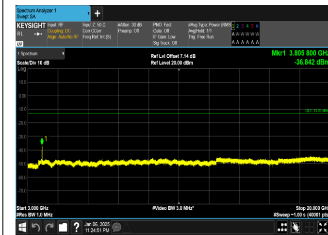
Band2-20MHz-QPSK-19100-100RB#0-3000~20000-PASS
