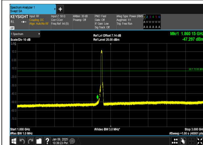
Band2-15MHz-16QAM-19125-75RB#0-1000~3000-PASS
