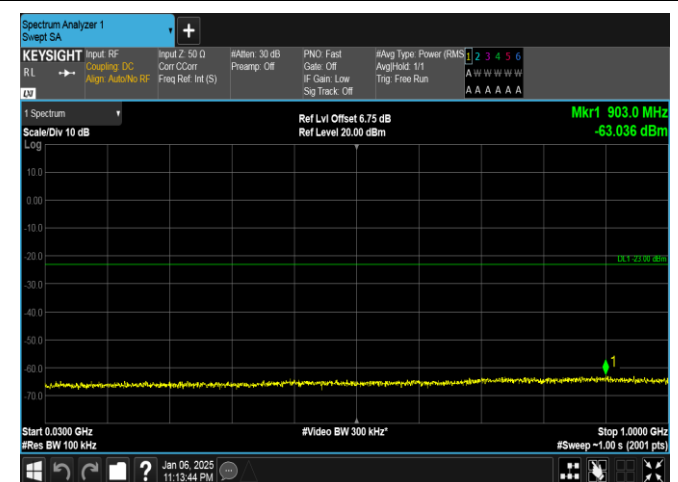
Band2-20MHz-QPSK-18900-1RB#0-30~1000-PASS
