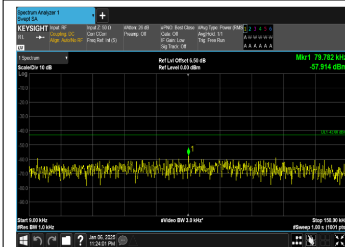
Band2-20MHz-QPSK-19100-100RB#0-0.009~0.15-PASS
