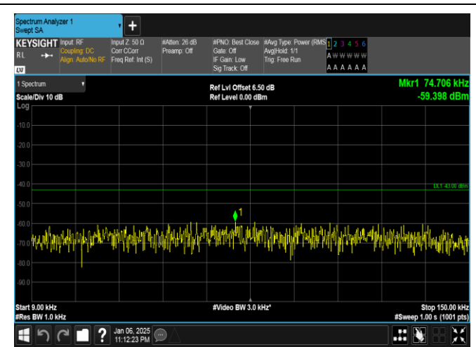
Band2-20MHz-16QAM-18700-100RB#0-0.009~0.15-PASS
