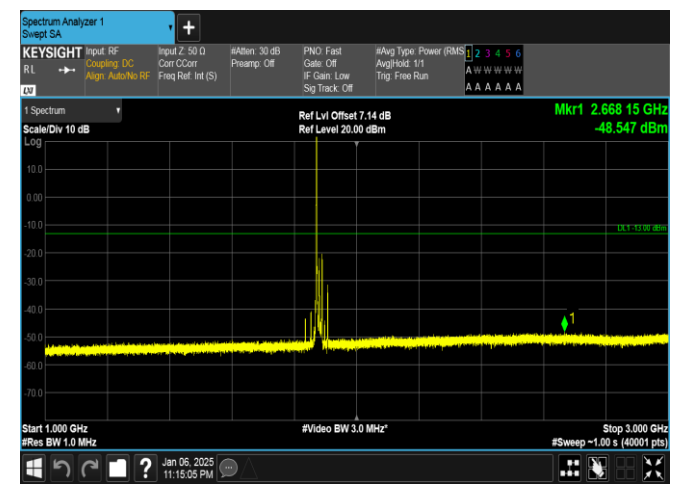
Band2-20MHz-16QAM-18900-1RB#0-1000~3000-PASS
