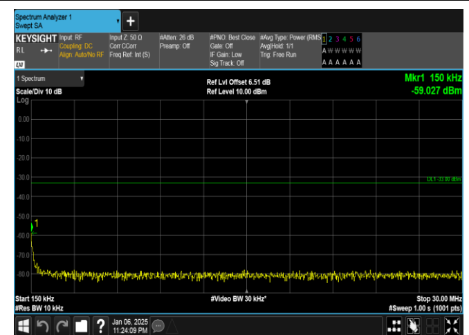
Band2-20MHz-QPSK-19100-100RB#0-0.15~30-PASS
