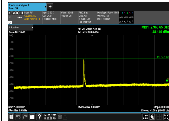
Band2-20MHz-QPSK-19100-1RB#99-1000~3000-PASS
