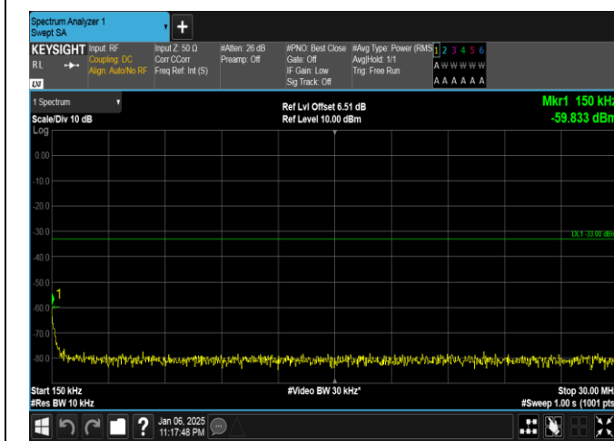
Band2-20MHz-QPSK-18900-100RB#0-0.15~30-PASS
