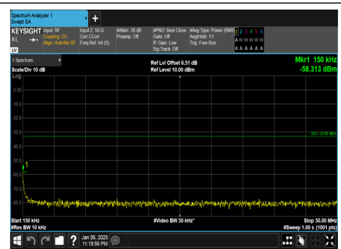
Band2-20MHz-QPSK-19100-1RB#0-0.15~30-PASS
