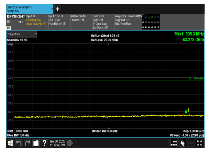
Band2-20MHz-16QAM-18700-100RB#0-30~1000-PASS
