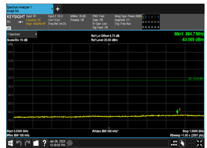
Band2-15MHz-16QAM-19125-75RB#0-30~1000-PASS
