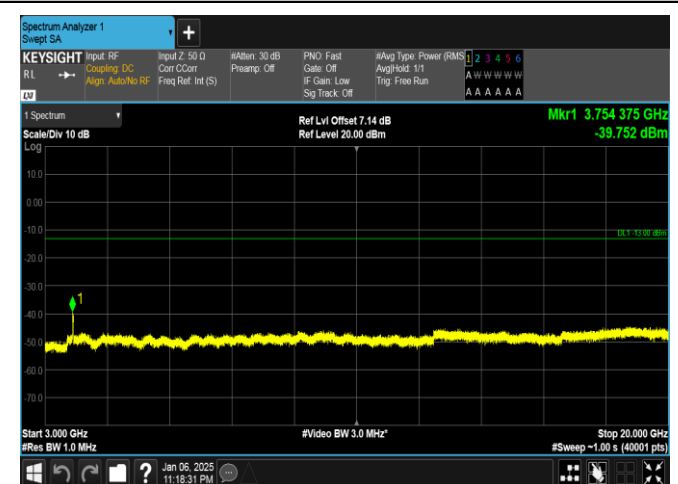
Band2-20MHz-QPSK-18900-100RB#0-3000~20000-PASS
