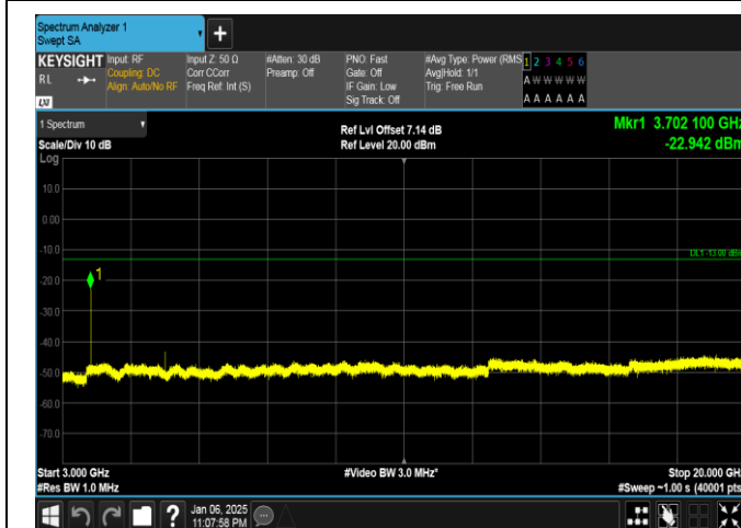
Band2-20MHz-QPSK-18700-1RB#0-3000~20000-PASS
