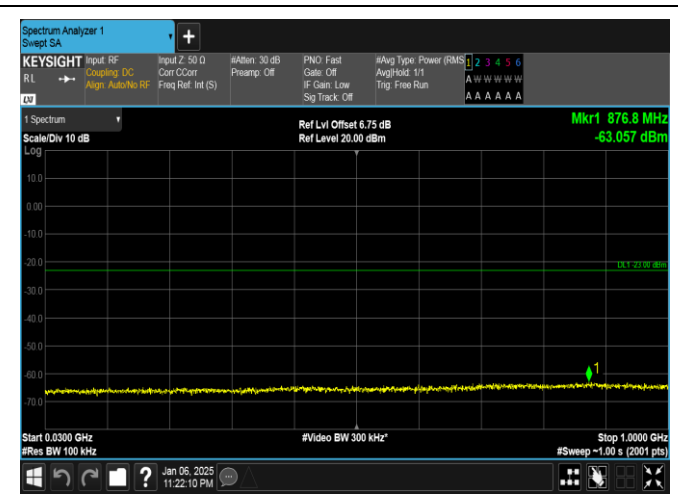
Band2-20MHz-QPSK-19100-1RB#99-30~1000-PASS
