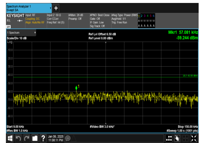
Band2-20MHz-16QAM-18700-1RB#0-0.009~0.15-PASS
