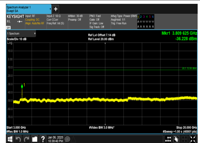
Band2-15MHz-16QAM-19125-75RB#0-3000~20000-PASS
