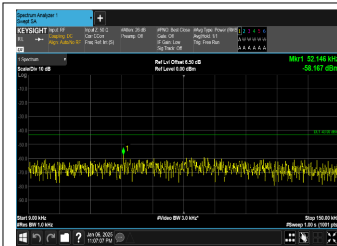
Band2-20MHz-QPSK-18700-1RB#0-0.009~0.15-PASS
