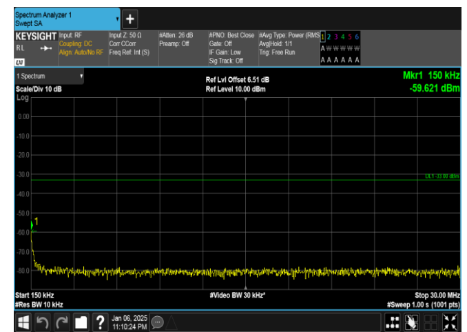
Band2-20MHz-16QAM-18700-1RB#99-0.15~30-PASS
