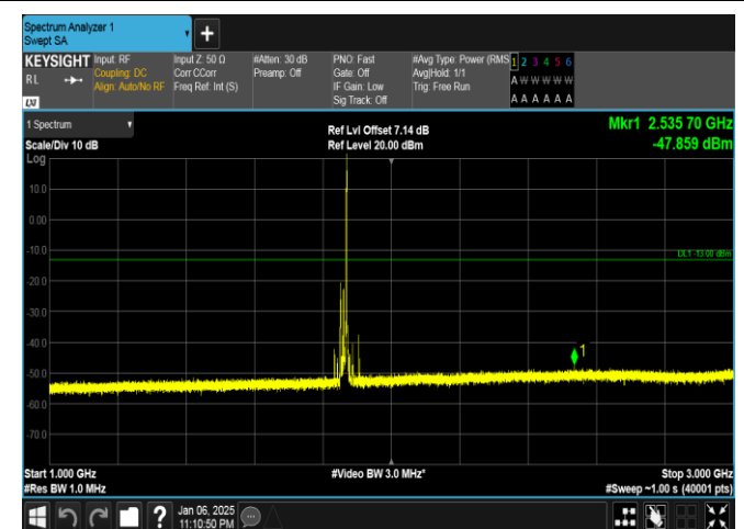
Band2-20MHz-16QAM-18700-1RB#99-1000~3000-PASS
