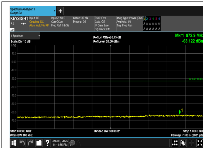
Band2-20MHz-QPSK-18700-100RB#0-30~1000-PASS
