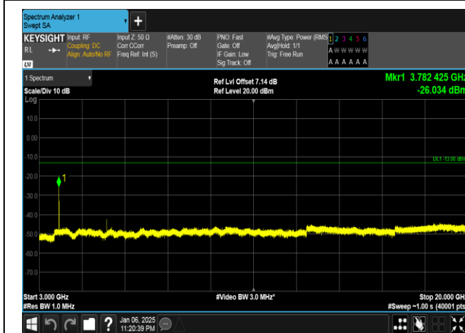
Band2-20MHz-QPSK-19100-1RB#0-3000~20000-PASS
