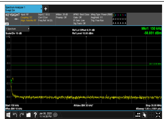
Band2-20MHz-16QAM-18900-1RB#0-0.15~30-PASS
