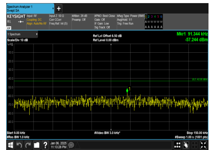
Band2-20MHz-QPSK-18900-1RB#0-0.009~0.15-PASS
