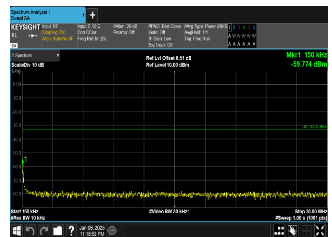
Band2-20MHz-16QAM-18900-100RB#0-0.15~30-PASS
