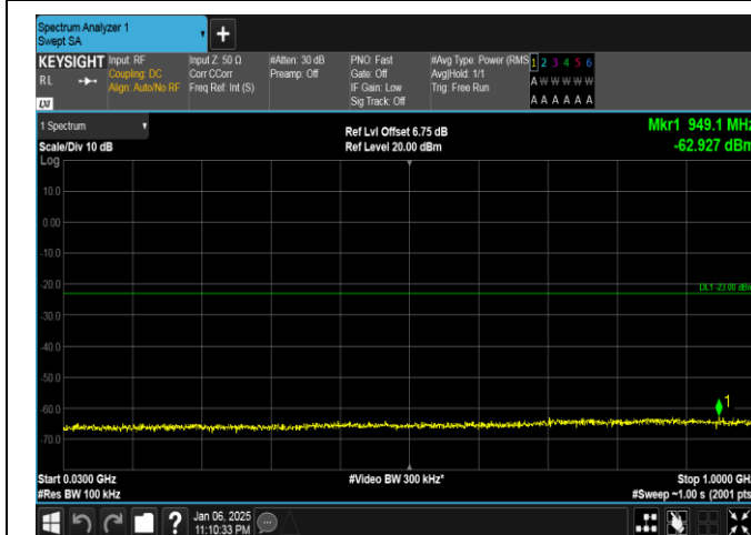
Band2-20MHz-16QAM-18700-1RB#99-30~1000-PASS
