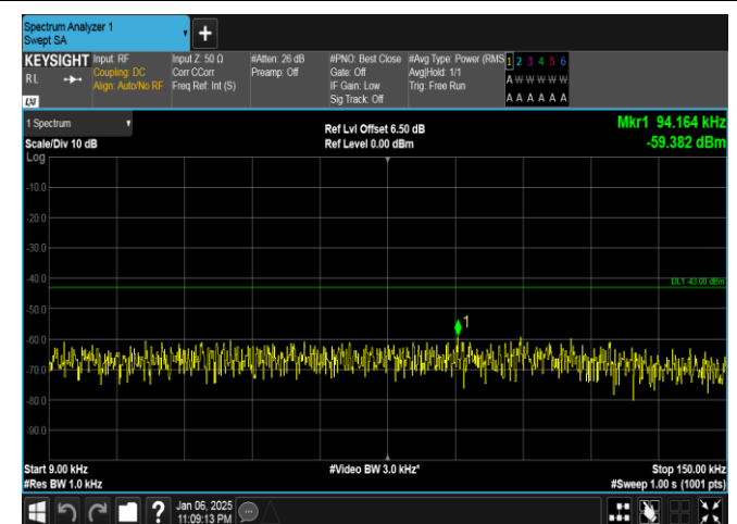
Band2-20MHz-QPSK-18700-1RB#99-0.009~0.15-PASS
