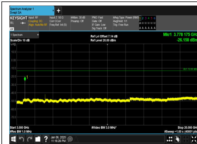
Band2-20MHz-QPSK-18900-1RB#99-3000~20000-PASS
