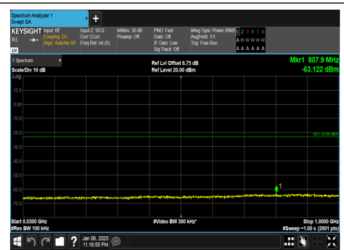
Band2-20MHz-16QAM-18900-1RB#99-30~1000-PASS
