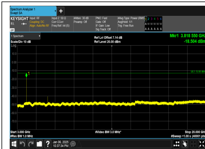
Band2-15MHz-16QAM-19125-1RB#74-3000~20000-PASS
