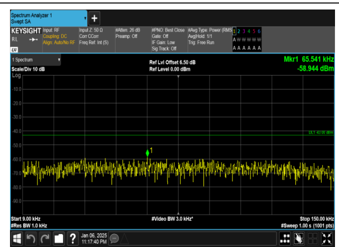
Band2-20MHz-QPSK-18900-100RB#0-0.009~0.15-PASS
