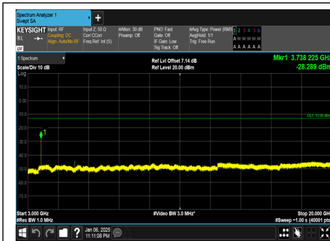
Band2-20MHz-16QAM-18700-1RB#99-3000~20000-PASS
