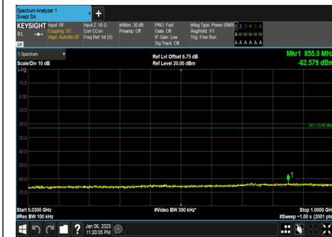
Band2-20MHz-QPSK-19100-1RB#0-30~1000-PASS
