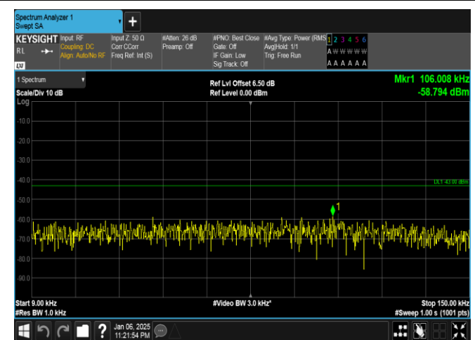
Band2-20MHz-QPSK-19100-1RB#99-0.009~0.15-PASS
