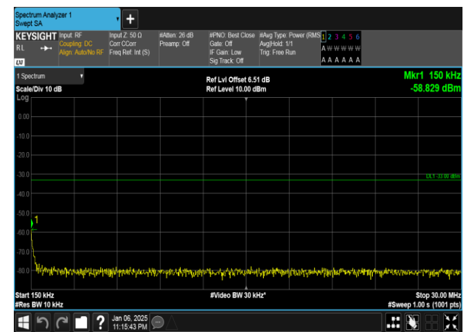
Band2-20MHz-QPSK-18900-1RB#99-0.15~30-PASS
