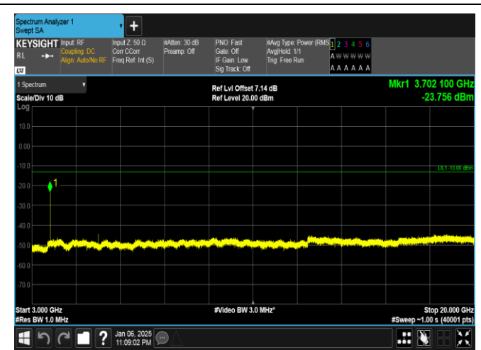
Band2-20MHz-16QAM-18700-1RB#0-3000~20000-PASS
