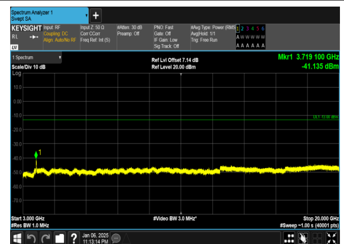
Band2-20MHz-16QAM-18700-100RB#0-3000~20000-PAS
