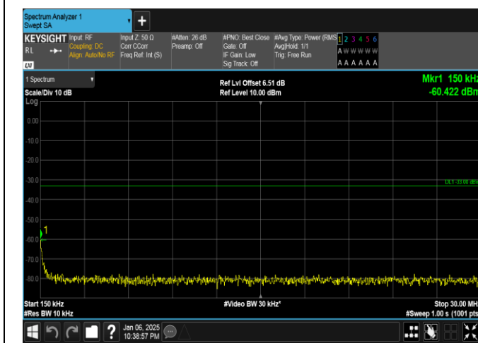
Band2-15MHz-16QAM-19125-75RB#0-0.15~30-PASS
