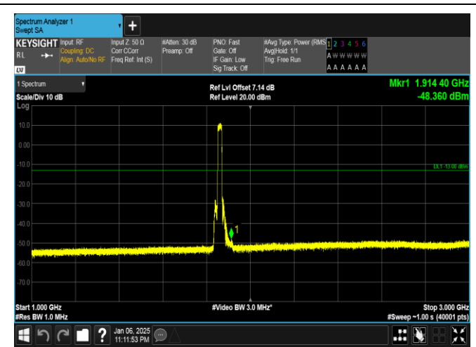
Band2-20MHz-QPSK-18700-100RB#0-1000~3000-PASS
