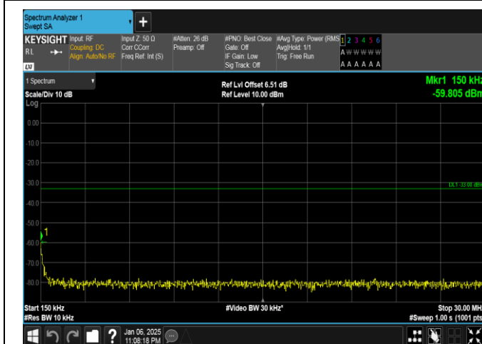
Band2-20MHz-16QAM-18700-1RB#0-0.15~30-PASS
