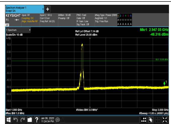
Band2-20MHz-QPSK-19100-100RB#0-1000~3000-PASS
