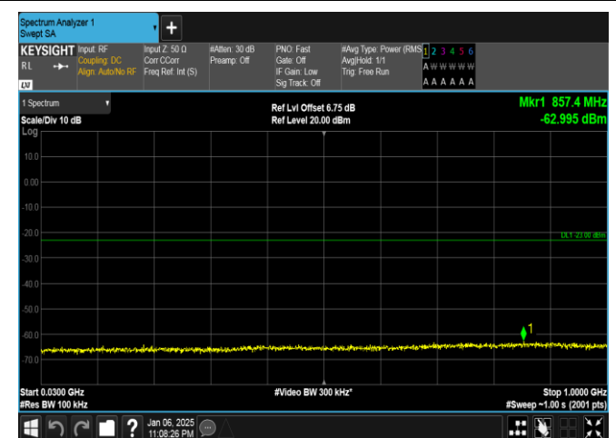
Band2-20MHz-16QAM-18700-1RB#0-30~1000-PASS
