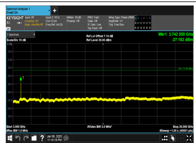
Band2-20MHz-QPSK-18900-1RB#0-3000~20000-PASS
