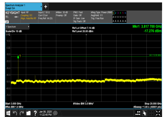
Band2-20MHz-QPSK-19100-1RB#99-3000~20000-PASS
