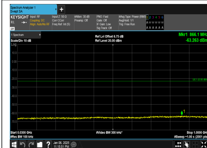
Band2-20MHz-QPSK-18900-1RB#99-30~1000-PASS
