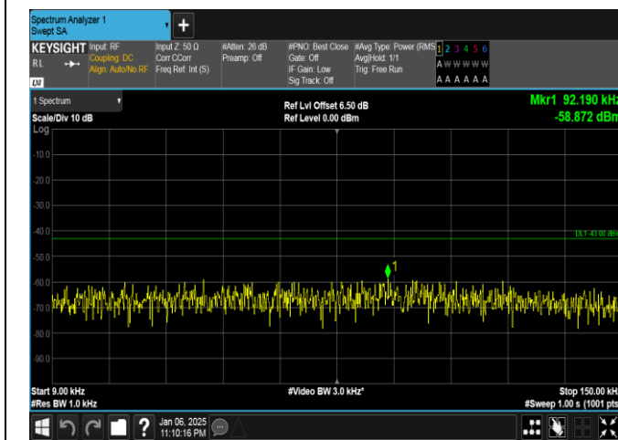
Band2-20MHz-16QAM-18700-1RB#99-0.009~0.15-PASS
