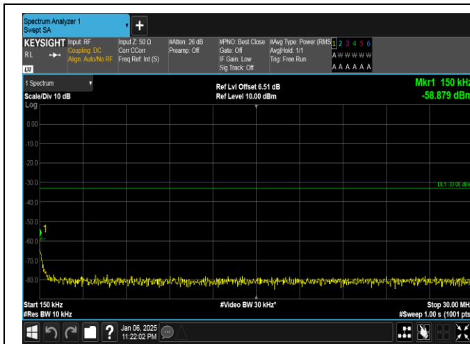
Band2-20MHz-QPSK-19100-1RB#99-0.15~30-PASS
