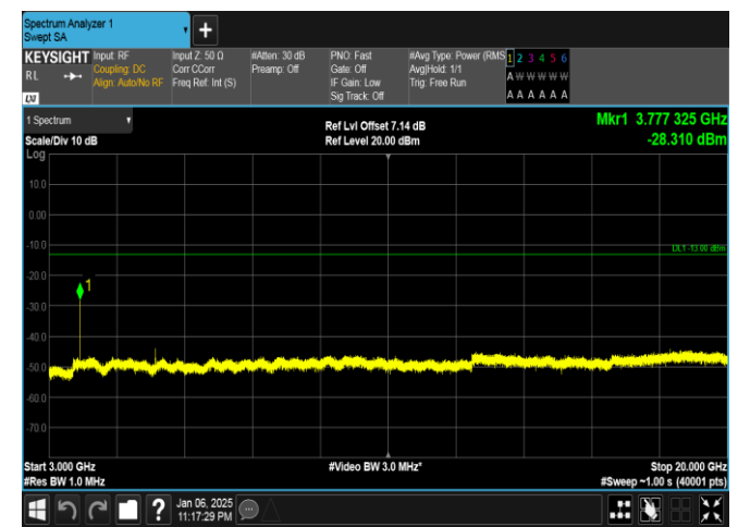
Band2-20MHz-16QAM-18900-1RB#99-3000~20000-PASS
