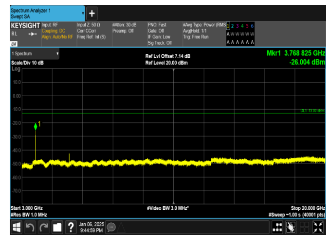
Band2-10MHz-16QAM-18900-1RB#49-3000~20000-PASS
