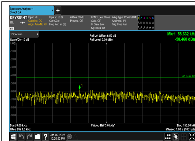
Band2-15MHz-QPSK-18675-1RB#0-0.009~0.15-PASS
