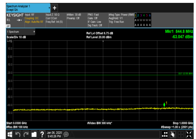
Band2-10MHz-QPSK-18900-50RB#0-30~1000-PASS
