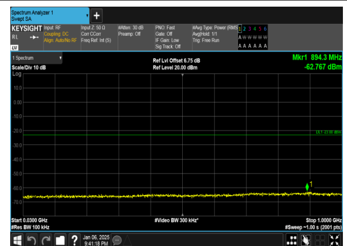
Band2-10MHz-QPSK-18900-1RB#0-30~1000-PASS
