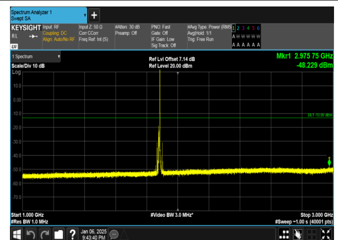
Band2-10MHz-QPSK-18900-1RB#49-1000~3000-PASS
