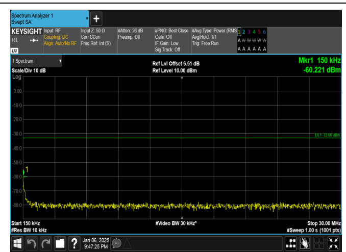
Band2-10MHz-QPSK-19150-1RB#0-0.15~30-PASS
