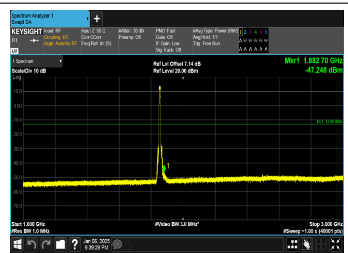
Band2-10MHz-QPSK-18650-50RB#0-1000~3000-PASS
