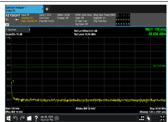
Band2-15MHz-QPSK-18675-1RB#0-0.15~30-PASS
