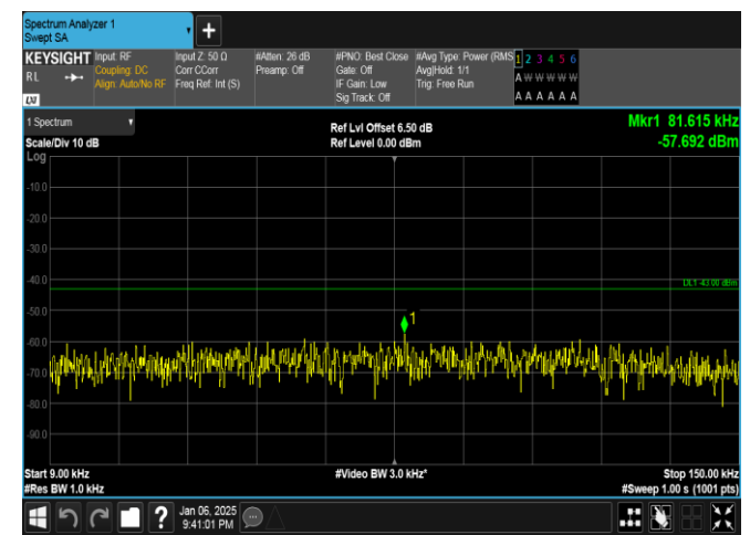
Band2-10MHz-QPSK-18900-1RB#0-0.009~0.15-PASS
