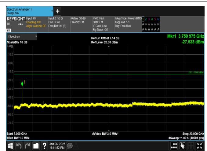
Band2-10MHz-QPSK-18900-1RB#0-3000~20000-PASS
