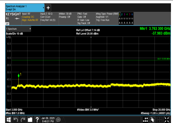
Band2-10MHz-QPSK-18900-50RB#0-3000~20000-PASS
