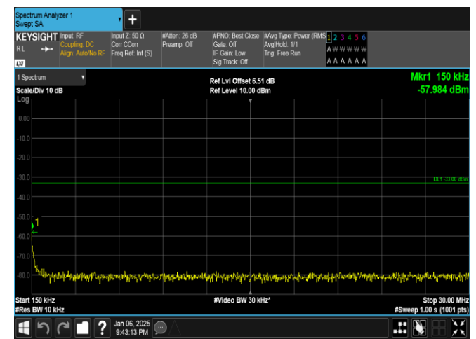
Band2-10MHz-QPSK-18900-1RB#49-0.15~30-PASS
