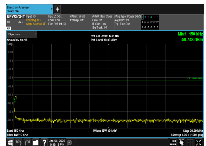
Band2-10MHz-16QAM-18900-50RB#0-0.15~30-PASS
