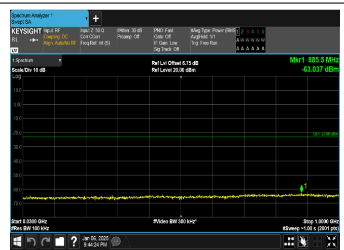
Band2-10MHz-16QAM-18900-1RB#49-30~1000-PASS
