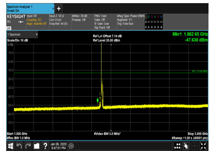
Band2-10MHz-QPSK-19150-1RB#0-1000~3000-PASS
