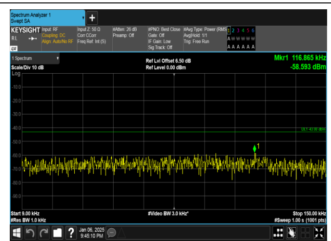
Band2-10MHz-QPSK-18900-50RB#0-0.009~0.15-PASS
