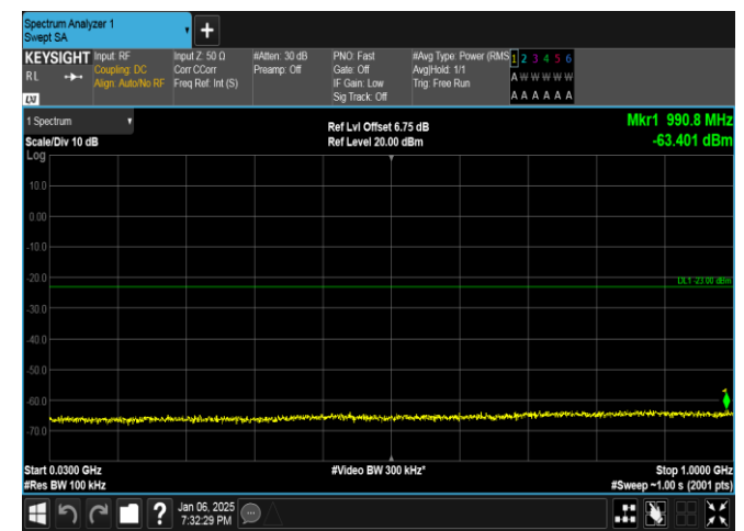
Band2-1.4MHz-16QAM-19193-6RB#0-30~1000-PASS
