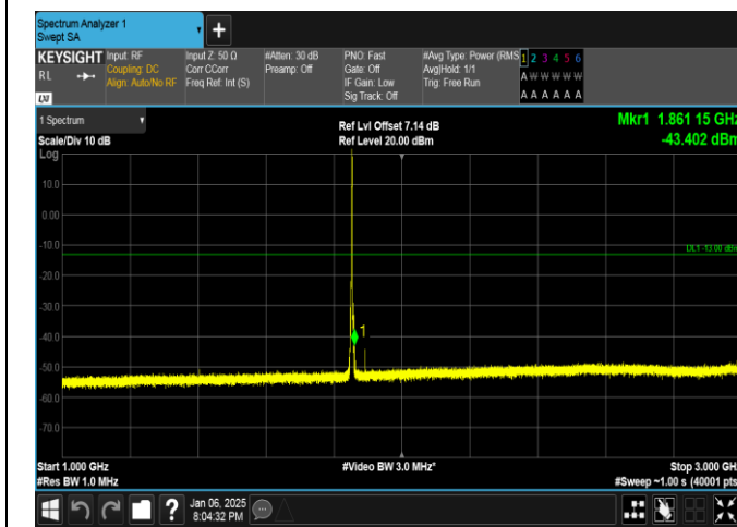
Band2-3MHz-QPSK-18615-1RB#14-1000~3000-PASS
