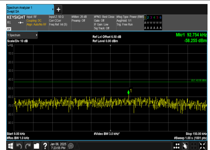
Band2-1.4MHz-16QAM-18900-1RB#5-0.009~0.15-PASS
