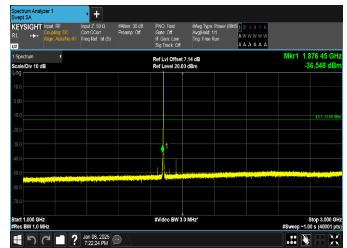
Band2-1.4MHz-16QAM-18900-1RB#0-1000~3000-PASS
