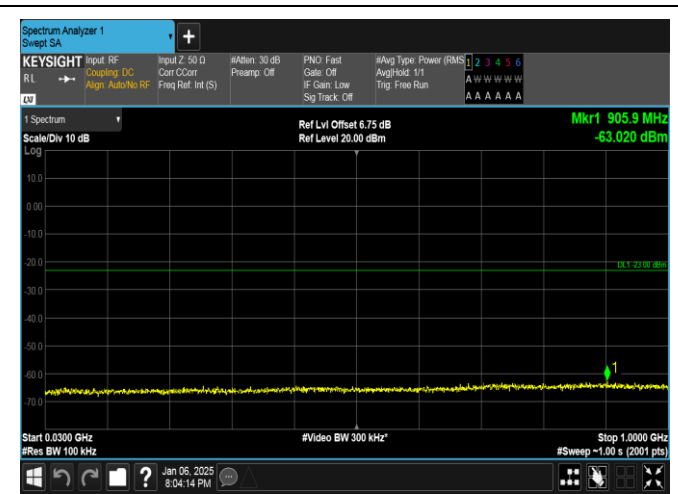
Band2-3MHz-QPSK-18615-1RB#14-30~1000-PASS
