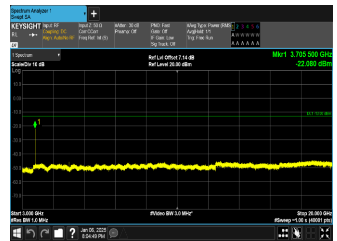
Band2-3MHz-QPSK-18615-1RB#14-3000~20000-PASS
