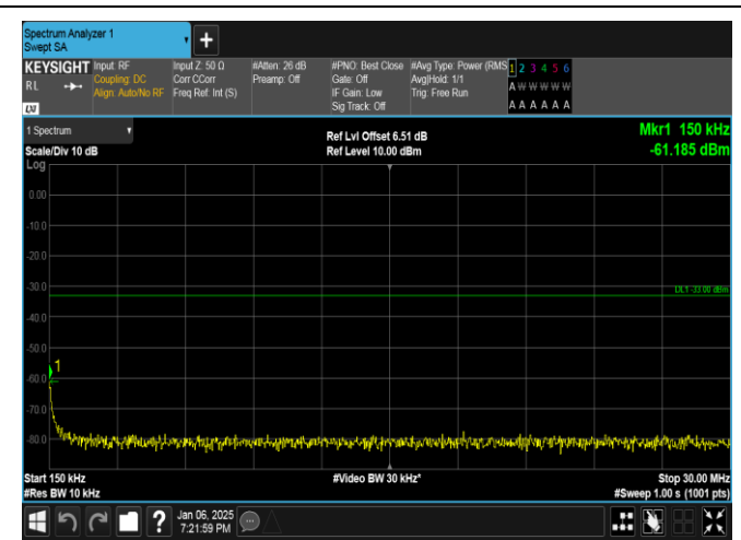
Band2-1.4MHz-16QAM-18900-1RB#0-0.15~30-PASS
