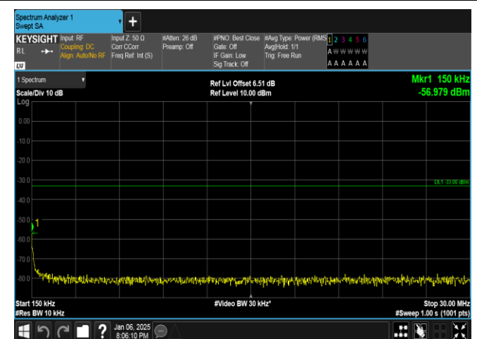
Band2-3MHz-QPSK-18615-15RB#0-0.15~30-PASS
