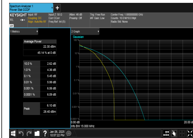
Band2-15MHz-QPSK-18900-1RB#0-PASS
