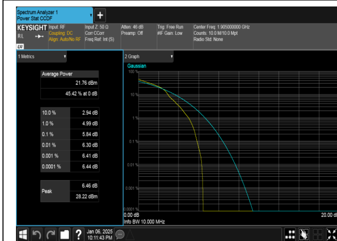
Band2-10MHz-16QAM-19150-1RB#0-PASS
