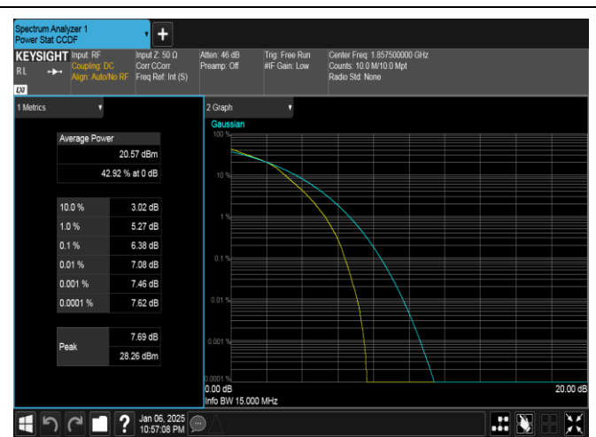
Band2-15MHz-16QAM-18675-75RB#0-PASS
