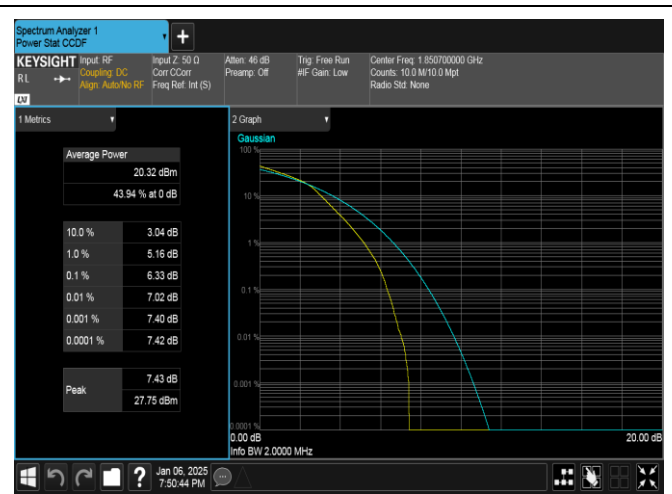
Band2-1.4MHz-16QAM-18607-6RB#0-PASS
