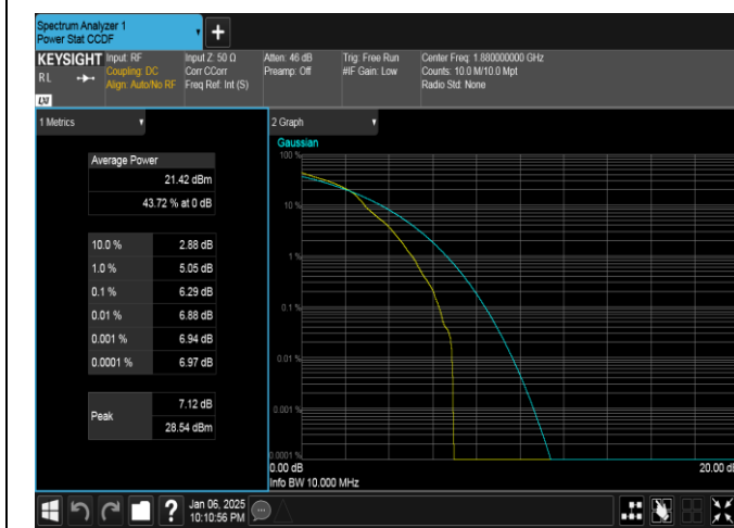
Band2-10MHz-16QAM-18900-1RB#0-PASS
