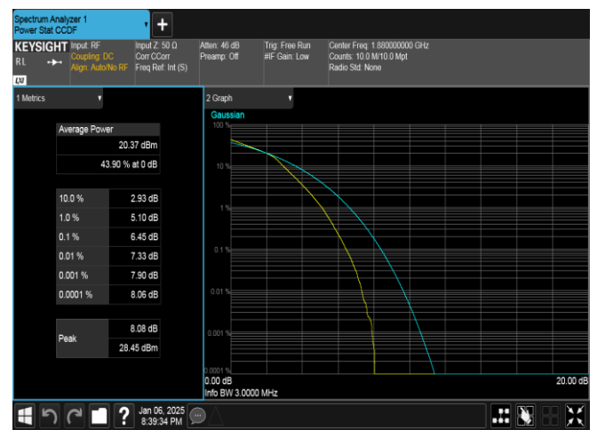
Band2-3MHz-16QAM-18900-15RB#0-PASS
