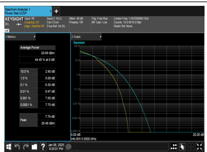
Band2-5MHz-16QAM-18625-25RB#0-PASS
