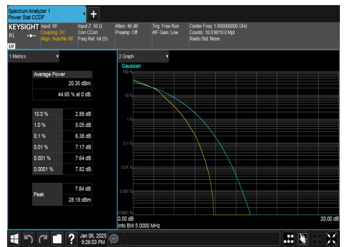
Band2-5MHz-16QAM-18900-25RB#0-PASS
