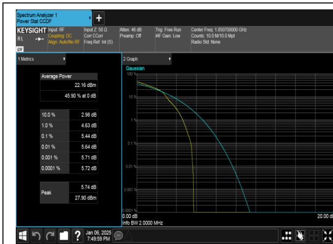
Band2-1.4MHz-16QAM-18607-1RB#0-PASS
