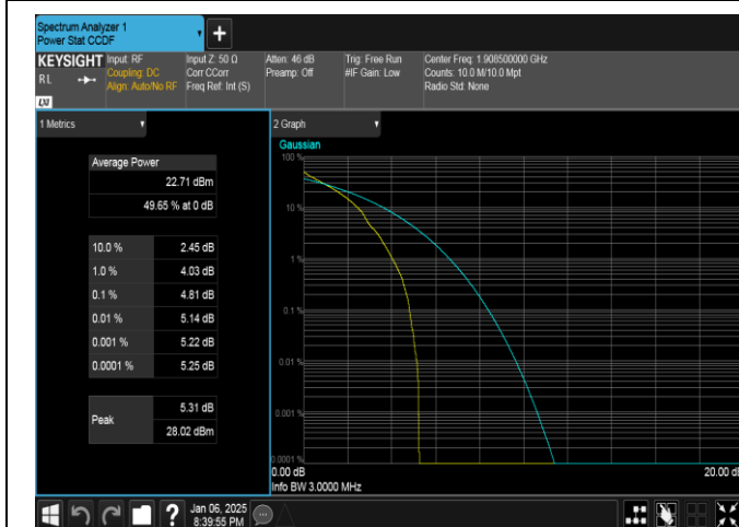
Band2-3MHz-QPSK-19185-1RB#0-PASS
