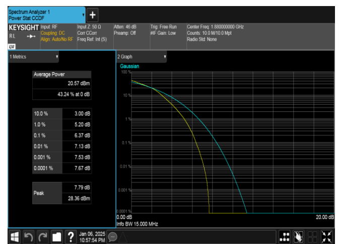
Band2-15MHz-16QAM-18900-75RB#0-PASS
