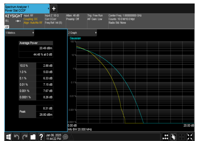
Band2-20MHz-16QAM-18900-100RB#0-PASS
