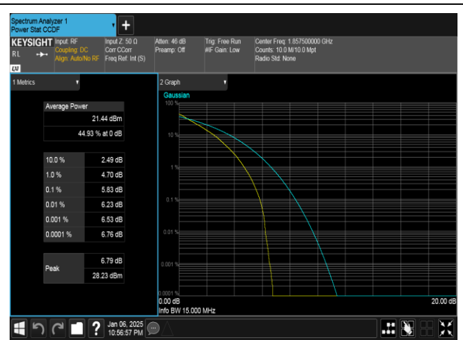
Band2-15MHz-QPSK-18675-75RB#0-PASS
