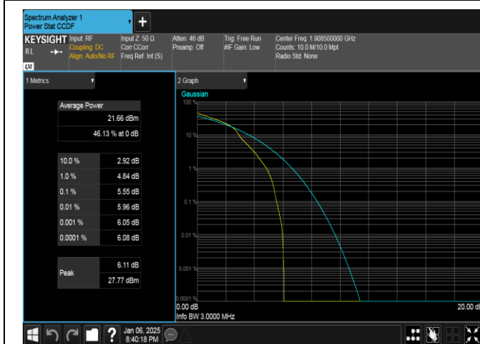
Band2-3MHz-16QAM-19185-1RB#0-PASS
