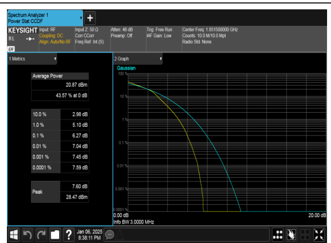
Band2-3MHz-16QAM-18615-15RB#0-PASS
