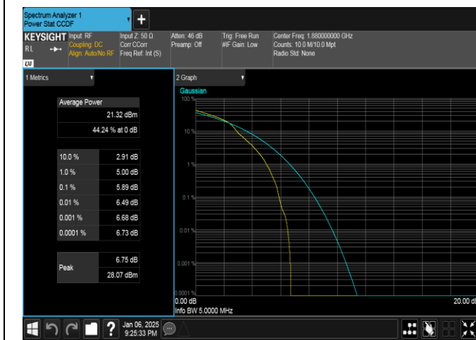
Band2-5MHz-16QAM-18900-1RB#0-PASS
