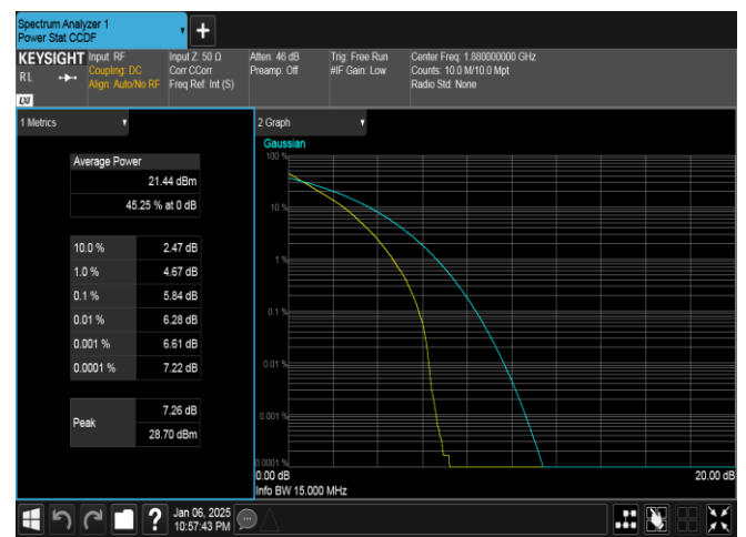
Band2-15MHz-QPSK-18900-75RB#0-PASS
