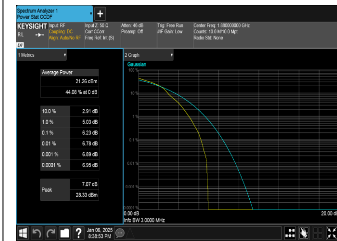
Band2-3MHz-16QAM-18900-1RB#0-PASS
