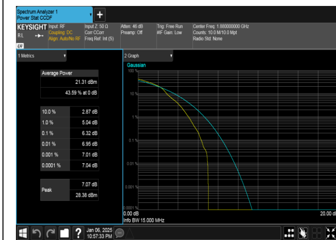
Band2-15MHz-16QAM-18900-1RB#0-PASS
