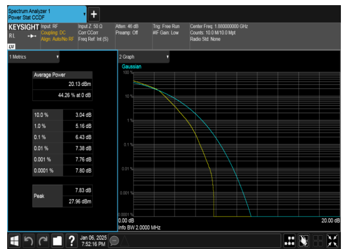
Band2-1.4MHz-16QAM-18900-6RB#0-PASS
