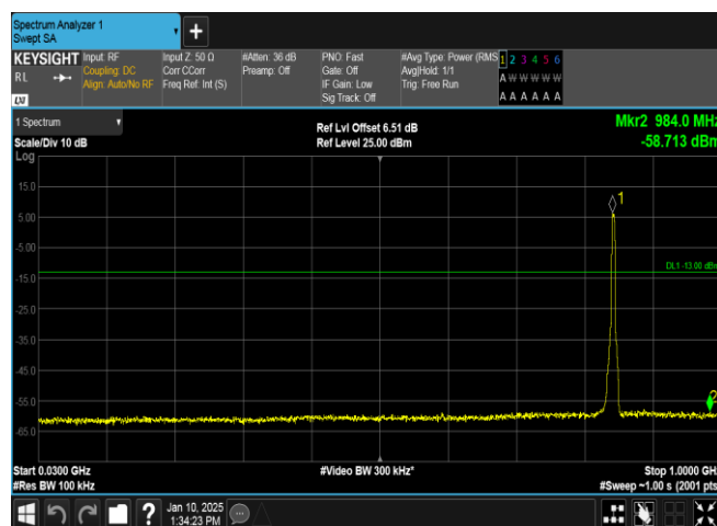
Band5-4233-3-30~1000MHz-PASS
