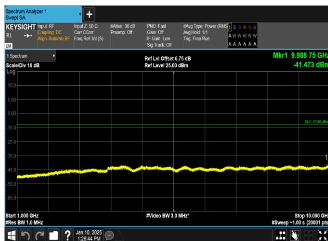
Band5-4182-1-1000~10000MHz-PASS
