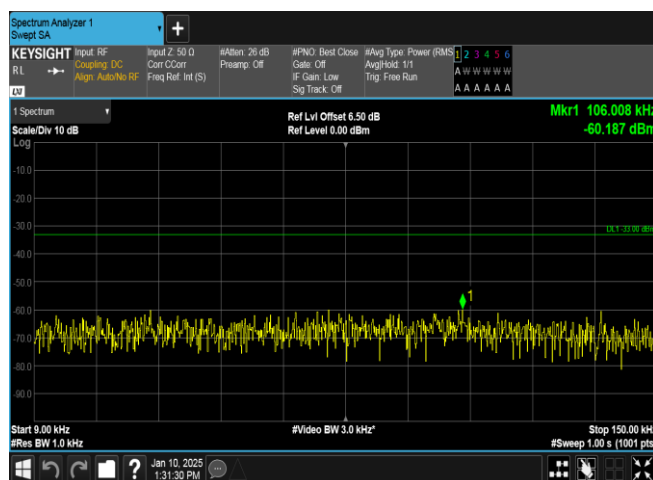
Band5-4233-2-0.009~0.15MHz-PASS
