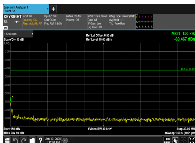
Band5-4132-5-0.15~30MHz-PASS
