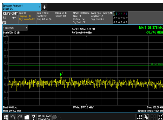
Band2-9538-5-0.009~0.15MHz-PASS
