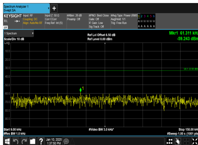
Band5-4132-5-0.009~0.15MHz-PASS
