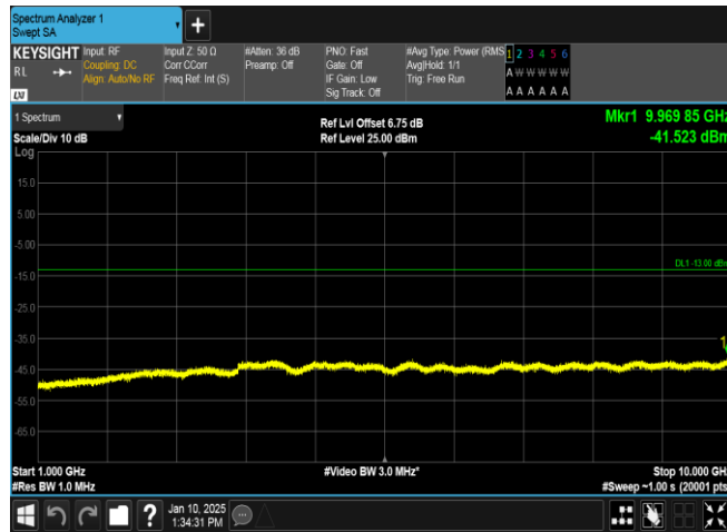
Band5-4233-3-1000~10000MHz-PASS
