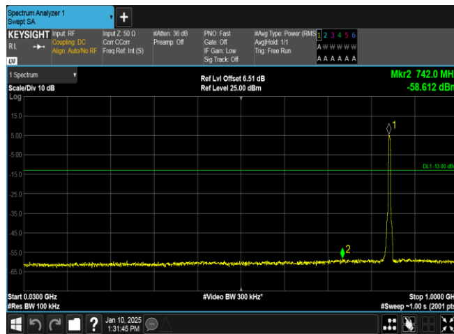
Band5-4233-2-30~1000MHz-PASS
