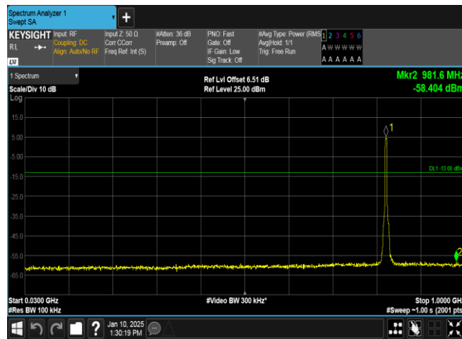
Band5-4132-2-30~1000MHz-PASS
