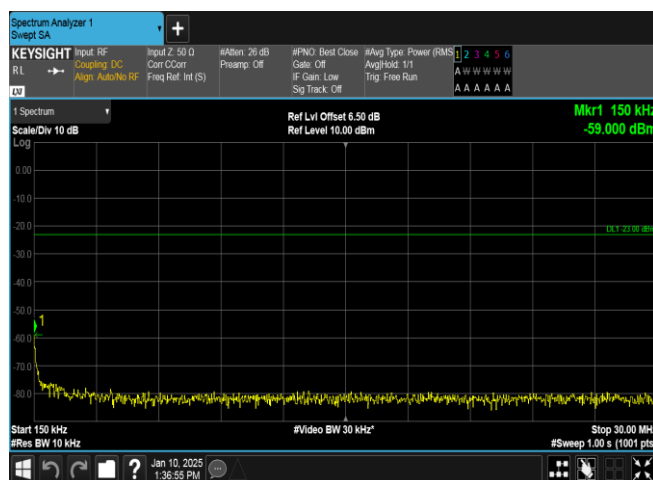
Band5-4233-4-0.15~30MHz-PASS
