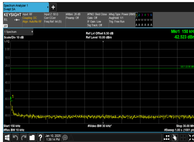
Band5-4233-5-0.15~30MHz-PASS
