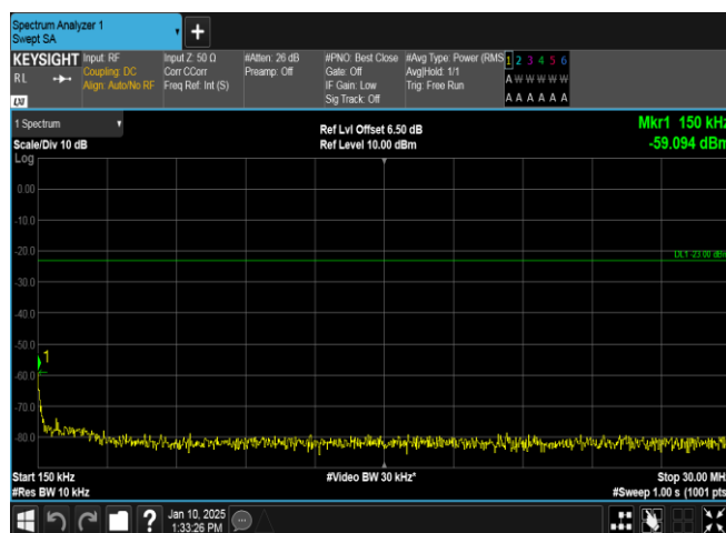
Band5-4182-3-0.15~30MHz-PASS
