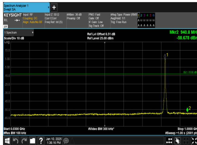
Band5-4182-4-30~1000MHz-PASS
