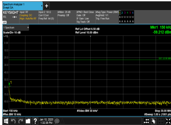
Band5-4132-3-0.15~30MHz-PASS
