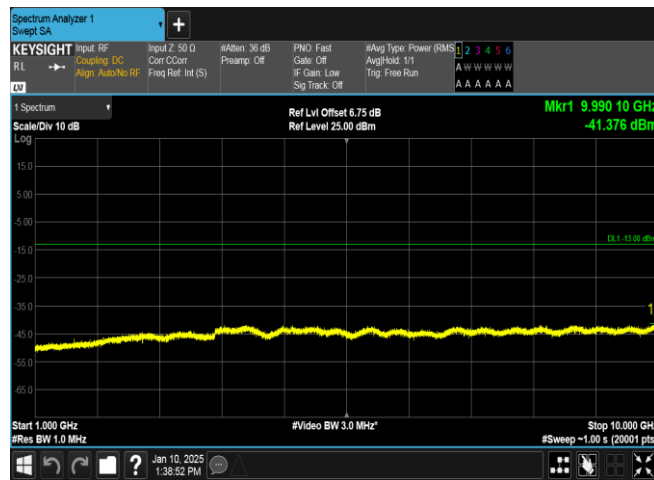
Band5-4182-5-1000~10000MHz-PASS
