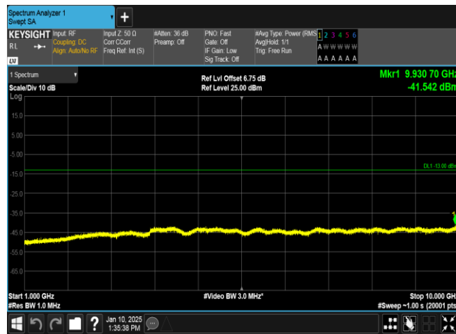
Band5-4132-4-1000~10000MHz-PASS
