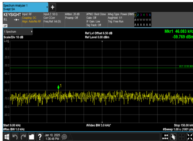
Band5-4233-4-0.009~0.15MHz-PASS
