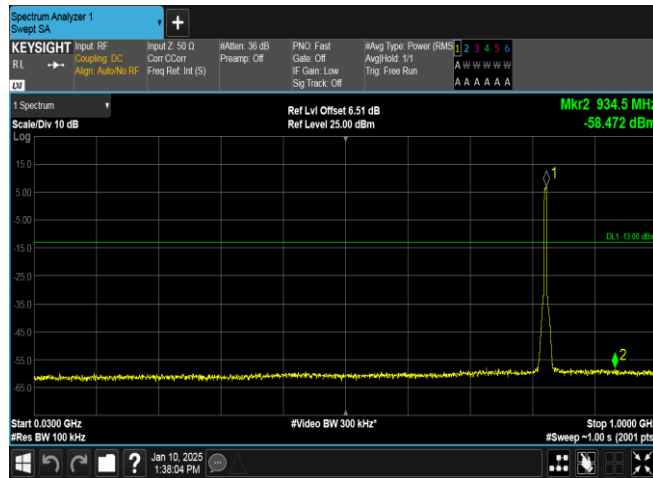
Band5-4132-5-30~1000MHz-PASS
