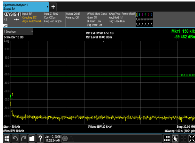
Band2-9538-5-0.15~30MHz-PASS
