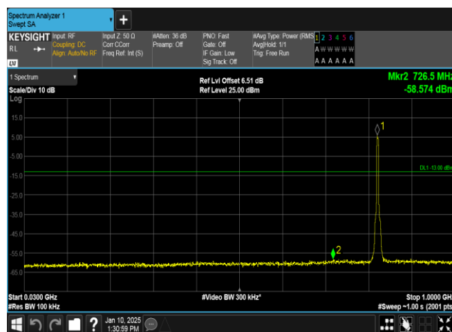
Band5-4182-2-30~1000MHz-PASS
