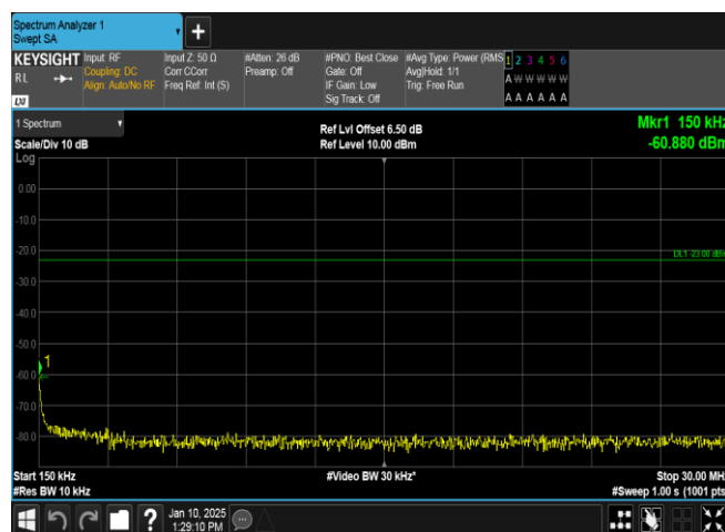
Band5-4233-1-0.15~30MHz-PASS
