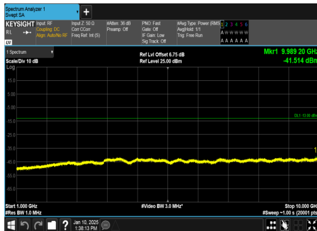
Band5-4132-5-1000~10000MHz-PASS
