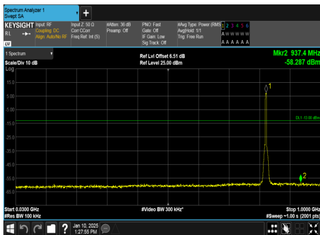
Band5-4132-1-30~1000MHz-PASS
