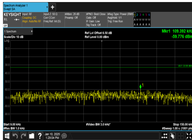
Band5-4233-1-0.009~0.15MHz-PASS
