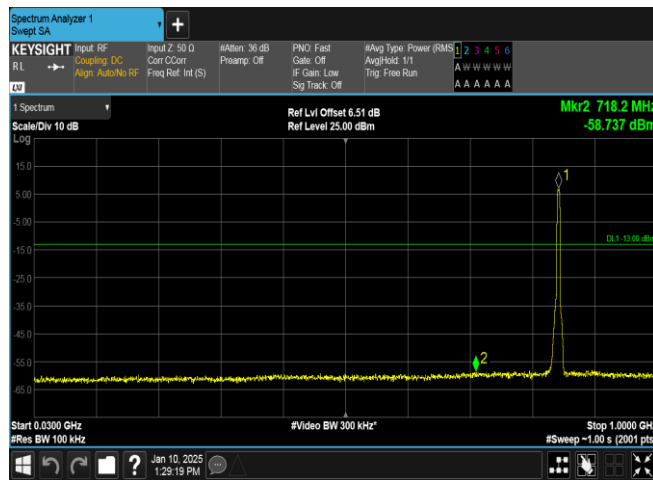
Band5-4233-1-30~1000MHz-PASS
