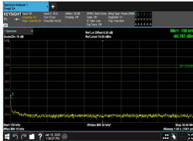
Band5-4182-4-0.15~30MHz-PASS
