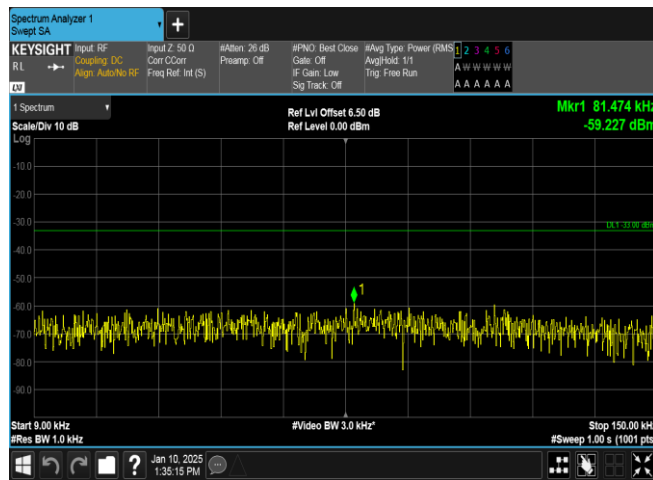
Band5-4132-4-0.009~0.15MHz-PASS
