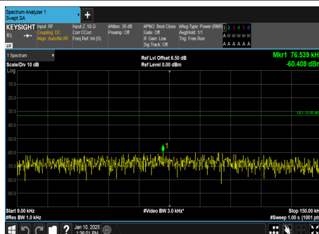
Band5-4182-4-0.009~0.15MHz-PASS
