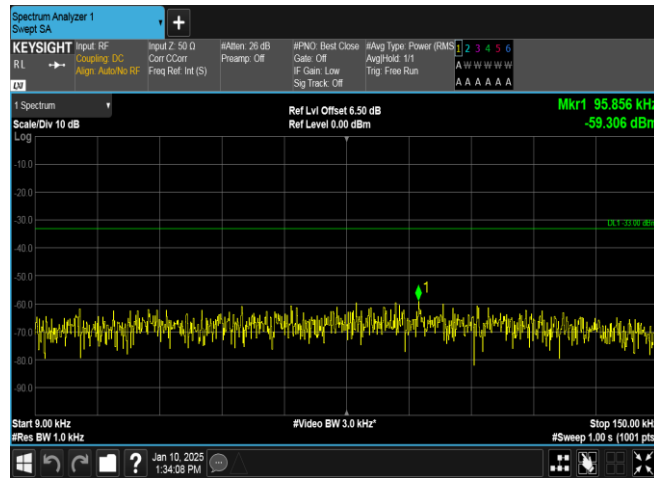
Band5-4233-3-0.009~0.15MHz-PASS
