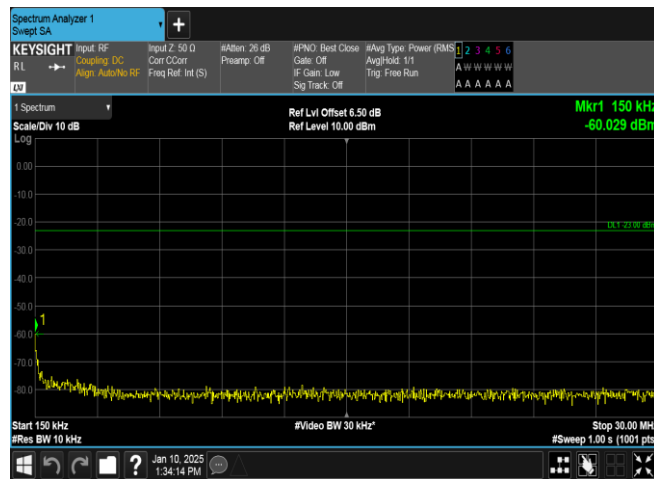
Band5-4233-3-0.15~30MHz-PASS
