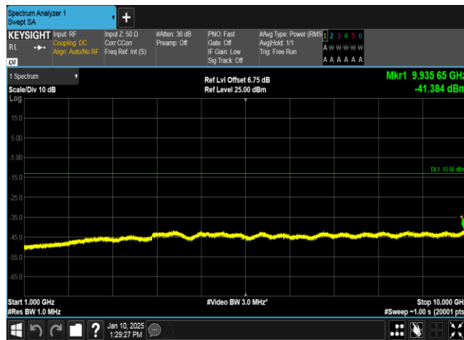
Band5-4233-1-1000~10000MHz-PASS
