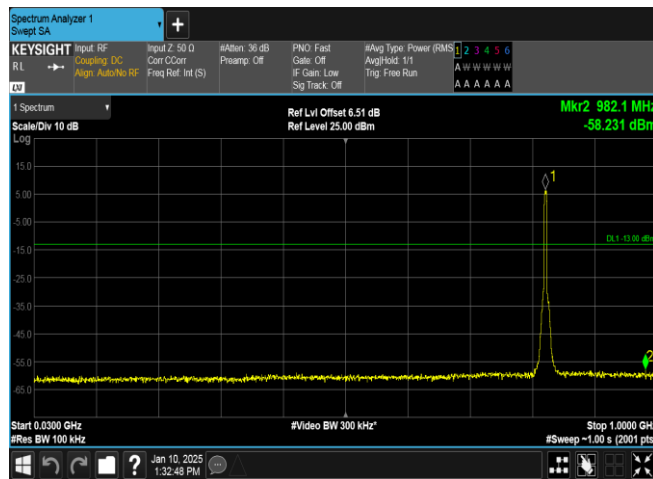
Band5-4132-3-30~1000MHz-PASS
