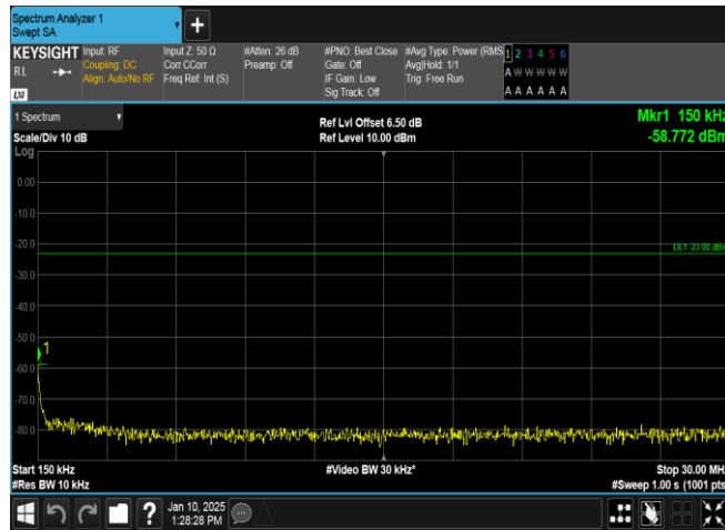
Band5-4182-1-0.15~30MHz-PASS
