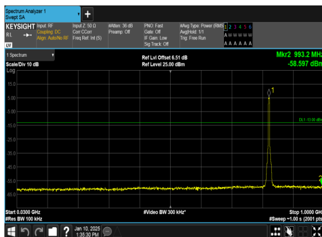
Band5-4132-4-30~1000MHz-PASS
