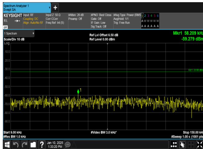
Band5-4182-3-0.009~0.15MHz-PASS
