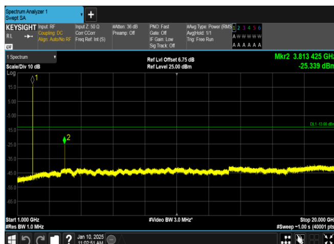
Band2-9538-5-1000~20000MHz-PASS
