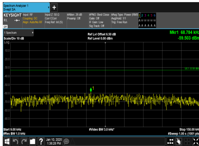
Band5-4182-5-0.009~0.15MHz-PASS
