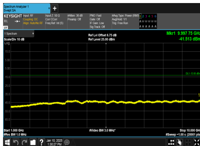
Band5-4132-2-1000~10000MHz-PASS
