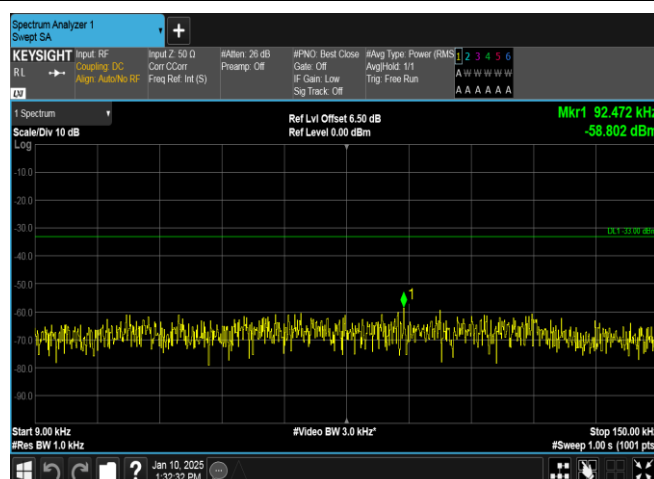
Band5-4132-3-0.009~0.15MHz-PASS
