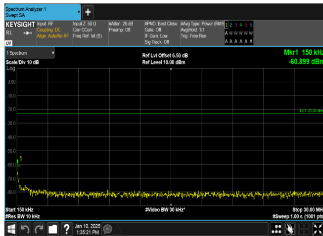
Band5-4132-4-0.15~30MHz-PASS
