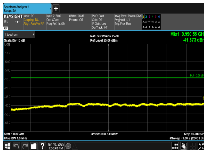
Band5-4182-3-1000~10000MHz-PASS
