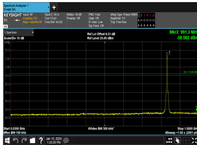
Band5-4182-3-30~1000MHz-PASS
