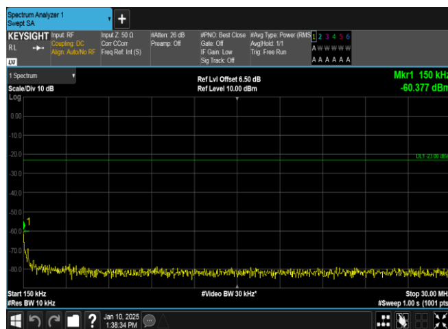
Band5-4182-5-0.15~30MHz-PASS
