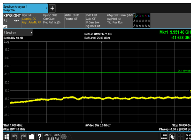
Band5-4233-2-1000~10000MHz-PASS
