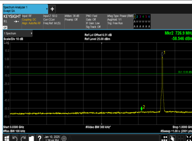
Band5-4182-5-30~1000MHz-PASS
