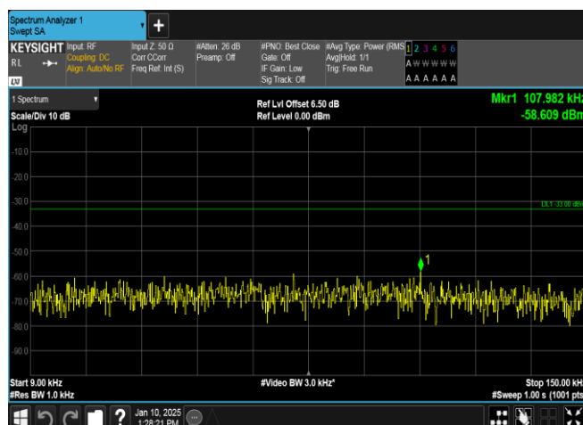
Band5-4182-1-0.009~0.15MHz-PASS
