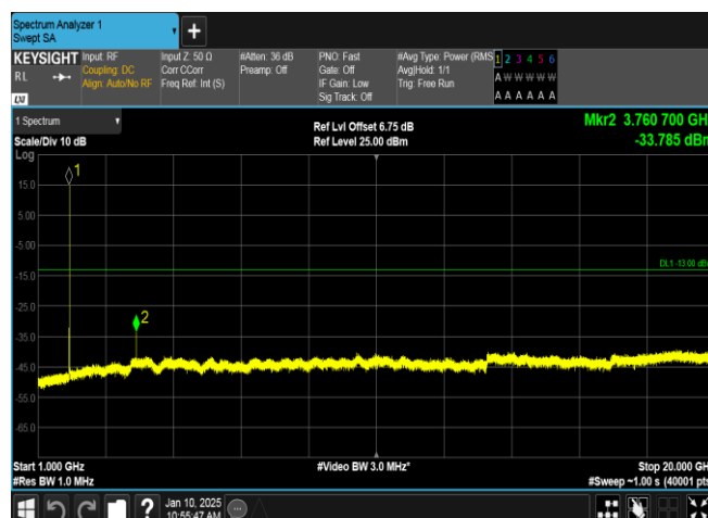
Band2-9538-2-1000~20000MHz-PASS
