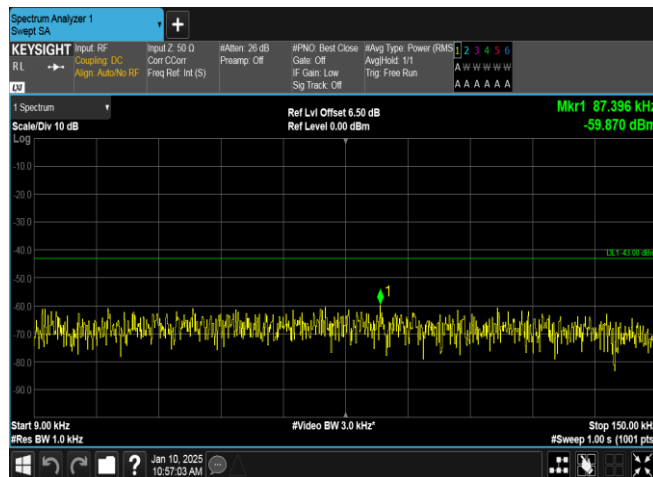
Band2-9400-3-0.009~0.15MHz-PASS
