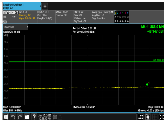
Band2-9262-3-30~1000MHz-PASS
