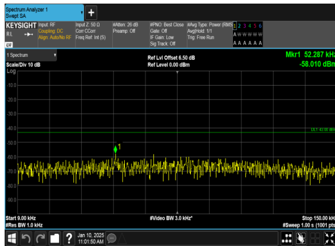
Band2-9400-5-0.009~0.15MHz-PASS
