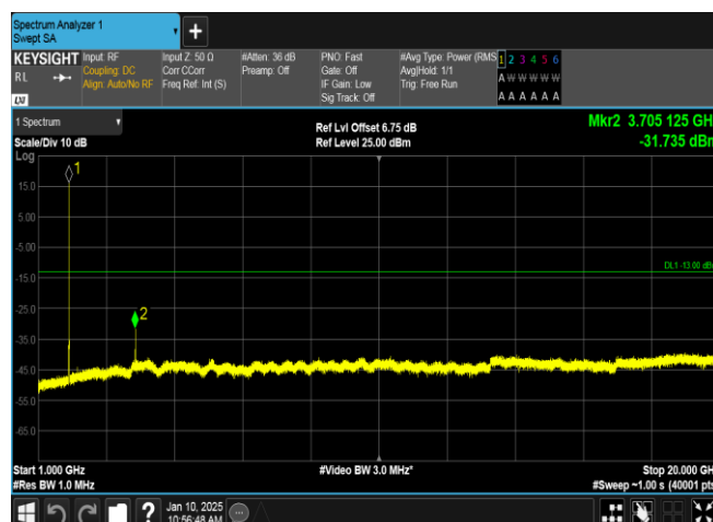
Band2-9262-3-1000~20000MHz-PASS
