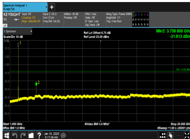
Band2-9400-4-1000~20000MHz-PASS
