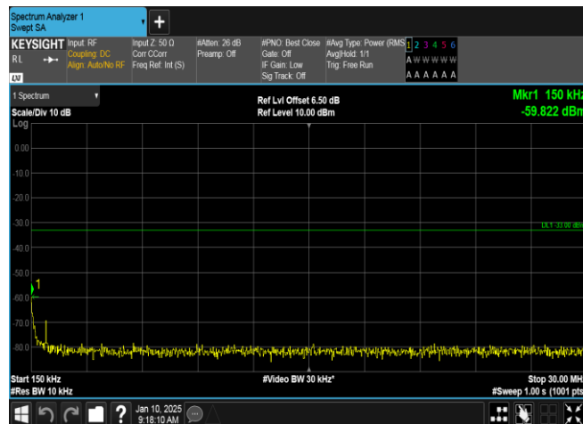
Band2-9538-4-0.15~30MHz-PASS
