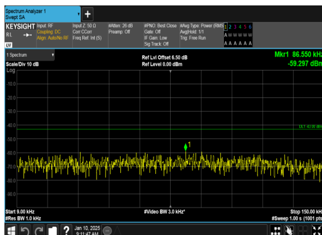
Band2-9538-1-0.009~0.15MHz-PASS
