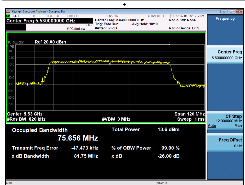
Test_Graph_802.11ac80_ANT1_5530_MCS0_OBW
