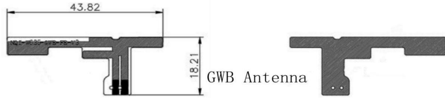
WIFI/BT FPC Antenna
