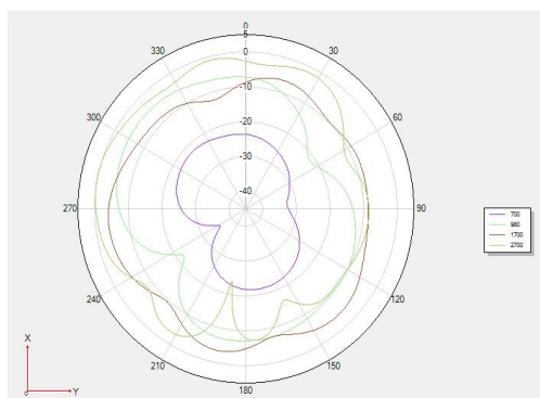
Theta 90°
