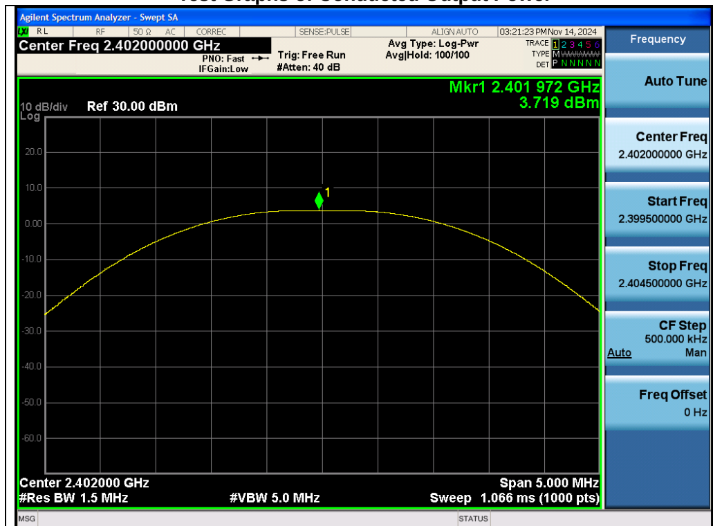
Test_Graph_LE1M_ANT1_2402_1Mbps_Peak Power
