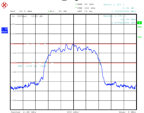
2DH1_High 1.320MHz
