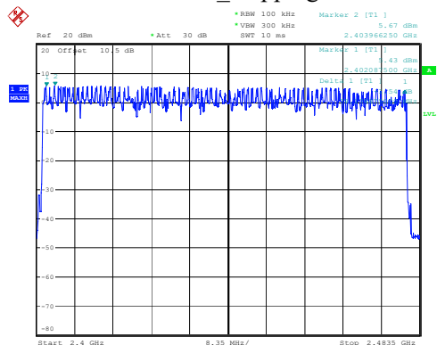
2DH1_Hopping 79
