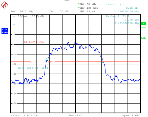
2DH1_Low 1.316MHz
