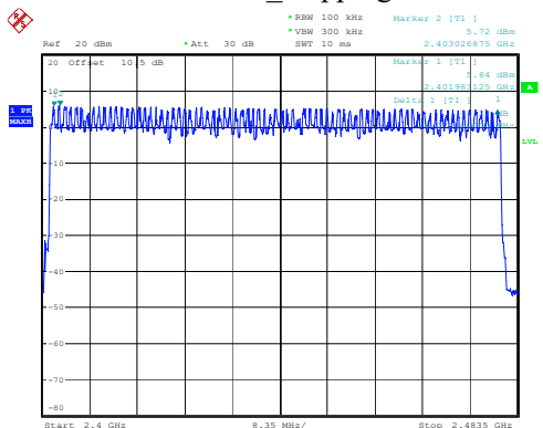
3DH1_Hopping 79
