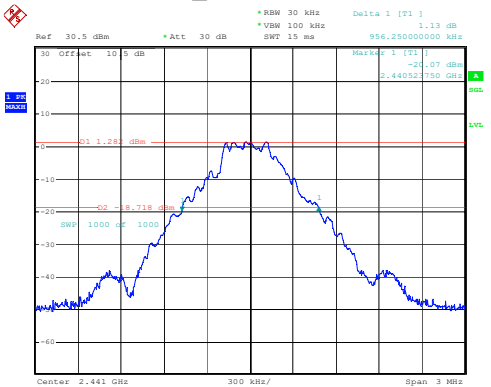
DH1_Middle 0.956MHz
