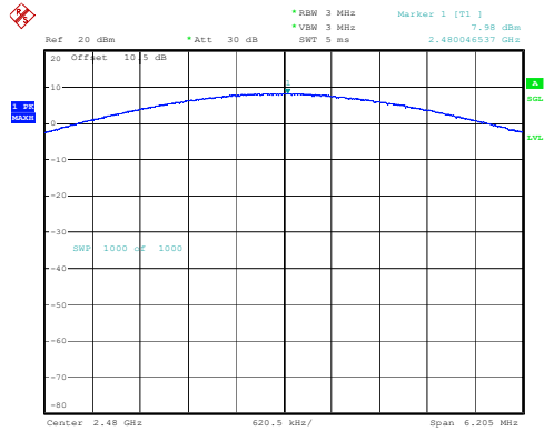
3DH1_High 7.98dBm
