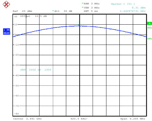
3DH1_Middle 8.31dBm
