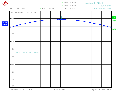
2DH1_Low 8.54dBm
