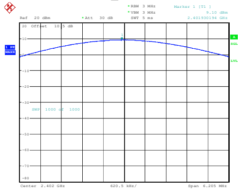
3DH1_Low 9.10dBm
