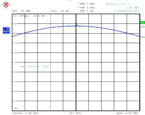
2DH1_High 7.45dBm
