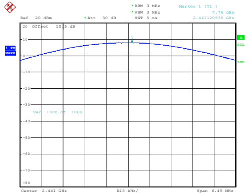
2DH1_Middle 7.76dBm
