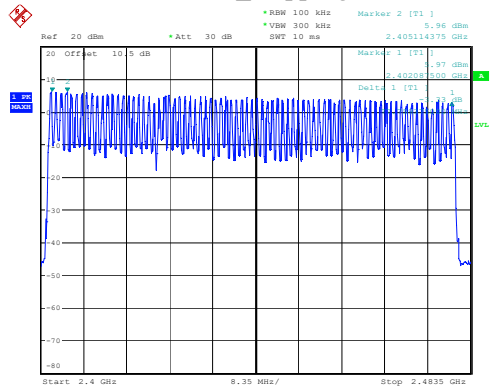
DH1_Hopping 79
