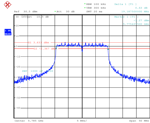
802.11ax20_5785MHz_RU_Full 19.188MHz
