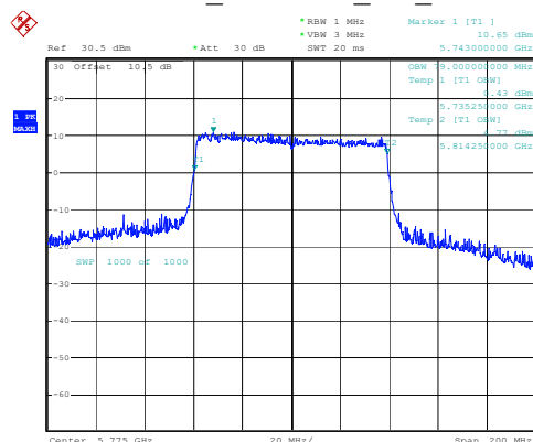
802.11ax80_5775MHz_RU_Full 79MHz
