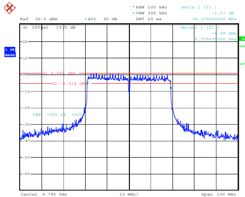
802.11ax40_5795MHz_RU_Full 38.375MHz
