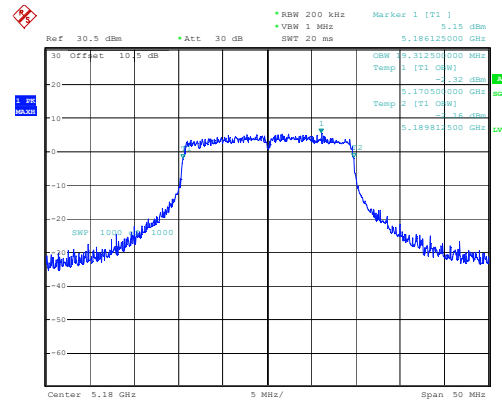
802.11ax20_5180MHz_RU_Full 19.313MHz
