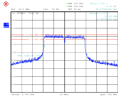
802.11ax40_5755MHz_RU_Full 38.375MHz
