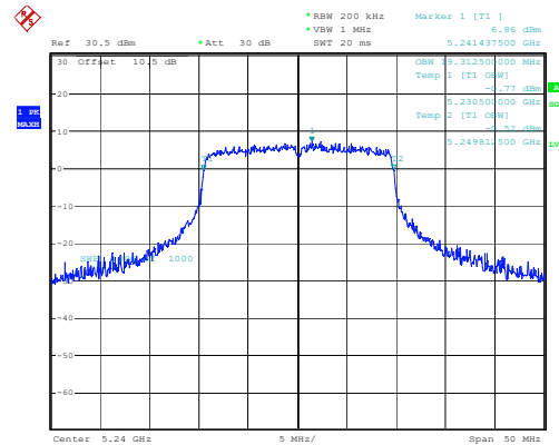
802.11ax20_5240MHz_RU_Full 19.313MHz
