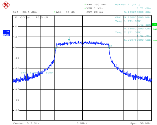
802.11ax20_5200MHz_RU_Full 19.250MHz
