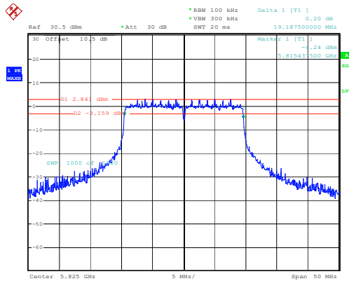
802.11ax20_5825MHz_RU_Full 19.188MHz
