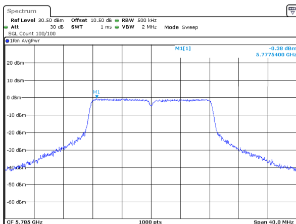
802.11a_5785MHz
