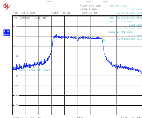
802.11ax40_5755MHz_RU_Full 38.625MHz
