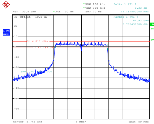
802.11ax20_5745MHz_RU_Full 19.188MHz
