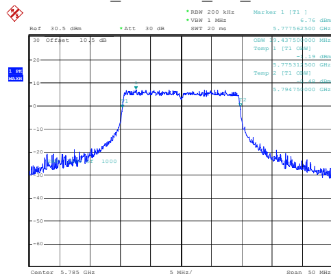
802.11ax20_5785MHz_RU_Full 19.438MHz
