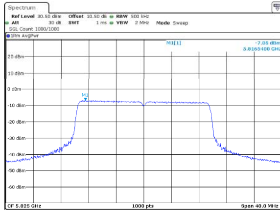
802.11ax20_5825MHz_RU_Full
