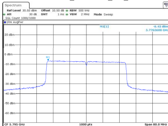
802.11ax40_5795MHz_RU_Full
