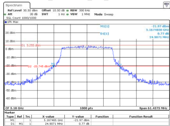
802.11ax20_5180MHz_RU_Full 24.907MHz
