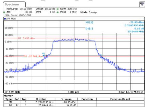
802.11ax20_5240MHz_RU_Full 25.845MHz
