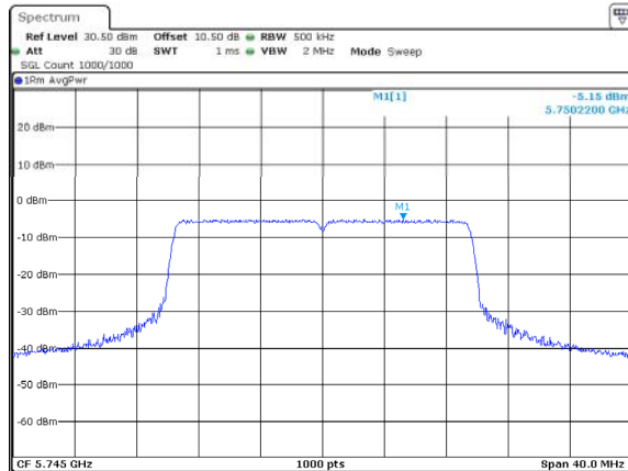
802.11ax20_5745MHz_RU_Full
