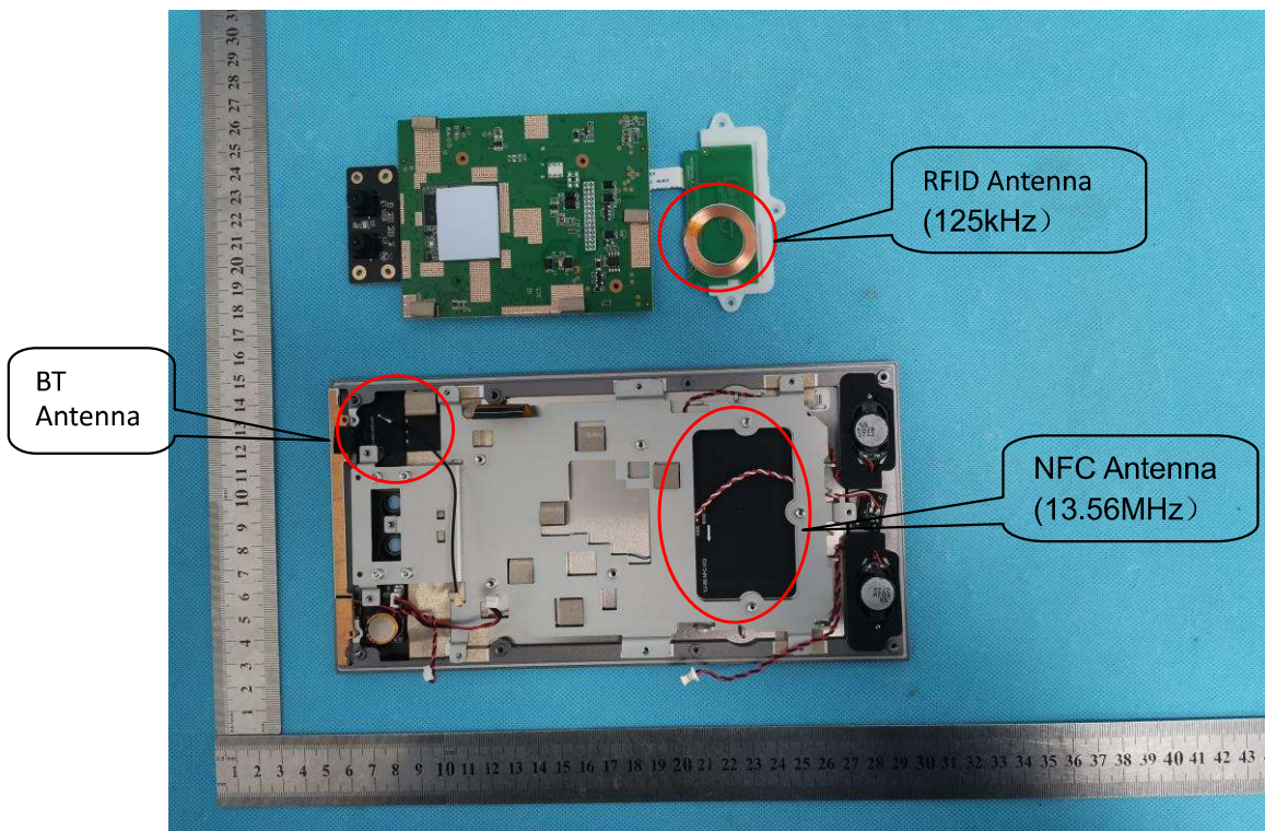
OPEN VIEW OF EUT (FIGURE 3)
