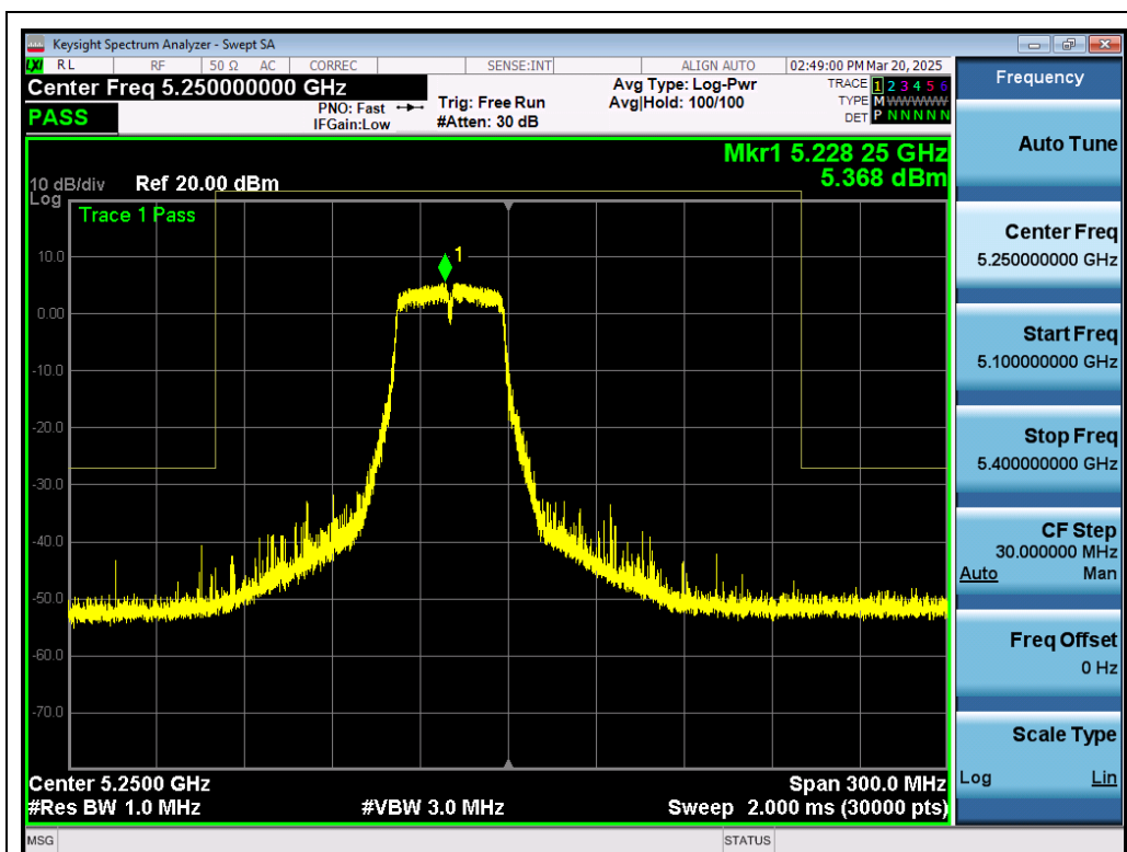
Test_Graph_802.11n40_ANT1_5230_MCS0_Frequency Band 3
