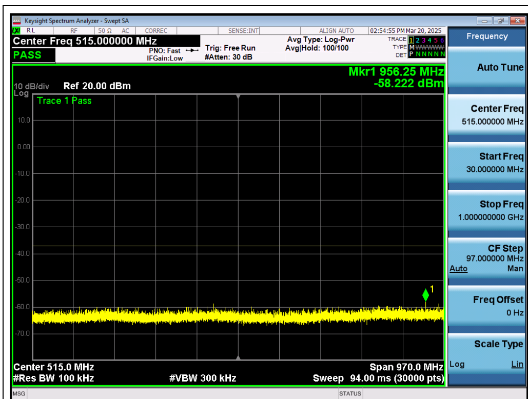
Test_Graph_802.11ac80_ANT1_5210_MCS0_Frequency Band 1
