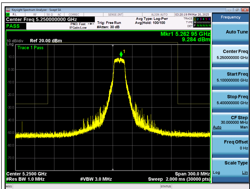
Test_Graph_802.11a_ANT1_5260_6Mbps_Frequency Band 3
