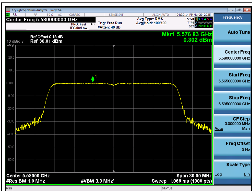
Test_Graph_802.11ax20_ANT1_5580_MCS0_PSD
