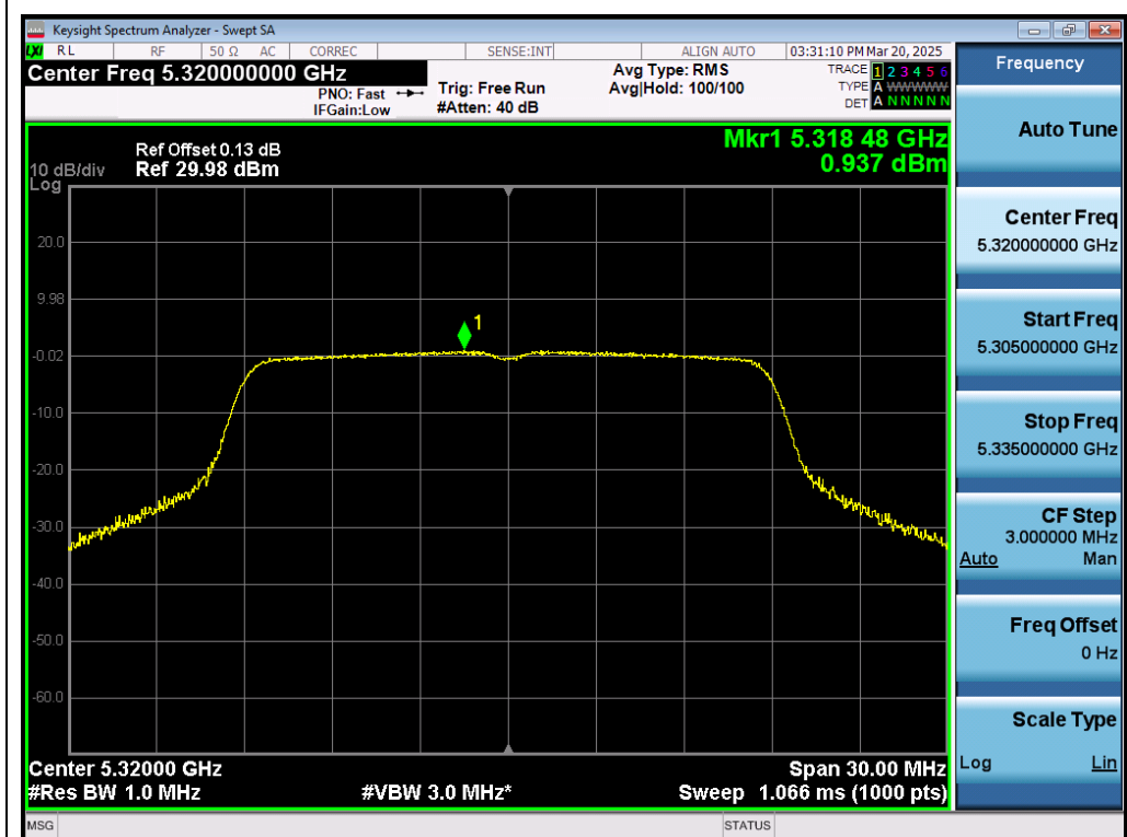
Test_Graph_802.11n20_ANT1_5320_MCS0_PSD
