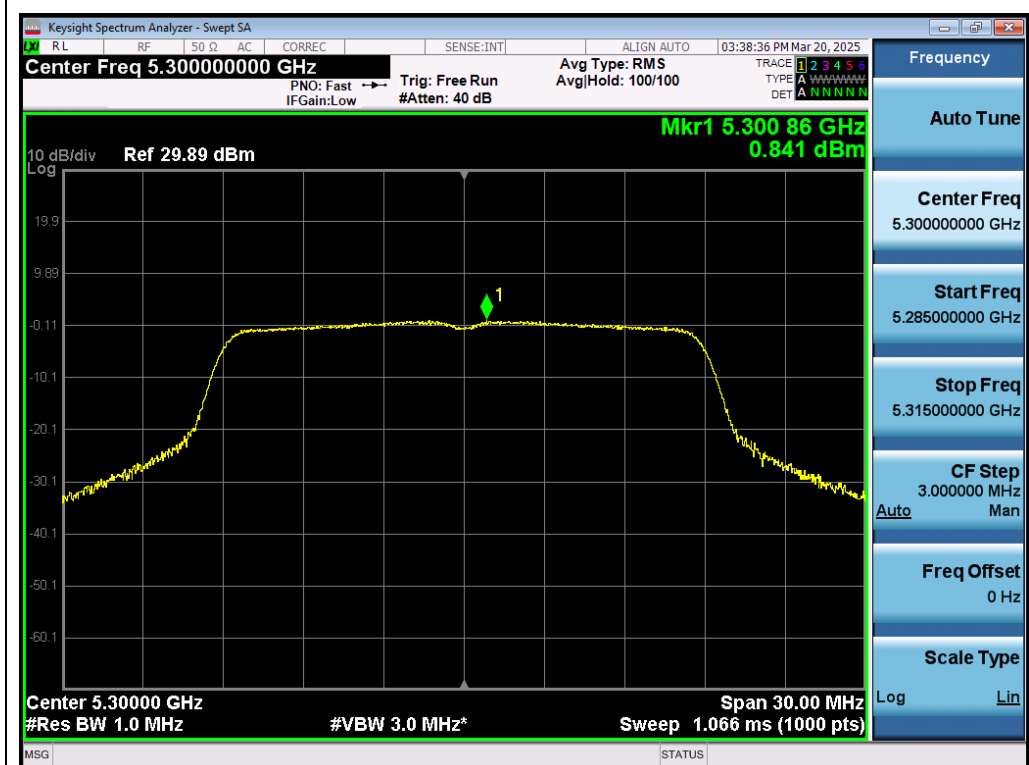
Test_Graph_802.11ac20_ANT1_5300_MCS0_PSD
