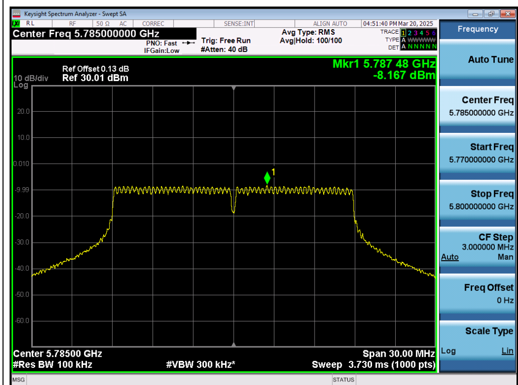
Test_Graph_802.11n20_ANT1_5785_MCS0_PSD
