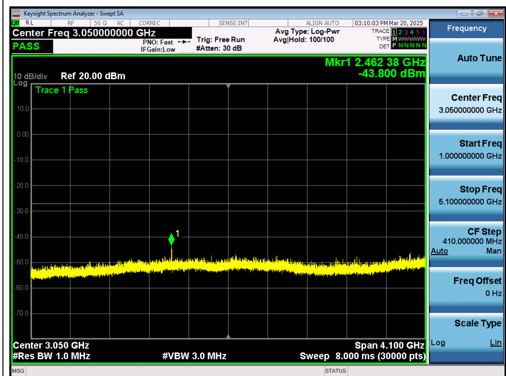
Test_Graph_802.11ax80_ANT1_5210_MCS0_Frequency Band 2
