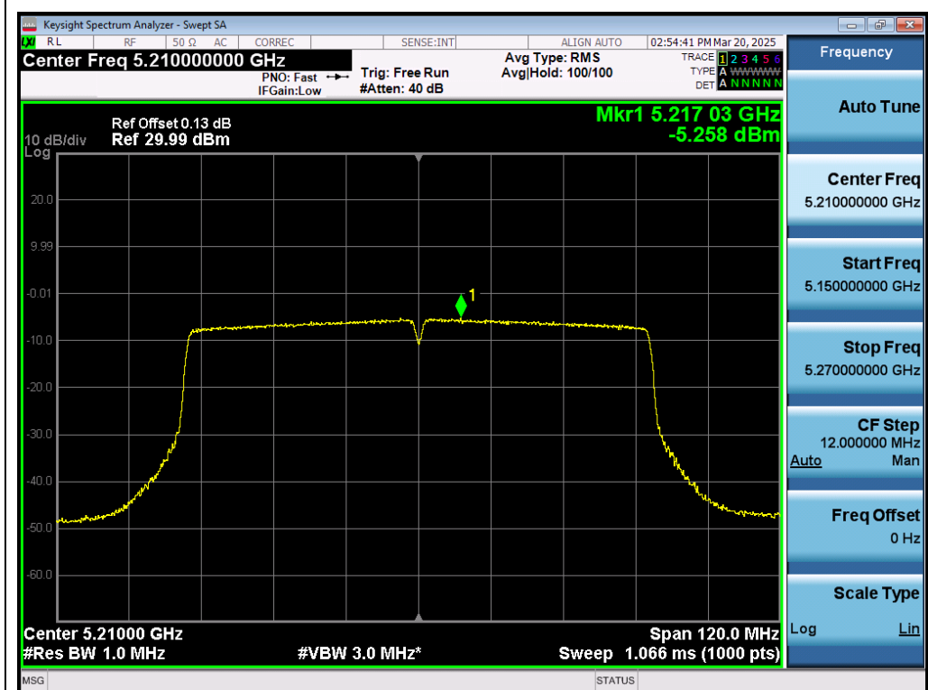
Test_Graph_802.11ac80_ANT1_5210_MCS0_PSD
