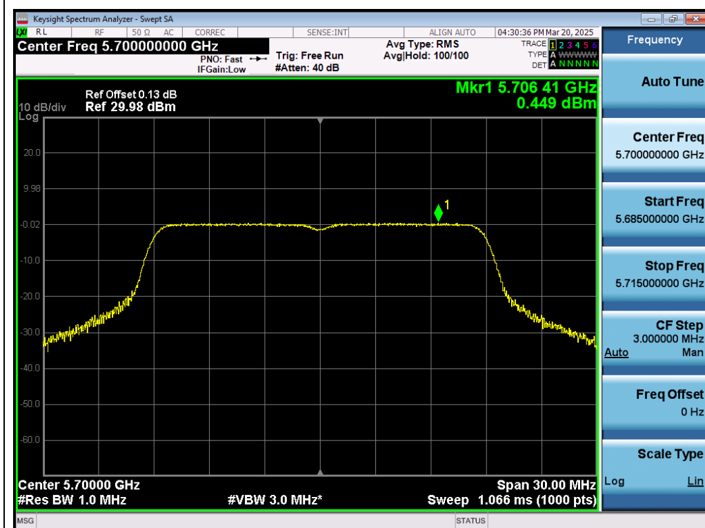
Test_Graph_802.11ac20_ANT1_5700_MCS0_PSD
