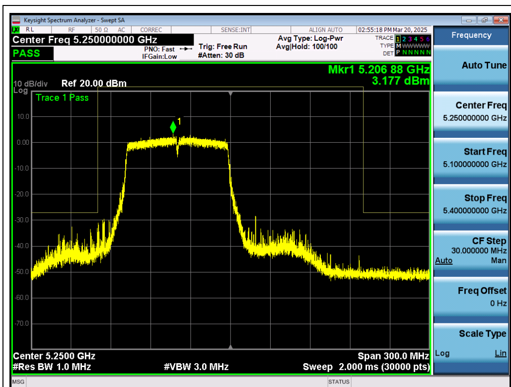
Test_Graph_802.11ac80_ANT1_5210_MCS0_Frequency Band 3
