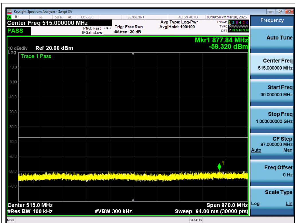
Test_Graph_802.11ax80_ANT1_5210_MCS0_Frequency Band 1
