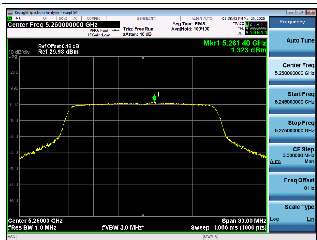
Test_Graph_802.11ac20_ANT1_5260_MCS0_PSD
