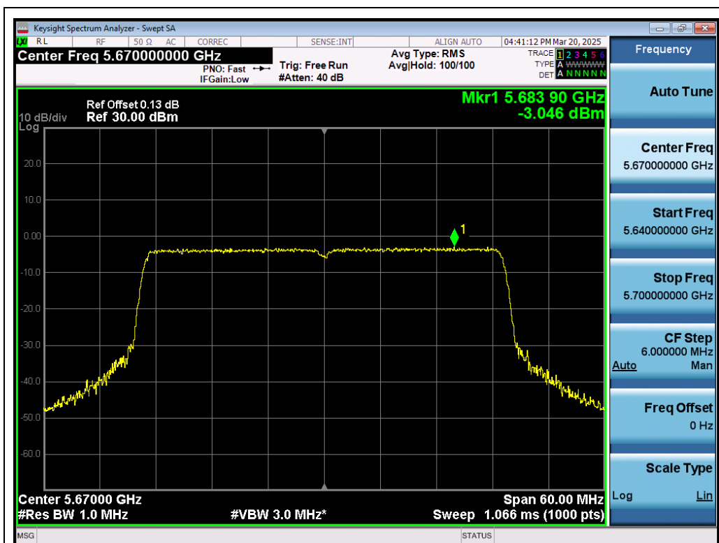
Test_Graph_802.11ax40_ANT1_5670_MCS0_PSD
