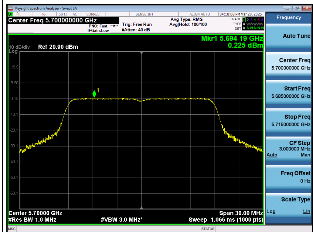
Test_Graph_802.11n20_ANT1_5700_MCS0_PSD
