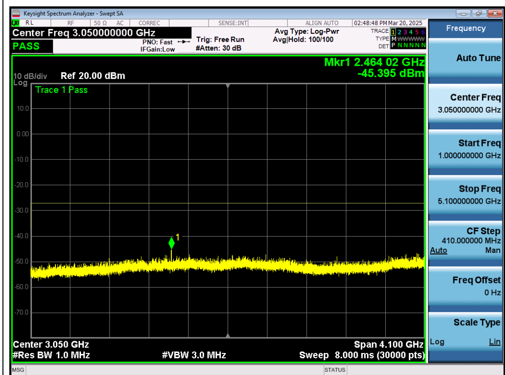
Test_Graph_802.11n40_ANT1_5230_MCS0_Frequency Band 2
