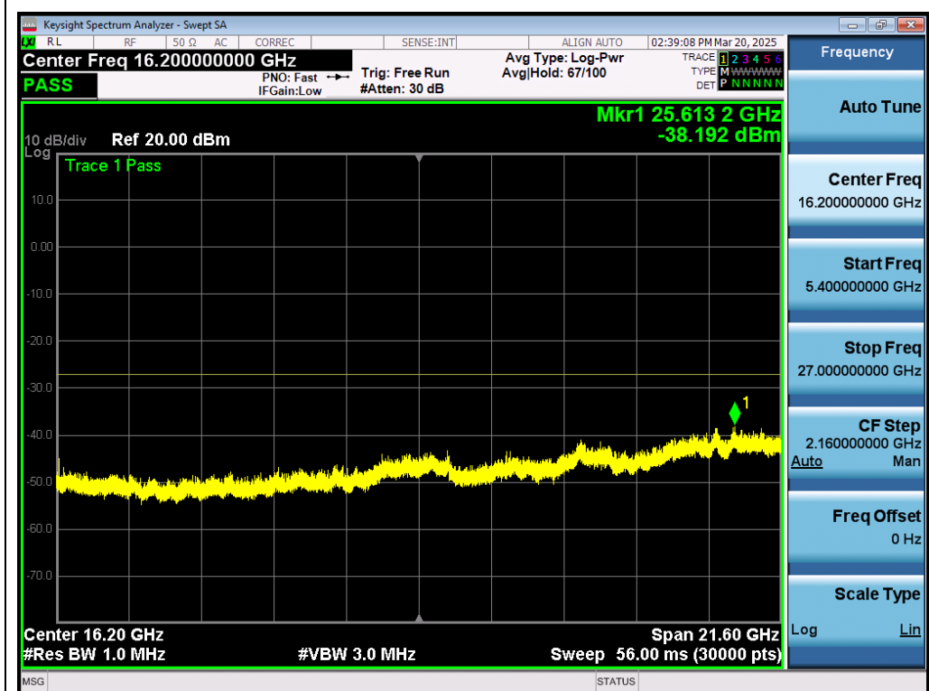
Test_Graph_802.11a_ANT1_5240_6Mbps_Frequency Band 4
