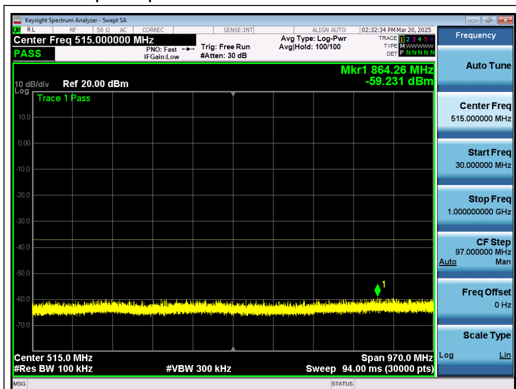
Test_Graph_802.11a_ANT1_5180_6Mbps_Frequency Band 1
