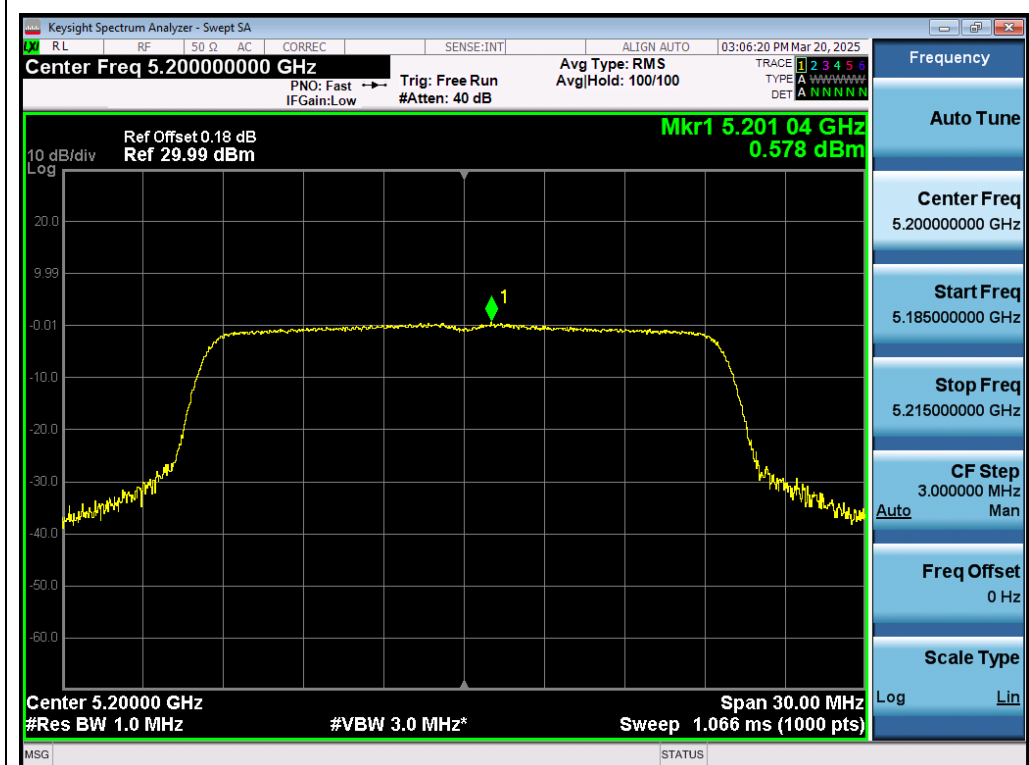
Test_Graph_802.11ax20_ANT1_5200_MCS0_PSD
