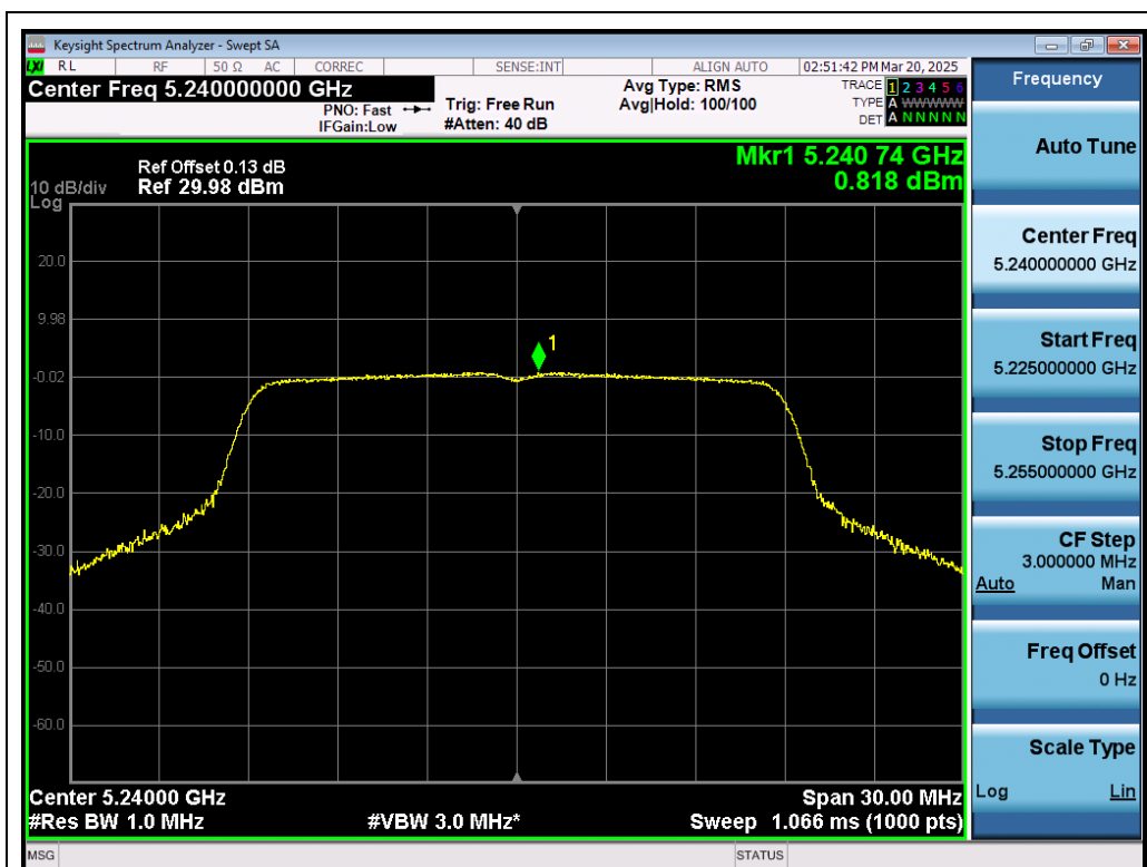
Test_Graph_802.11ac20_ANT1_5240_MCS0_PSD
