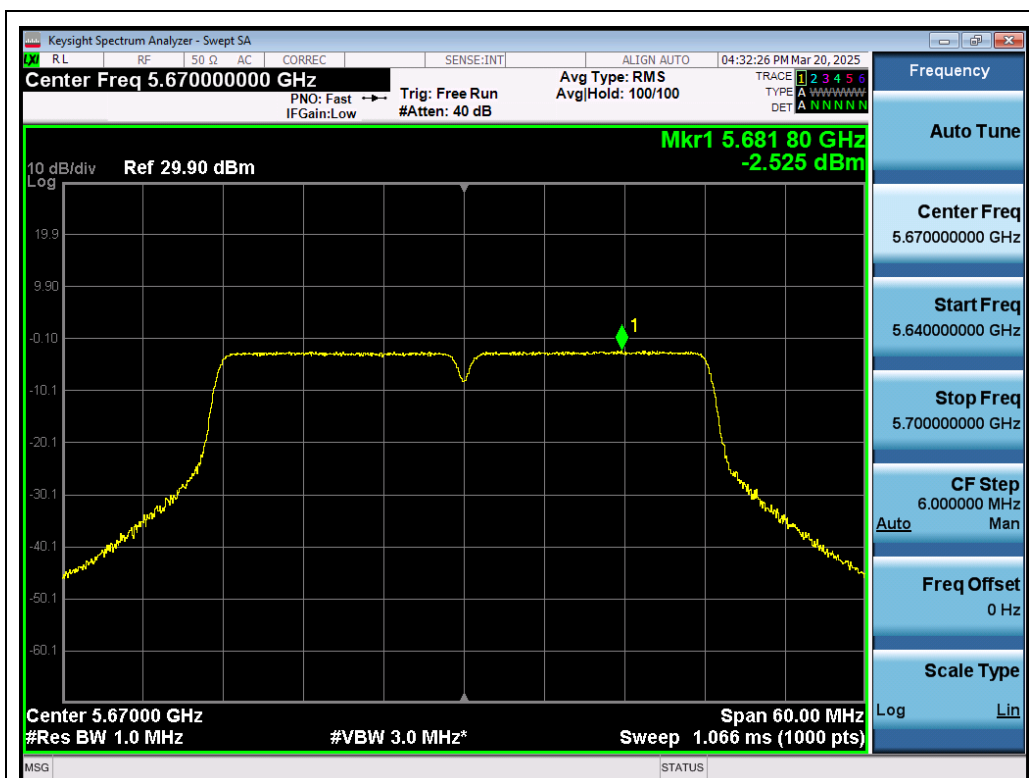
Test_Graph_802.11ac40_ANT1_5670_MCS0_PSD
