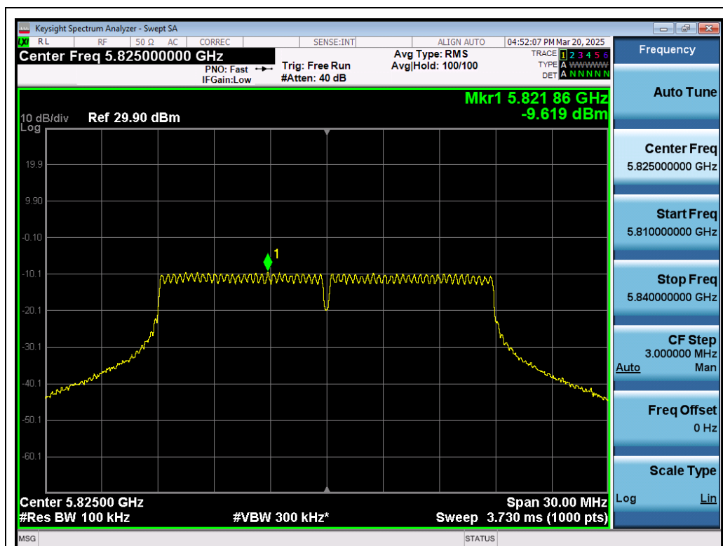
Test_Graph_802.11n20_ANT1_5825_MCS0_PSD
