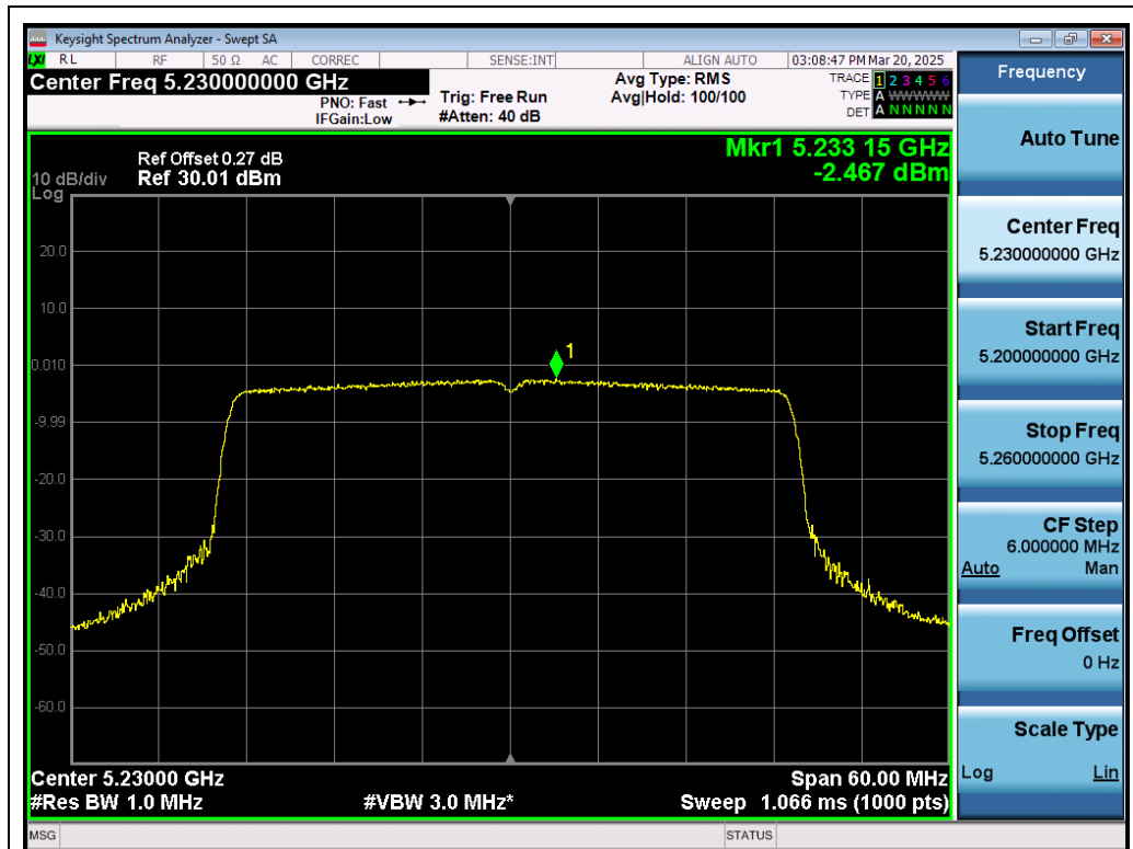
Test_Graph_802.11ax40_ANT1_5230_MCS0_PSD
