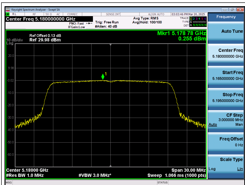
Test_Graph_802.11ax20_ANT1_5180_MCS0_PSD
