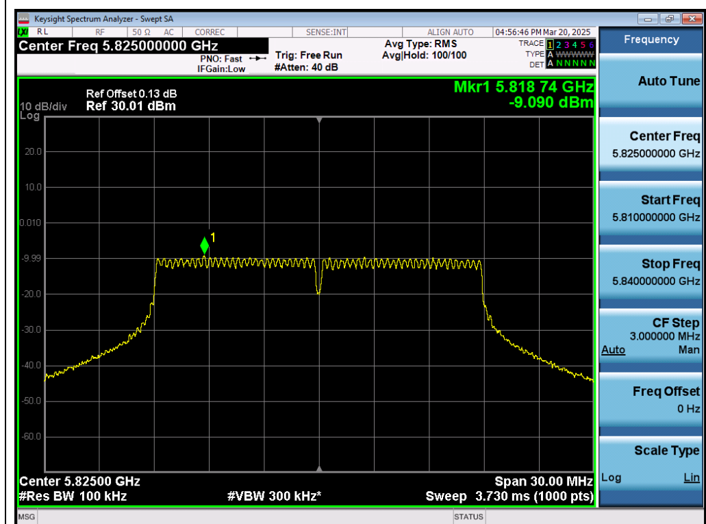
Test_Graph_802.11ac20_ANT1_5825_MCS0_PSD
