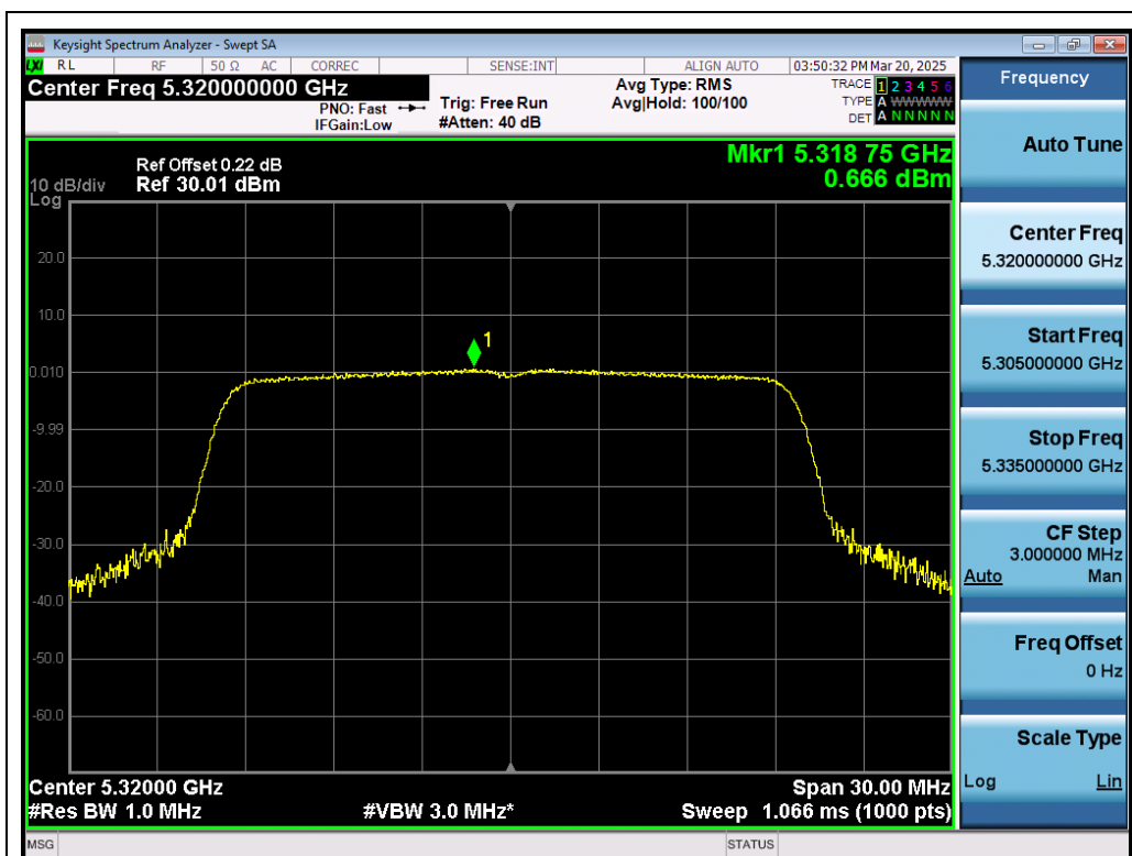
Test_Graph_802.11ax20_ANT1_5320_MCS0_PSD
