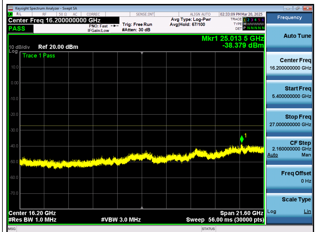
Test_Graph_802.11a_ANT1_5180_6Mbps_Frequency Band 4
