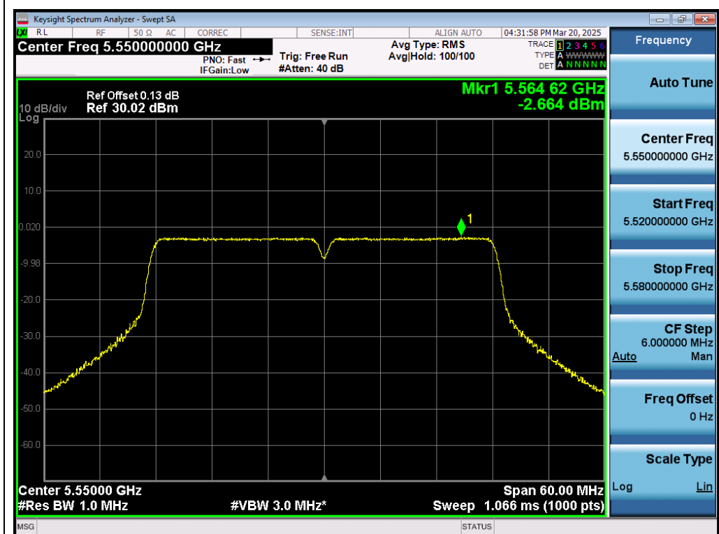
Test_Graph_802.11ac40_ANT1_5550_MCS0_PSD
