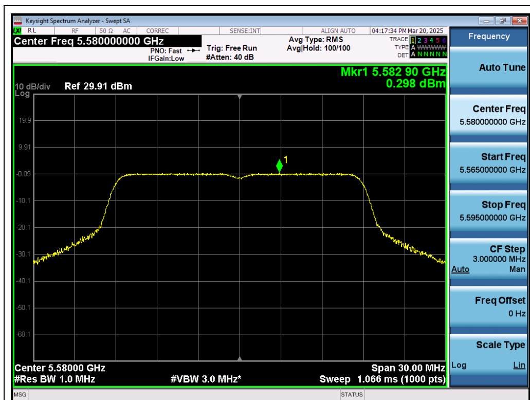
Test_Graph_802.11n20_ANT1_5580_MCS0_PSD
