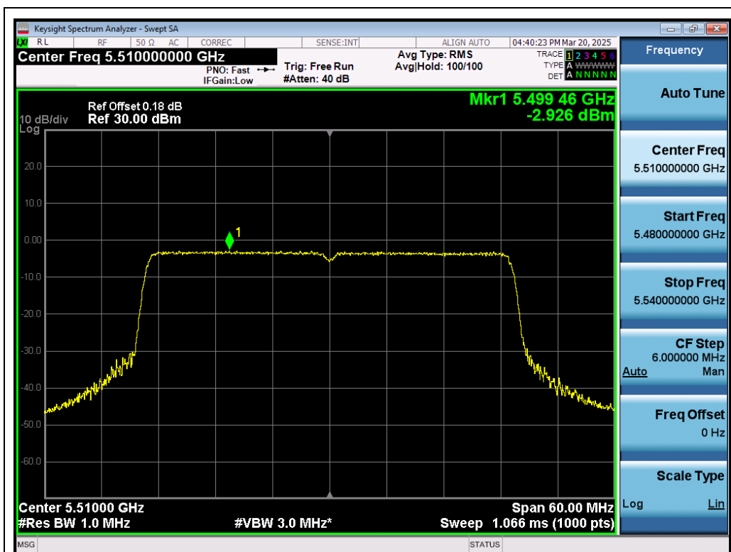
Test_Graph_802.11ax40_ANT1_5510_MCS0_PSD
