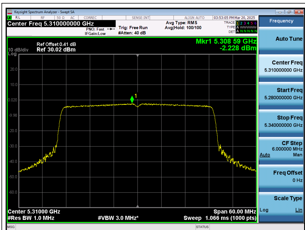
Test_Graph_802.11ax40_ANT1_5310_MCS0_PSD
