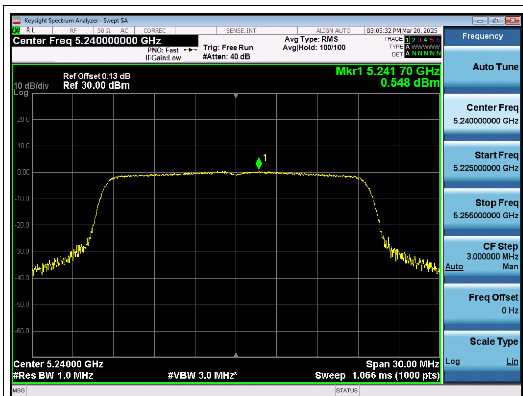
Test_Graph_802.11ax20_ANT1_5240_MCS0_PSD
