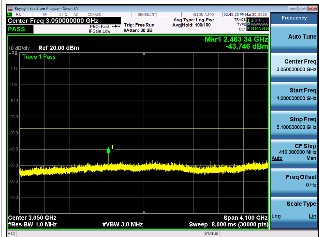
Test_Graph_802.11n40_ANT1_5190_MCS0_Frequency Band 2
