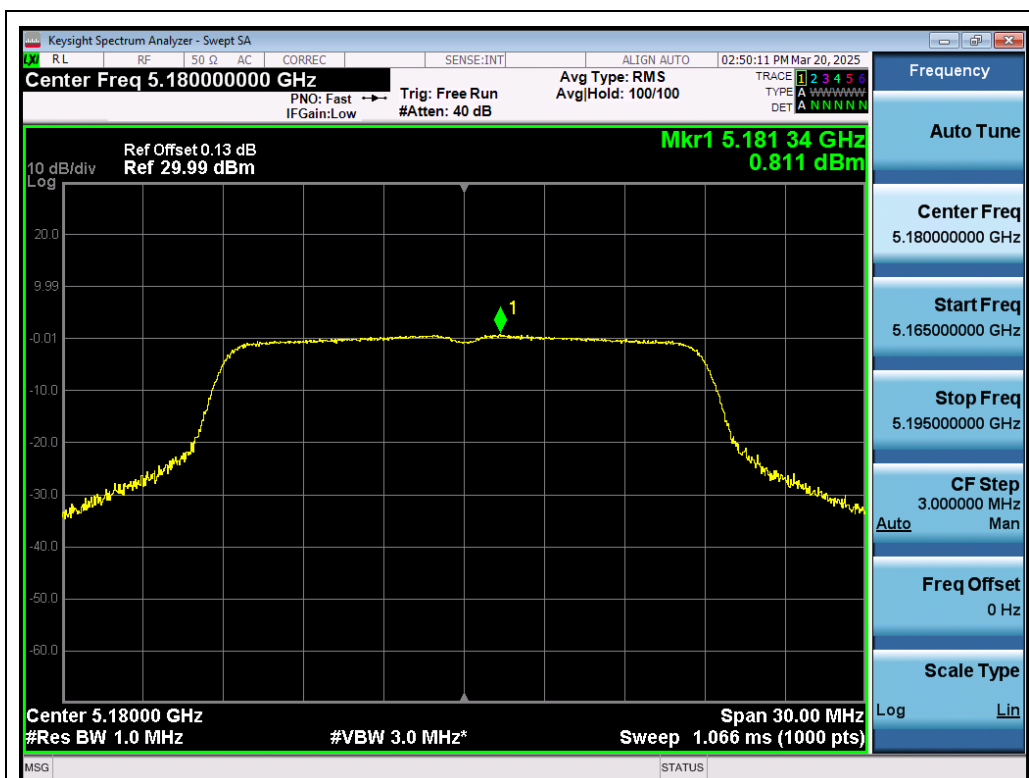
Test_Graph_802.11ac20_ANT1_5180_MCS0_PSD
