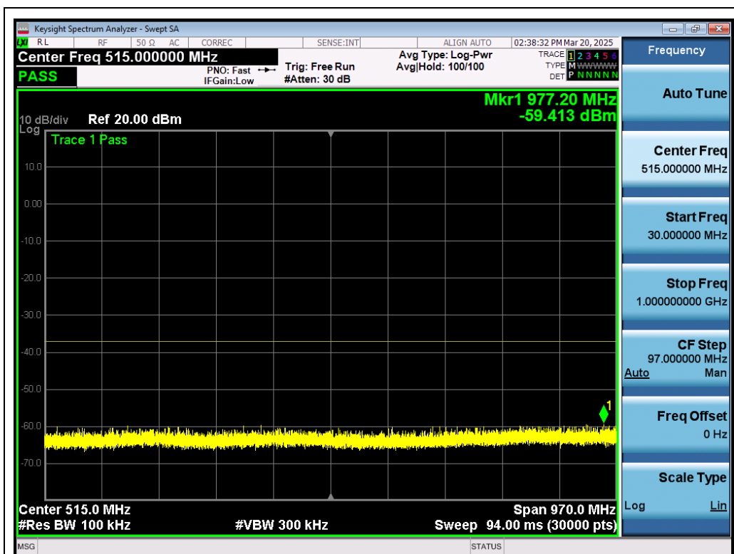
Test_Graph_802.11a_ANT1_5240_6Mbps_Frequency Band 1
