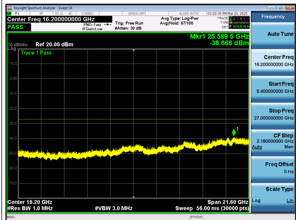
Test_Graph_802.11a_ANT1_5260_6Mbps_Frequency Band 4
