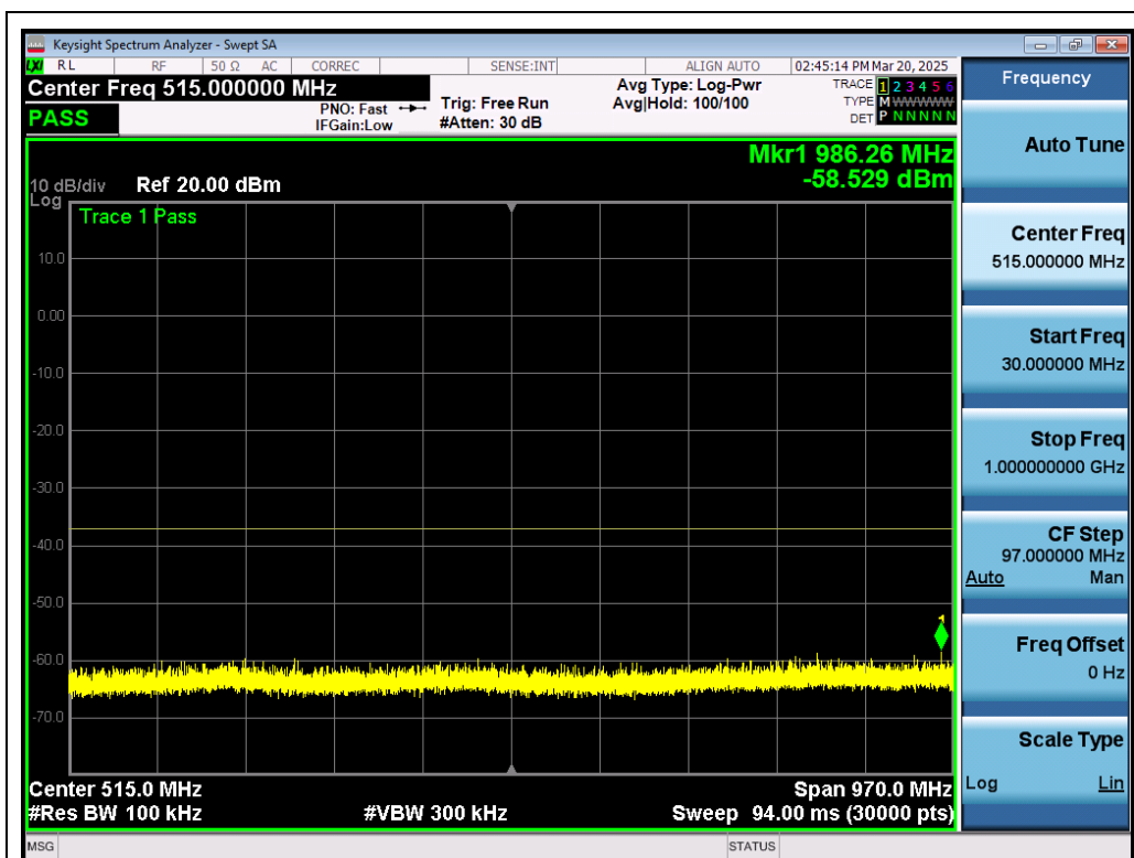
Test_Graph_802.11n40_ANT1_5190_MCS0_Frequency Band 1
