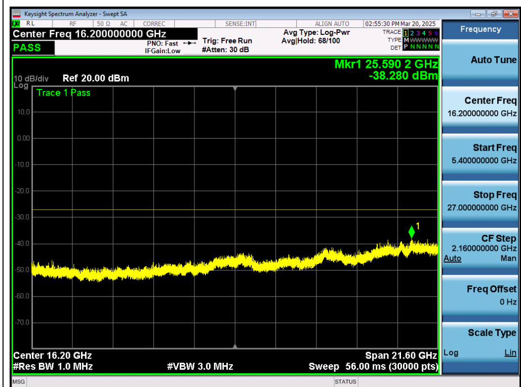
Test_Graph_802.11ac80_ANT1_5210_MCS0_Frequency Band 4
