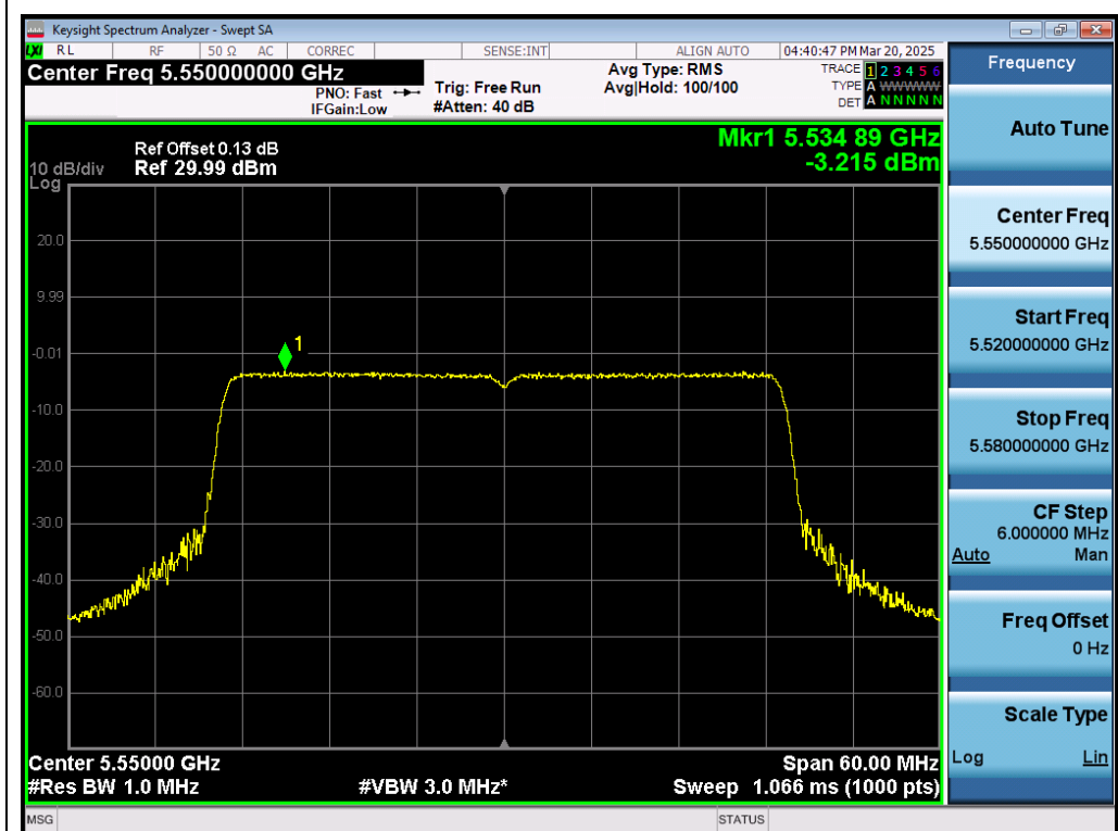
Test_Graph_802.11ax40_ANT1_5550_MCS0_PSD
