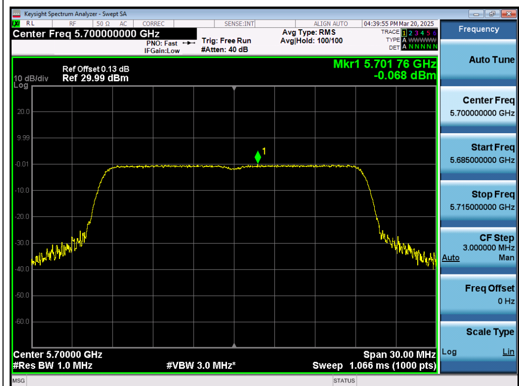
Test_Graph_802.11ax20_ANT1_5700_MCS0_PSD
