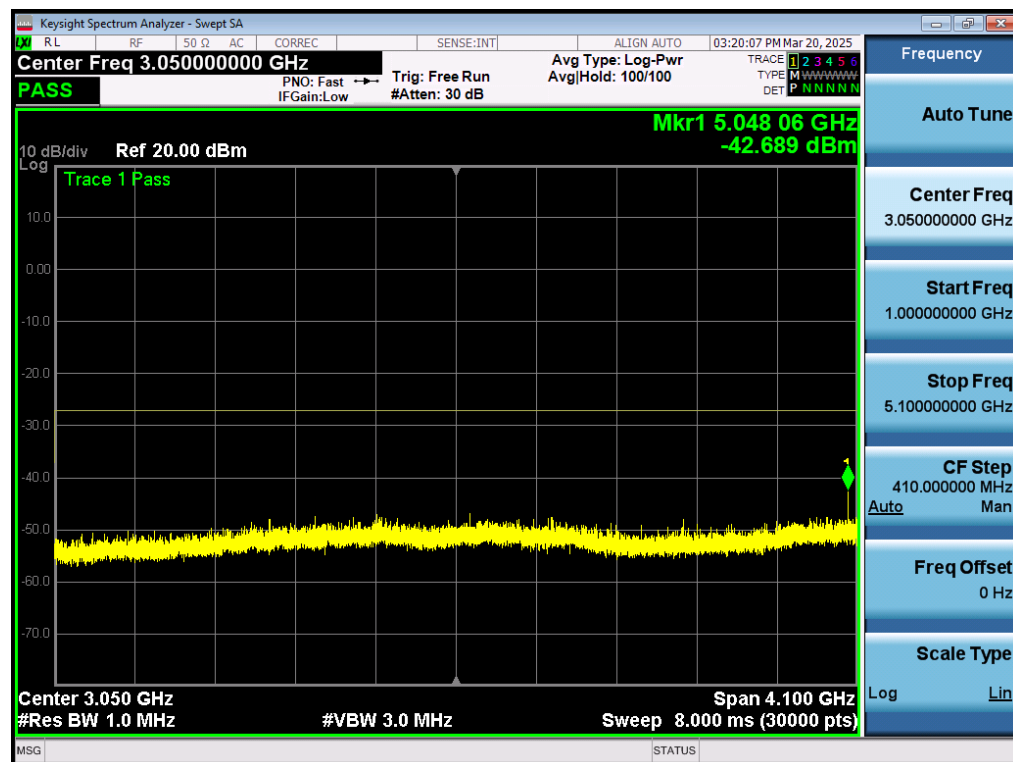
Test_Graph_802.11a_ANT1_5260_6Mbps_Frequency Band 2
