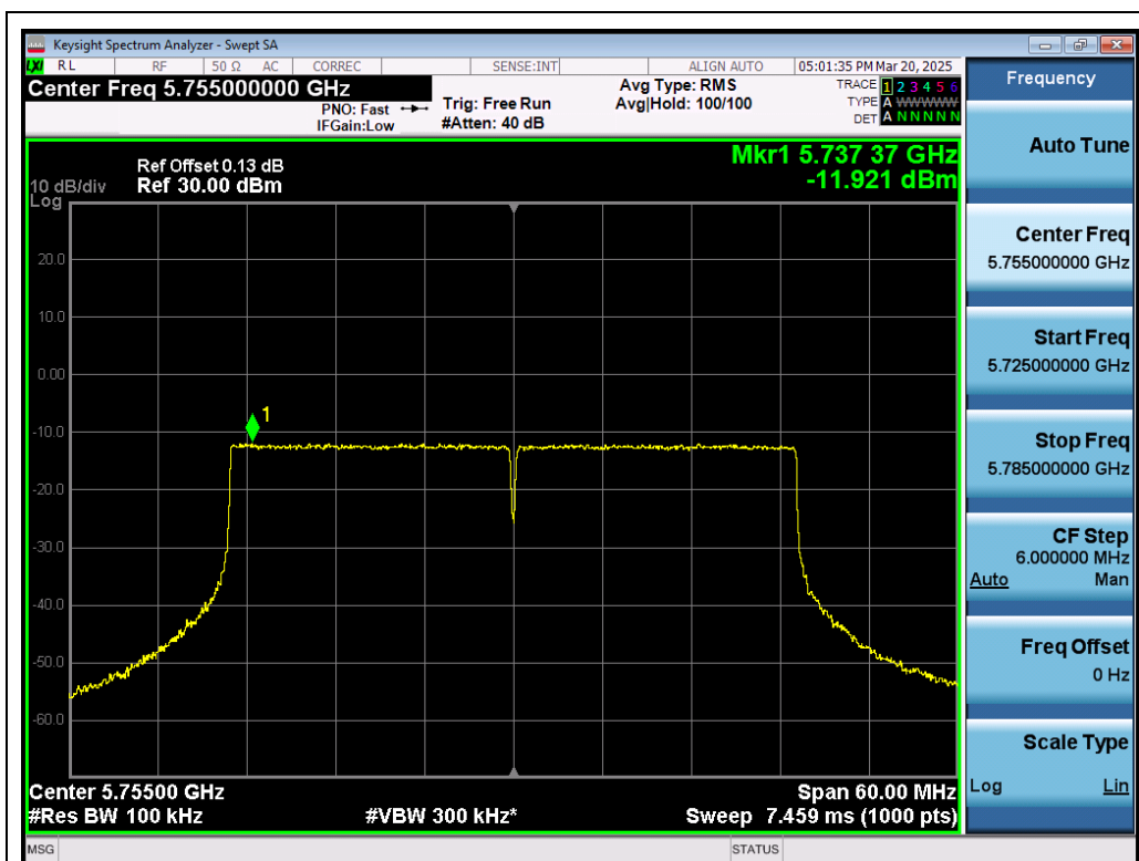
Test_Graph_802.11ax40_ANT1_5755_MCS0_PSD
