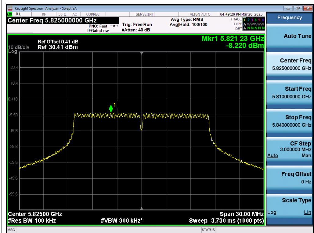
Test_Graph_802.11a_ANT1_5825_6Mbps_PSD
