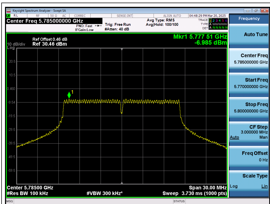
Test_Graph_802.11a_ANT1_5785_6Mbps_PSD
