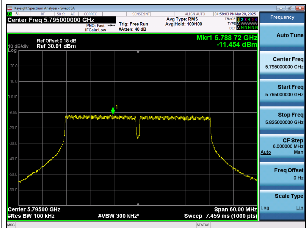
Test_Graph_802.11ac40_ANT1_5795_MCS0_PSD
