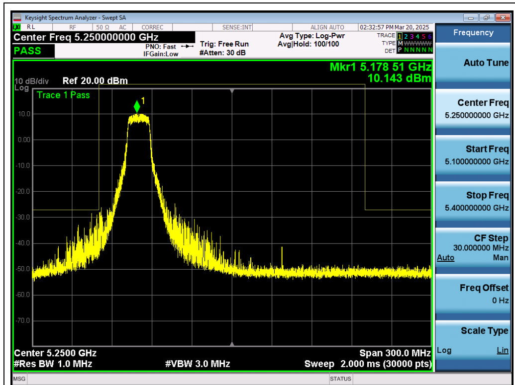
Test_Graph_802.11a_ANT1_5180_6Mbps_Frequency Band 3
