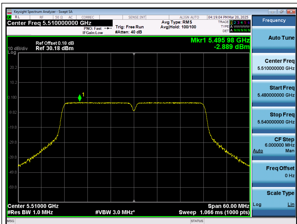
Test_Graph_802.11n40_ANT1_5510_MCS0_PSD
