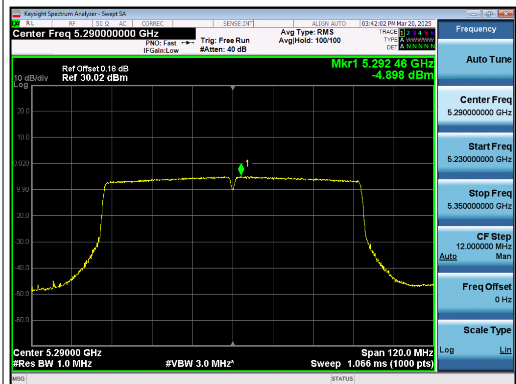
Test_Graph_802.11ac80_ANT1_5290_MCS0_PSD
