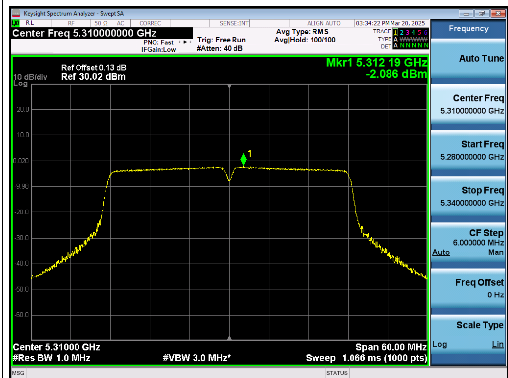
Test_Graph_802.11n40_ANT1_5310_MCS0_PSD
