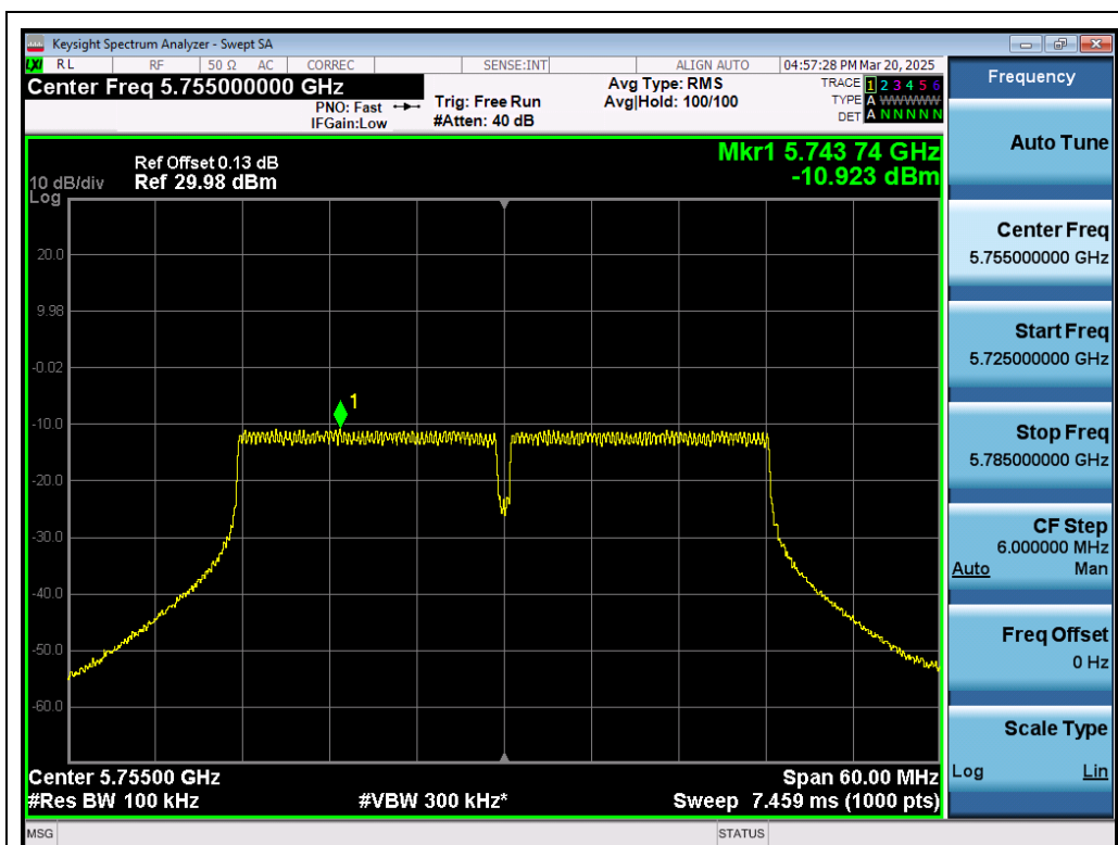
Test_Graph_802.11ac40_ANT1_5755_MCS0_PSD
