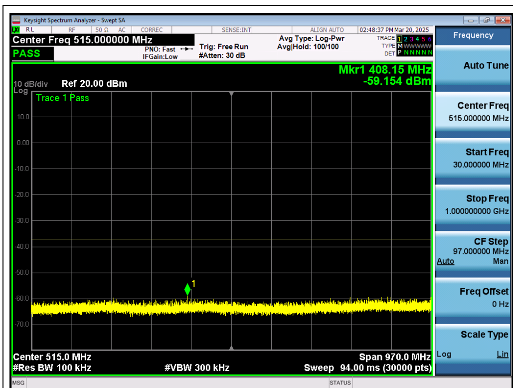
Test_Graph_802.11n40_ANT1_5230_MCS0_Frequency Band 1
