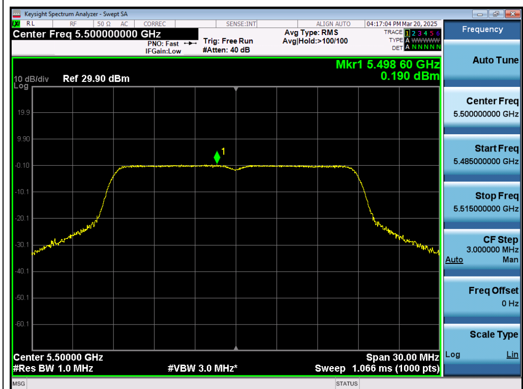
Test_Graph_802.11n20_ANT1_5500_MCS0_PSD
