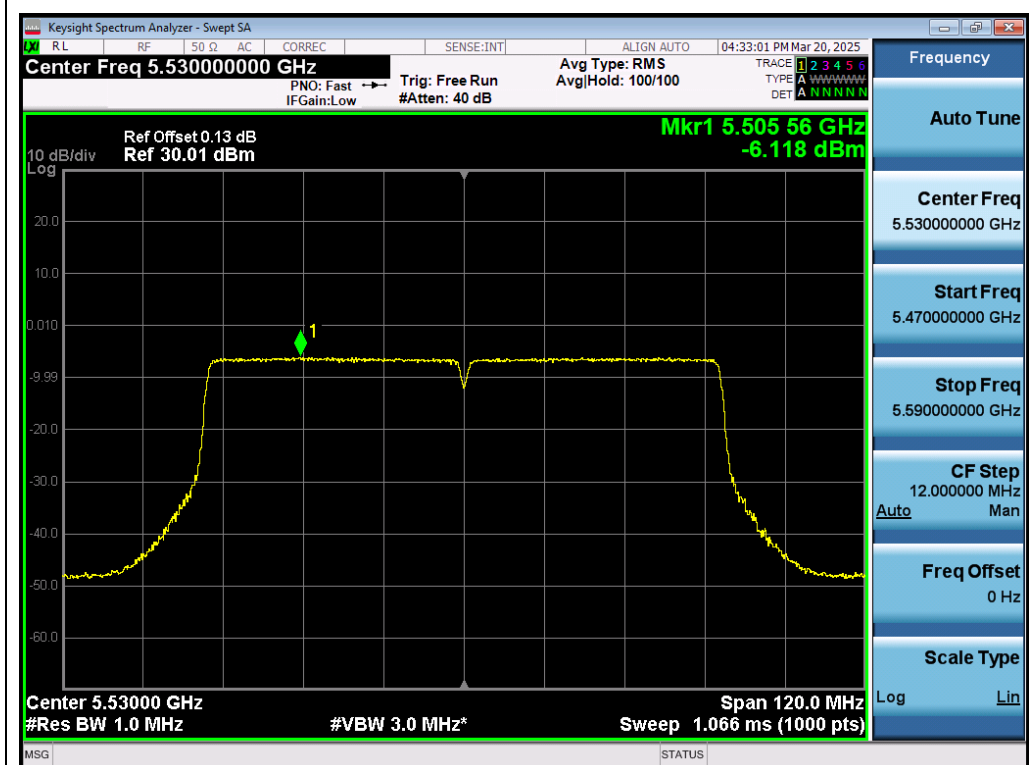
Test_Graph_802.11ac80_ANT1_5530_MCS0_PSD
