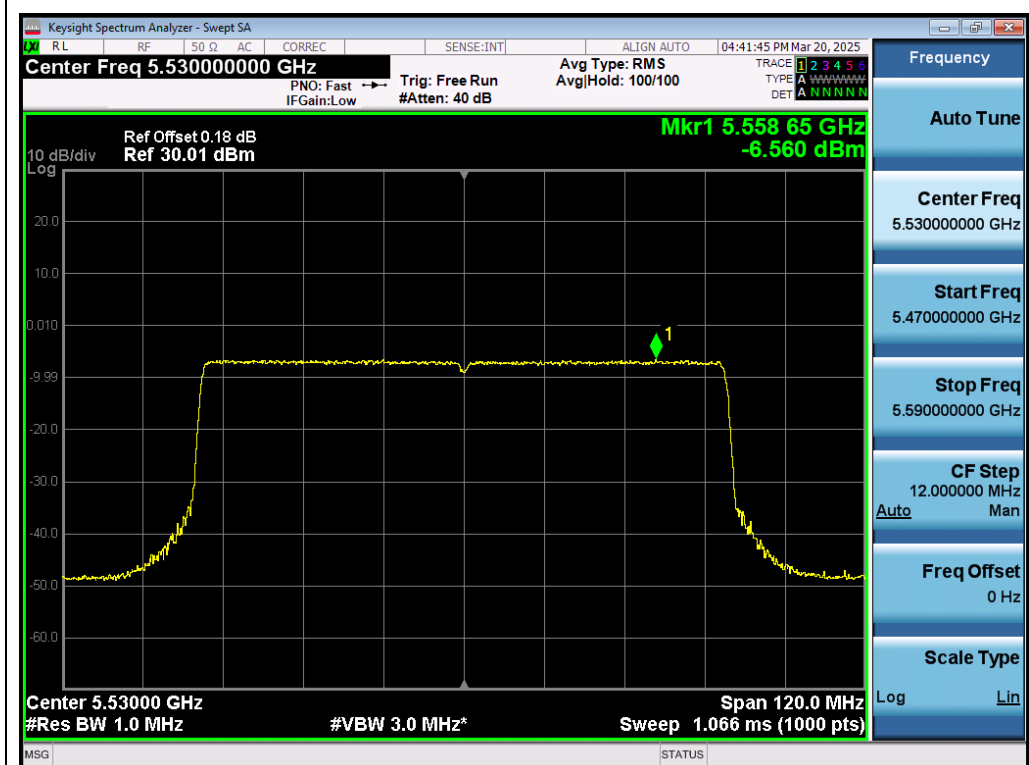
Test_Graph_802.11ax80_ANT1_5530_MCS0_PSD
