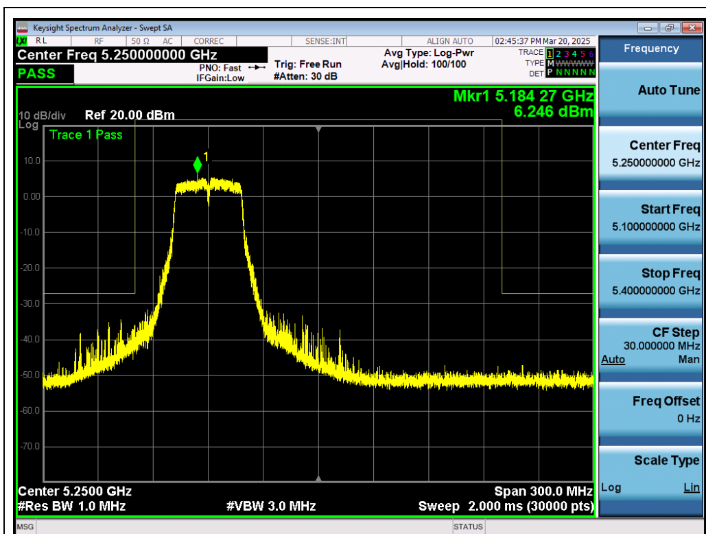
Test_Graph_802.11n40_ANT1_5190_MCS0_Frequency Band 3
