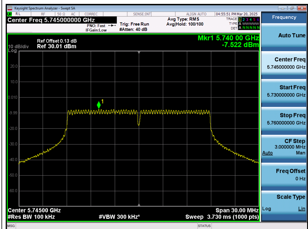
Test_Graph_802.11ac20_ANT1_5745_MCS0_PSD
