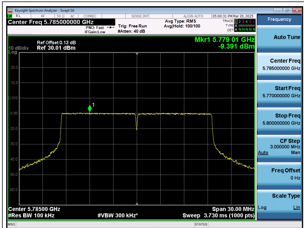
Test_Graph_802.11ax20_ANT1_5785_MCS0_PSD
