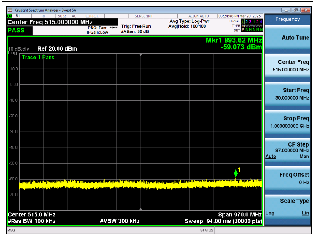
Test_Graph_802.11a_ANT1_5320_6Mbps_Frequency Band 1
