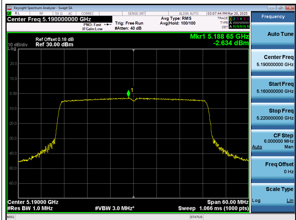
Test_Graph_802.11ax40_ANT1_5190_MCS0_PSD
