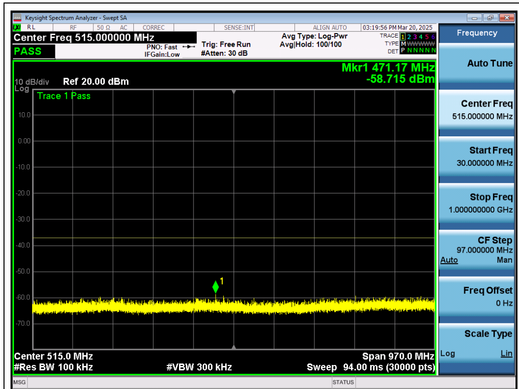
Test_Graph_802.11a_ANT1_5260_6Mbps_Frequency Band 1
