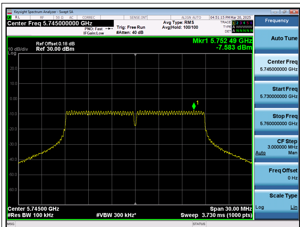
Test_Graph_802.11n20_ANT1_5745_MCS0_PSD
