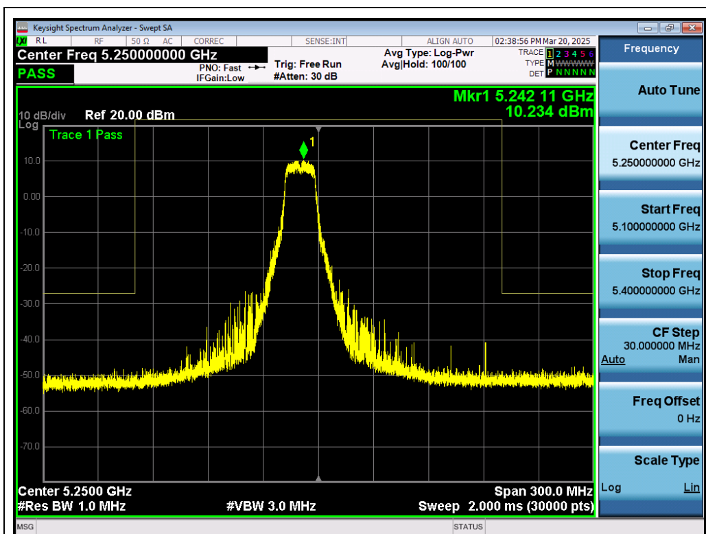
Test_Graph_802.11a_ANT1_5240_6Mbps_Frequency Band 3
