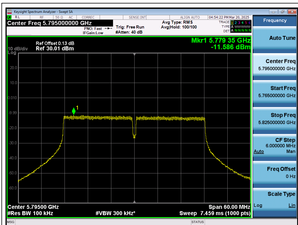
Test_Graph_802.11n40_ANT1_5795_MCS0_PSD
