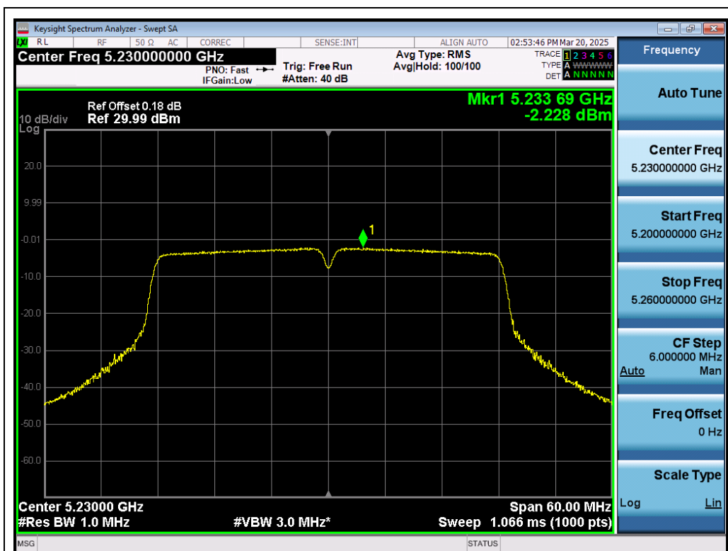
Test_Graph_802.11ac40_ANT1_5230_MCS0_PSD
