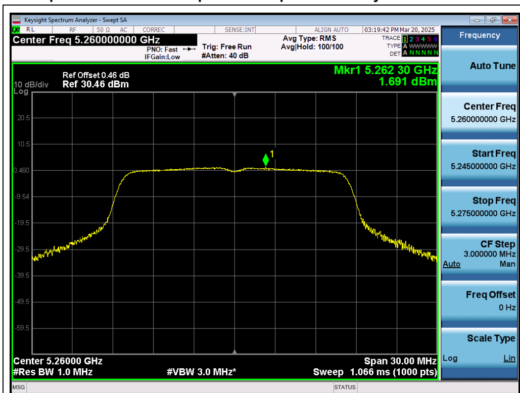
Test_Graph_802.11a_ANT1_5260_6Mbps_PSD
