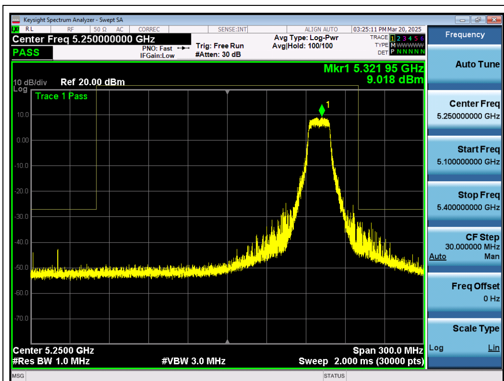
Test_Graph_802.11a_ANT1_5320_6Mbps_Frequency Band 3
