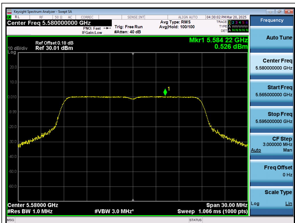
Test_Graph_802.11ac20_ANT1_5580_MCS0_PSD
