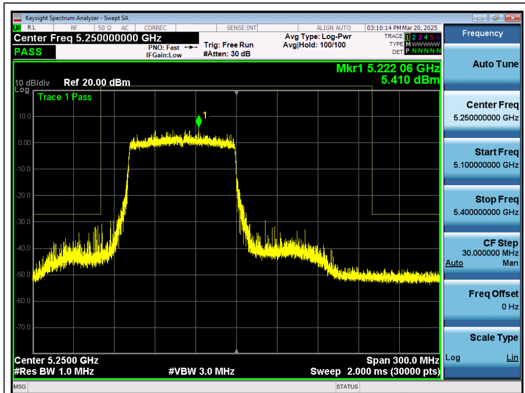
Test_Graph_802.11ax80_ANT1_5210_MCS0_Frequency Band 3
