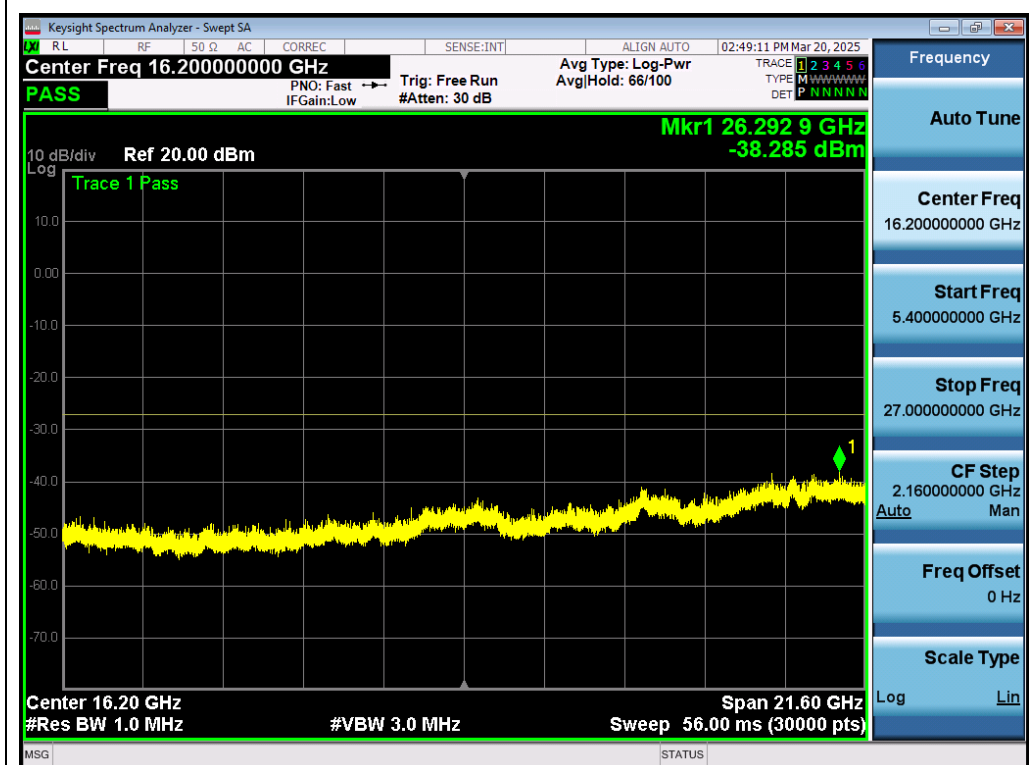
Test_Graph_802.11n40_ANT1_5230_MCS0_Frequency Band 4
