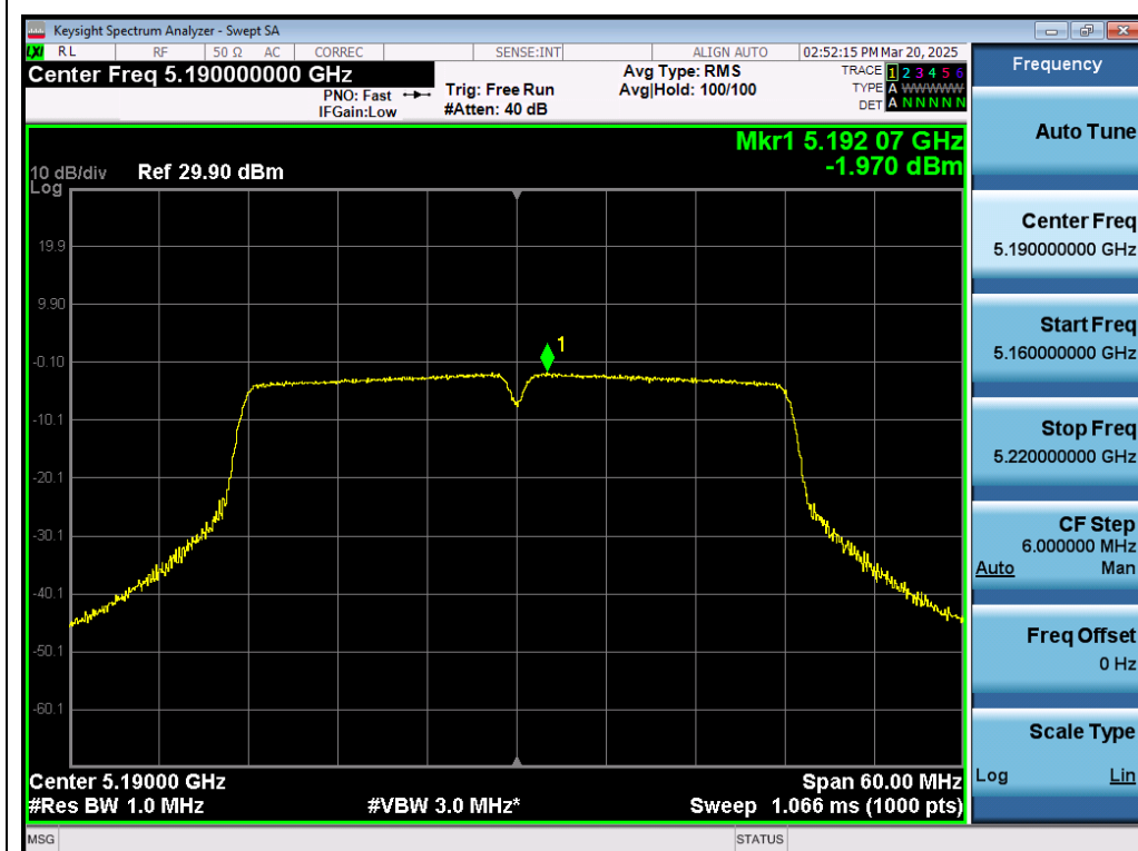
Test_Graph_802.11ac40_ANT1_5190_MCS0_PSD
