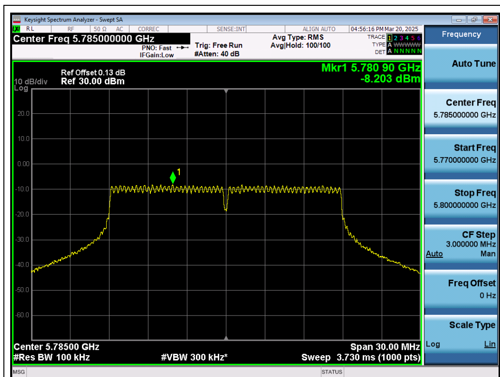
Test_Graph_802.11ac20_ANT1_5785_MCS0_PSD
