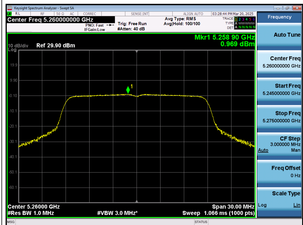
Test_Graph_802.11n20_ANT1_5260_MCS0_PSD
