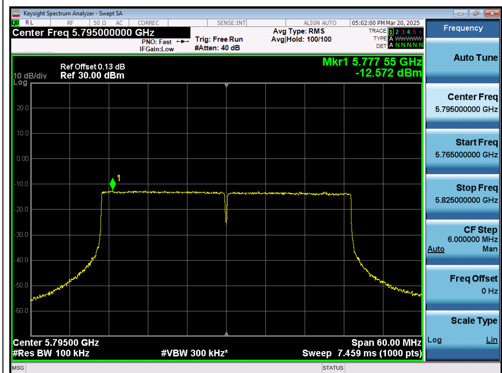
Test_Graph_802.11ax40_ANT1_5795_MCS0_PSD
