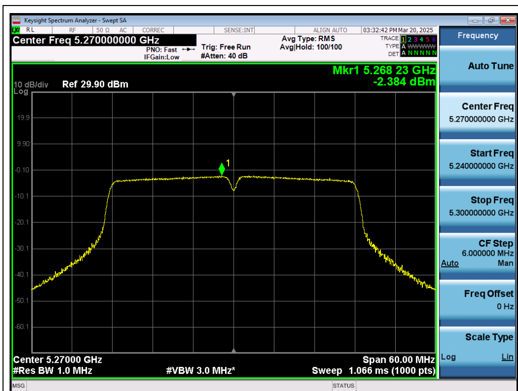
Test_Graph_802.11n40_ANT1_5270_MCS0_PSD
