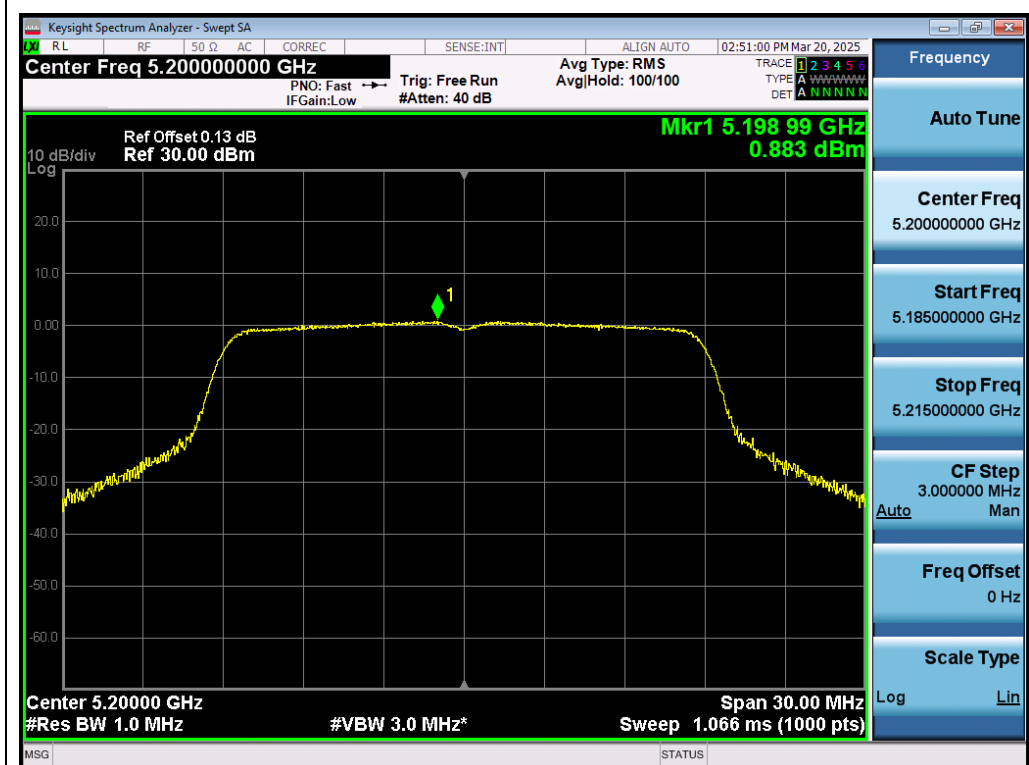
Test_Graph_802.11ac20_ANT1_5200_MCS0_PSD
