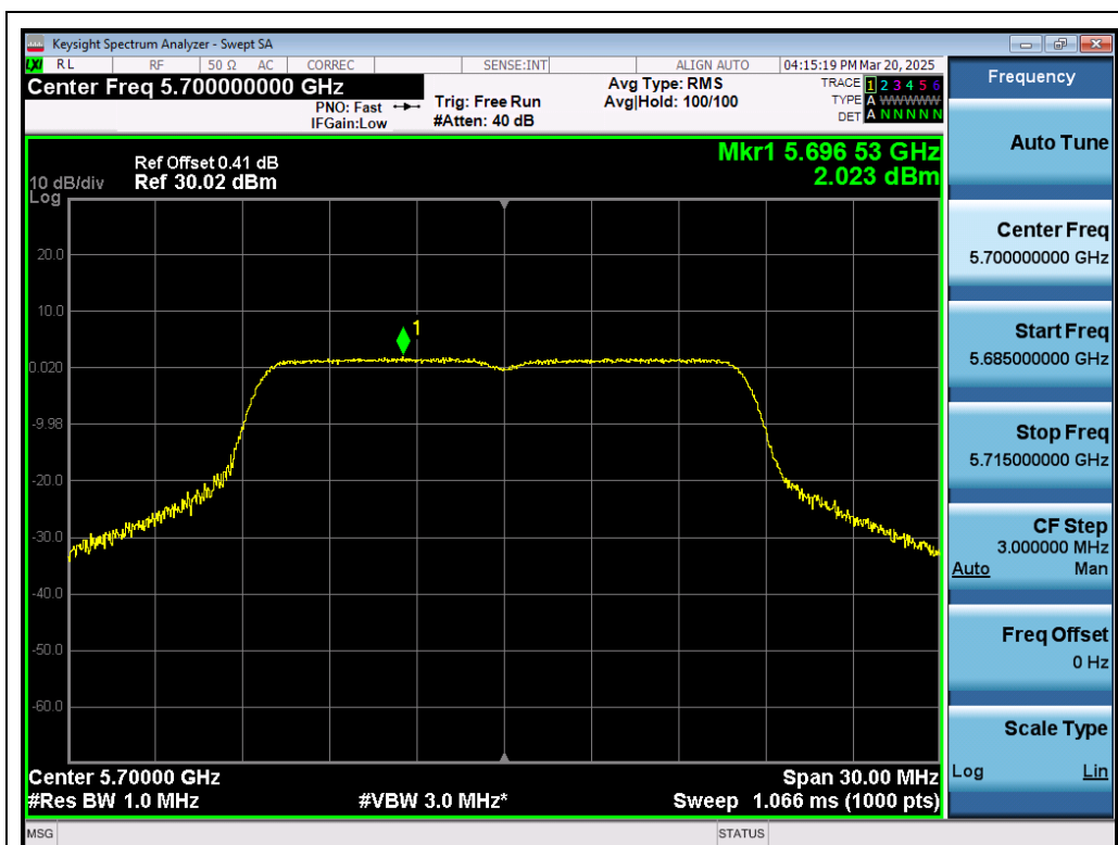
Test_Graph_802.11a_ANT1_5700_6Mbps_PSD
