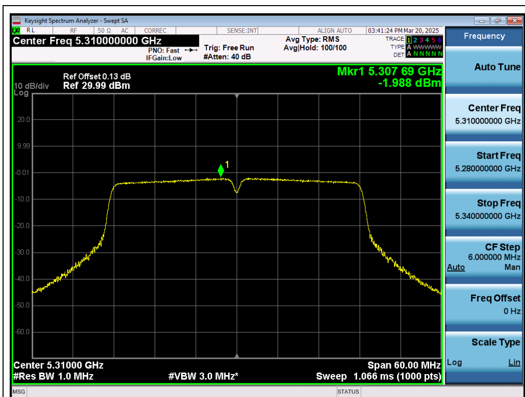
Test_Graph_802.11ac40_ANT1_5310_MCS0_PSD
