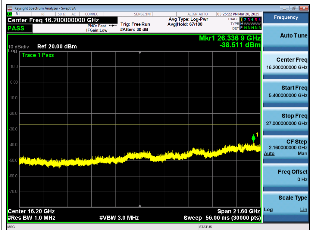
Test_Graph_802.11a_ANT1_5320_6Mbps_Frequency Band 4
