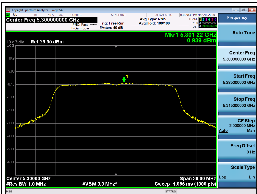
Test_Graph_802.11n20_ANT1_5300_MCS0_PSD
