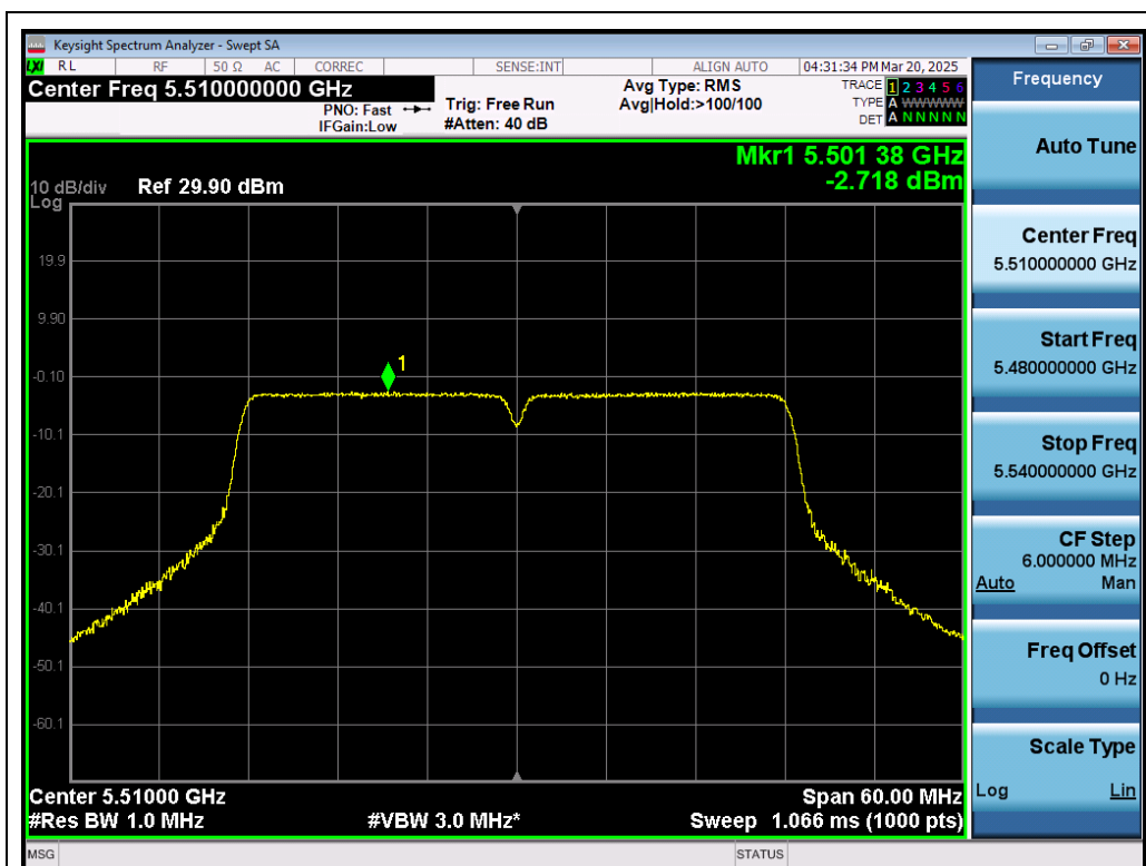
Test_Graph_802.11ac40_ANT1_5510_MCS0_PSD
