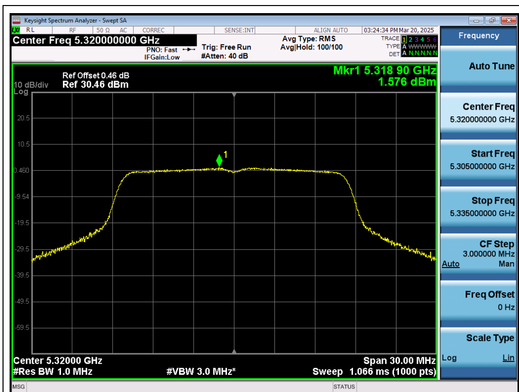
Test_Graph_802.11a_ANT1_5320_6Mbps_PSD
