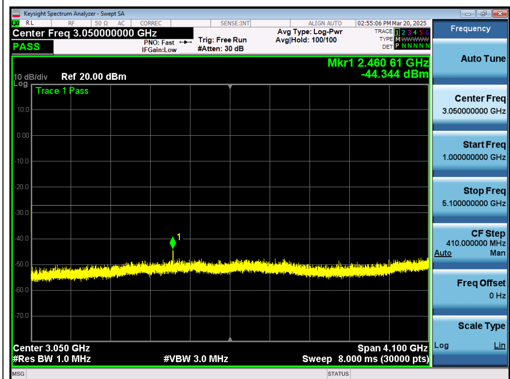
Test_Graph_802.11ac80_ANT1_5210_MCS0_Frequency Band 2
