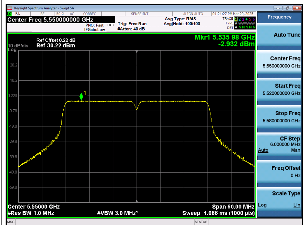
Test_Graph_802.11n40_ANT1_5550_MCS0_PSD
