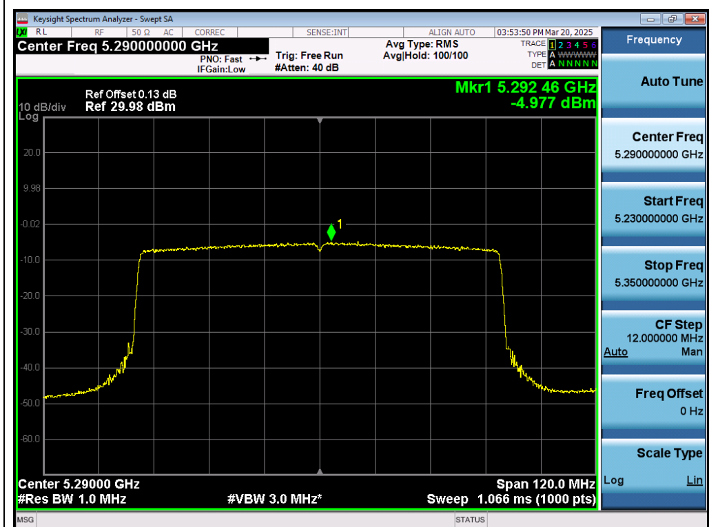
Test_Graph_802.11ax80_ANT1_5290_MCS0_PSD
