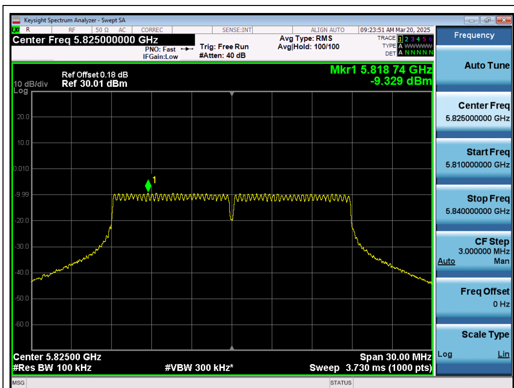
Test_Graph_802.11ac20_ANT1_5825_MCS0_PSD
