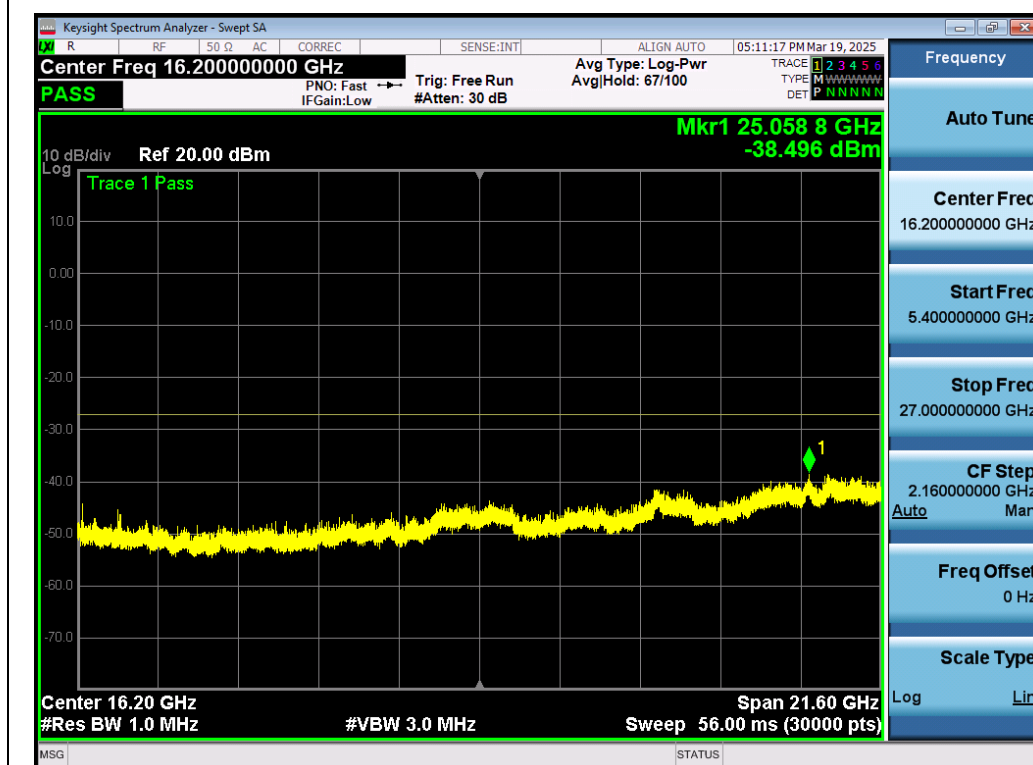
Test Graph 802.11ax80 ANT1 5210 MCS0 Frequency Band 4
