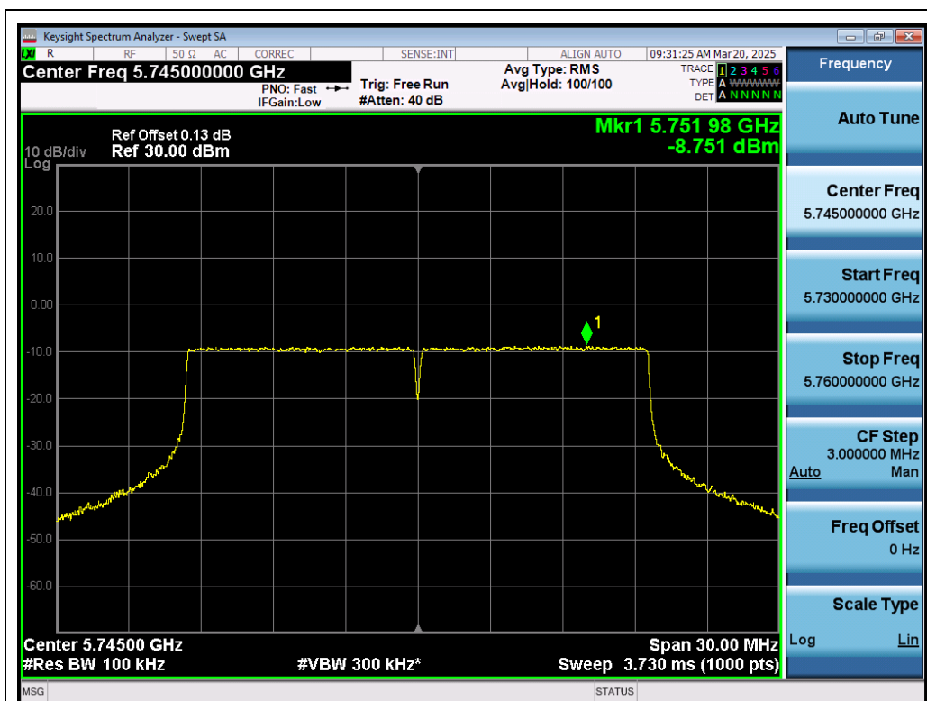
Test_Graph_802.11ax20_ANT1_5745_MCS0_PSD
