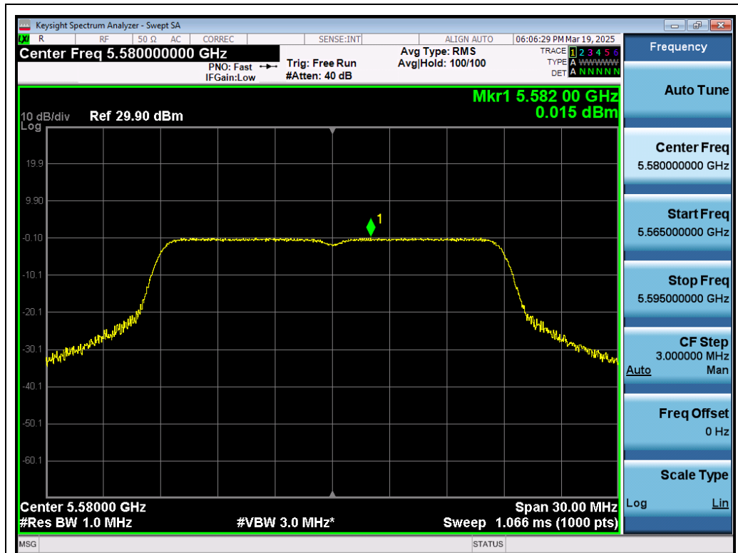
Test_Graph_802.11ac20_ANT1_5580_MCS0_PSD
