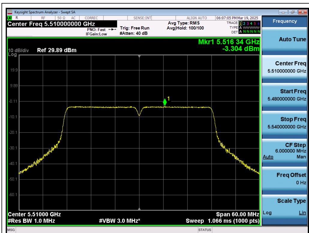
Test_Graph_802.11ac40_ANT1_5510_MCS0_PSD
