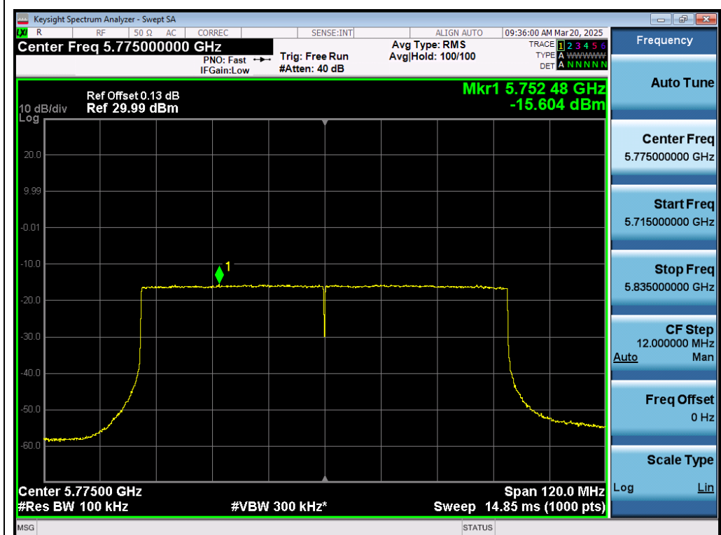
Test_Graph_802.11ax80_ANT1_5775_MCS0_PSD
