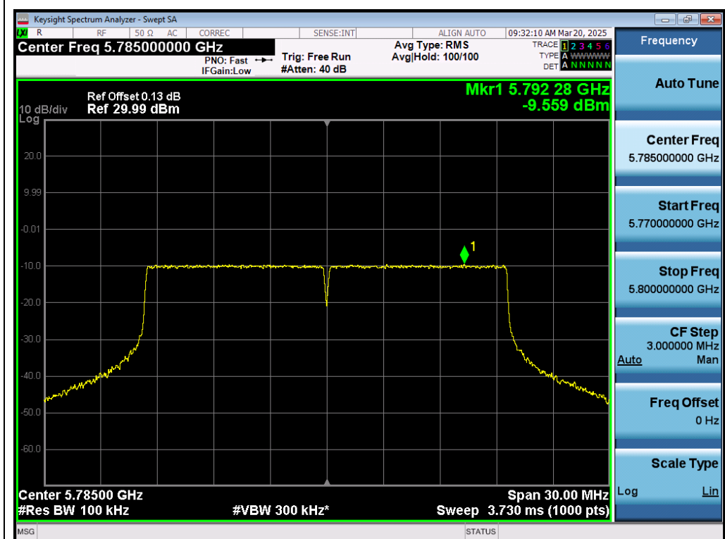
Test_Graph_802.11ax20_ANT1_5785_MCS0_PSD
