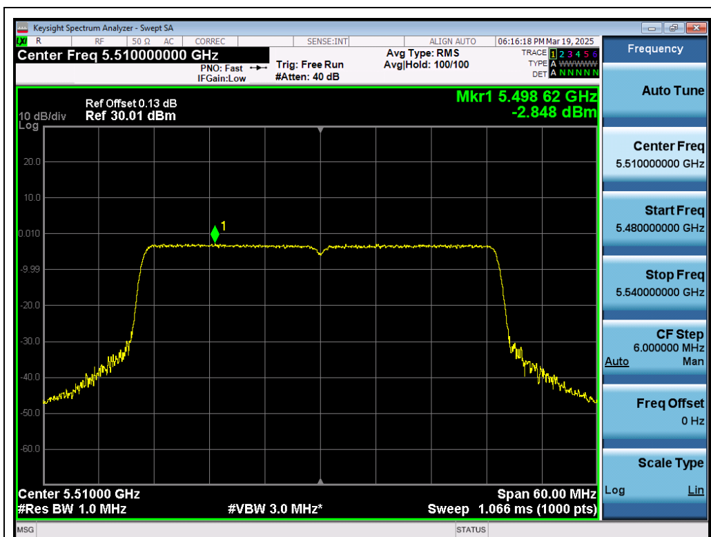
Test_Graph_802.11ax40_ANT1_5510_MCS0_PSD
