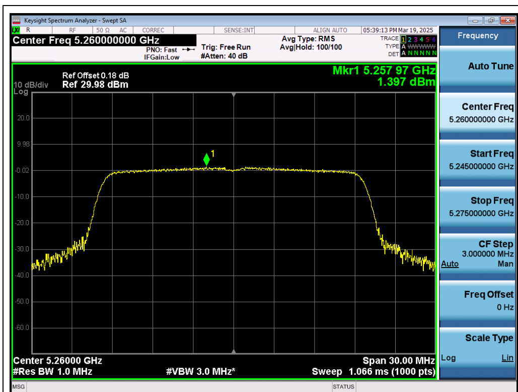
Test_Graph_802.11ax20_ANT1_5260_MCS0_PSD
