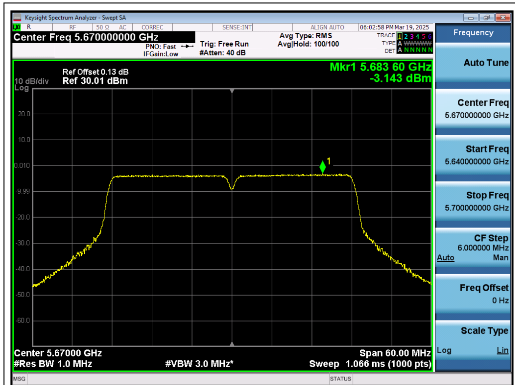
Test_Graph_802.11n40_ANT1_5670_MCS0_PSD
