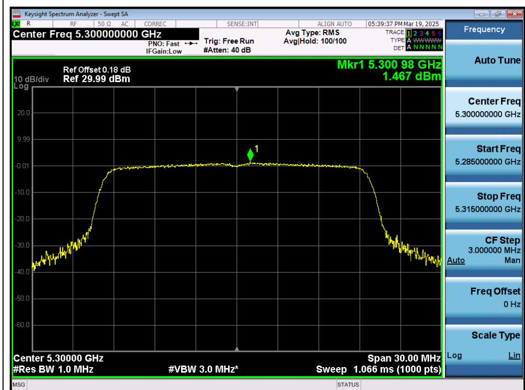
Test_Graph_802.11ax20_ANT1_5300_MCS0_PSD
