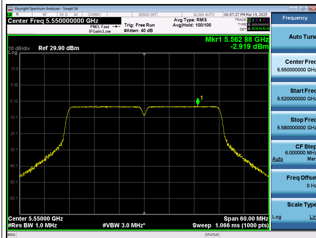
Test_Graph_802.11ac40_ANT1_5550_MCS0_PSD
