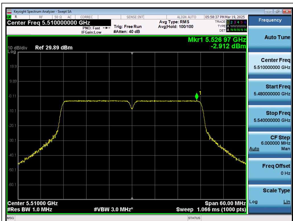
Test_Graph_802.11n40_ANT1_5510_MCS0_PSD
