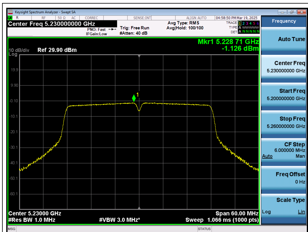
Test_Graph_802.11ac40_ANT1_5230_MCS0_PSD
