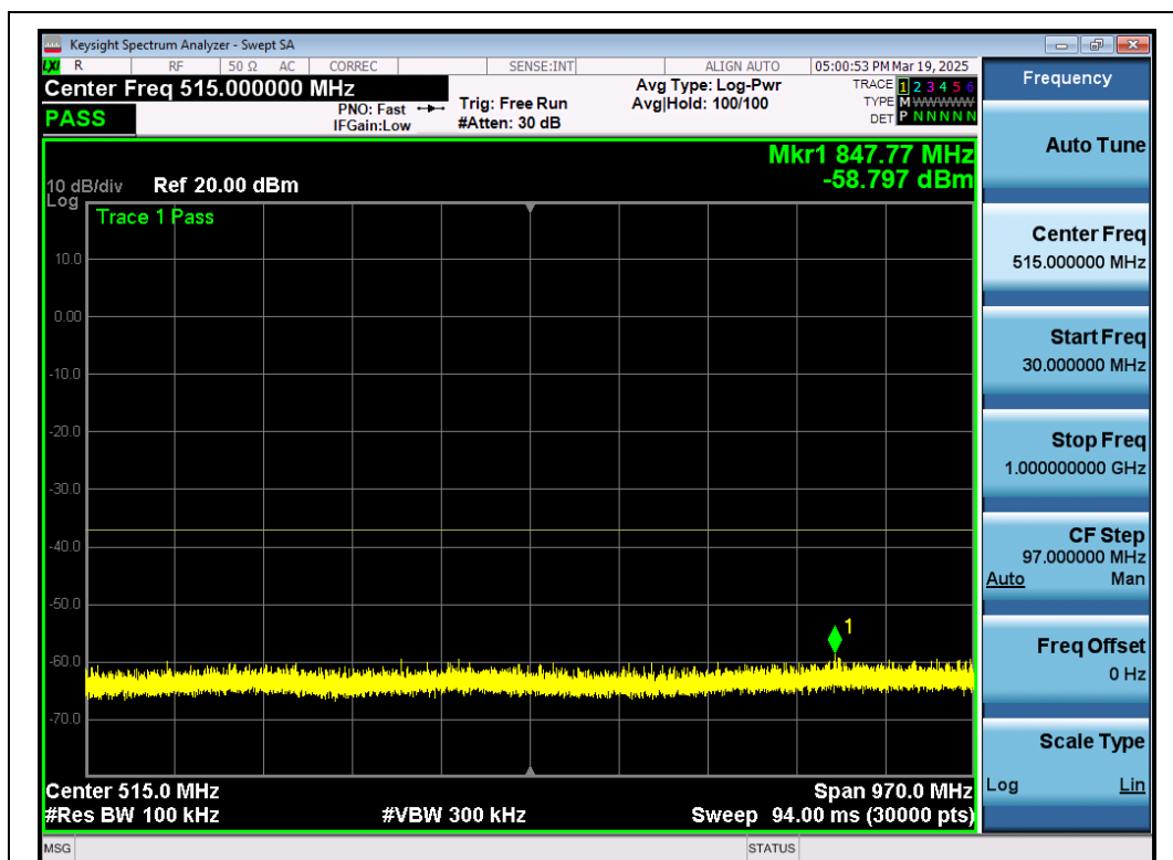
Test_Graph_802.11ac80_ANT1_5210_MCS0_Frequency Band 1
