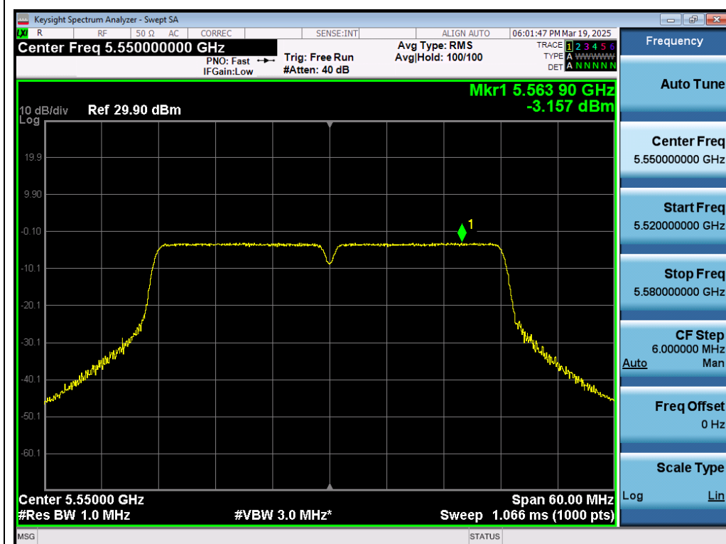
Test_Graph_802.11n40_ANT1_5550_MCS0_PSD
