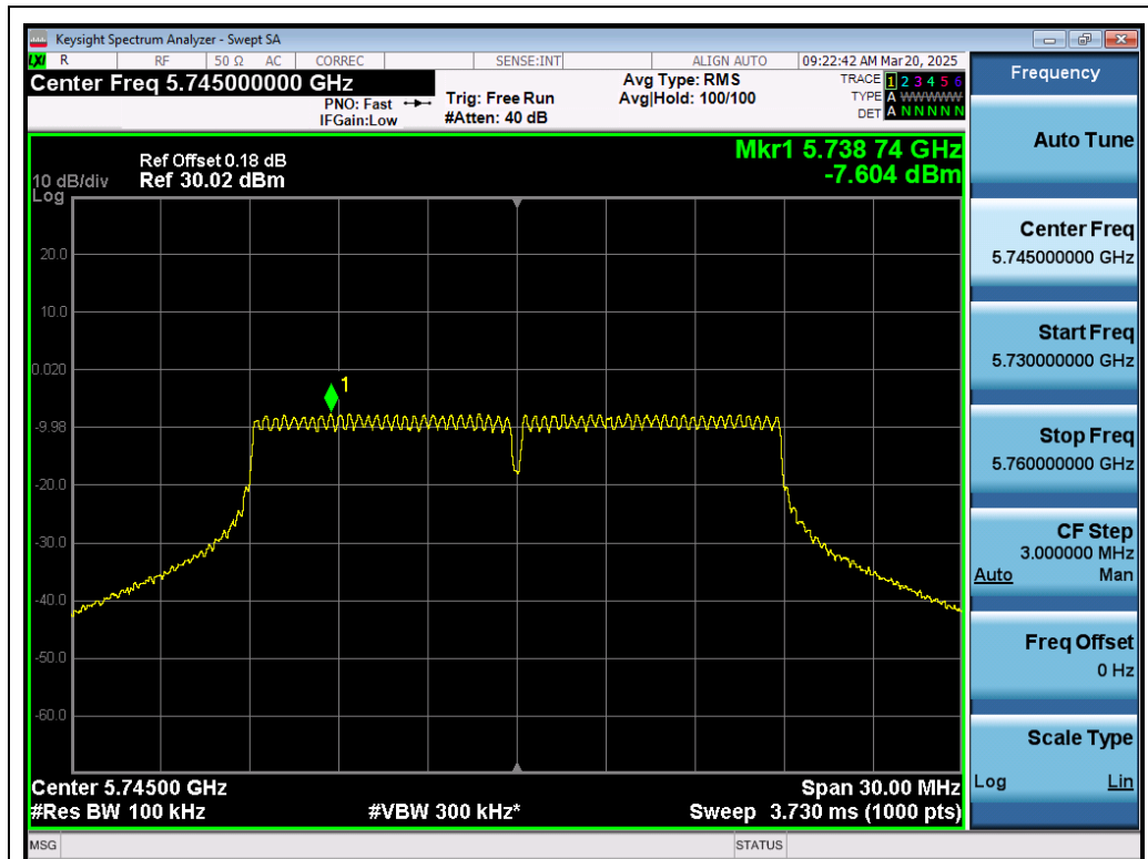
Test_Graph_802.11ac20_ANT1_5745_MCS0_PSD
