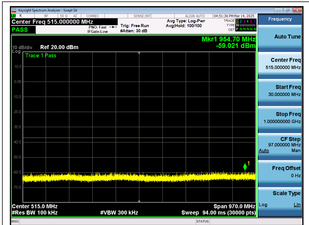
Test_Graph_802.11n40_ANT1_5190_MCS0_Frequency Band 1
