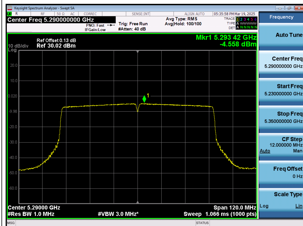
Test_Graph_802.11ac80_ANT1_5290_MCS0_PSD
