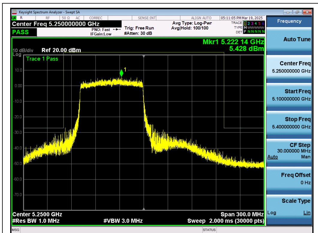
Test Graph 802.11ax80 ANT1 5210 MCS0 Frequency Band 3
