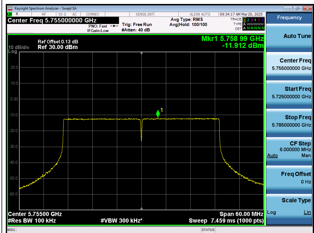
Test_Graph_802.11ax40_ANT1_5755_MCS0_PSD
