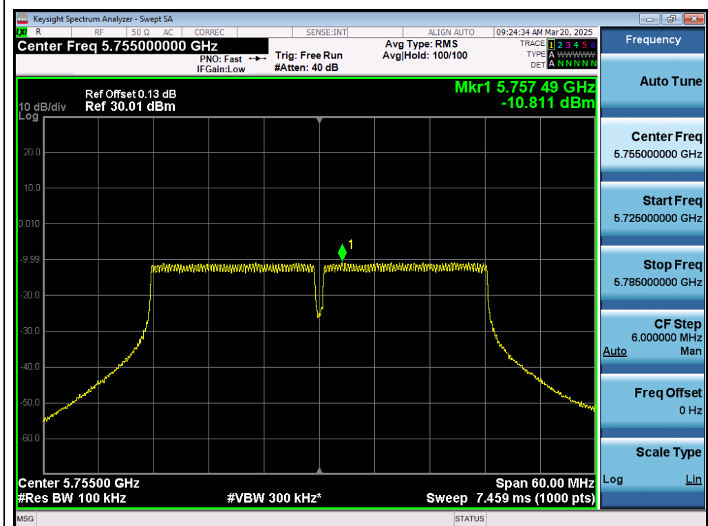
Test_Graph_802.11ac40_ANT1_5755_MCS0_PSD
