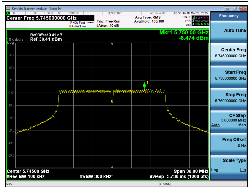
Test_Graph_802.11a_ANT1_5745_6Mbps_PSD
