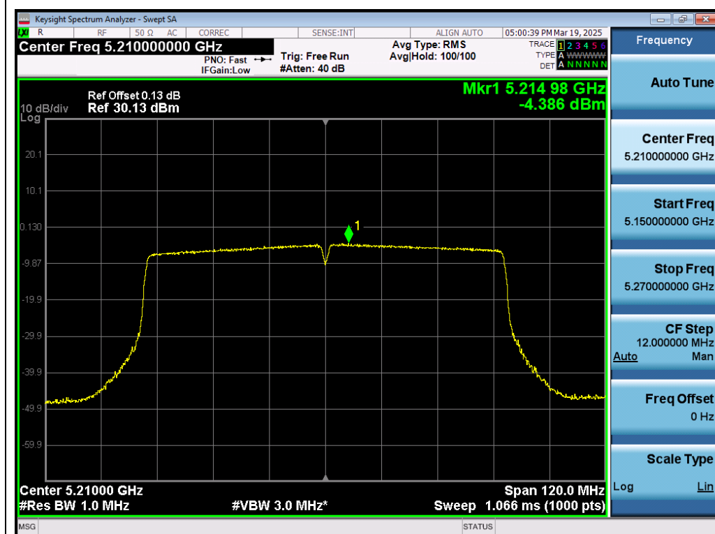
Test_Graph_802.11ac80_ANT1_5210_MCS0_PSD
