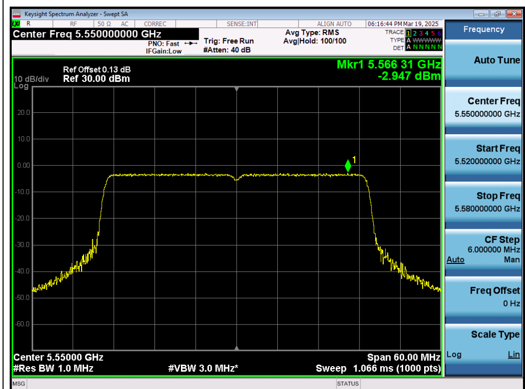
Test_Graph_802.11ax40_ANT1_5550_MCS0_PSD
