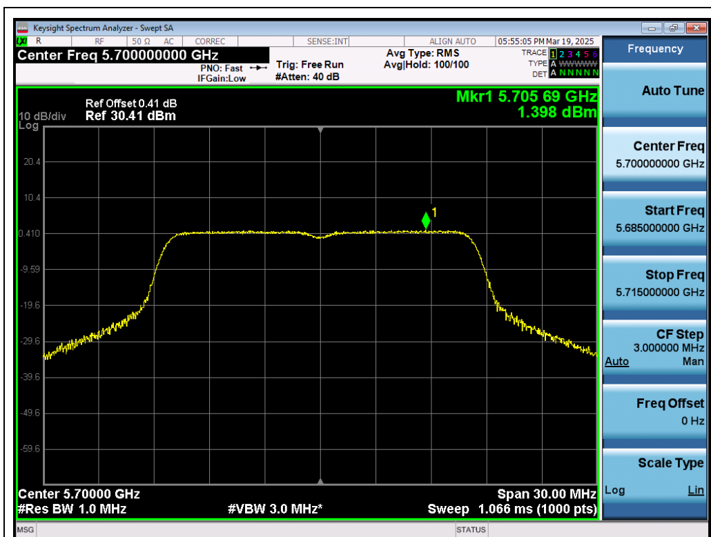
Test_Graph_802.11a_ANT1_5700_6Mbps_PSD
