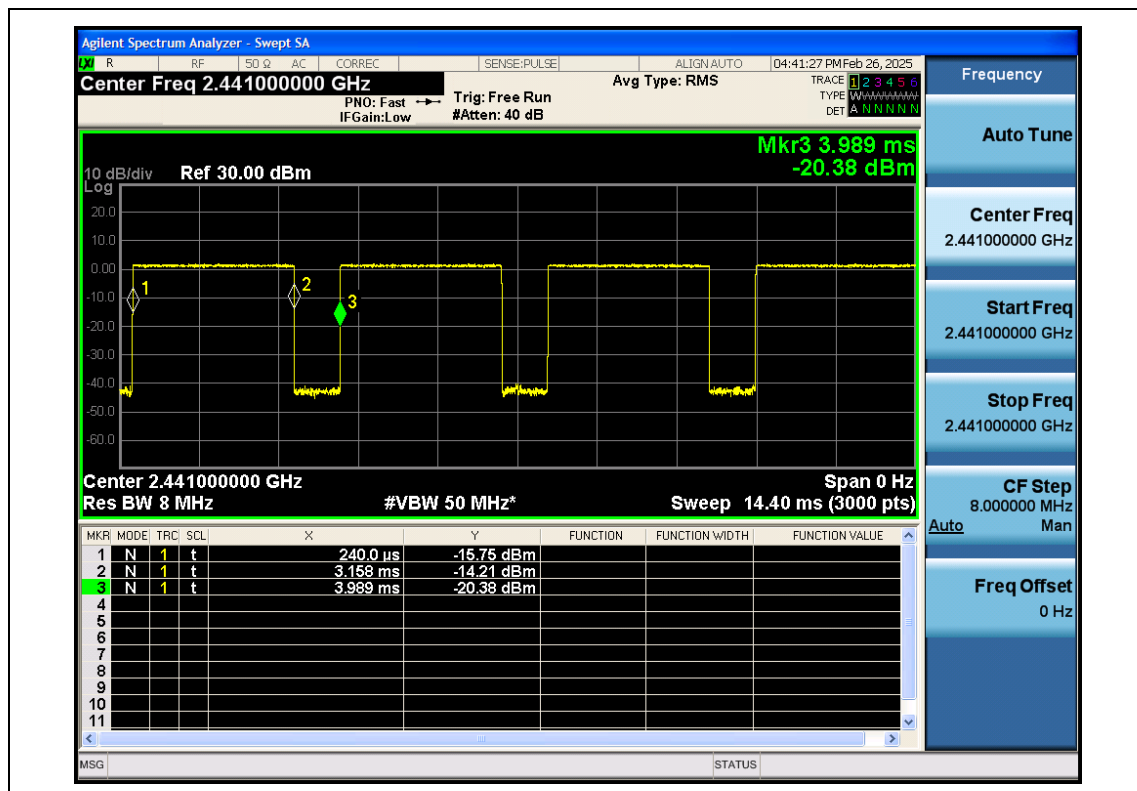
EDR-π /4-DQPSK-ANT1-2441
