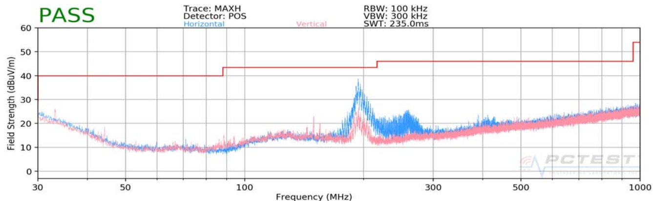
Plot 7-63. Radiated Spurious Plot below 1GHz
