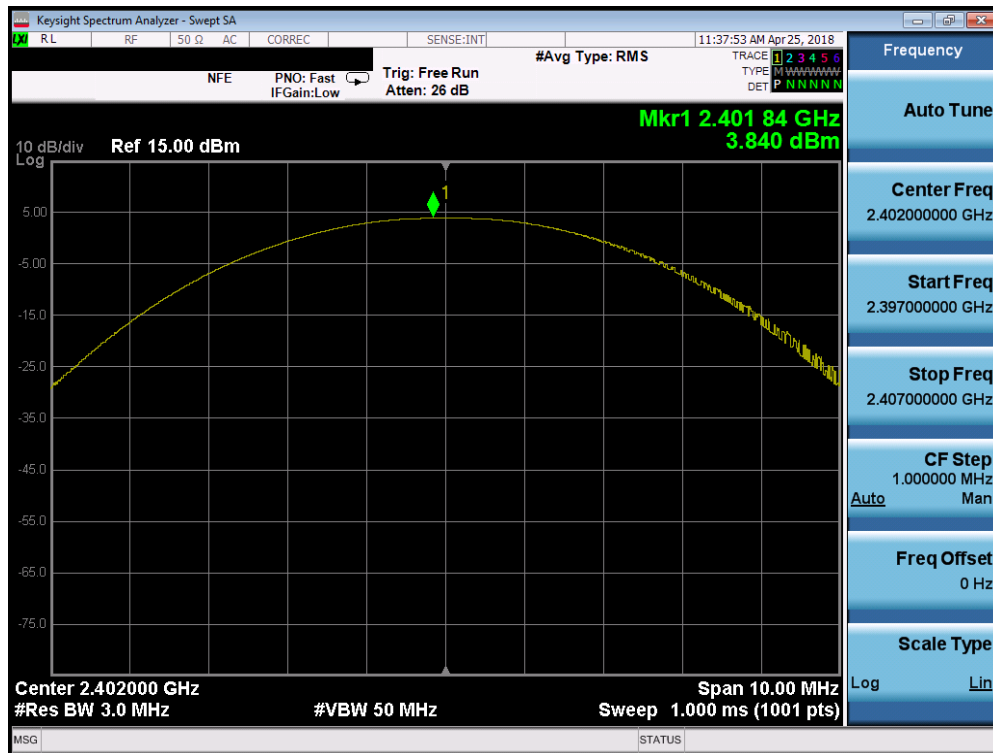
Plot 7-13. Peak Power Plot (Bluetooth (LE), 1Mbps – Ch. 0)
