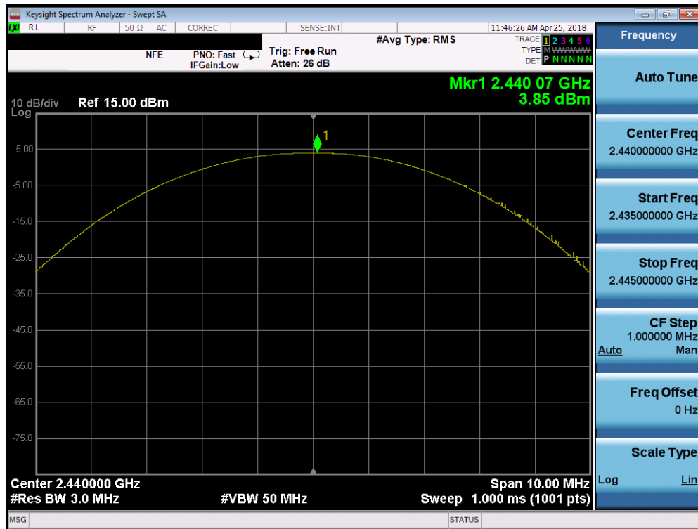
Plot 7-11. Peak Power Plot (Bluetooth (LE), 250kbps – Ch. 19)
