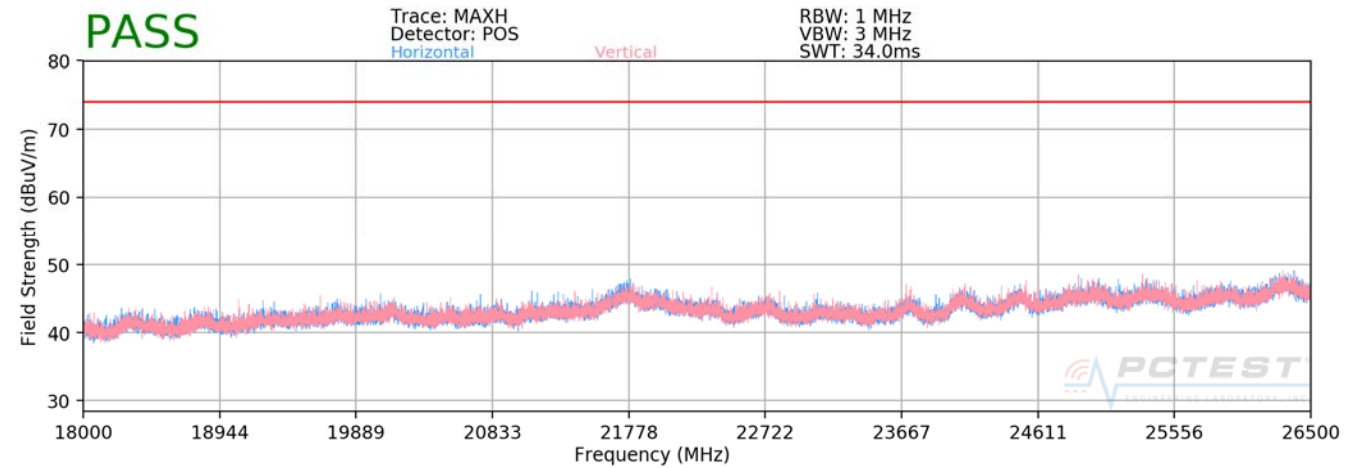
Plot 7-58. Radiated Spurious Plot above 18GHz
