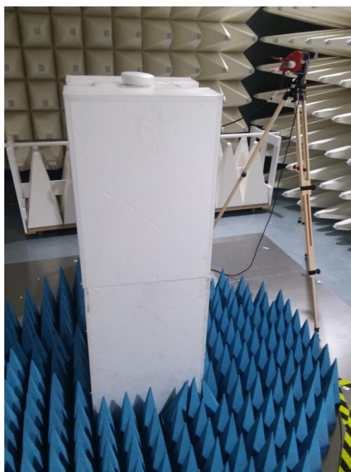
Fig B4. High Range measurement setup using Horn Antenna
