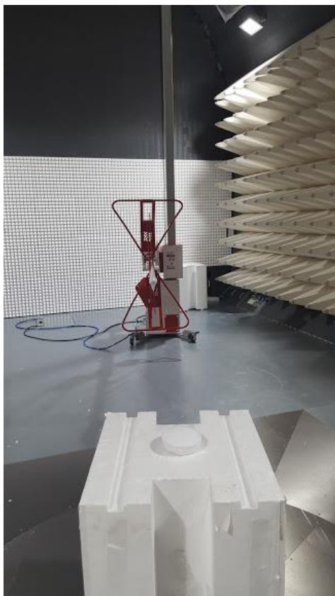
Fig B3. Low Range measurement setup using Biconical Antenna
