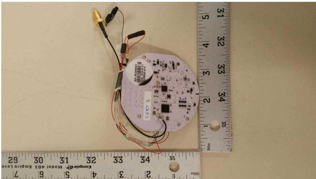
Figure B2. Conducted DUT Rear view
