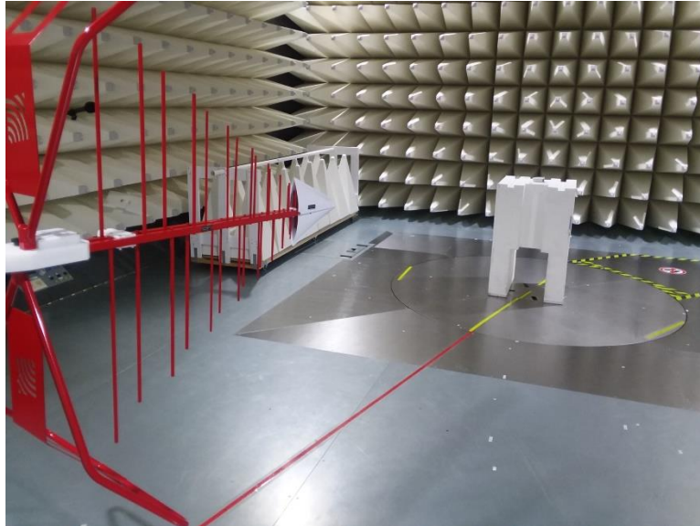
Figure B5. Radiated Setup – Low Range.
