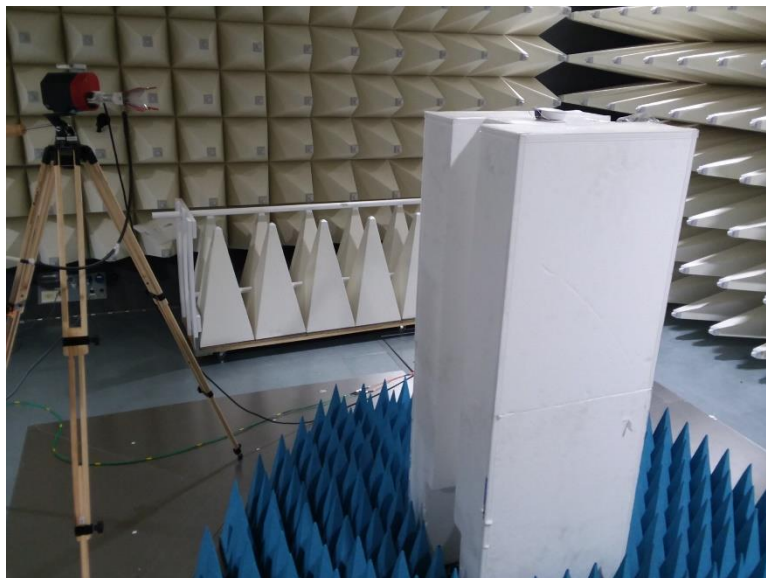
Figure B6. Radiated Setup – High Range.
