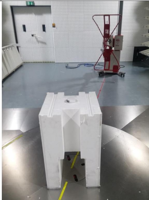
Figure B5. Radiated Setup – Low Range
