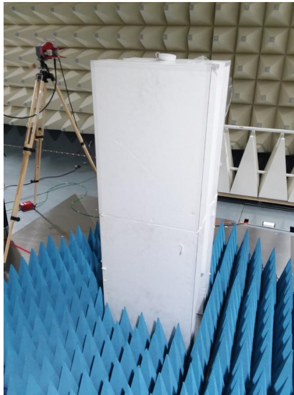
Figure B6. Radiated Setup – High Range.
