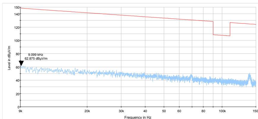
Plot 7.7.2 Radiated emission measurements from 9 to 150 kHz at the mid carrier frequency
