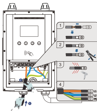
Single Charge Coupler Input Wiring
