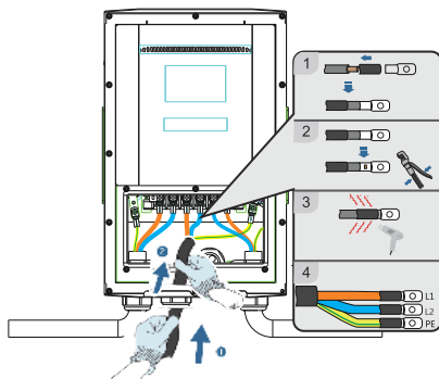
Dual Charge Coupler Input Wiring
