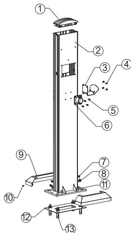
Schematic Diagram of Column Decomposition
