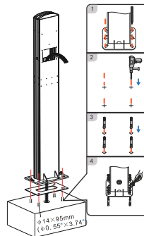
2 Fixed column
