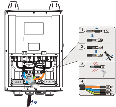
Single Charge Coupler Input Wiring
