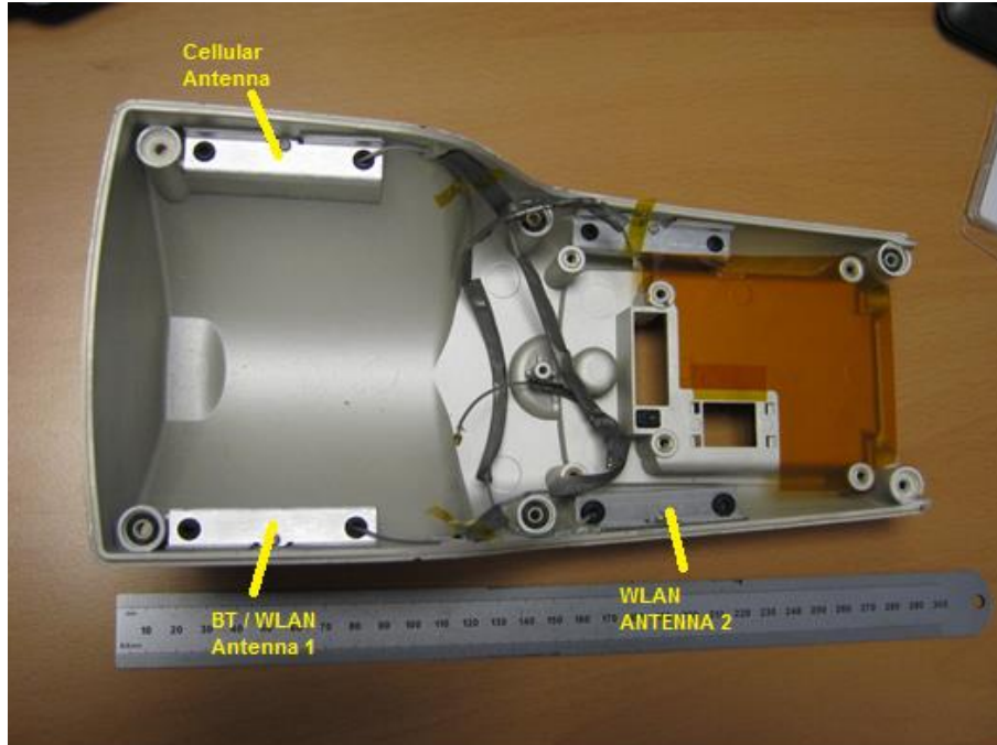
Antenna Locations
