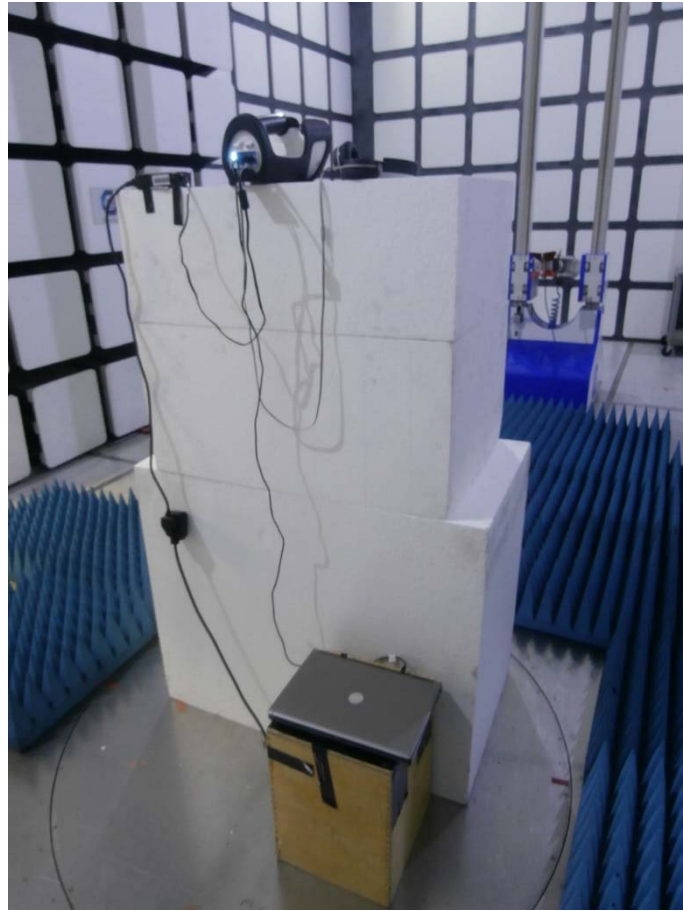
Radiated Emission – 8 GHz to 18 GHz
