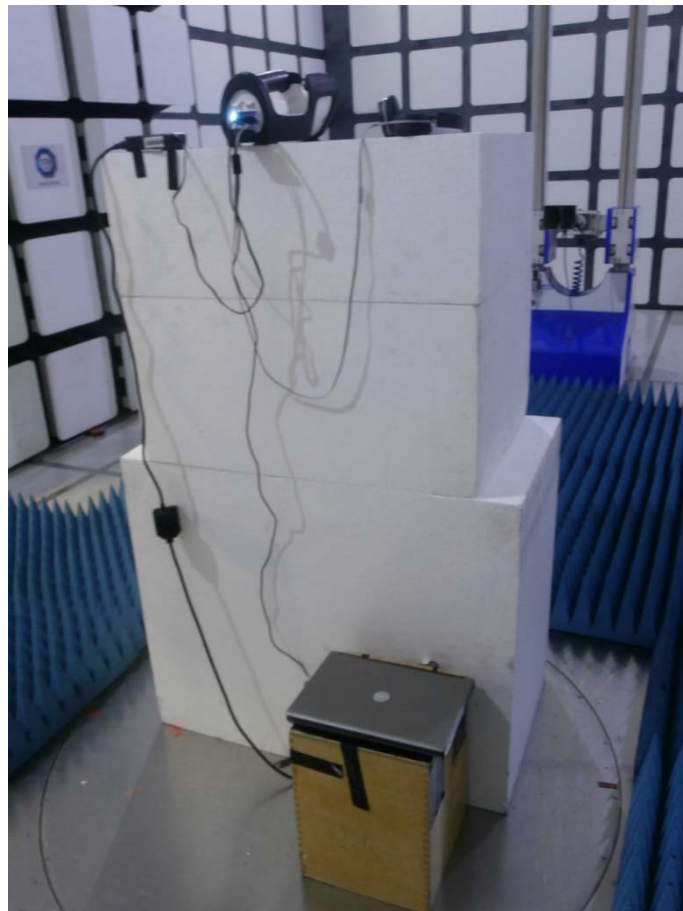
Radiated Emission – 1 GHz to 8 GHz
