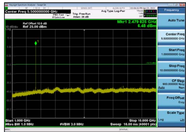
Conducted Emission: 8DPSK,2480,3DH5 ,1000MHz~10000MHz
