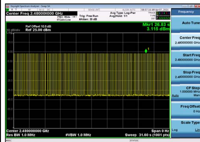
GFSK,2480,DH5,Transmission Number
