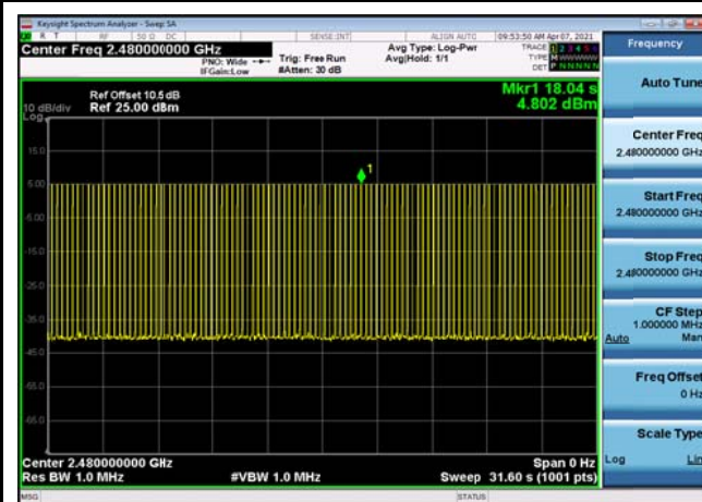
DQPSK,2480,2DH5,Transmission Number
