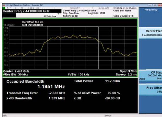
99% Bandwidth: DQPSK,2441MHz,2DH5
