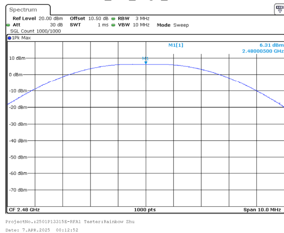
BLE_2M_High_Channel
