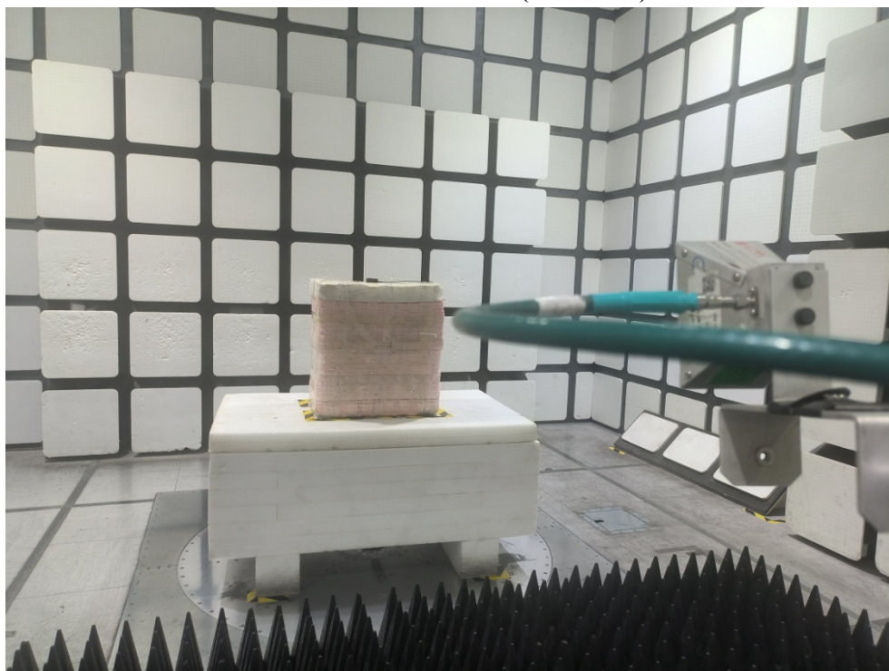
Radiated Emissions View (18-25 GHz)
