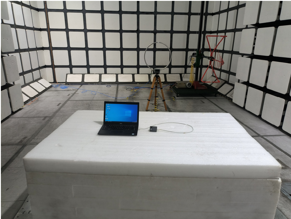
Radiated Emissions View (Below 30MHz)
