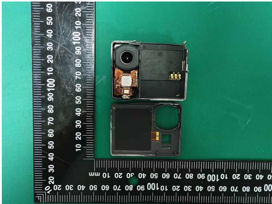
NFC ANT(RX only)
