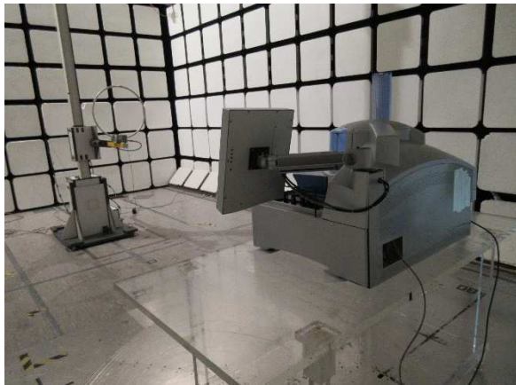
Radio-frequency radiated emissions (9k-30MHz)
