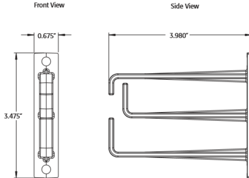
Figure 4-2: Sensus Cable Support Fingers
