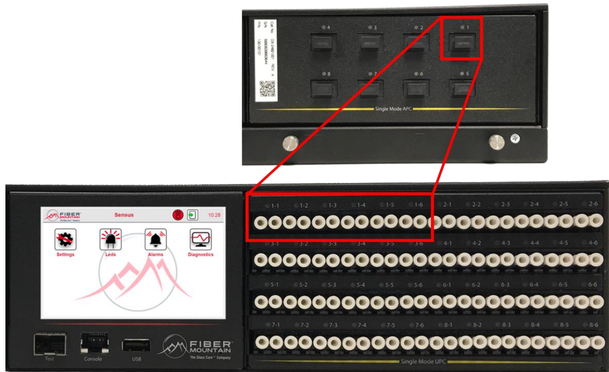
Figure 5-1: 96xLC to 8xMPO-12 Port Mapping
