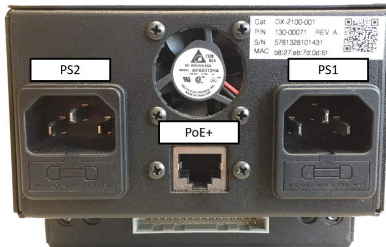
Figure 4-6 Sensus Management Module Power Sources
