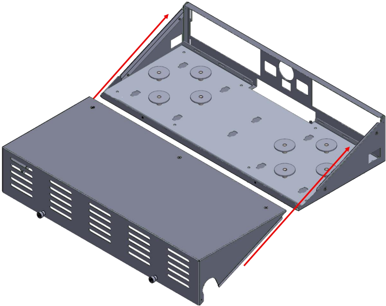
Figure 4-5: Installing LC-to-LC Extension Cover
